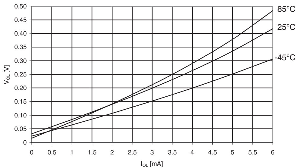
Figure 31-459. ATmega649P: I/O pin output voltage vs. sink current, port B ( V_{CC} = 1.8V ).
