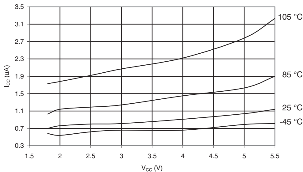
Figure 32-13. ATmega169PA-105°C: Power-save Supply Current vs. V_{CC} (Watchdog Timer Disabled)
