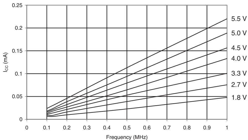
Figure 32-6. ATmega169PA-105°C: Idle Supply Current vs. Frequency (0.1 - 1.0MHz)
