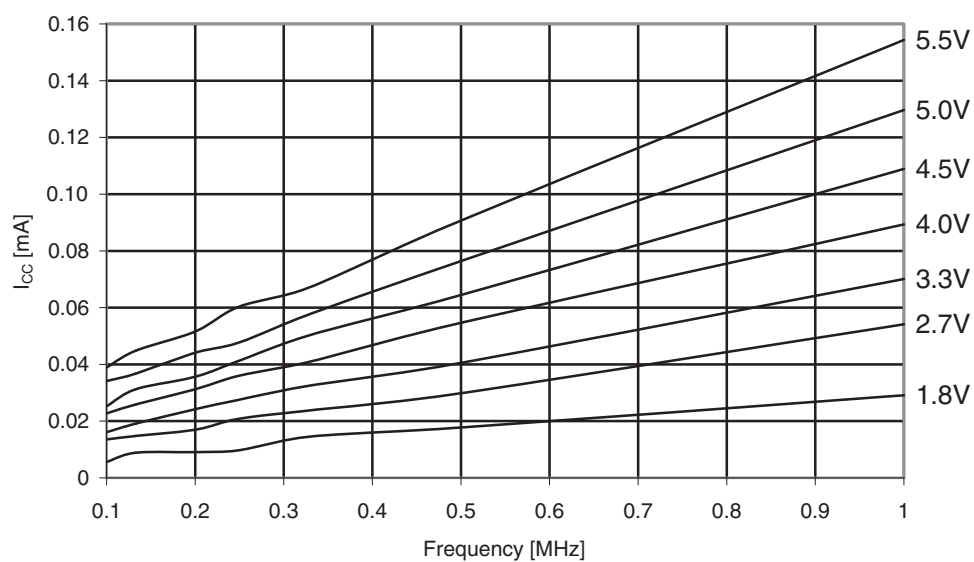
Figure 31-60. ATmega169A: Reset supply current vs. V_{CC} (0.1 - 1.0MHz, excluding current through the reset pull-up).
