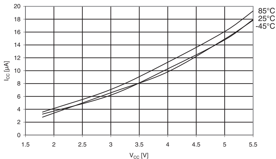
Figure 31-74. ATmega169PA: Power-down supply current vs. V_{CC} (Watchdog Timer enabled).
