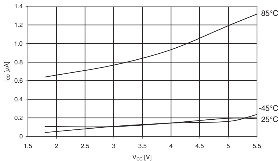
Figure 31-73. Atmel ATmega169PA: Power-down supply current vs. V_{CC} (Watchdog Timer disabled).
