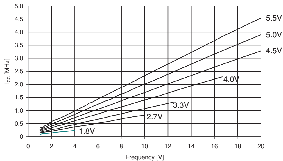
Figure 31-131. Atmel ATmega329A: Idle supply current vs. frequency (1 - 20MHz).
