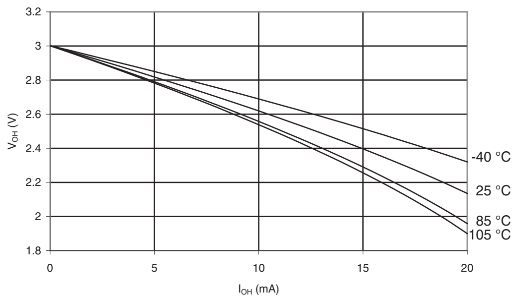
Figure 32-143. ATmega329P-105°C: I/O Pin Output Voltage vs. Source Current, Ports A,C,D,E,F,G ( V_{CC} = 3V )
