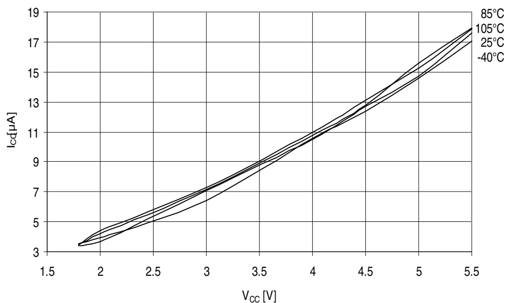
Figure 32-230. ATmega329PA - 105°C: Watchdog Timer Current vs. V_{CC}
