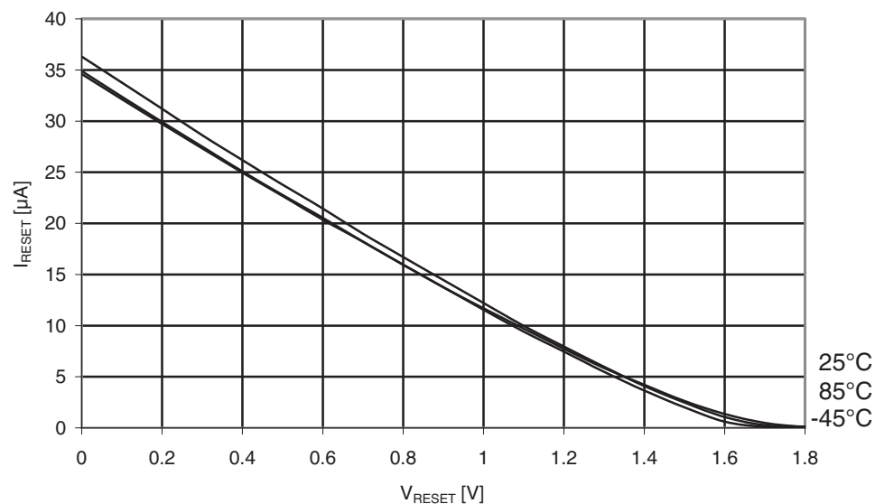
Figure 31-83. Atmel ATmega169PA: Reset pull-up resistor current vs. Reset pin voltage ( V_{CC} = 1.8V ).
