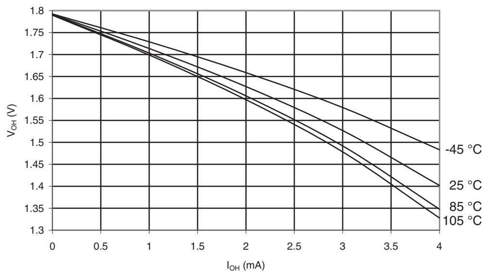
Figure 32-23. ATmega169PA-105°C: I/O Pin Output Voltage vs. Source Current, Ports A, C, D, E, F, G ( V_{CC} = 1.8V )
