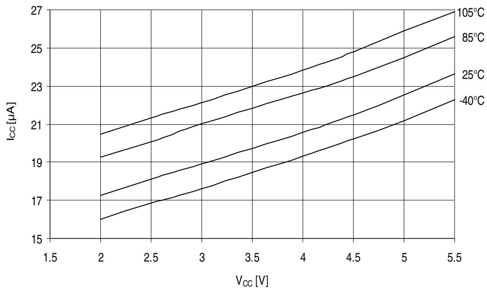
Figure 32-287. ATmega3290A - 105°C: Brownout Detector Current vs. V_{CC}
