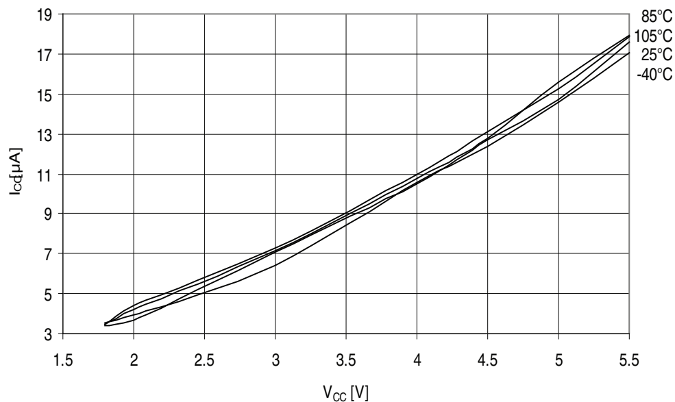
Figure 32-115. ATmega329A - 105°C: Watchdog Timer Current vs. V_{CC}
