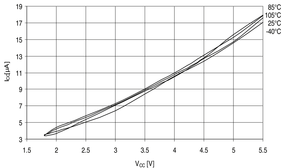
Figure 32-409. ATmega3290PA - 105°C: Watchdog Timer Current vs. V_{CC}
