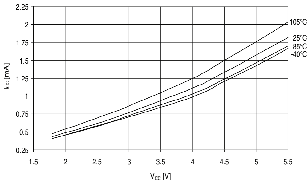
Figure 32-66. ATmega329A - 105°C: Idle Supply Current vs. V_{CC} (Internal RC Oscillator, 8 MHz)
