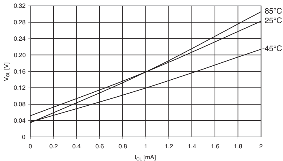
Figure 31-579. ATmega6490P: I/O pin output voltage vs. sink current, port B ( V_{CC} = 5V ).
