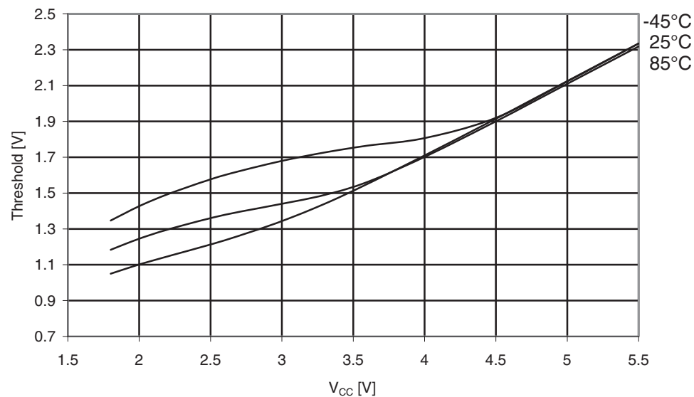
Figure 31-37. Atmel ATmega169A: Reset input Threshold voltage vs. V_{CC} ( V_{IH} , reset pin read as “1”).
