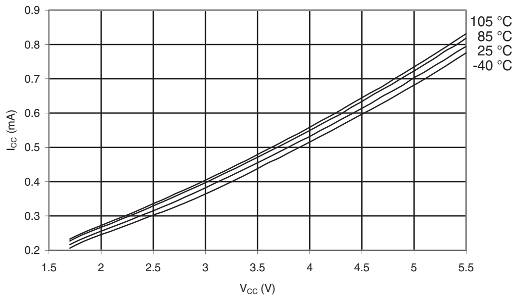
Figure 32-130. ATmega329P-105°C: Idle Supply Current vs. V_{CC} (Internal RC Oscillator, 1MHz)
