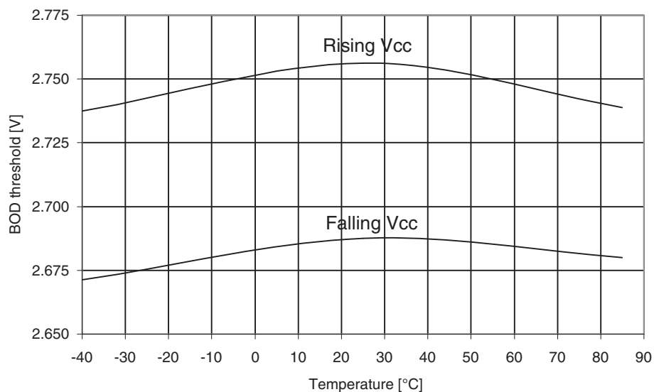
Figure 31-165. Atmel ATmega329A: BOD Thresholds vs. temperature (BOD level is 2.7V).
