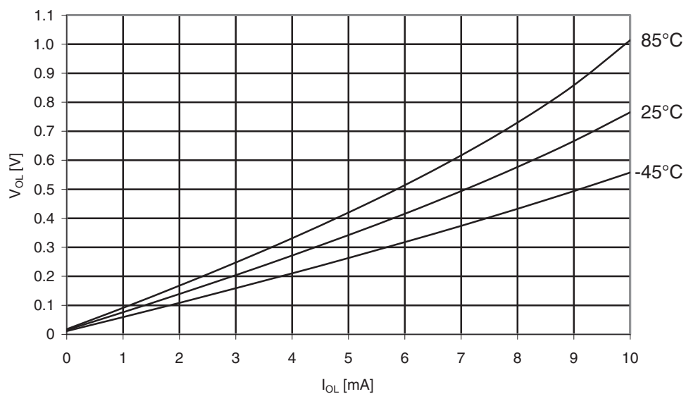
Figure 31-91. Atmel ATmega169PA. I/O pin output voltage vs. Sink current, ports A, C, D, E, F, G ( V_{CC} = 2.7V ).
