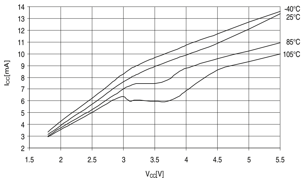
Figure 32-295. ATmega3290A - 105°C: Programming Current vs. V_{CC}
