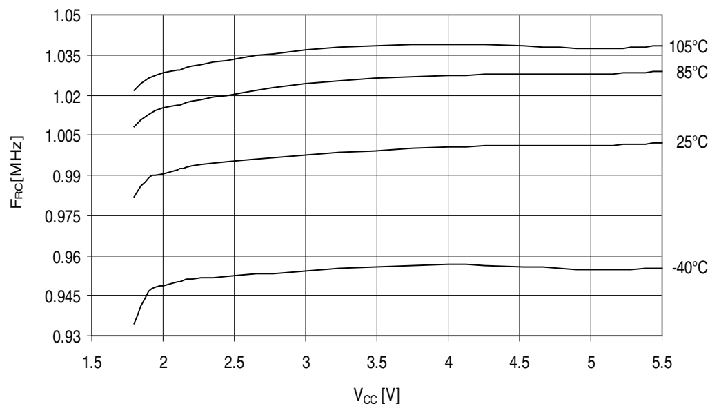
Figure 32-105. ATmega329A - 105°C: Calibrated 1MHz RC Oscillator Frequency vs. V_{CC}
