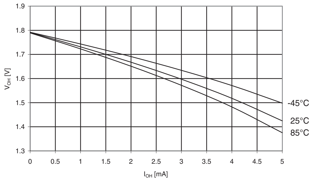
Figure 31-27. Atmel ATmega169A: I/O pin output voltage vs. source current, port B ( V_{CC} = 1.8V ).
