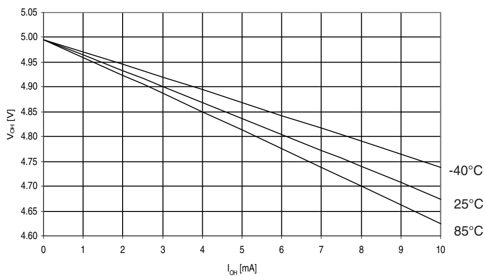
Figure 31-206. ATmega329PA: I/O pin output voltage vs. source current, ports A, C, D, E, F, G ( V_{CC} = 5V ).
