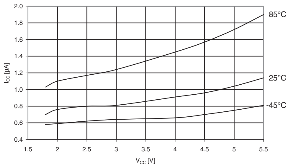
Figure 31-75. Atmel ATmega169PA: Power-save supply current vs. V_{CC} (Watchdog Timer disabled).
