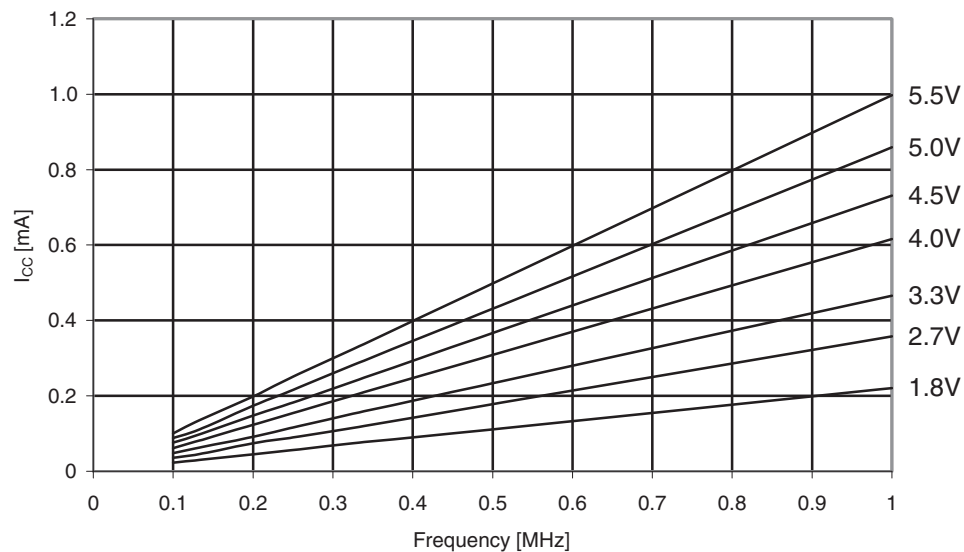
Figure 31-63. ATmega169PA: Active supply current vs. frequency (0.1 - 1.0MHz).
