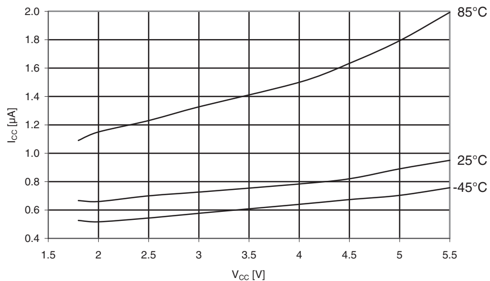
Figure 31-14. ATmega169A standby supply current vs. V_{CC} (32kHz watch XTAL, Watchdog Timer disabled).
