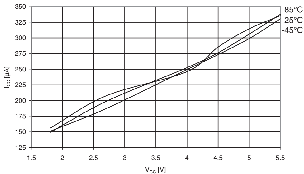
Figure 31-117. Atmel ATmega169PA: Active supply current with ADC at 1MHz vs. V_{CC} .
