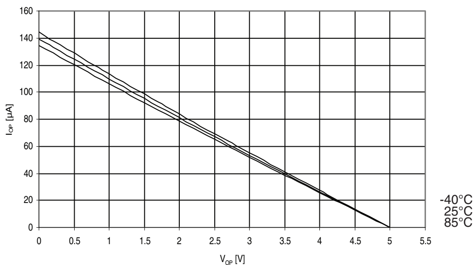
Figure 31-140. ATmega329A: I/O pin pull-up resistor current vs. input voltage ( V_{CC} = 5V ).
