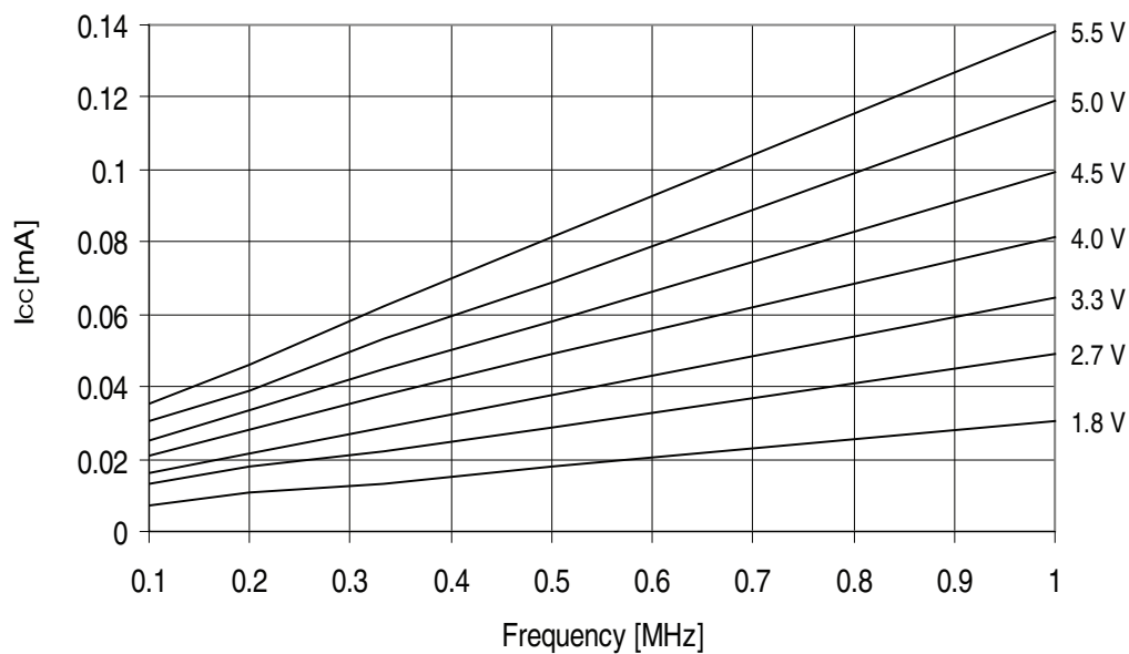
Figure 32-233. ATmega329PA - 105°C: Reset Supply Current vs. V_{CC} (0.1 - 1.0MHz, Excluding Current Through The Reset Pull-up)
