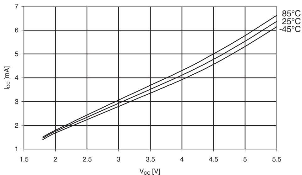
Figure 31-550. Atmel ATmega6490P: Active supply current vs. V_{CC} (Internal RC oscillator, 8MHz).
