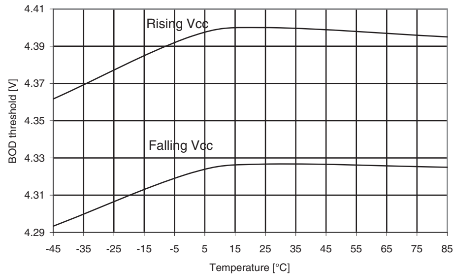
Figure 31-588. Atmel ATmega6490P: BOD Thresholds vs. temperature (BOD level is 4.3V).
