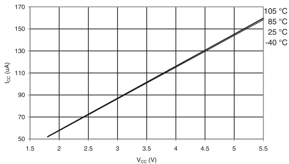
Figure 32-345. ATmega3290PA-105°C: AREF External Reference Current vs. V_{CC}
