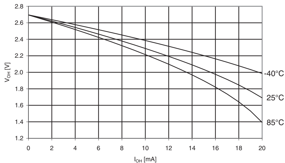
Figure 31-270. ATmega3290A: I/O pin output voltage vs. source current, port B ( V_{CC} = 2.7V ).
