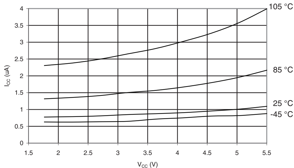
Figure 32-250. ATmega3290A - 105°C: Standby Supply Current vs. V_{CC} (32kHz Watch Crystal, Watchdog Timer Disabled)
