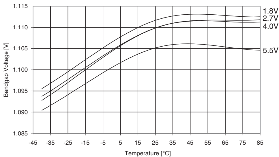
Figure 31-228. ATmega329PA: Bandgap voltage vs. temperature.
