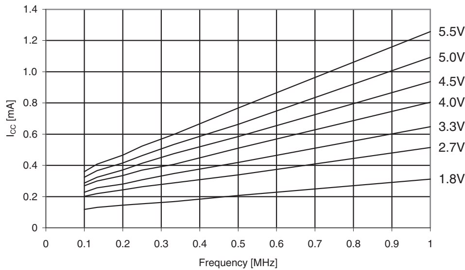
Figure 31-245. ATmega3290A: Active supply current vs. low frequency (0.1 - 1.0MHz).
