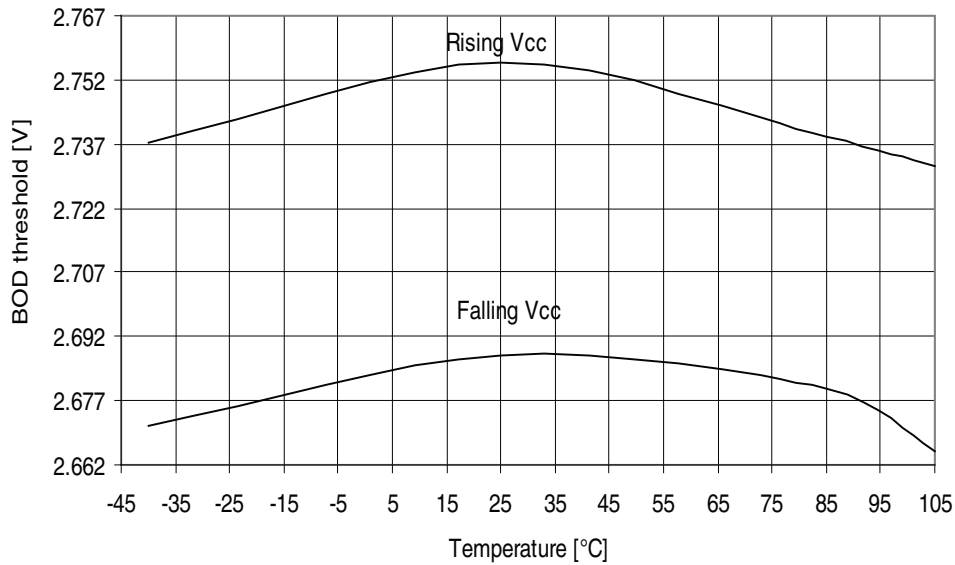
Figure 32-276. ATmega3290A - 105°C: BOD Thresholds vs. Temperature (BOD Level is 2.7V)
