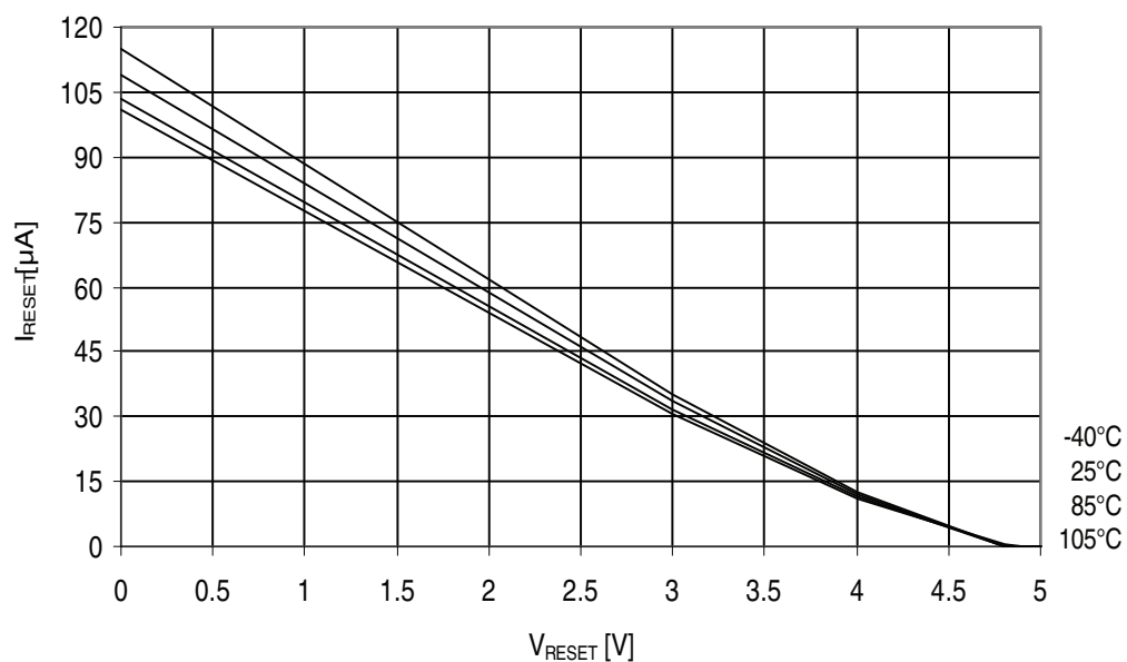
Figure 32-370. ATmega3290PA - 105°C: Reset Pull-up Resistor Current vs. Reset Pin Voltage ( V_{CC} = 5V )
