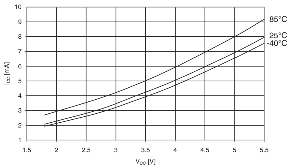
Figure 31-134. ATmega329A: Idle supply current vs. V_{CC} (32kHz watch XTAL).
