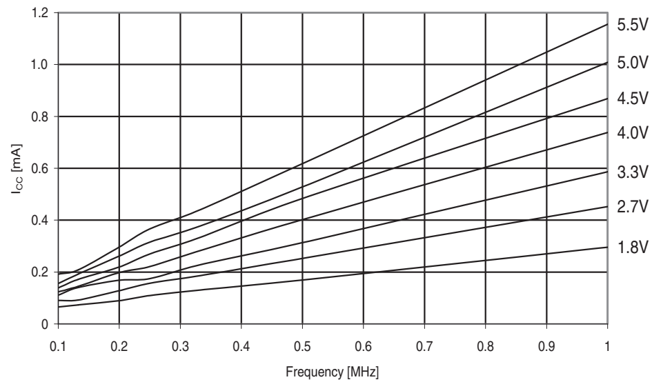
Figure 31-365. ATmega649A: Active supply current vs. low frequency (0.1 - 1.0MHz).
