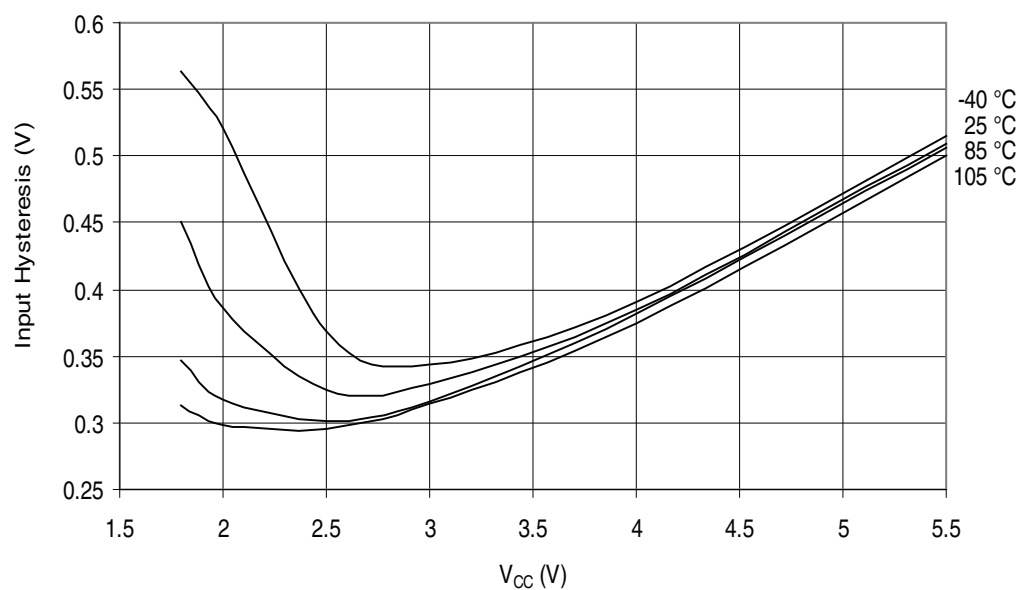
Figure 32-93. ATmega329A - 105°C: I/O Pin Input Hysteresis vs. V_{CC}
