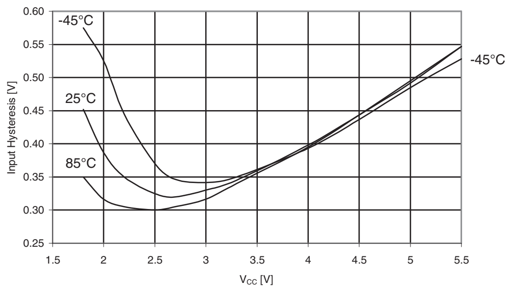
Figure 31-523. Atmel ATmega6490A: I/O pin input Hysteresis vs. V_{CC} .
