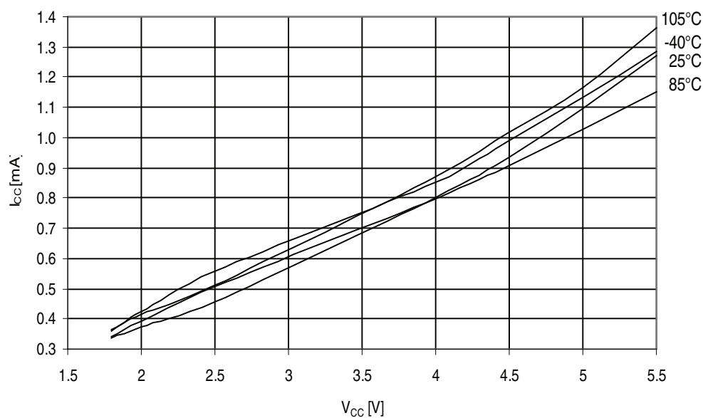
Figure 32-355. ATmega3290PA - 105°C: Active Supply Current vs. V_{CC} (Internal RC Oscillator, 1 MHz)S
