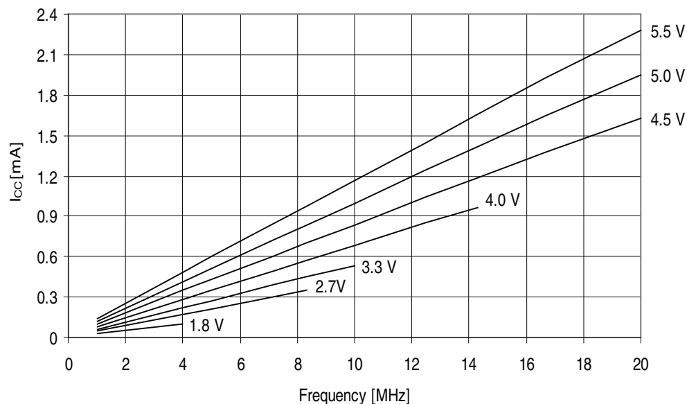
Figure 32-119. ATmega329A - 105°C: Reset Supply Current vs. V_{CC} (1 - 20MHz, Excluding Current Through The Reset Pull-up)
