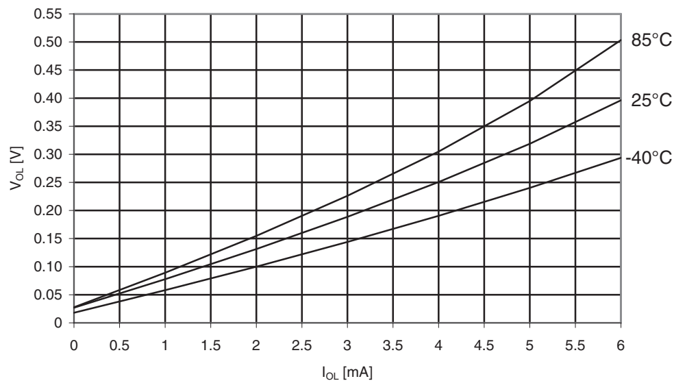
Figure 31-157. Atmel ATmega329A: I/O pin output voltage vs. sink current, port B ( V_{CC} = 1.8V ).
