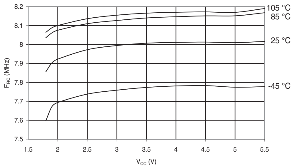
Figure 32-46. ATmega169PA-105°C: Calibrated 8MHz RC Oscillator Frequency vs. V_{CC}
