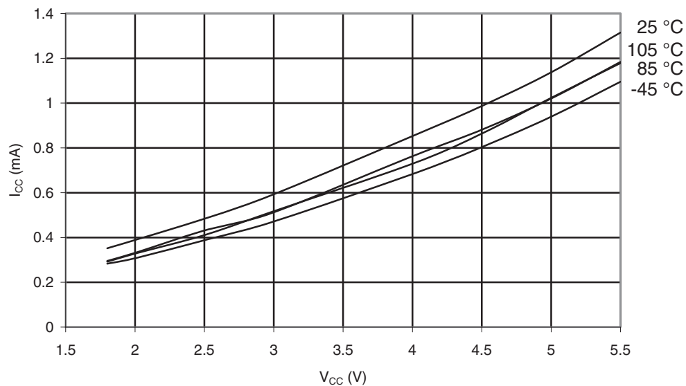
Figure 32-4. ATmega169PA-105°C: Active Supply Current vs. V_{CC} (Internal RC Oscillator, 1MHz)
