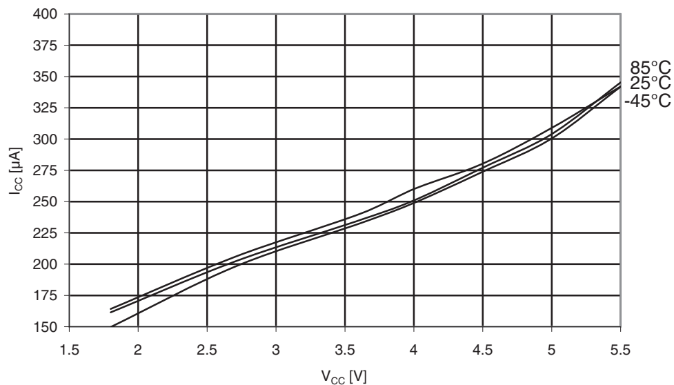
Figure 31-53. Atmel ATmega169A: Active supply current with ADC at 50kHz vs. V_{CC} .
