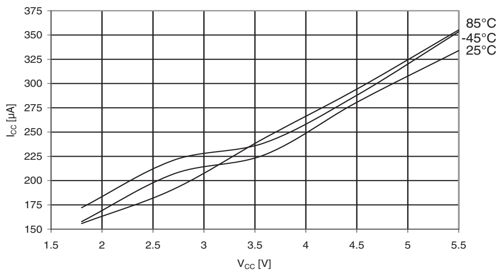
Figure 31-54. ATmega169A: Active supply current with ADC at 200kHz vs. V_{CC} .
