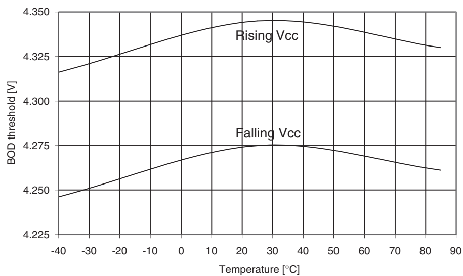
Figure 31-284. ATmega3290A: BOD Thresholds vs. temperature (BOD level is 4.3V).
