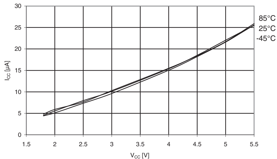
Figure 31-119. Atmel ATmega169PA: Watchdog Timer current vs. V_{CC} .
