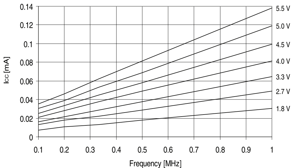
Figure 32-412. ATmega3290PA - 105°C: Reset Supply Current vs. V_{CC} (0.1 - 1.0MHz, Excluding Current Through The Reset Pull-up)
