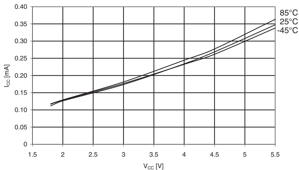
Figure 31-71. Atmel ATmega169PA: Idle supply current vs. V_{CC} (Internal RC oscillator, 1MHz).
