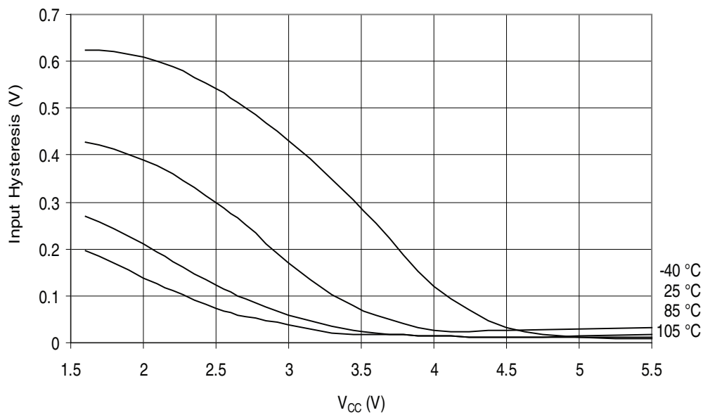
Figure 32-96. ATmega329A - 105°C: Reset Input Pin Hysteresis vs. V_{CC}
