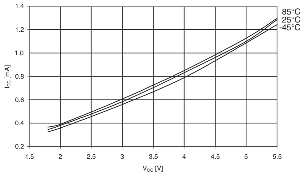
Figure 31-556. Atmel ATmega6490P: Idle supply current vs. V_{CC} (Internal RC oscillator, 1MHz).
