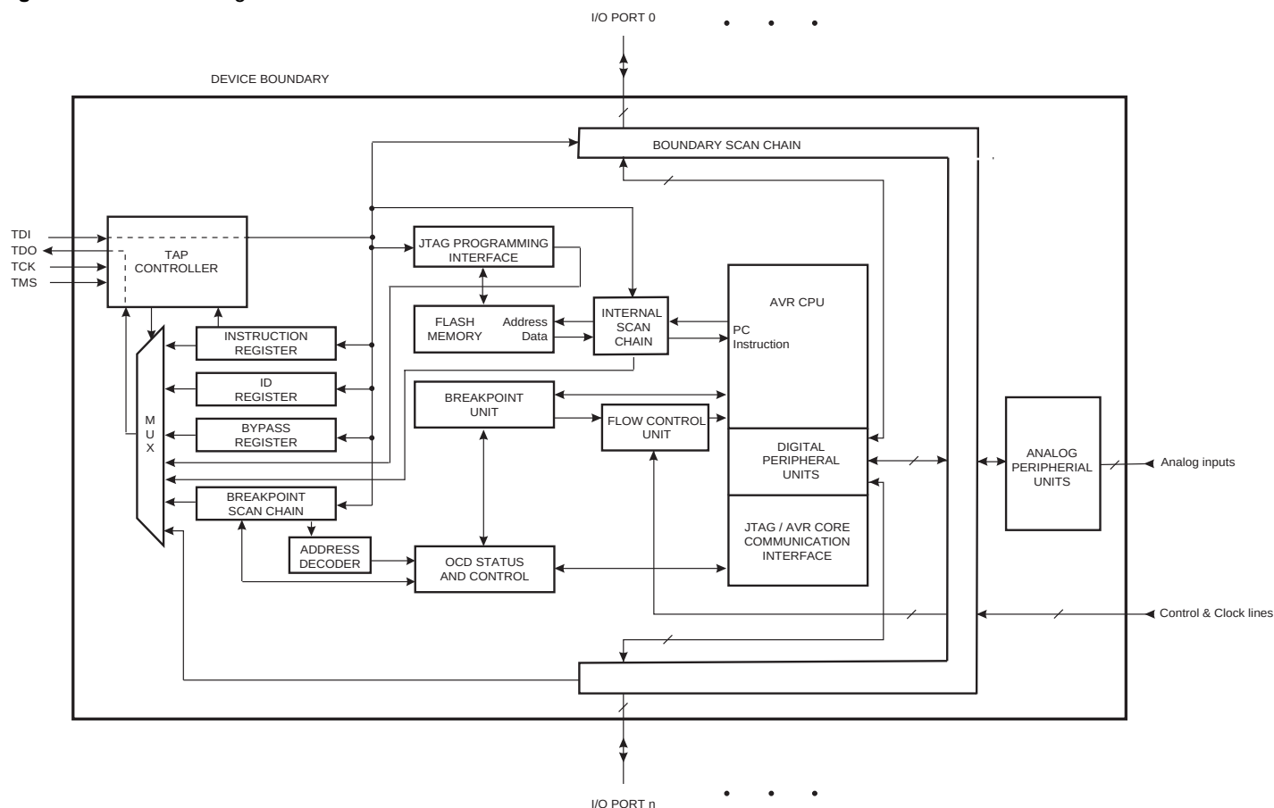
Figure 25-1. Block diagram.
