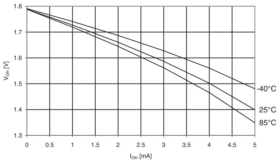
Figure 31-151. Atmel ATmega329A: I/O pin output voltage vs. source current, port B ( V_{CC} = 1.8V ).
