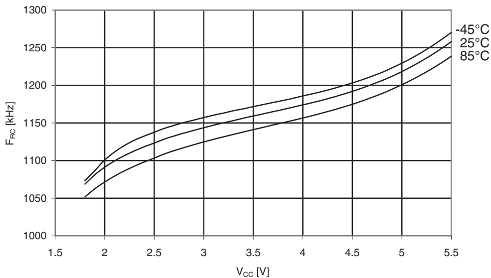
Figure 31-109. Atmel ATmega169PA: Watchdog oscillator frequency vs. V_{CC} .
