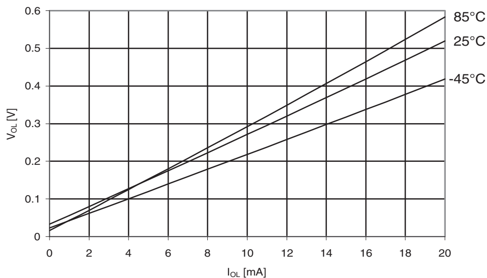
Figure 31-457. ATmega649P: I/O pin output voltage vs. sink current, port B ( V_{CC} = 5V ).
