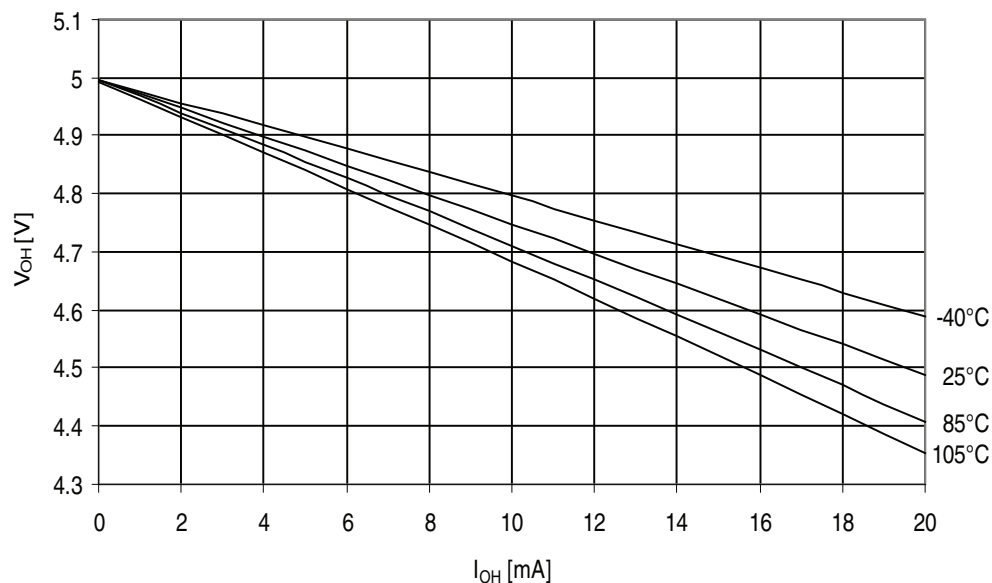
Figure 32-376. ATmega3290PA - 105°C: I/O Pin Output Voltage vs. Source Current, Port B ( V_{CC} = 5V )
