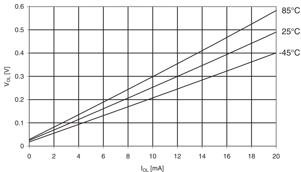
Figure 31-31. Atmel ATmega169A: I/O pin output voltage vs. sink current, port B ( V_{CC} = 5V ).
