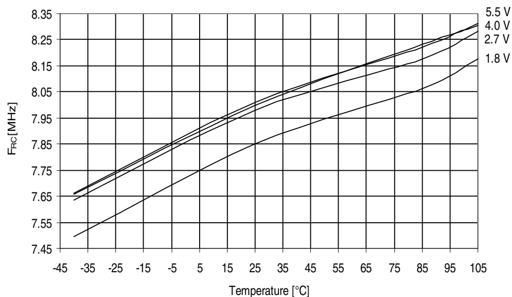
Figure 32-400. AATmega3290PA - 105°C: Calibrated 8MHz RC Oscillator Frequency vs. Temperature
