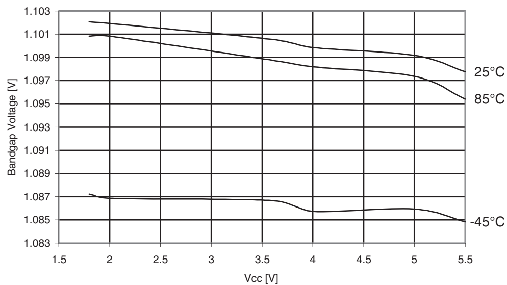
Figure 31-408. ATmega649A: Bandgap voltage vs. V_{CC} .
