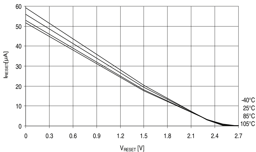
Figure 32-371. ATmega3290PA - 105°C: Reset Pull-up Resistor Current vs. Reset Pin Voltage ( V_{CC} = 2.7V )
