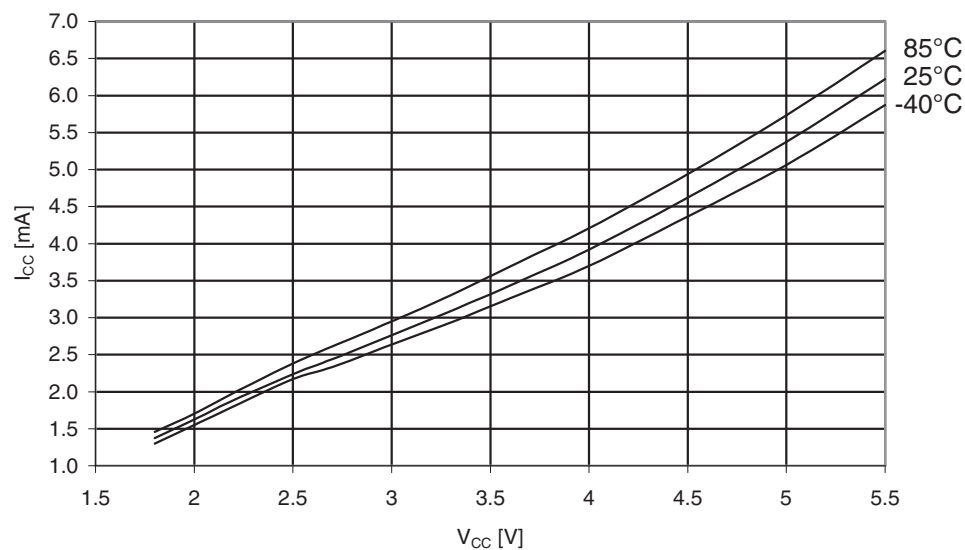
Figure 31-247. Atmel ATmega3290A: Active supply current vs. V_{CC} (Internal RC oscillator, 8MHz).
