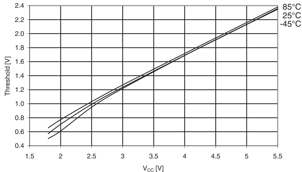
Figure 31-583. ATmega6490P: I/O pin input Threshold voltage vs. V_{CC} ( V_{IL} , I/O pin read as “0”).
