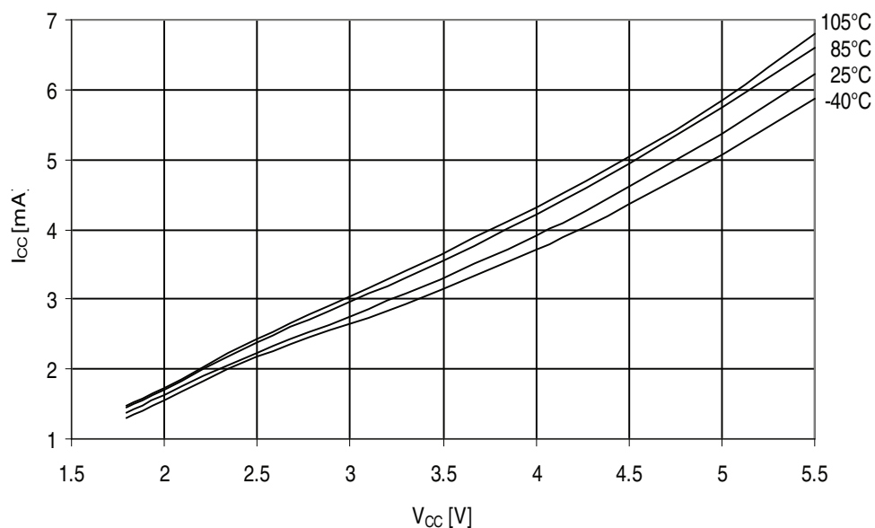
Figure 32-176. ATmega329PA - 105°C: Active Supply Current vs. V_{CC} (Internal RC Oscillator, 8MHz)
