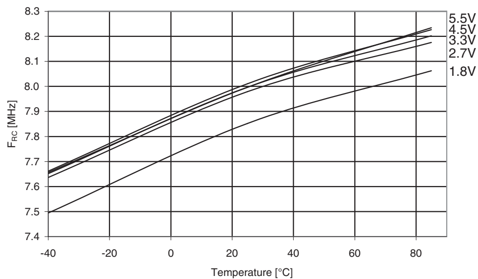
Figure 31-171. Atmel ATmega329A: Calibrated 8MHz RC oscillator frequency vs. temperature.
