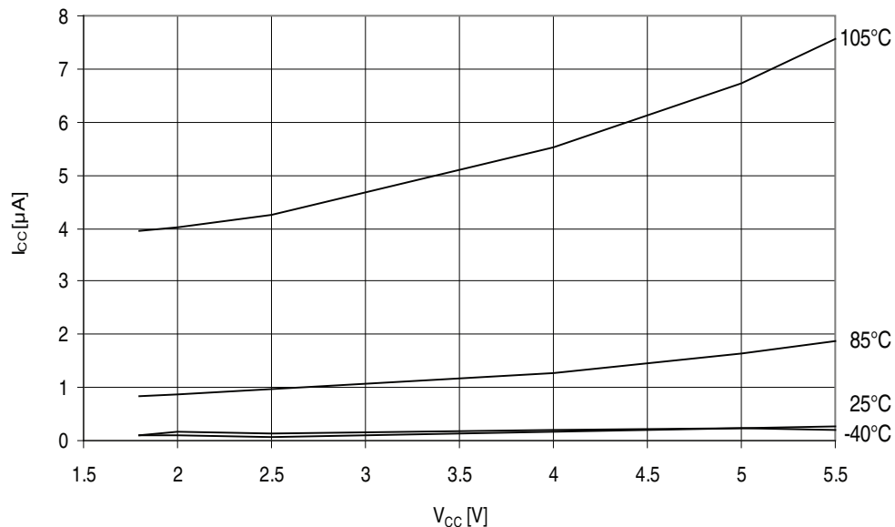
Figure 32-362. ATmega3290PA - 105°C: Power-down Supply Current vs. V_{CC} (Watchdog Timer Disabled)
