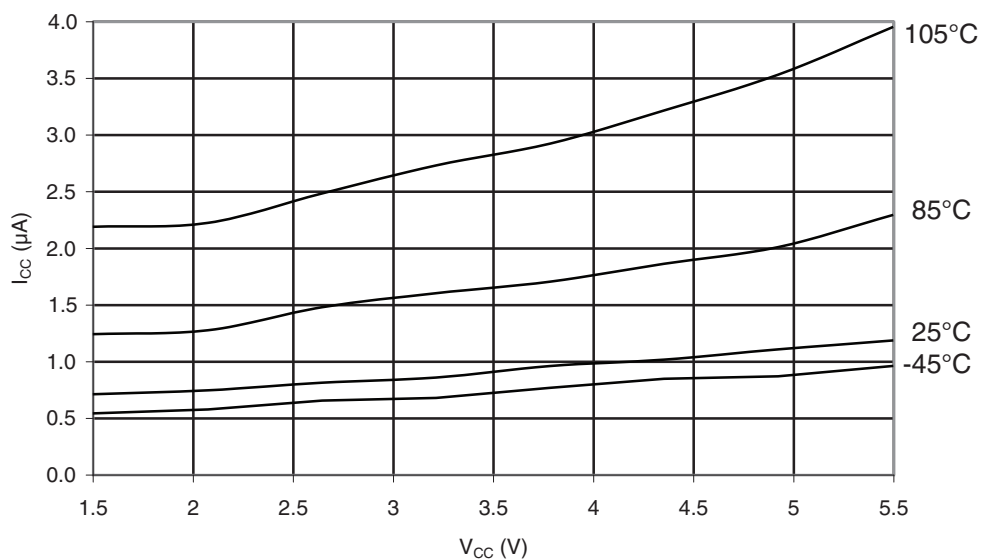
Figure 32-249. ATmega3290A - 105°C: Power-save Supply Current vs. V_{CC} (Watchdog Timer Disabled)
