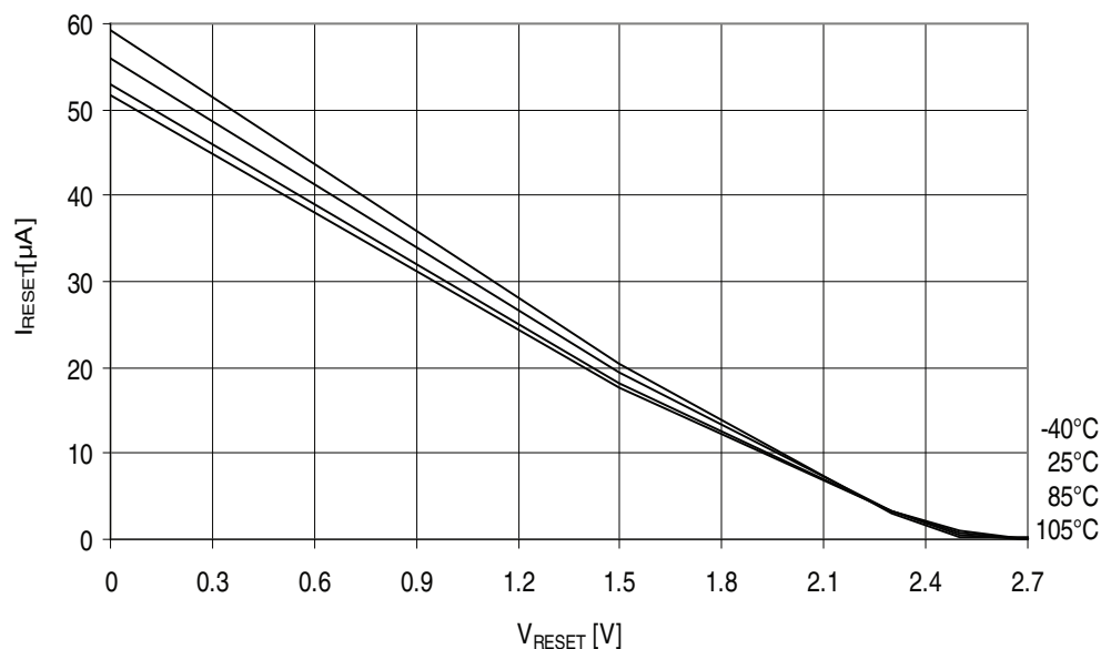
Figure 32-255. ATmega3290A - 105°C: Reset Pull-up Resistor Current vs. Reset Pin Voltage ( V_{CC} = 2.7V )
