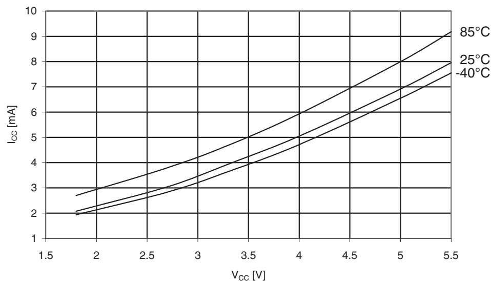
Figure 31-254. ATmega3290A: Idle supply current vs. V_{CC} (32kHz watch XTAL).
