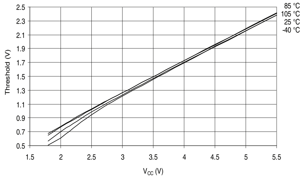
Figure 32-92. ATmega329A - 105°C: I/O Pin Input Threshold Voltage vs. V_{CC} ( V_{IL} , I/O Pin Read as “0”)
