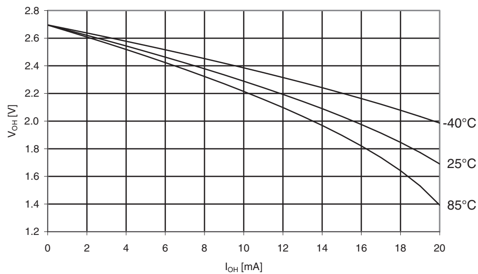
Figure 31-330. Atmel ATmega3290PA: I/O pin output voltage vs. source current, port B ( V_{CC} = 2.7V ).
