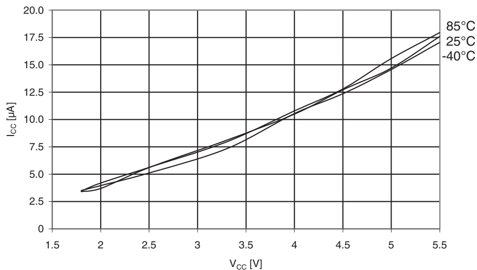
Figure 31-179. Atmel ATmega329A: Watchdog Timer current vs. V_{CC} .
