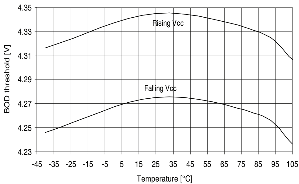
Figure 32-391. ATmega3290PA - 105°C: BOD Thresholds vs. Temperature (BOD Level is 4.3V)
