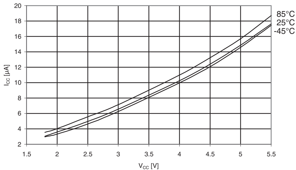
Figure 31-437. ATmega649P: Power-down supply current vs. V CC (Watchdog Timer enabled).
