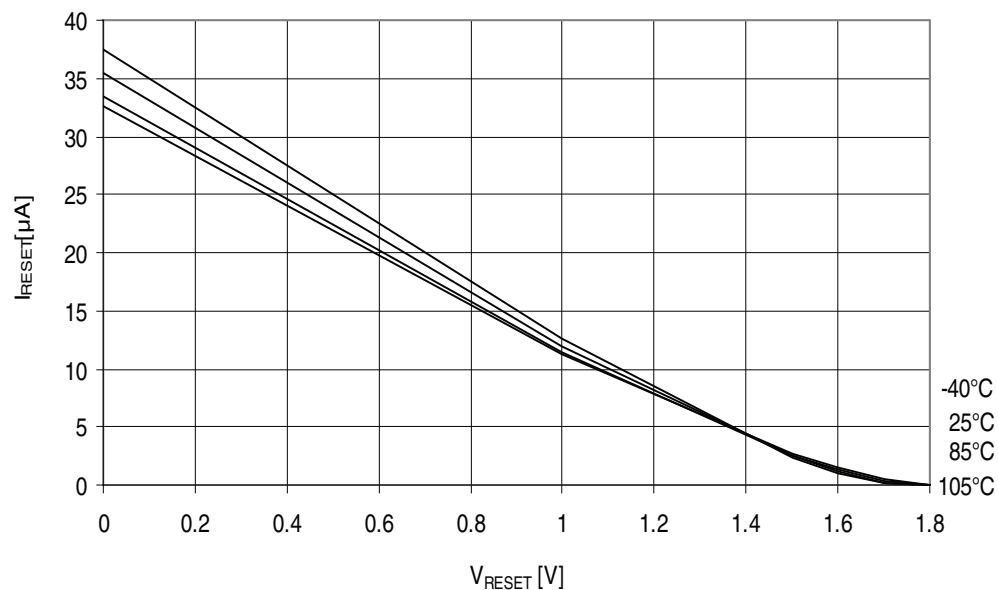
Figure 32-372. ATmega3290PA - 105°C: Reset Pull-up Resistor Current vs. Reset Pin Voltage ( V_{CC} = 1.8V )
