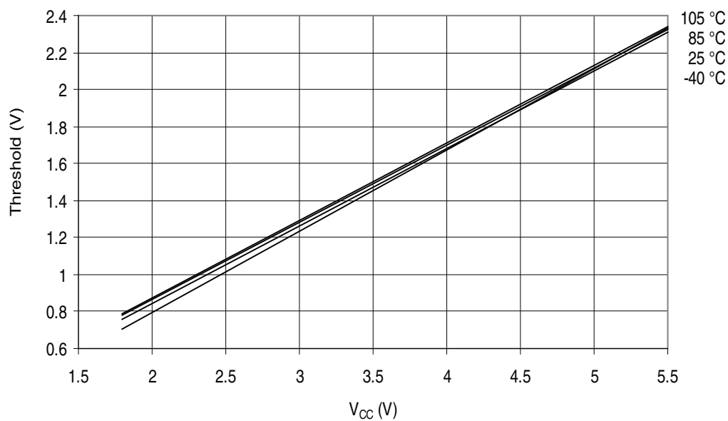
Figure 32-210. ATmega329PA - 105°C: Reset Input Threshold Voltage vs. V_{CC} ( V_{IL} , Reset Pin Read as “0”)
