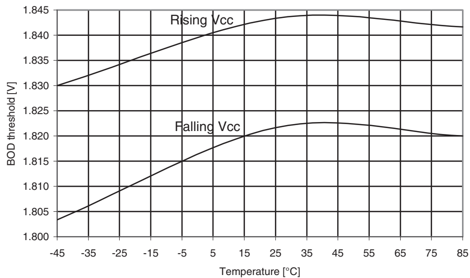
Figure 31-468. Atmel ATmega649P: BOD Thresholds vs. temperature (BOD level is 1.8V).
