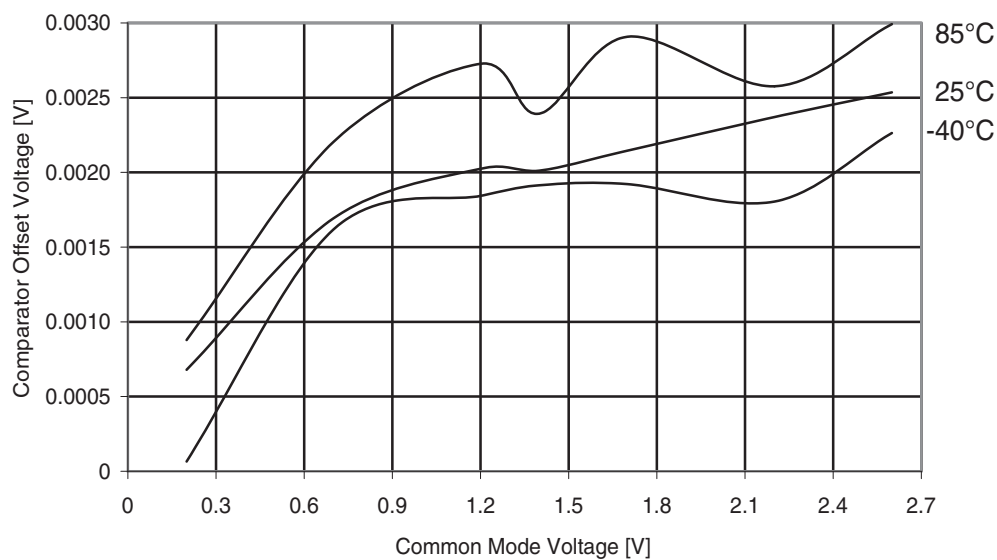
Figure 31-108. ATmega169PA: Analog Comparator offset voltage vs. Common Mode voltage ( V_{CC} = 2.7V ).
