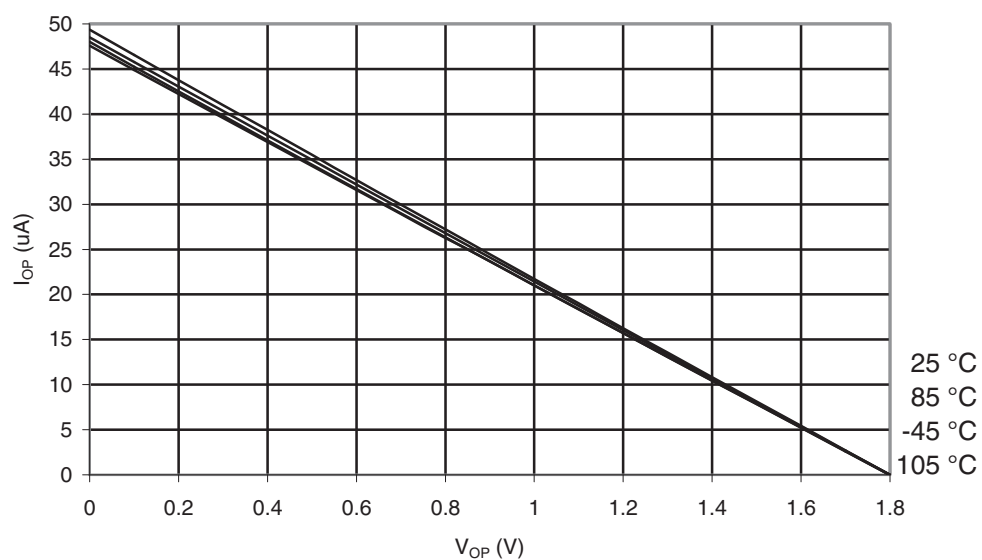
Figure 32-17. ATmega169PA-105°C: I/O Pin Pull-up Resistor Current vs. Input Voltage ( V_{CC} = 1.8V )
