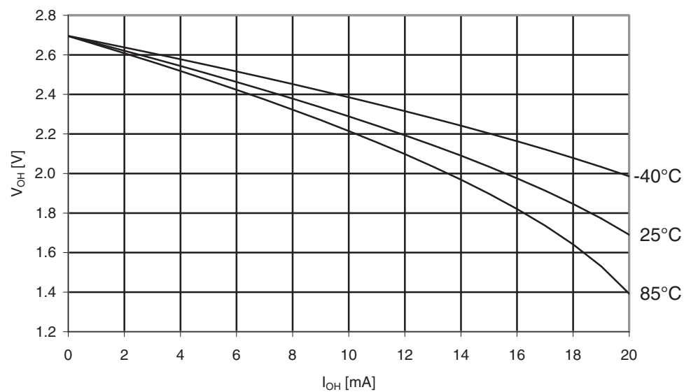
Figure 31-210. ATmega329PA: I/O pin output voltage vs. source current, port B ( V_{CC} = 2.7V ).
