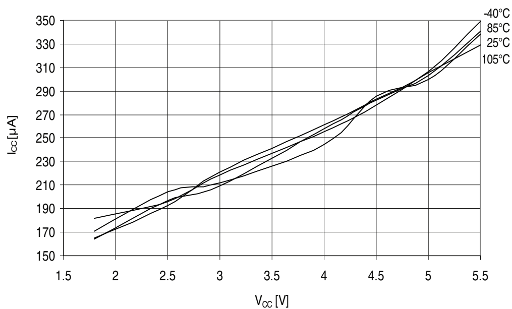
Figure 32-227. ATmega329PA - 105°C: Active Supply Current with ADC at 1MHz vs. V_{CC}
