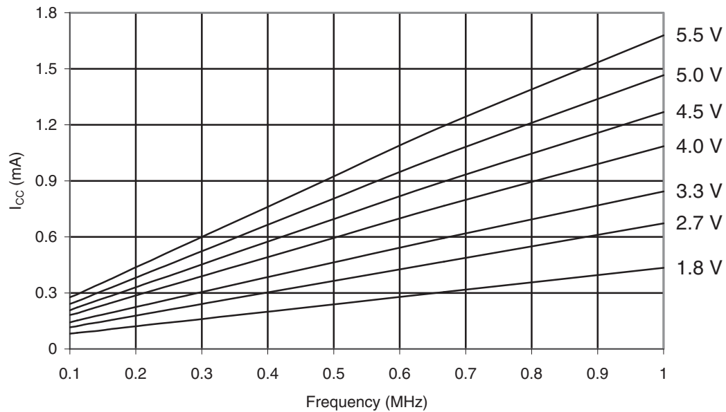
Figure 32-300. ATmega3290PA-105°C: Active Supply Current vs. Frequency (0.1 - 1.0MHz)
