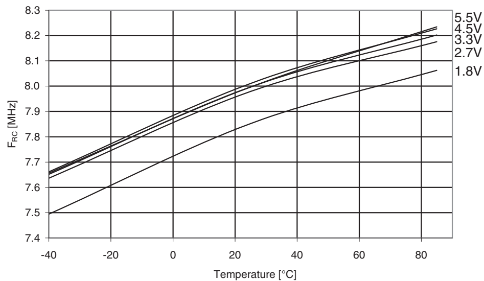
Figure 31-351. ATmega3290PA: Calibrated 8MHz RC oscillator frequency vs. temperature.
