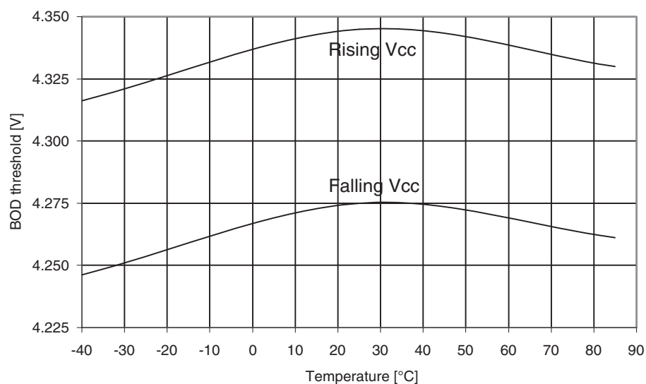
Figure 31-224. ATmega329PA: BOD Thresholds vs. temperature (BOD level is 4.3V).
