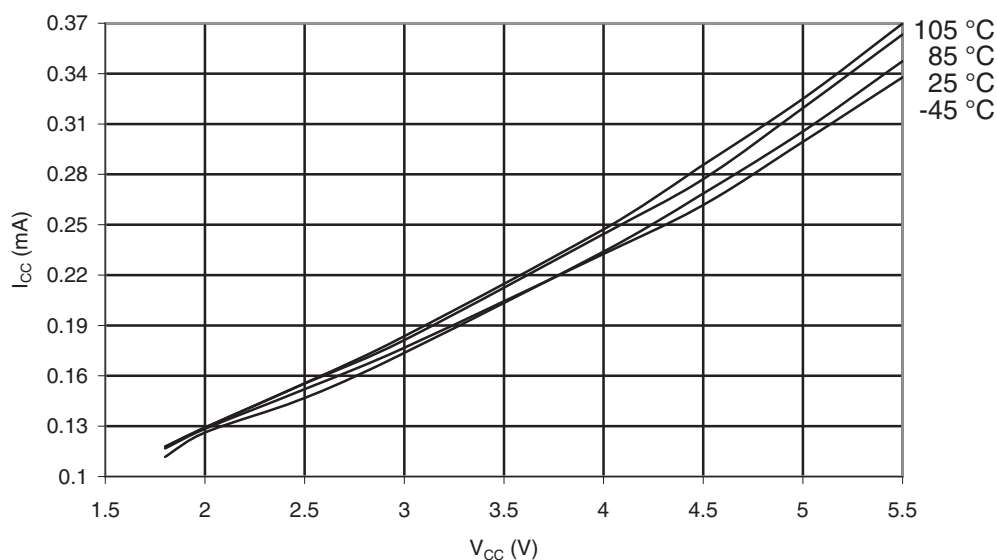
Figure 32-9. ATmega169PA-105°C: Idle Supply Current vs. V_{CC} (Internal RC Oscillator, 1MHz)
