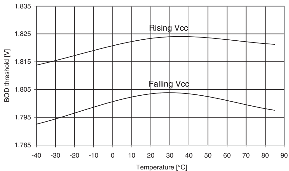
Figure 31-286. ATmega3290A: BOD Thresholds vs. temperature (BOD level is 1.8V).
