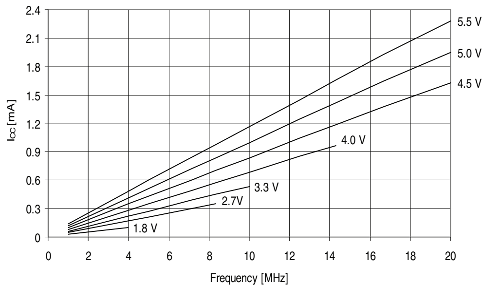
Figure 32-413. ATmega3290PA - 105°C: Reset Supply Current vs. V_{CC} (1 - 20MHz, Excluding Current Through The Reset Pull-up)
