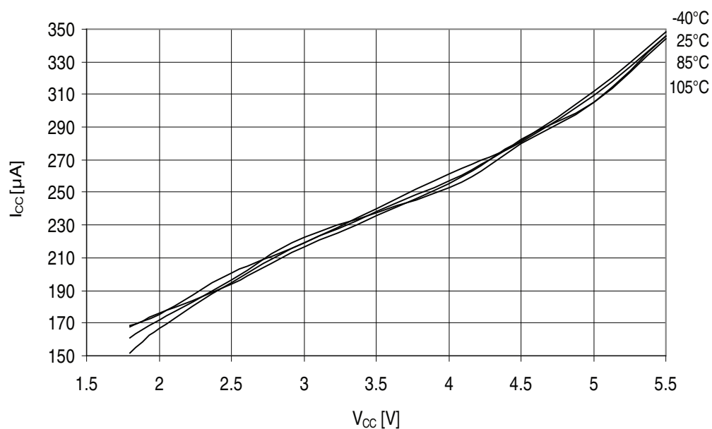
Figure 32-111. ATmega329A - 105°C: Active Supply Current with ADC at 200kHz vs. V_{CC}
