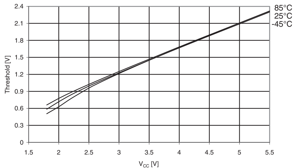
Figure 31-97. Atmel ATmega169PA. I/O pin Input Threshold voltage vs. V_{CC} ( V_{IL} , I/O pin read as “0”).
