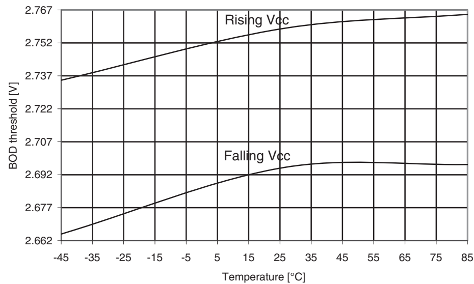
Figure 31-103. Atmel ATmega169PA: BOD Thresholds vs. temperature (BOD level is 2.7V).
