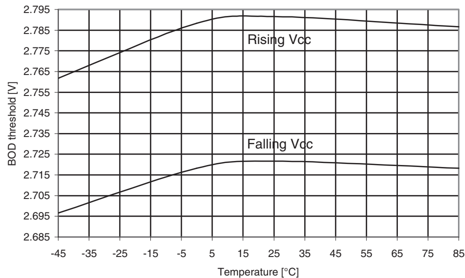
Figure 31-406. ATmega649A: BOD Thresholds vs. temperature (BOD level is 2.7V).
