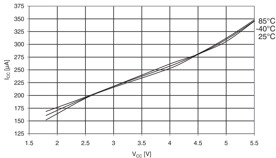
Figure 31-296. ATmega3290A: Active supply current with ADC at 200kHz vs. V_{CC} .
