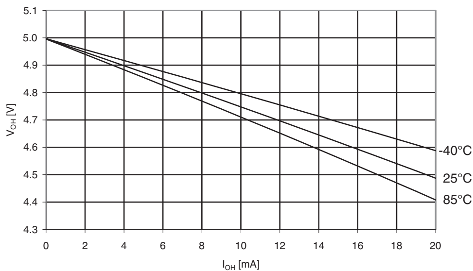
Figure 31-209. Atmel ATmega329PA: I/O pin output voltage vs. source current, port B ( V_{CC} = 5V ).
