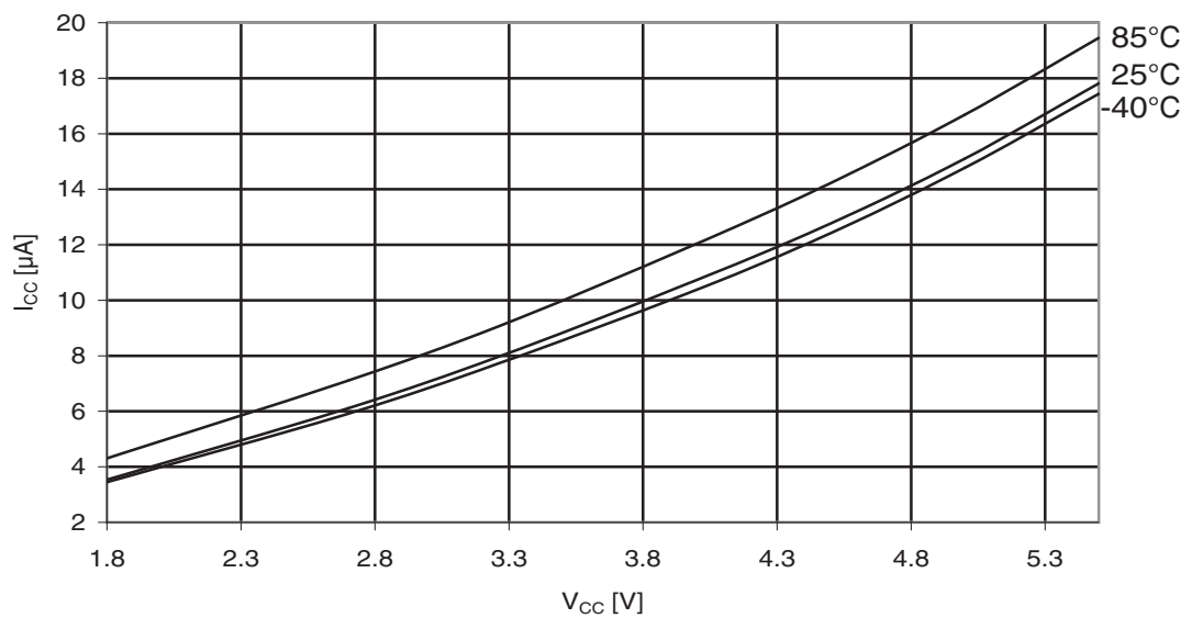
Figure 31-196. ATmega329PA: Power-down supply current vs. V_{CC} (Watchdog Timer enabled).
