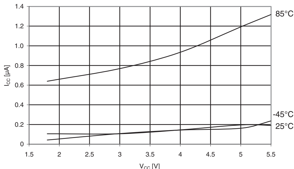
Figure 31-12. ATmega169A: Power-down supply current vs. V_{CC} (Watchdog Timer enabled).
