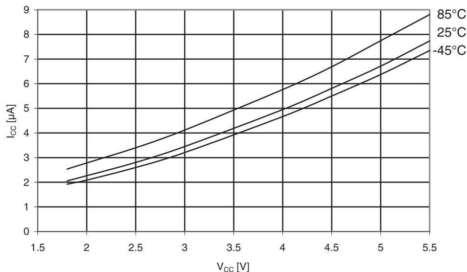
Figure 31-10. Atmel ATmega169A: Idle supply current vs. V_{CC} (32kHz watch XTAL).
