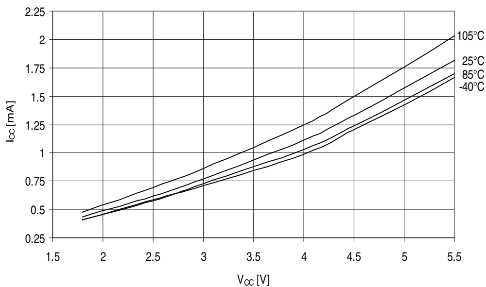
Figure 32-244. ATmega3290A - 105°C: Idle Supply Current vs. V_{CC} (Internal RC Oscillator, 8 MHz)
