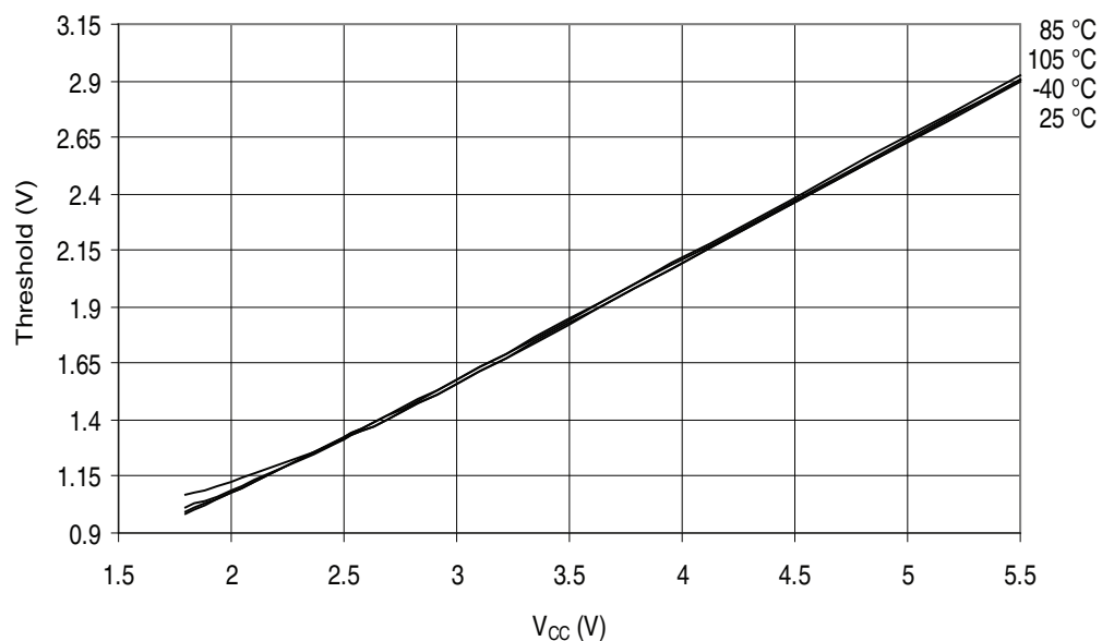
Figure 32-385. ATmega3290PA - 105°C: I/O Pin Input Threshold Voltage vs. V_{CC} ( V_{IH} , I/O Pin Read as “1”)
