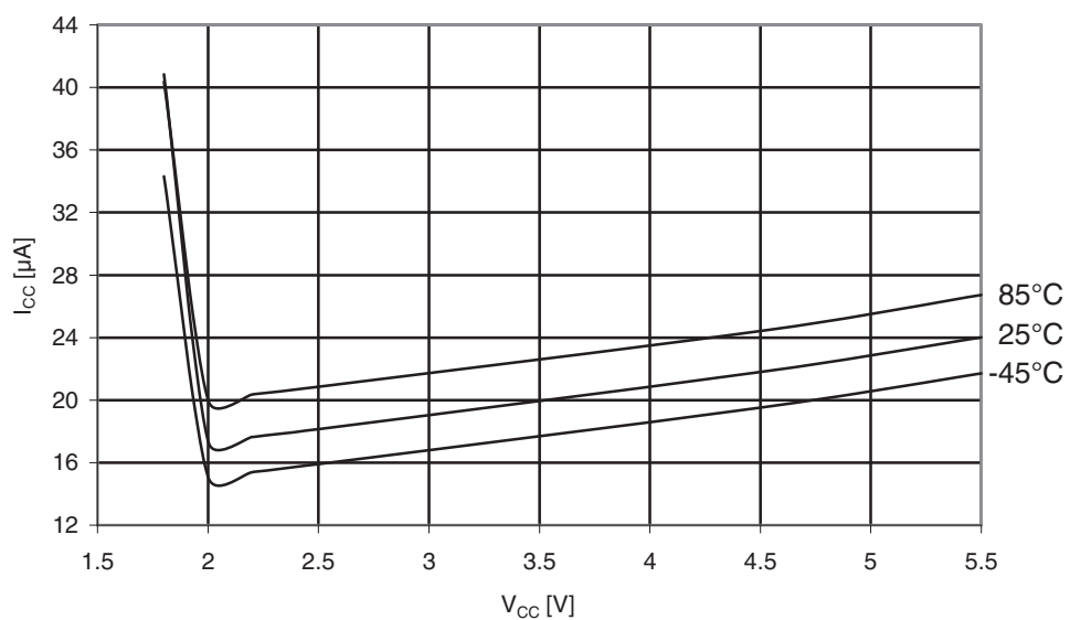
Figure 31-52. ATmega169A: Brownout Detector current vs. V_{CC} .
