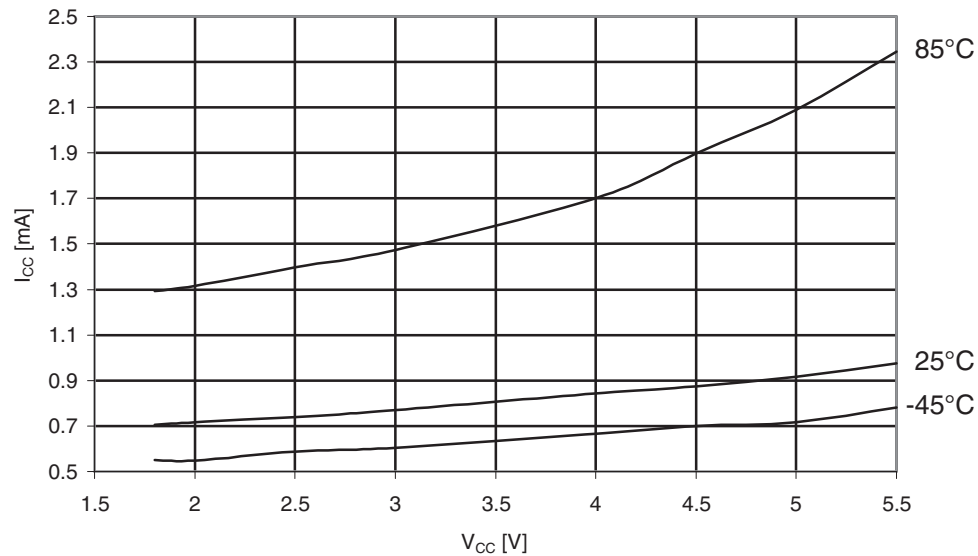
Figure 31-501. Atmel ATmega6490A standby supply current vs. V_{CC} (32kHz watch XTAL, Watchdog Timer disabled).
