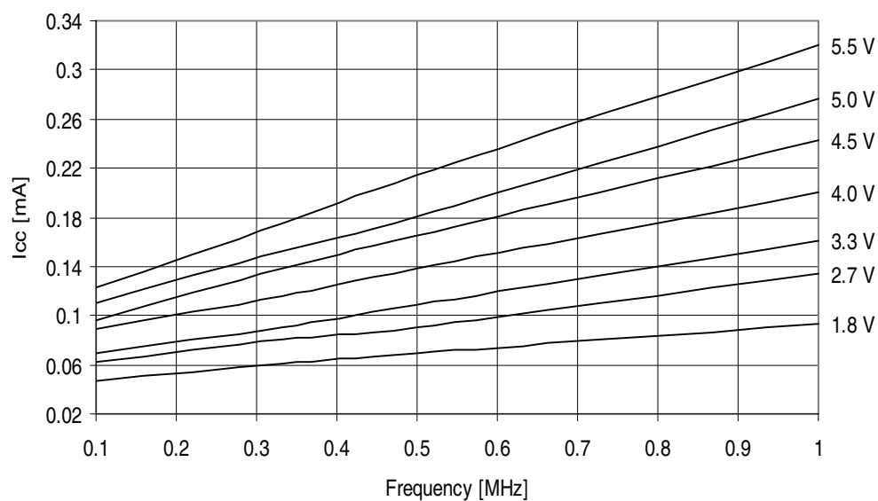
Figure 32-357. ATmega3290PA - 105°C: Idle Supply Current vs. Frequency (0.1 - 1.0MHz)
