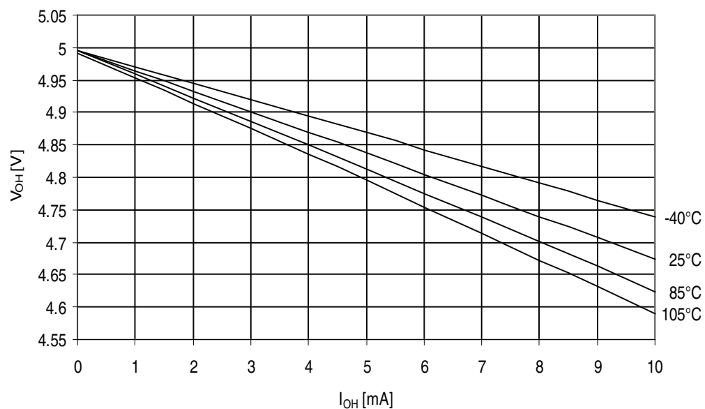
Figure 32-373. ATmega3290PA - 105°C: I/O Pin Output Voltage vs. Source Current, Ports A, C, D, E, F, G, H ( V_{CC} = 5V )
