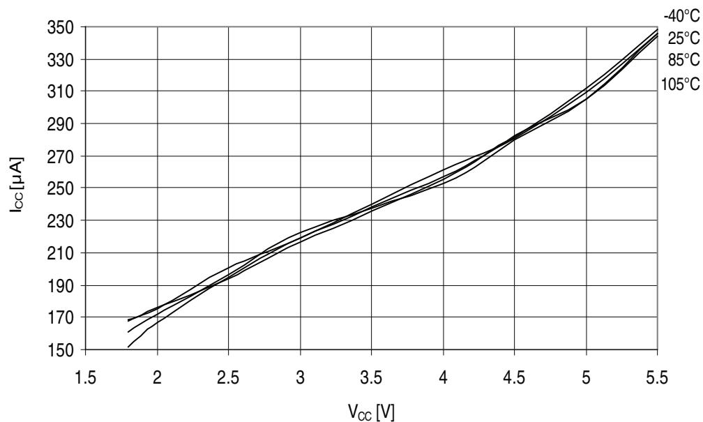
Figure 32-289. ATmega3290A - 105°C: Active Supply Current with ADC at 200kHz vs. V_{CC}
