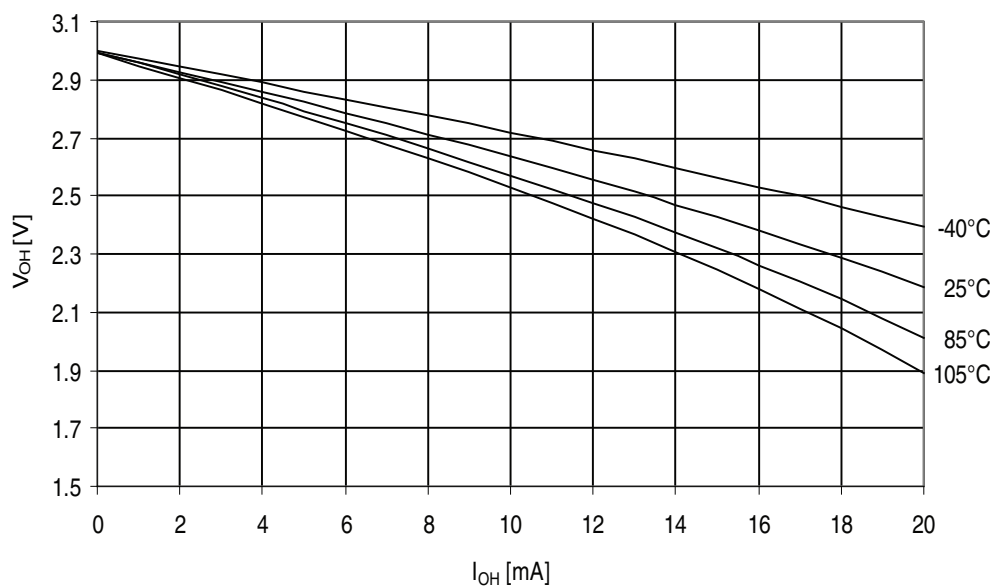
Figure 32-377. ATmega3290PA - 105°C: I/O Pin Output Voltage vs. Source Current, Port B ( V_{CC} = 3V )
