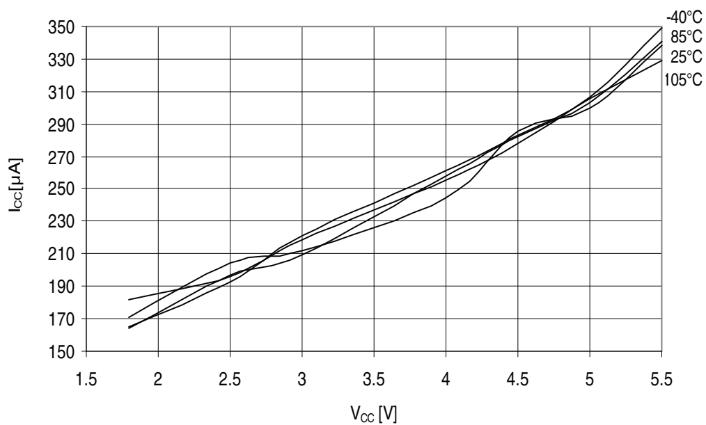
Figure 32-407. ATmega3290PA - 105°C: Active Supply Current with ADC at 2MHz vs. V_{CC} )
