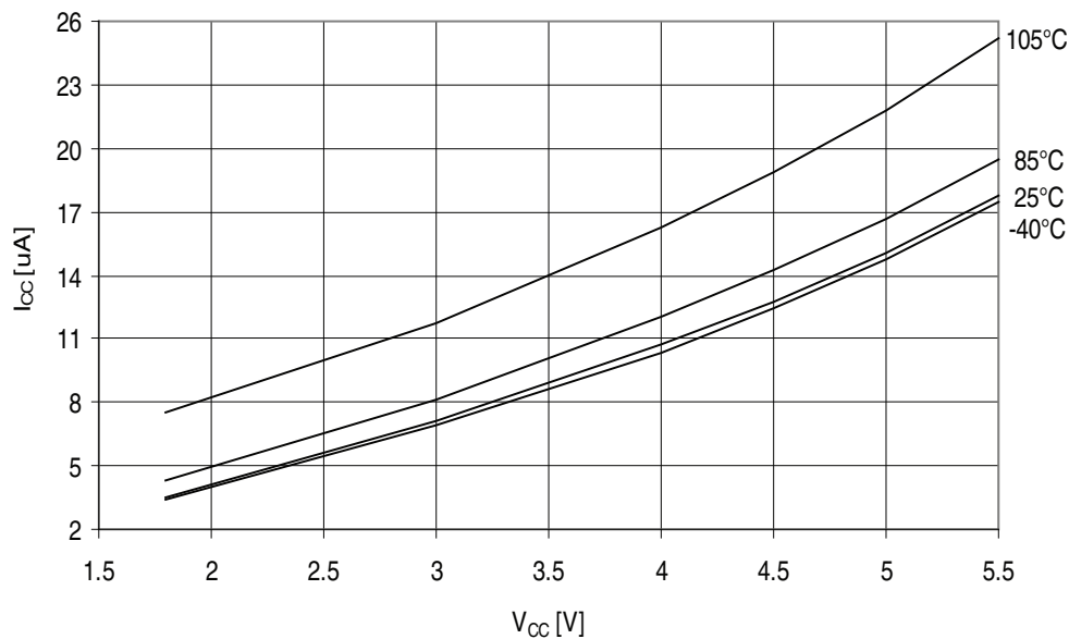
Figure 32-70. ATmega329A - 105°C: Power-down Supply Current vs. V CC (Watchdog Timer Enabled)
