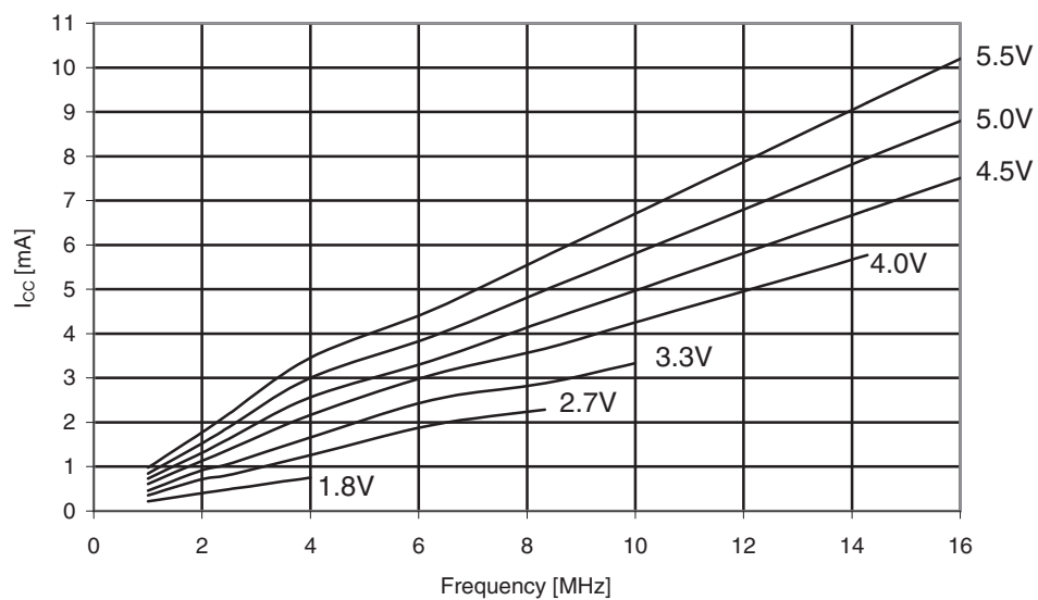
Figure 31-2. Atmel ATmega169A: Active supply current vs. frequency (1 - 16MHz).
