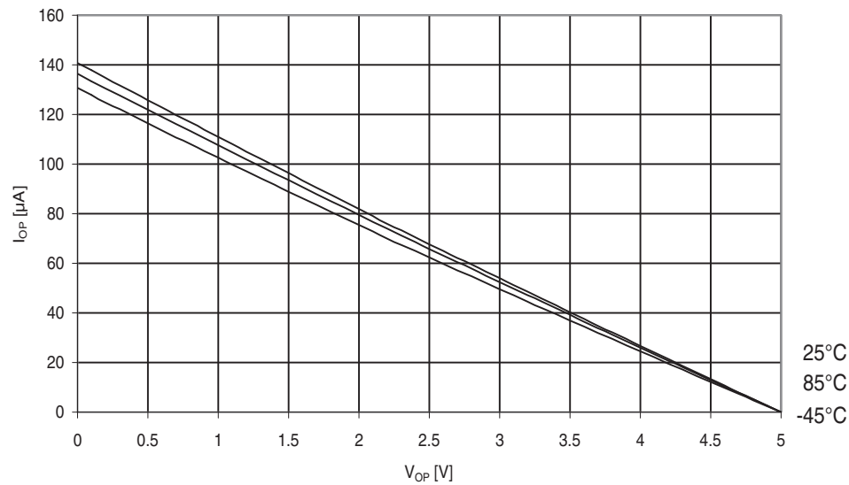
Figure 31-564. Atmel ATmega6490P: I/O pin pull-up resistor current vs. input voltage ( V_{CC} = 5V ).
