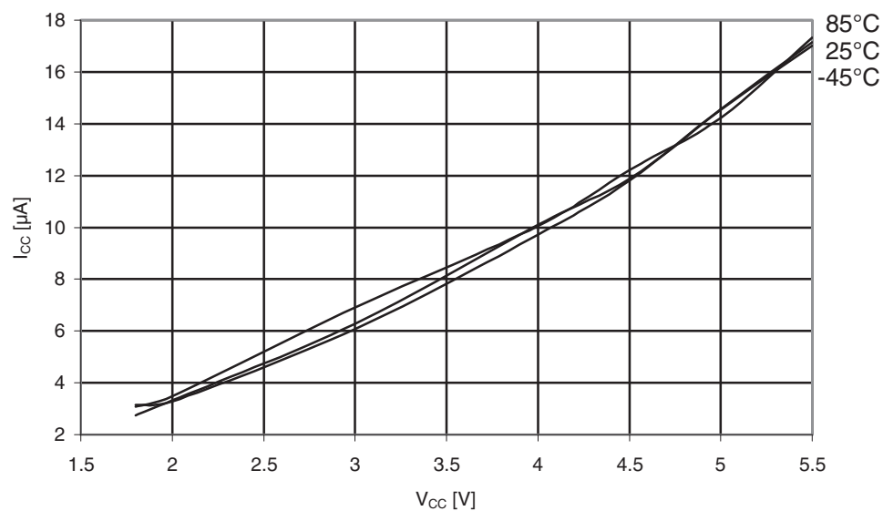
Figure 31-542. ATmega6490A: Watchdog Timer current vs. V_{CC} .
