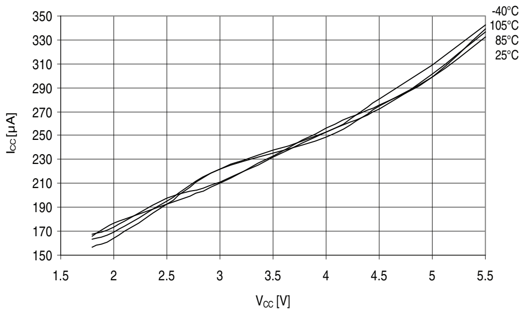
Figure 32-110. ATmega329A - 105°C: Active Supply Current with ADC at 50kHz vs. V_{CC}
