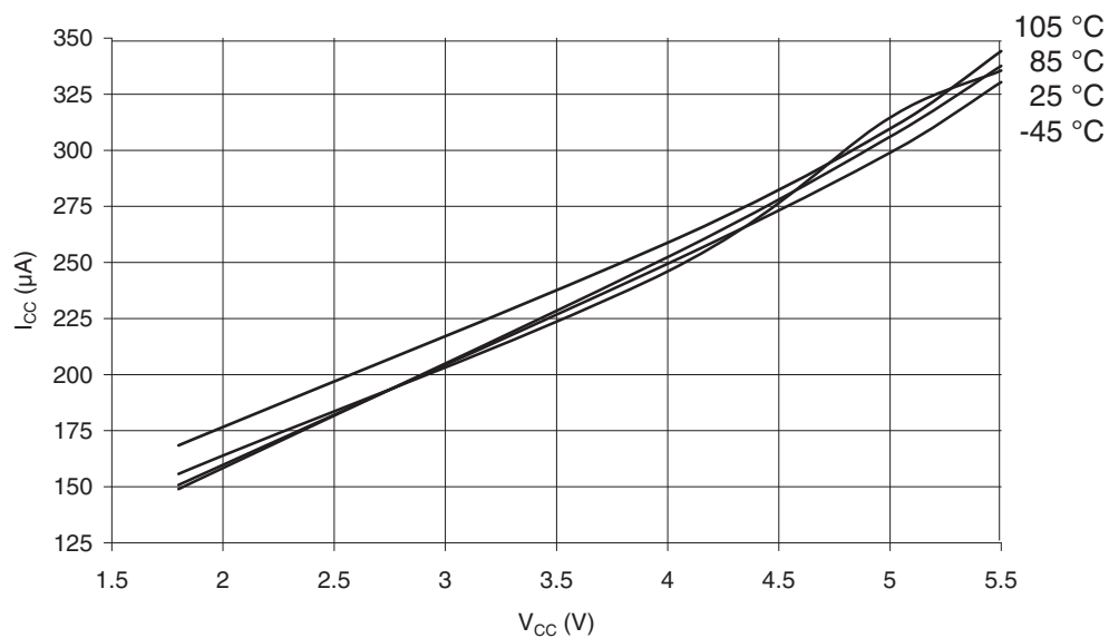
Figure 32-51. ATmega169PA-105°C: Active Supply Current with ADC at 1MHz vs. V_{CC}
