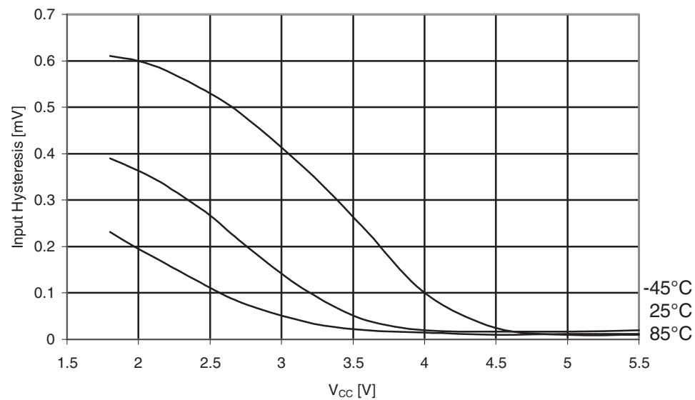
Figure 31-587. ATmega6490P: Reset input pin Hysteresis vs. V_{CC} .
