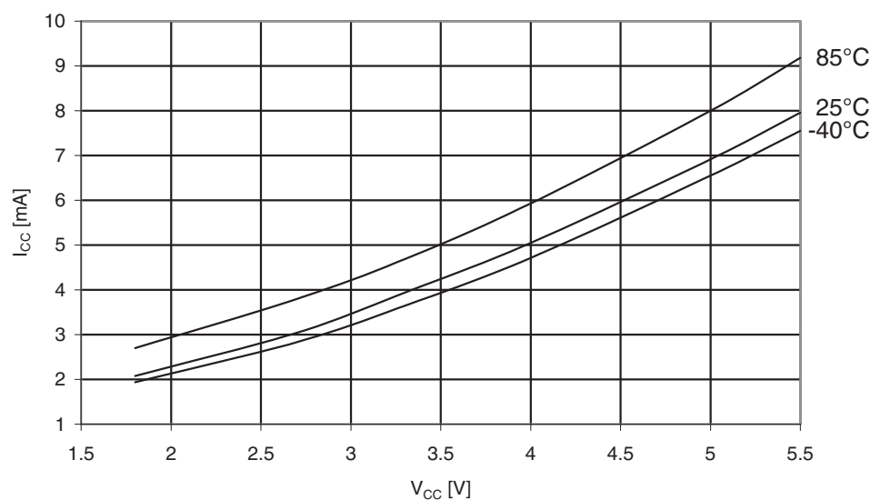
Figure 31-314. ATmega3290PA: Idle supply current vs. V_{CC} (32kHz watch XTAL).
