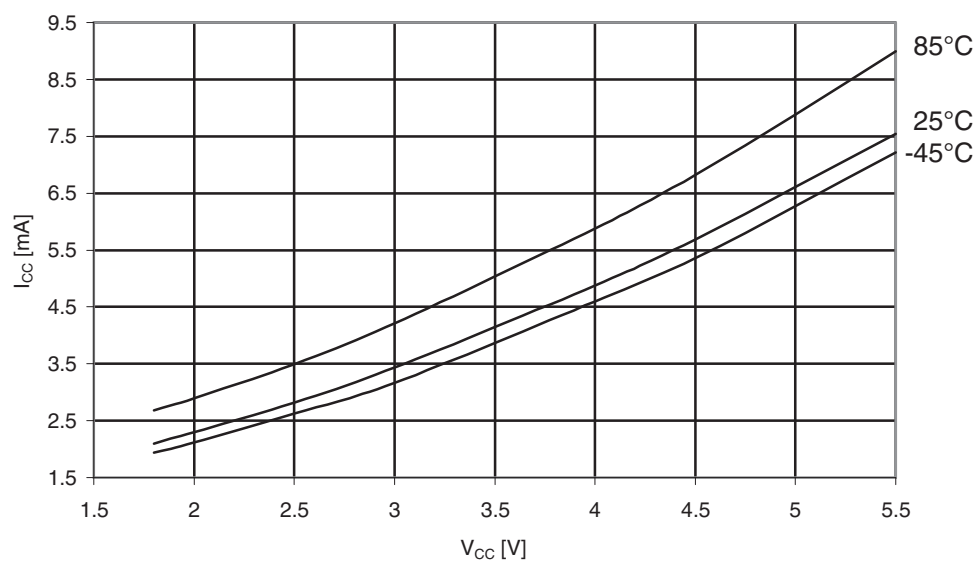
Figure 31-435. ATmega649P: Idle supply current vs. V_{CC} (32kHz watch XTAL).
