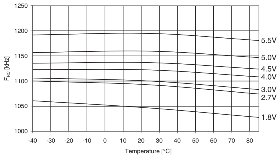
Figure 31-350. Atmel ATmega3290PA: Watchdog Oscillator frequency vs. temperature.
