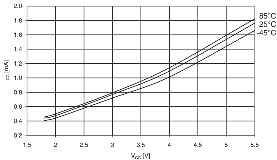
Figure 31-372. ATmega649A: Idle supply current vs. V_{CC} (Internal RC oscillator, 8MHz).
