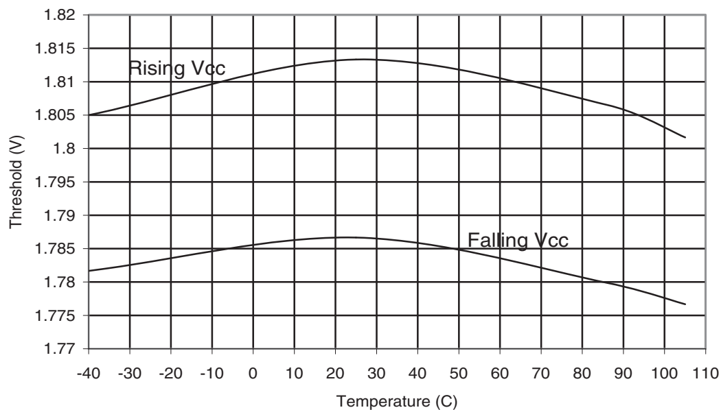
Figure 32-158. ATmega329P-105°C: BOD Thresholds vs. Temperature (BOD Level is 1.8V)
