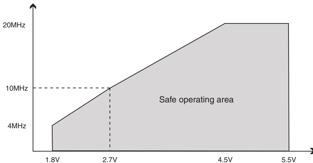
Figure 29-2. Maximum frequency vs. V_{CC} (0 - 20MHz) Atmel ATmega329A/ATmega329PA/ATmega3290A/ATmega3290PA/ATmega6490A/ATmega6490P.
