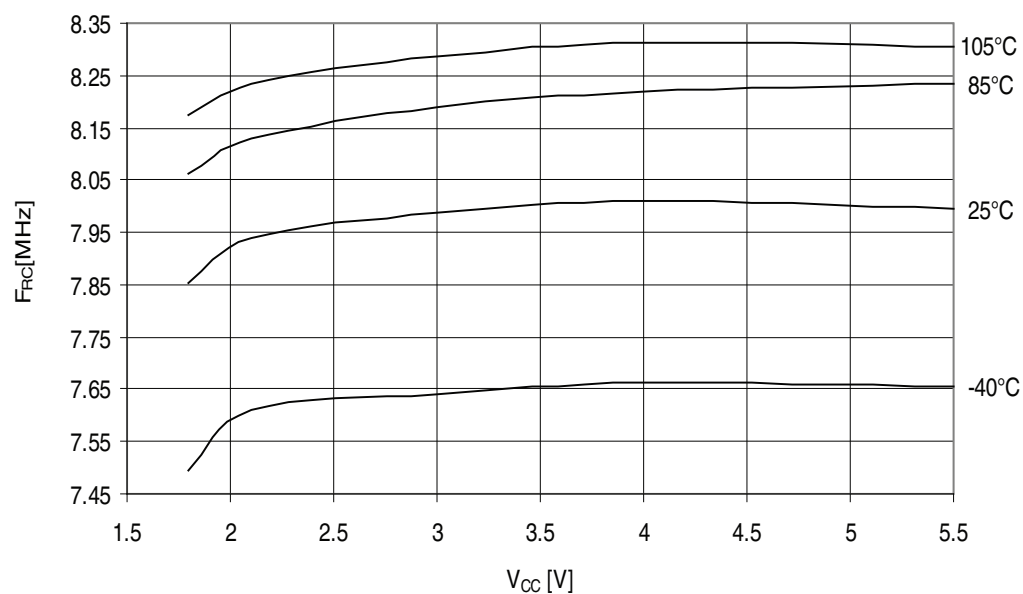
Figure 32-401. ATmega3290PA - 105°C: Calibrated 8MHz RC Oscillator Frequency vs. V_{CC}
