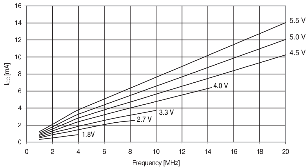
Figure 32-175. ATmega329PA - 105°C: Active Supply Current vs. Frequency (1 - 20MHz)
