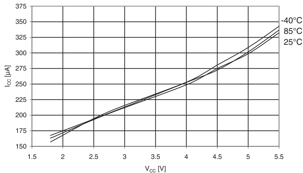
Figure 31-295. Atmel ATmega3290A: Active supply current with ADC at 50kHz vs. V_{CC} .
