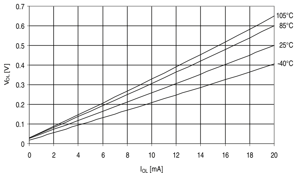
Figure 32-382. ATmega3290PA - 105°C: I/O Pin Output Voltage vs. Sink Current, Port B ( V_{CC} = 5V )
