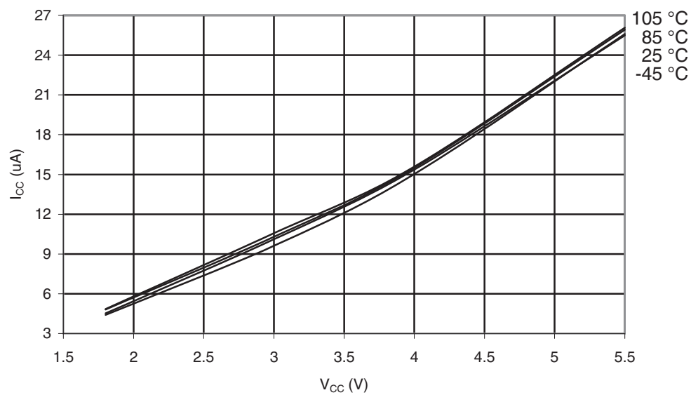
Figure 32-53. ATmega169PA-105°C: Watchdog Timer Current vs. V_{CC}
