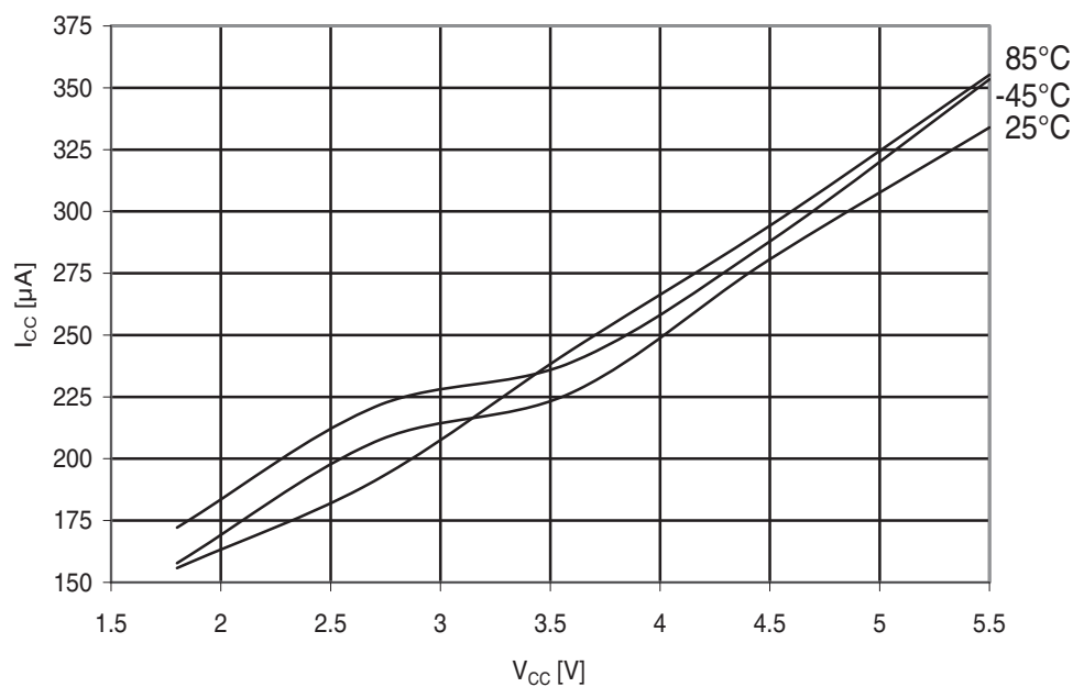
Figure 31-116. ATmega169PA: Active supply current with ADC at 200kHz vs. V_{CC} .
