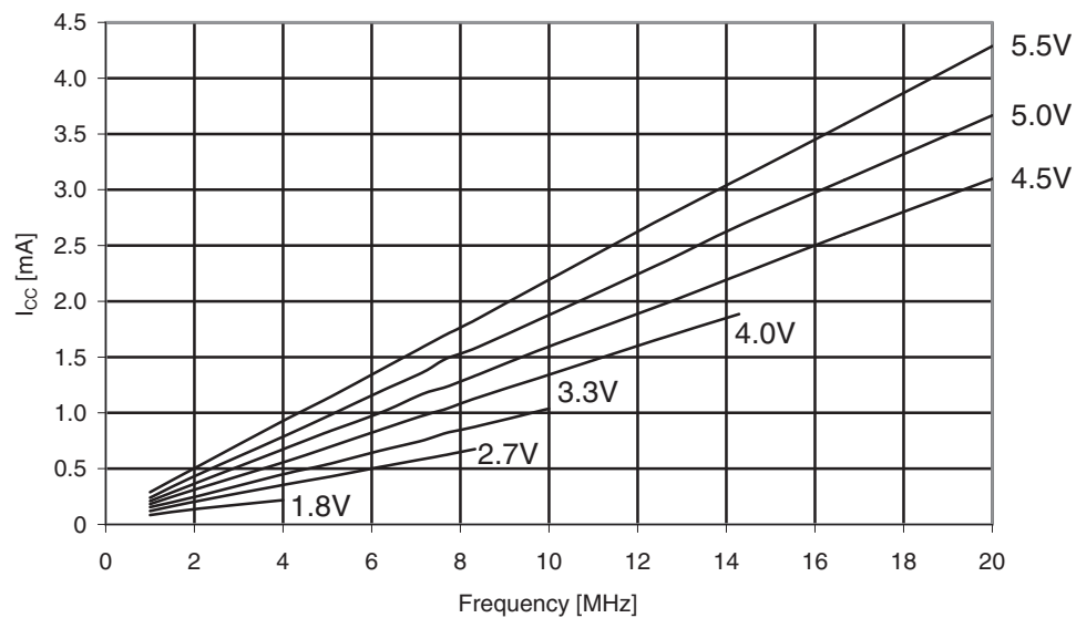
Figure 31-432. Atmel ATmega649P: Idle supply current vs. frequency (1 - 20MHz).
