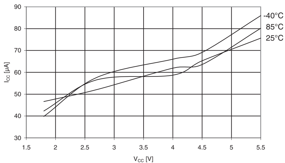
Figure 31-300. ATmega3290A: Analog Comparator current vs. V_{CC} .
