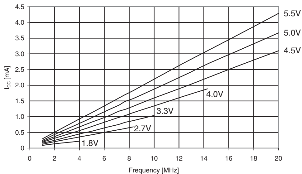
Figure 31-493. Atmel ATmega6490A: Idle supply current vs. frequency (1 - 20MHz).
