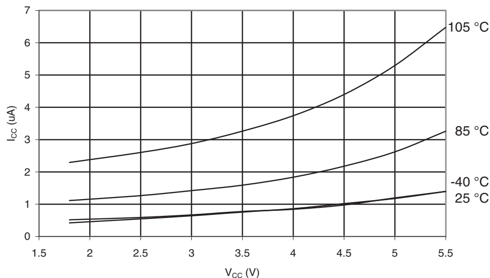
Figure 32-312. ATmega3290PA -105°C: Power-save Supply Current vs. V_{CC} (Watchdog Timer Disabled)
