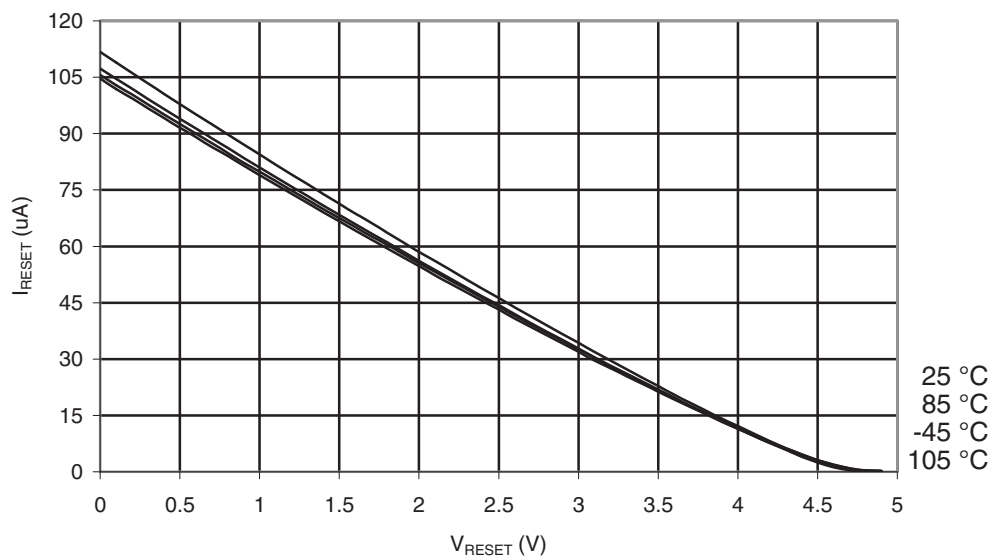
Figure 32-18. ATmega169PA-105°C: Reset Pull-up Resistor Current vs. Reset Pin Voltage ( V_{CC} = 5V )
