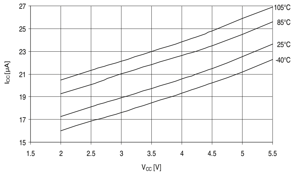
Figure 32-403. ATmega3290PA - 105°C: Brownout Detector Current vs. V_{CC}
