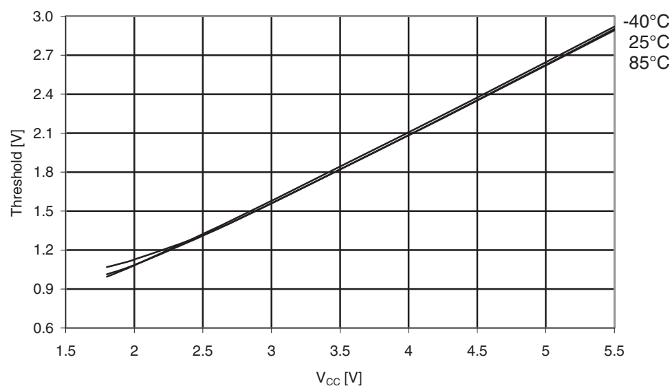
Figure 31-158. ATmega329A: I/O pin Input Threshold voltage vs. V_{CC} ( V_{IH} , I/O pin read as “1”).
