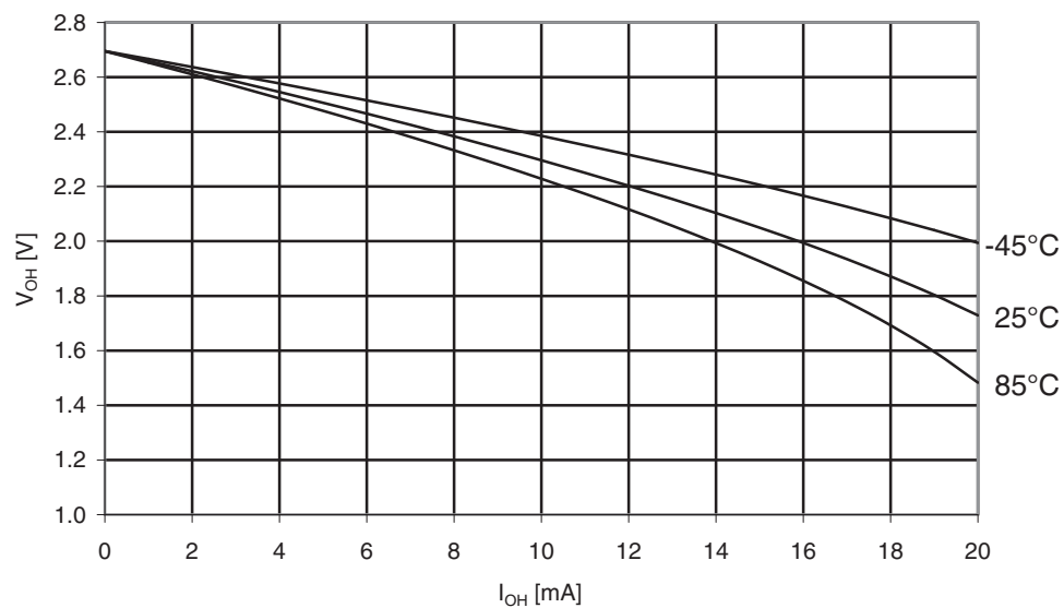
Figure 31-26. ATmega169A: I/O pin output voltage vs. source current, port B ( V_{CC} = 2.7V ).
