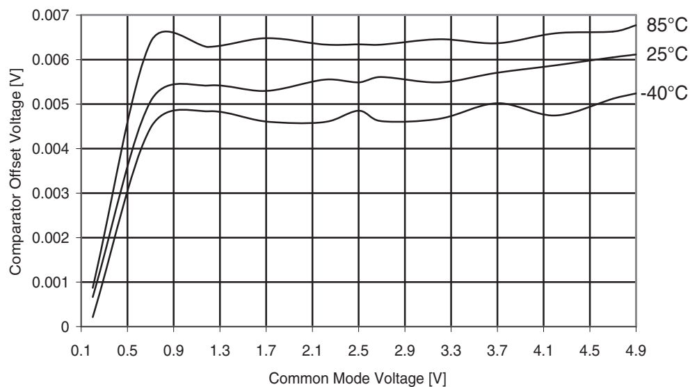
Figure 31-107. Atmel ATmega169PA: Analog Comparator offset voltage vs. Common Mode voltage ( V_{CC} = 5V ).
