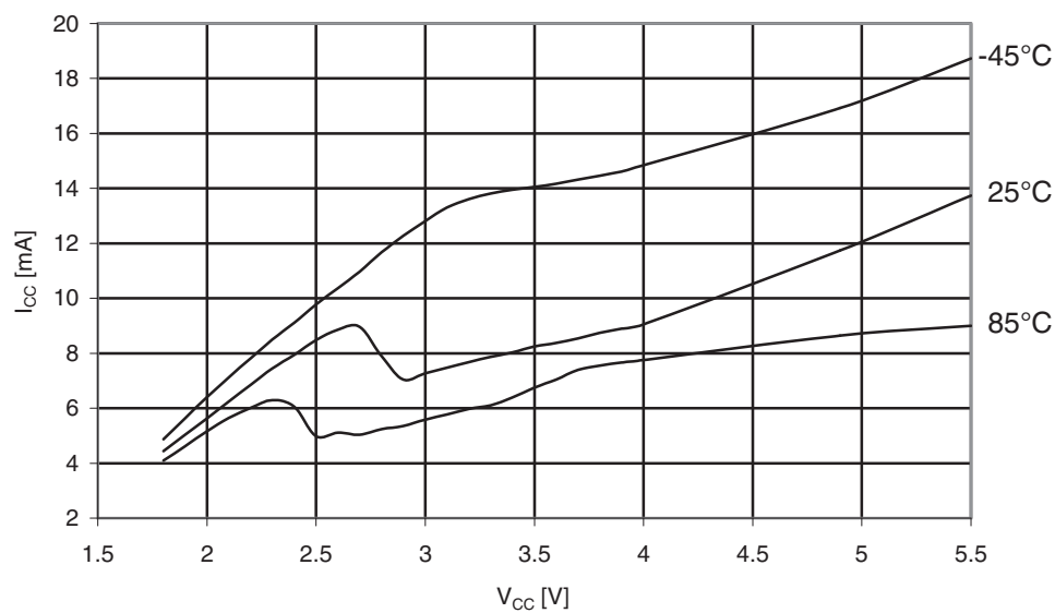
Figure 31-544. ATmega6490A: Programming current vs. V_{CC} .
