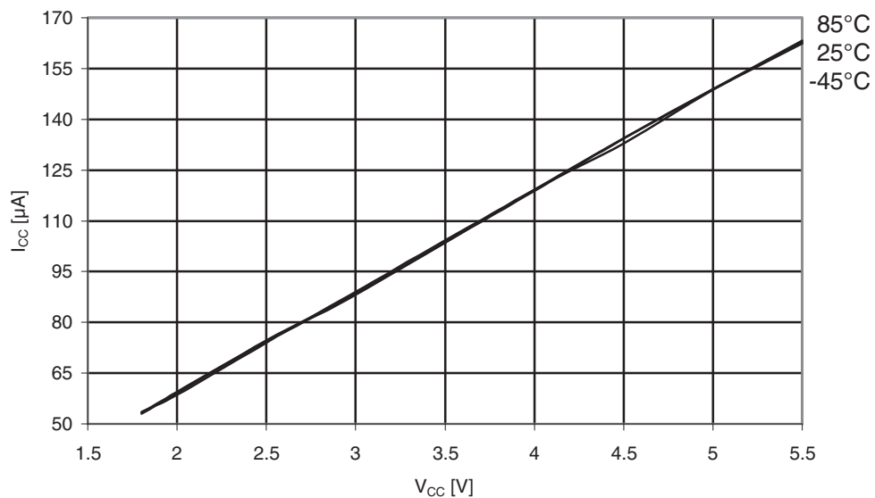
Figure 31-480. Atmel ATmega649P: AREF external reference current vs. V_{CC} .
