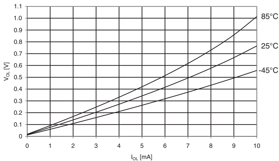
Figure 31-90. ATmega169PA: I/O pin output voltage vs. Sink current, ports A, C, D, E, F, G ( V_{CC} = 5V ).
