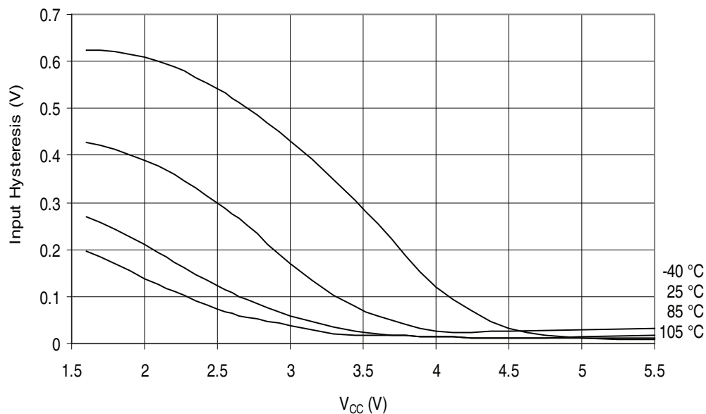
Figure 32-390. ATmega3290PA - 105°C: Reset Input Pin Hysteresis vs. V_{CC}
