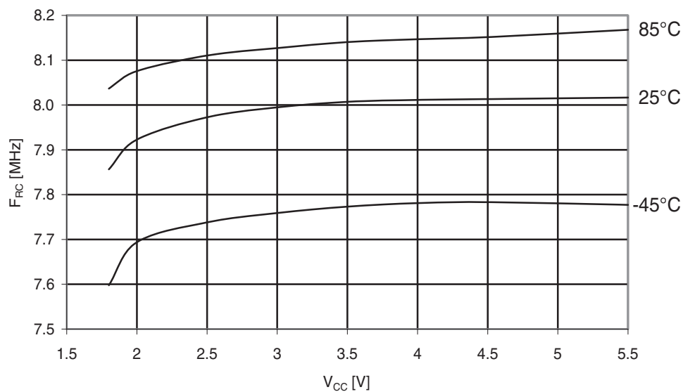
Figure 31-50. ATmega169A: Calibrated 8MHz RC oscillator frequency vs. V_{CC} .
