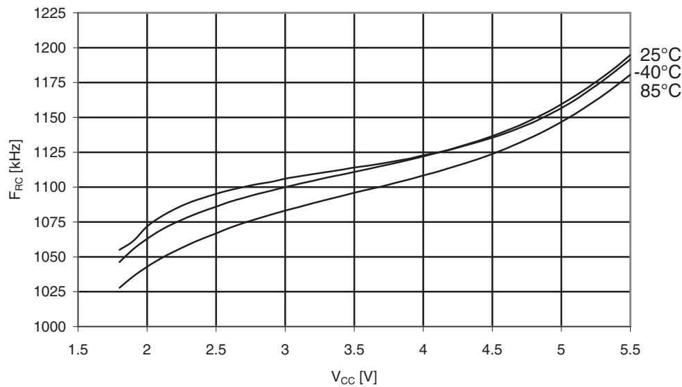
Figure 31-169. Atmel ATmega329A: Watchdog oscillator frequency vs. V_{CC} .
