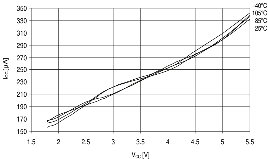
Figure 32-288. ATmega3290A - 105°C: Active Supply Current with ADC at 50kHz vs. V_{CC}
