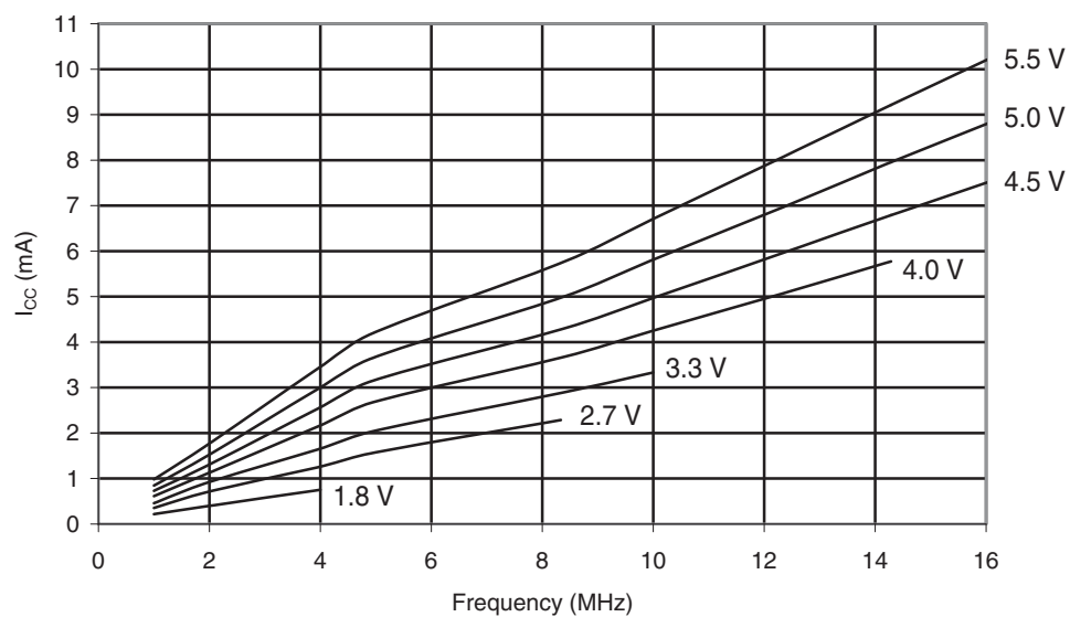
Figure 32-2. ATmega169PA-105°C: Active Supply Current vs. Frequency (1 - 16MHz)
