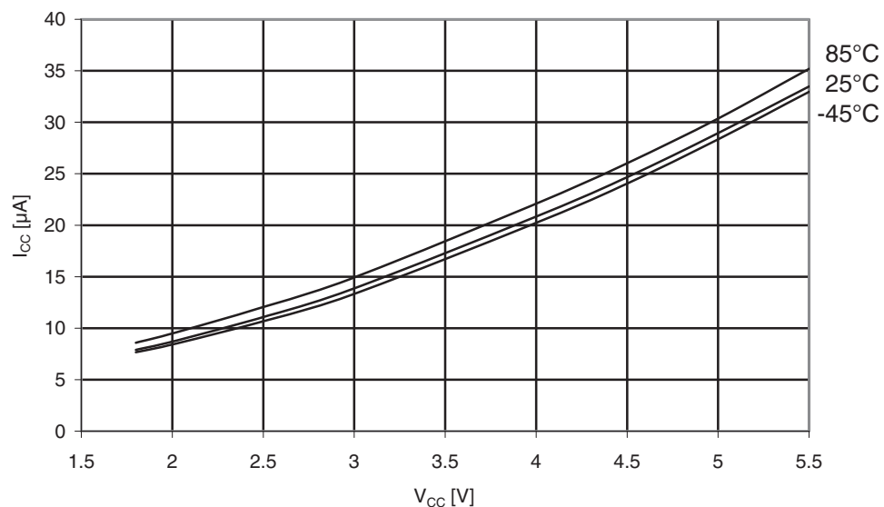
Figure 31-67. Atmel ATmega169PA: Active supply current vs. V_{CC} (32kHz watch XTAL).
