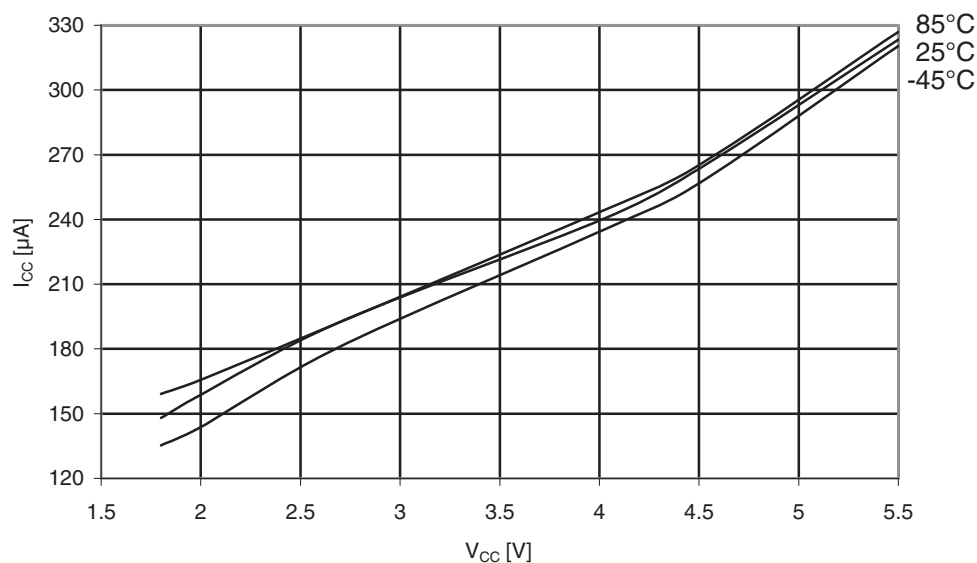
Figure 31-599. ATmega6490P: Active supply current with ADC at 50kHz vs. V_{CC} .
