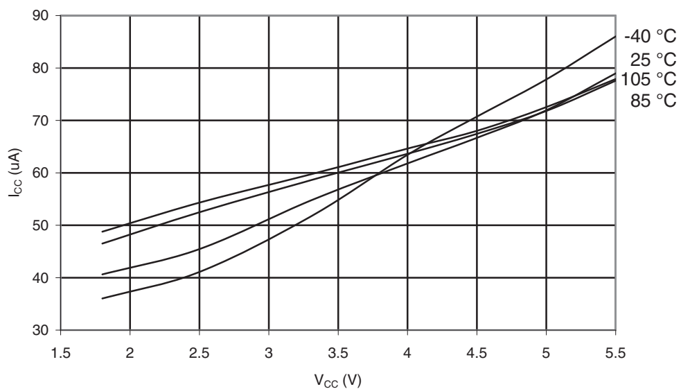
Figure 32-347. ATmega3290PA-105°C: Analog Comparator Current vs. V_{CC}
