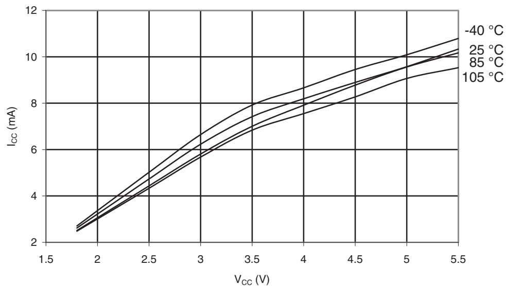
Figure 32-170. ATmega329P-105°C: Programming Current vs. V_{CC}
