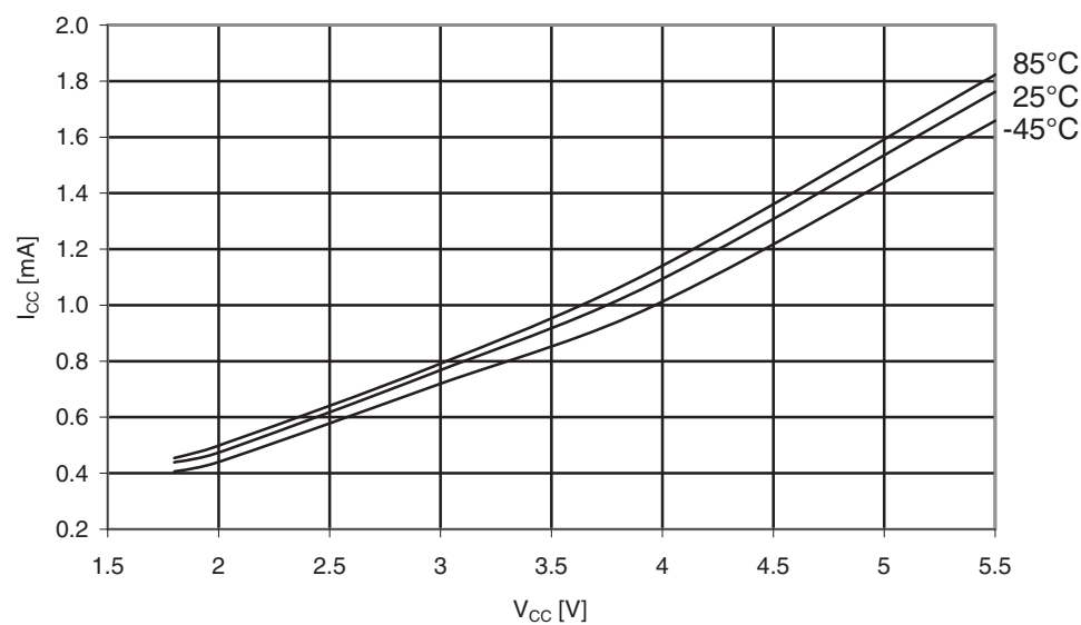
Figure 31-494. ATmega6490A: Idle supply current vs. V_{CC} (Internal RC oscillator, 8MHz).
