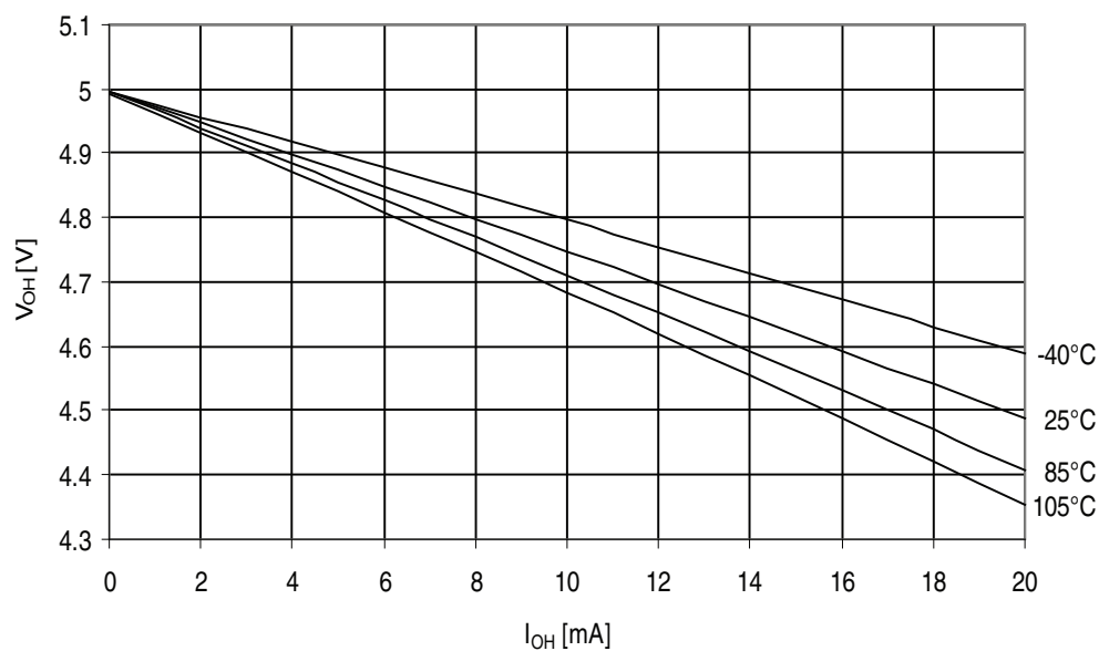
Figure 32-197. ATmega329PA - 105°C: I/O Pin Output Voltage vs. Source Current, Port B ( V_{CC} = 5V )
