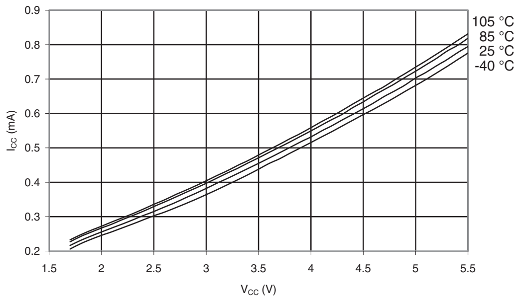
Figure 32-308. ATmega3290PA-105°C: Idle Supply Current vs. V_{CC} (Internal RC Oscillator, 1MHz)
