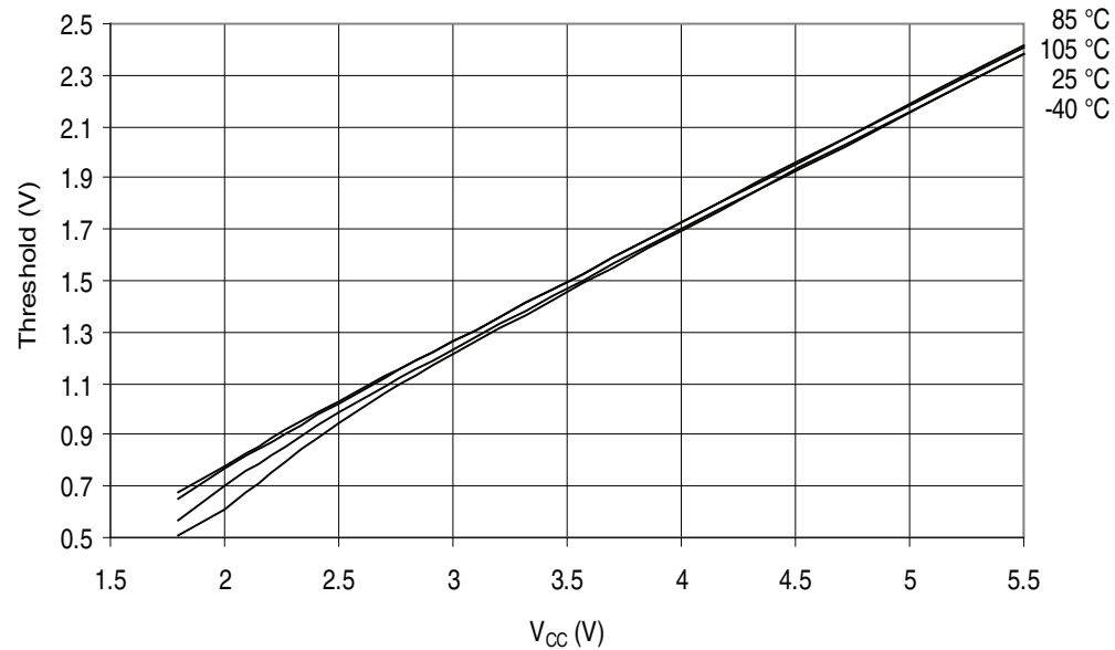
Figure 32-207. ATmega329PA - 105°C: I/O Pin Input Threshold Voltage vs. V_{CC} ( V_{IL} , I/O Pin Read as “0”)
