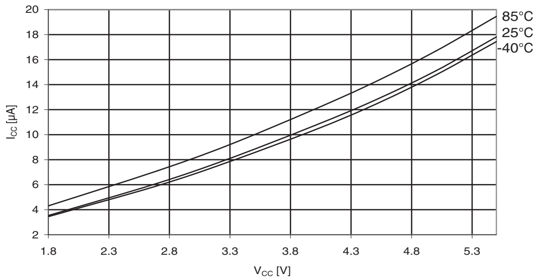
Figure 31-316. ATmega3290PA: Power-down Supply current vs. V_{CC} (Watchdog Timer enabled).
