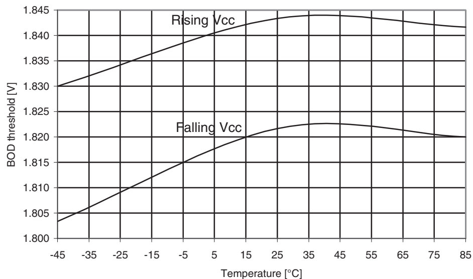
Figure 31-529. Atmel ATmega6490A: BOD Thresholds vs. temperature (BOD level is 1.8V).
