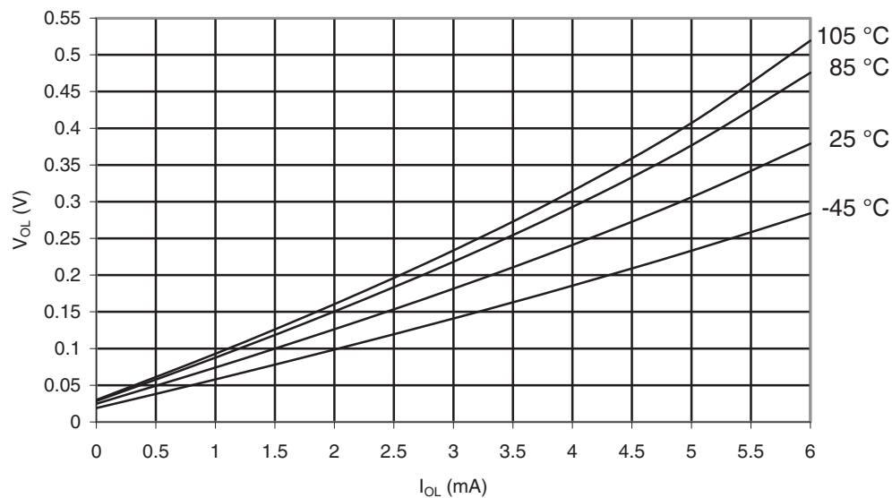
Figure 32-32. ATmega169PA-105°C: I/O Pin Output Voltage vs. Sink Current, Port B ( V_{CC} = 1.8V )
