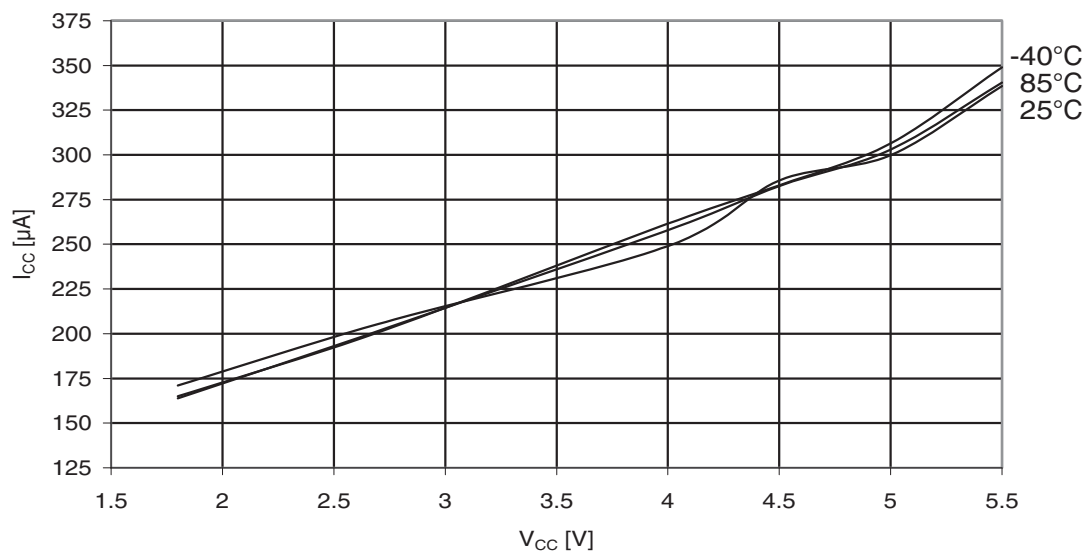
Figure 31-237. Atmel ATmega329PA: Active supply current with ADC at 1MHz vs. V_{CC} .
