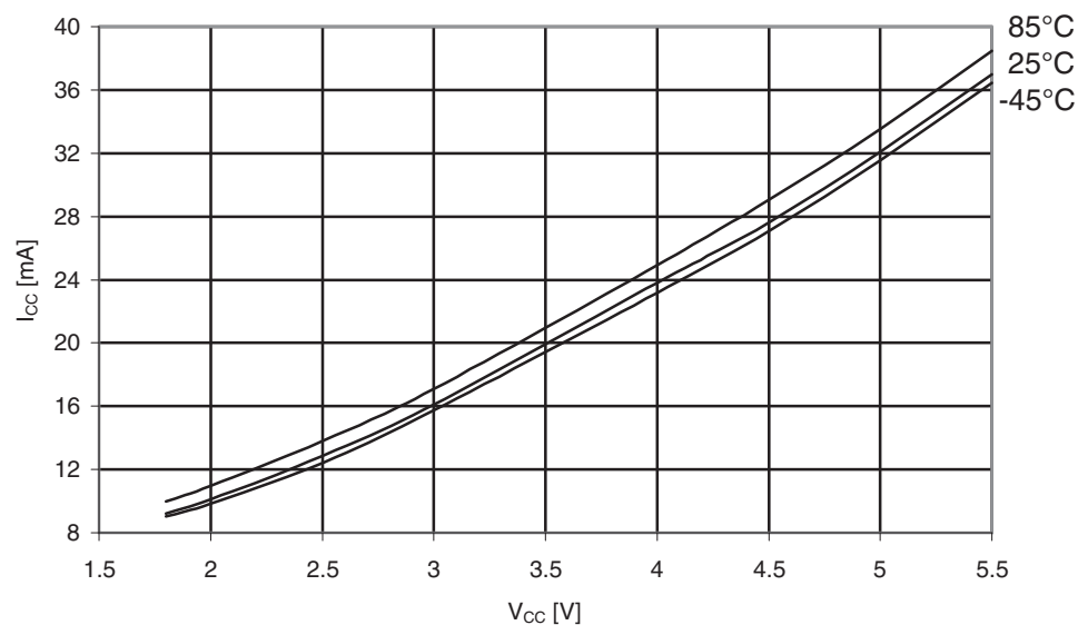
Figure 31-430. Atmel ATmega649P: Active supply current vs. V_{CC} (32kHz watch XTAL).
