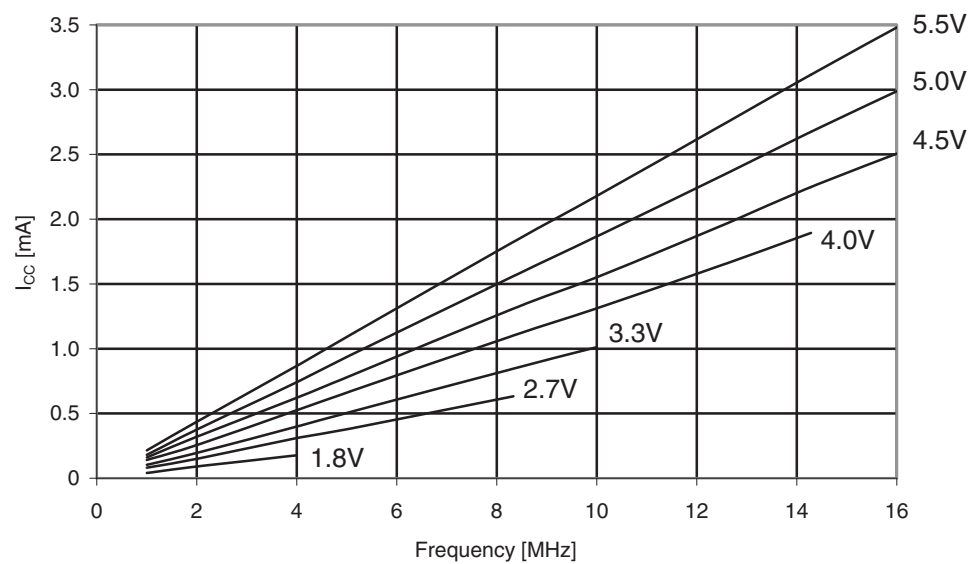
Figure 31-7. ATmega169A: Idle supply current vs. frequency (1 - 16MHz).
