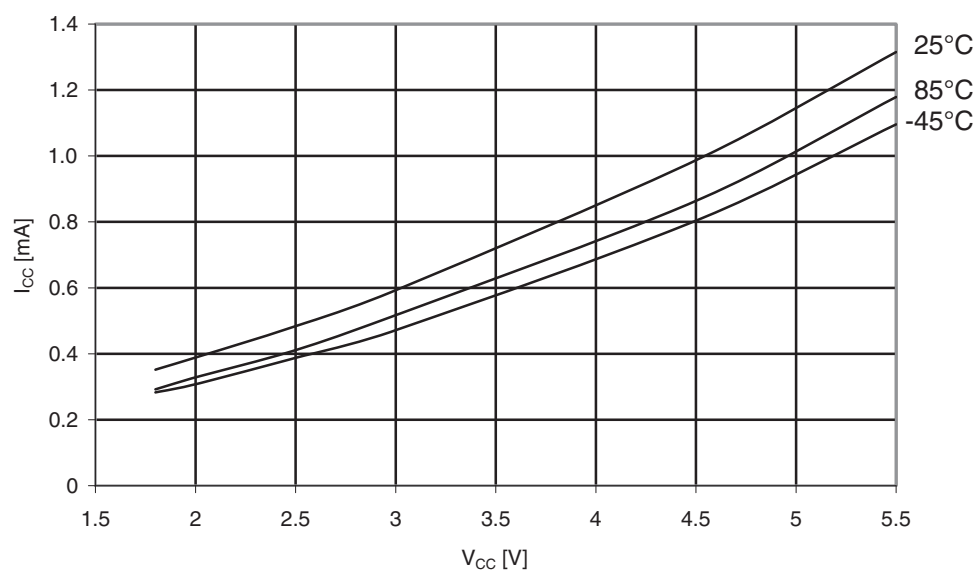
Figure 31-4. Atmel ATmega169A: Active supply current vs. V_{CC} (Internal RC oscillator, 1MHz).
