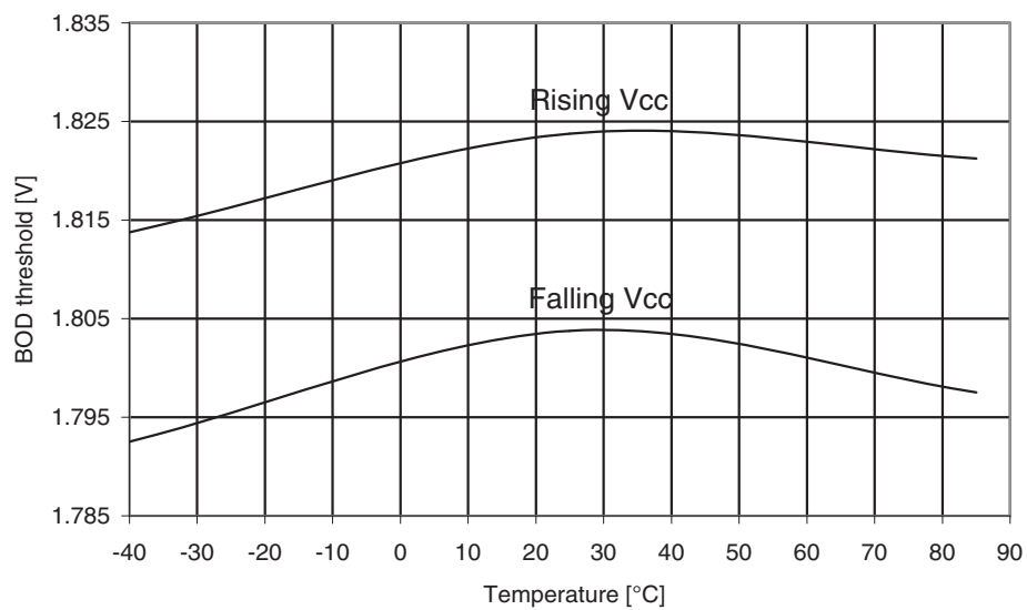
Figure 31-166. ATmega329A: BOD Thresholds vs. temperature (BOD level is 1.8V).
