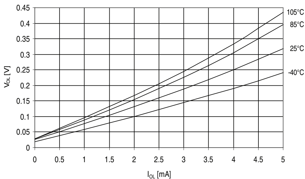
Figure 32-205. ATmega329PA - 105°C: I/O Pin Output Voltage vs. Sink Current, Port B ( V_{CC} = 1.8V )
