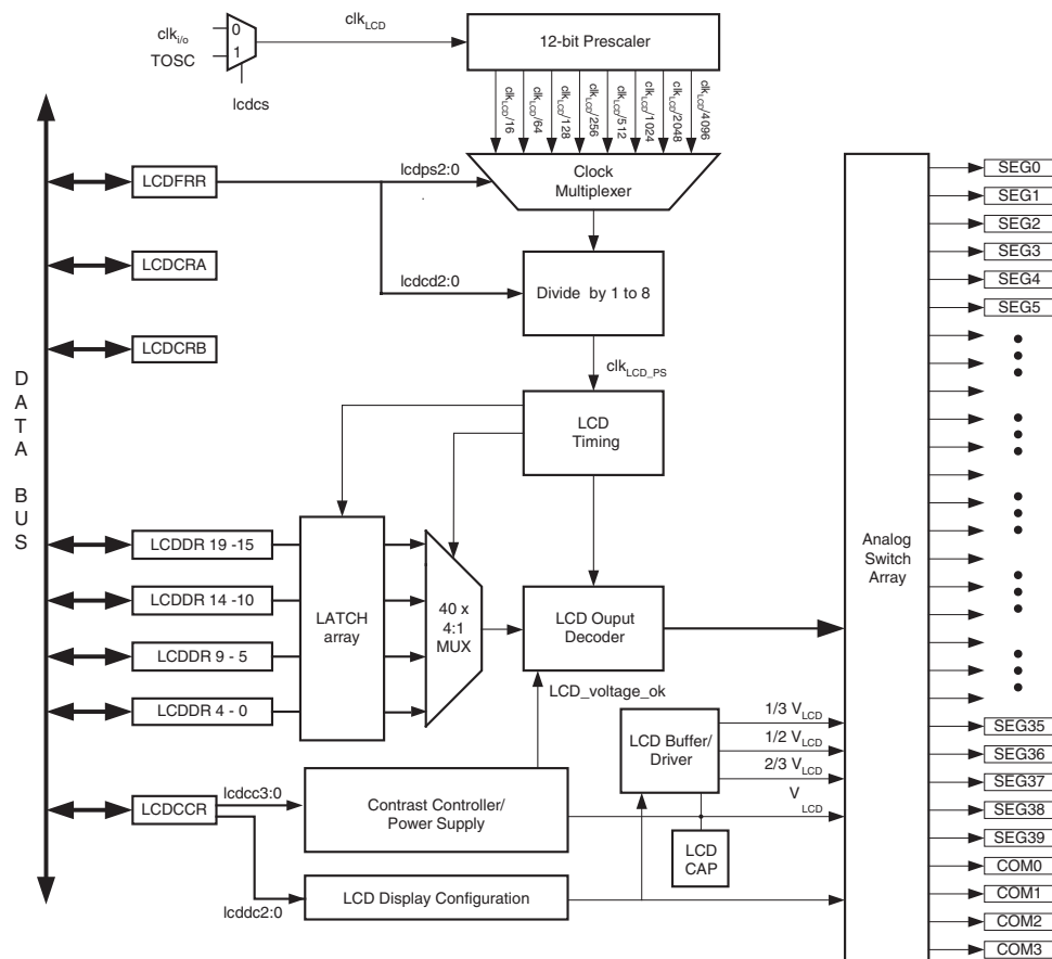
Figure 24-1. LCD Module, block diagram.
