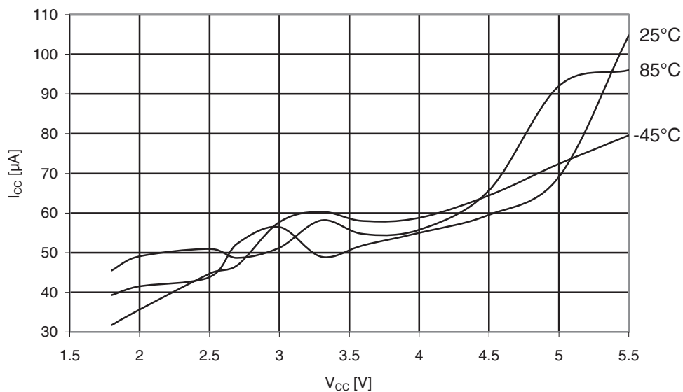
Figure 31-482. Atmel ATmega649P: Analog Comparator current vs. V_{CC} .
