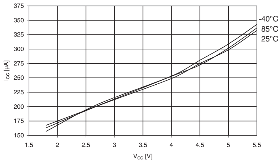
Figure 31-175. Atmel ATmega329A: Active supply current with ADC at 50kHz vs. V_{CC} .
