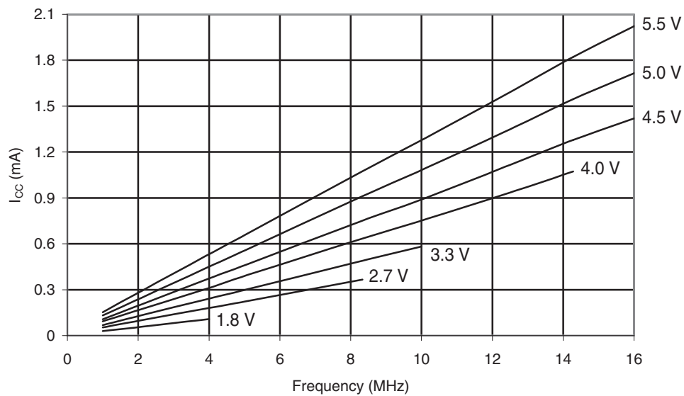
Figure 32-57. ATmega169PA-105°C: Reset Supply Current vs. V_{CC} (1 - 16 MHz, Excluding Current Through The Reset Pull-up)
