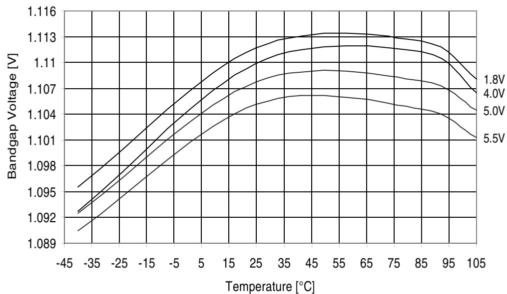
Figure 32-101. ATmega329A - 105°C: Bandgap Voltage vs. Temperature
