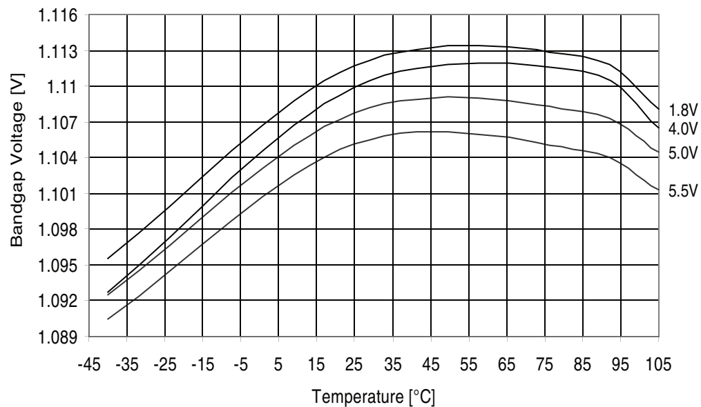
Figure 32-395. ATmega3290PA: Bandgap Voltage vs. Temperature
