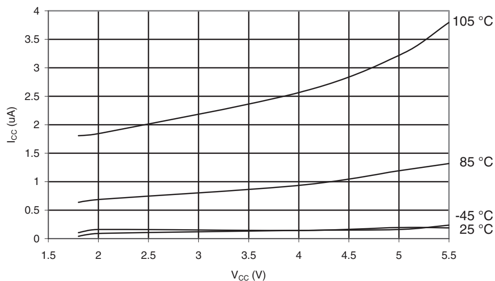
Figure 32-11. ATmega169PA-105°C: Power-down Supply Current vs. V_{CC} (Watchdog Timer Disabled)
