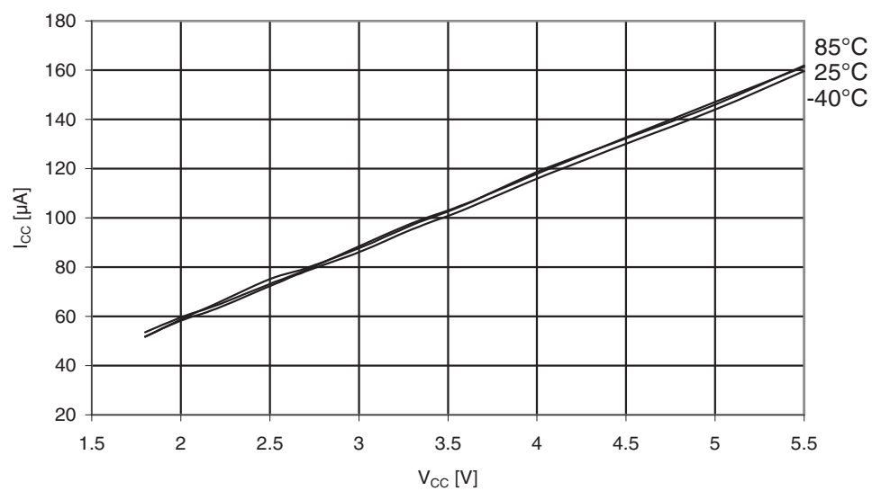
Figure 31-298. ATmega3290A: AREF external reference current vs. V_{CC} .
