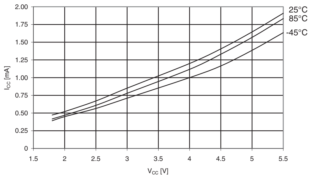
Figure 31-70. ATmega169PA: Idle supply current vs. V_{CC} (Internal RC oscillator, 8MHz).
