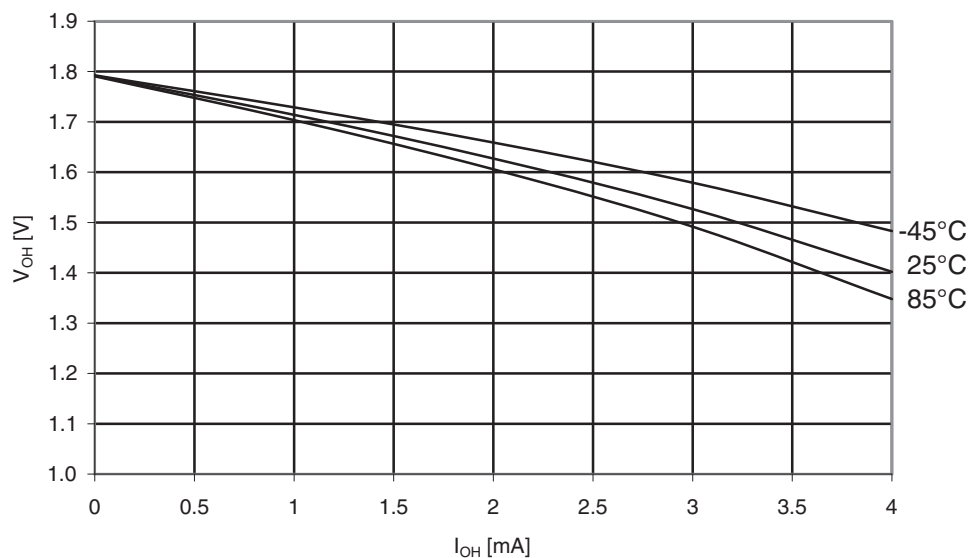
Figure 31-24. ATmega169A: I/O pin output voltage vs. source current, ports A, C, D, E, F, G ( V_{CC} = 1.8V ).
