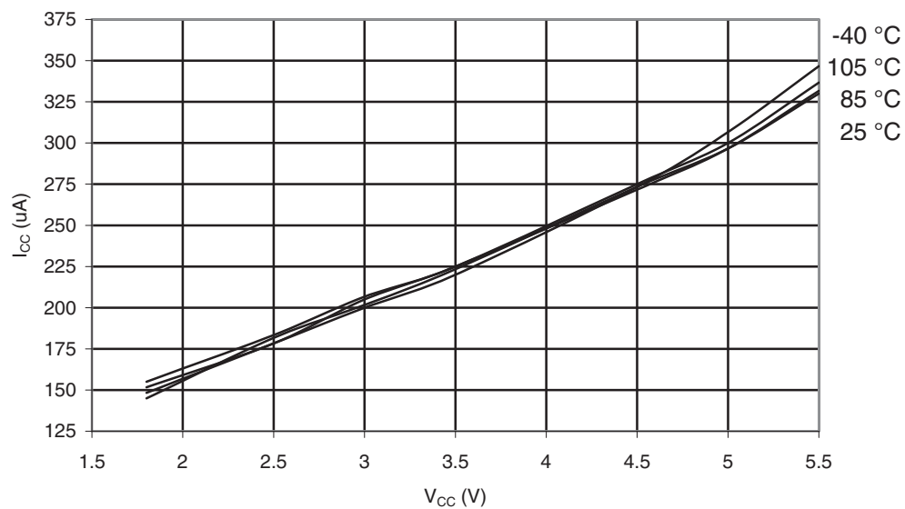
Figure 32-344. ATmega3290PA-105°C: Active supply current with ADC vs. V_{CC}
