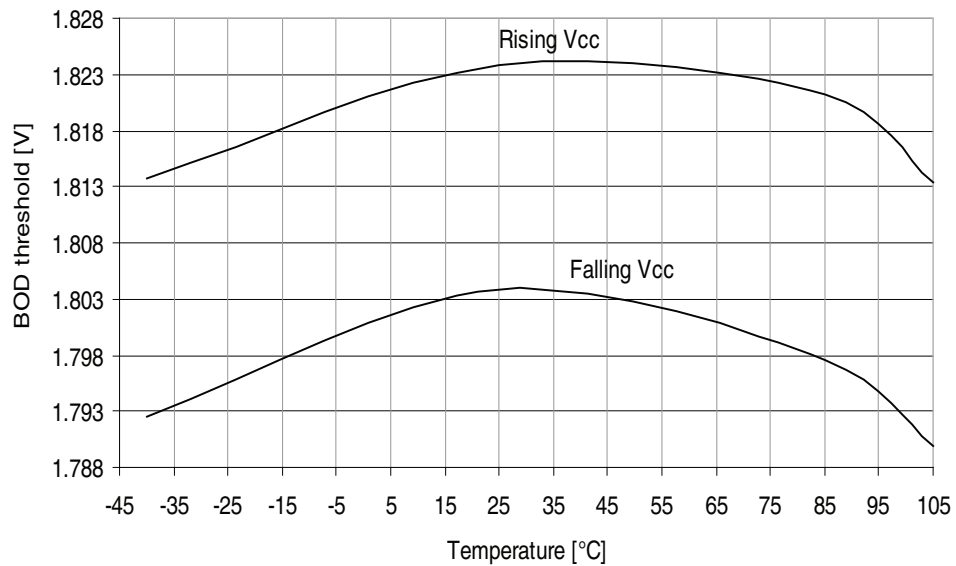
Figure 32-277. ATmega3290A - 105°C: BOD Thresholds vs. Temperature (BOD Level is 1.8V)
