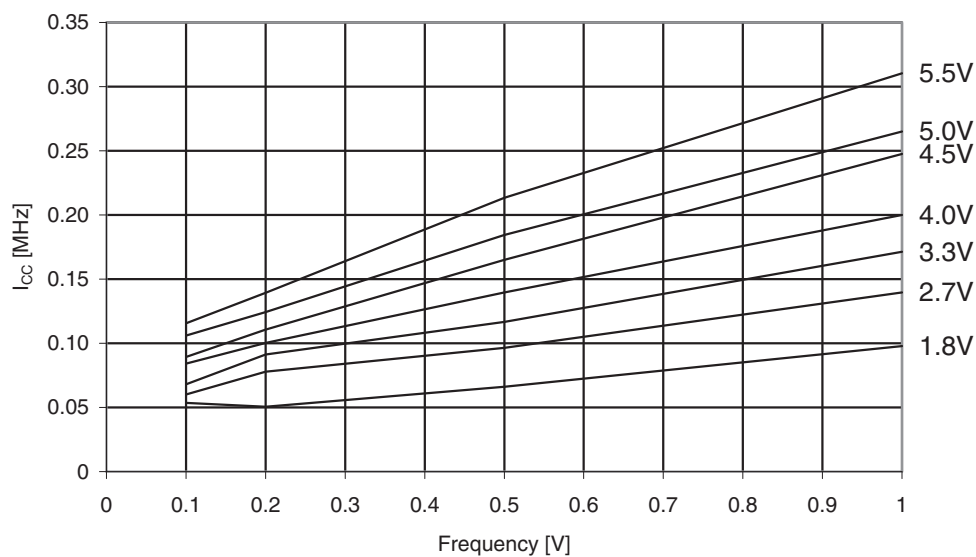
Figure 31-310. ATmega3290PA: Idle supply current vs. low frequency (0.1 - 1.0MHz).
