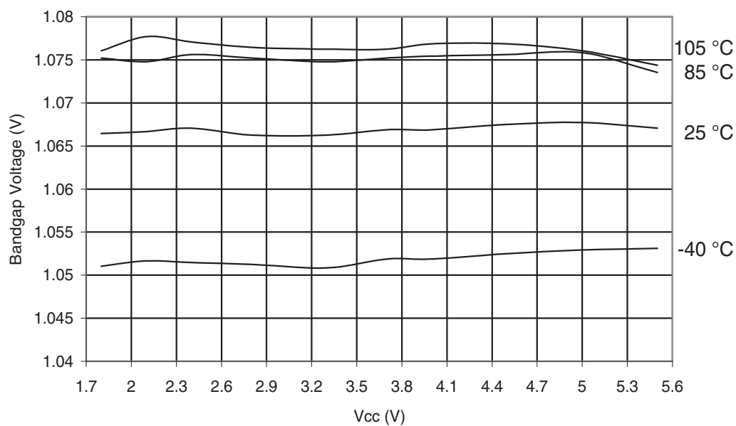
Figure 32-159. ATmega329P-105°C: Bandgap Voltage vs. V_{CC}
