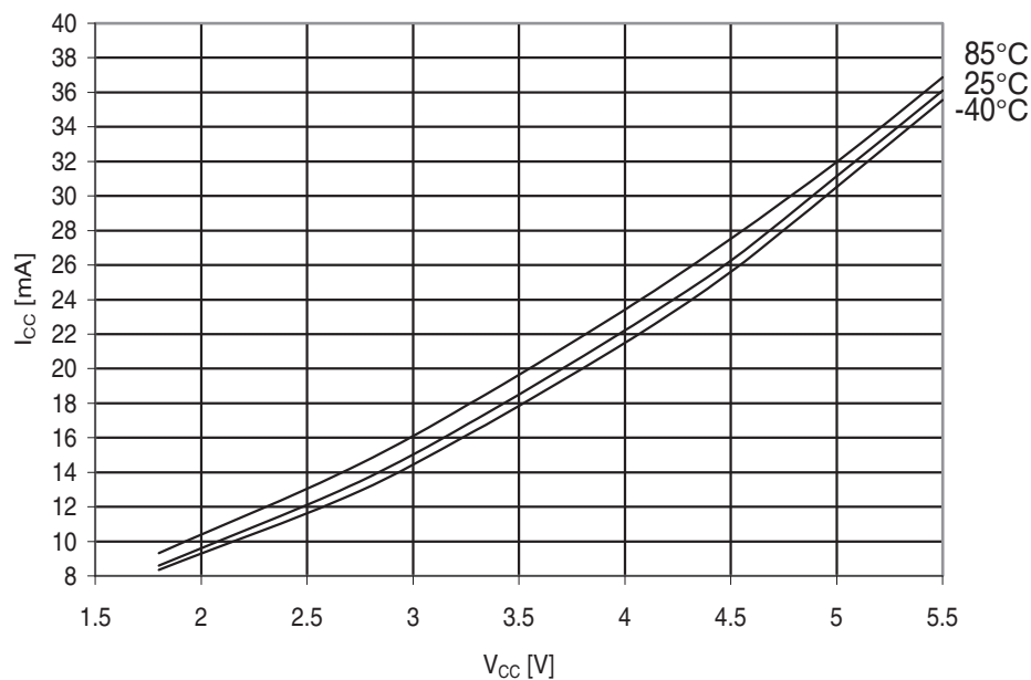
Figure 31-249. Atmel ATmega3290A: Active supply current vs. V_{CC} (32kHz watch XTAL).
