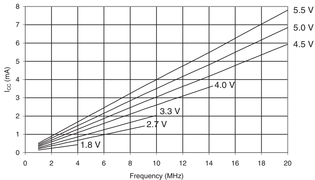
Figure 32-306. ATmega3290PA-105°C: Idle Supply Current vs. Frequency (1 - 20MHz)
