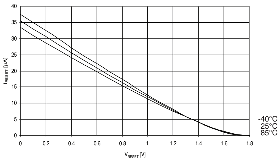
Figure 31-145. Atmel ATmega329A: Reset pull-up resistor current vs. reset pin voltage ( V_{CC} = 1.8V ).
