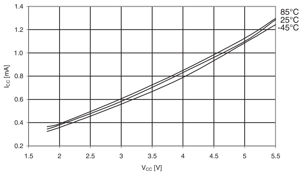
Figure 31-429. ATmega649P: Active supply current vs. V_{CC} (Internal RC oscillator, 1MHz).
