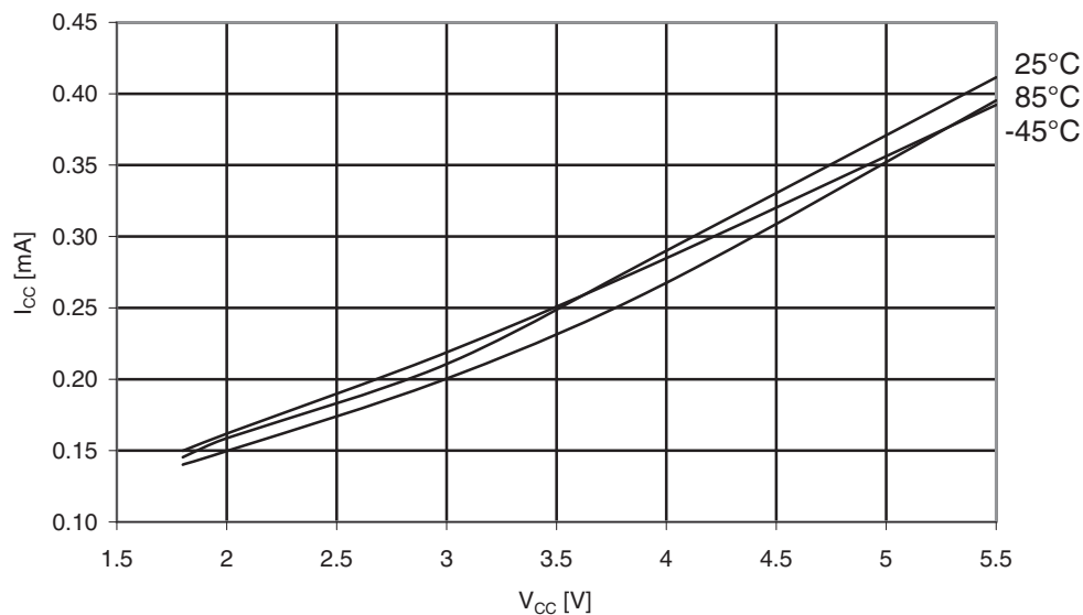
Figure 31-434. Atmel ATmega649P: Idle supply current vs. V_{CC} (Internal RC oscillator, 1MHz).
