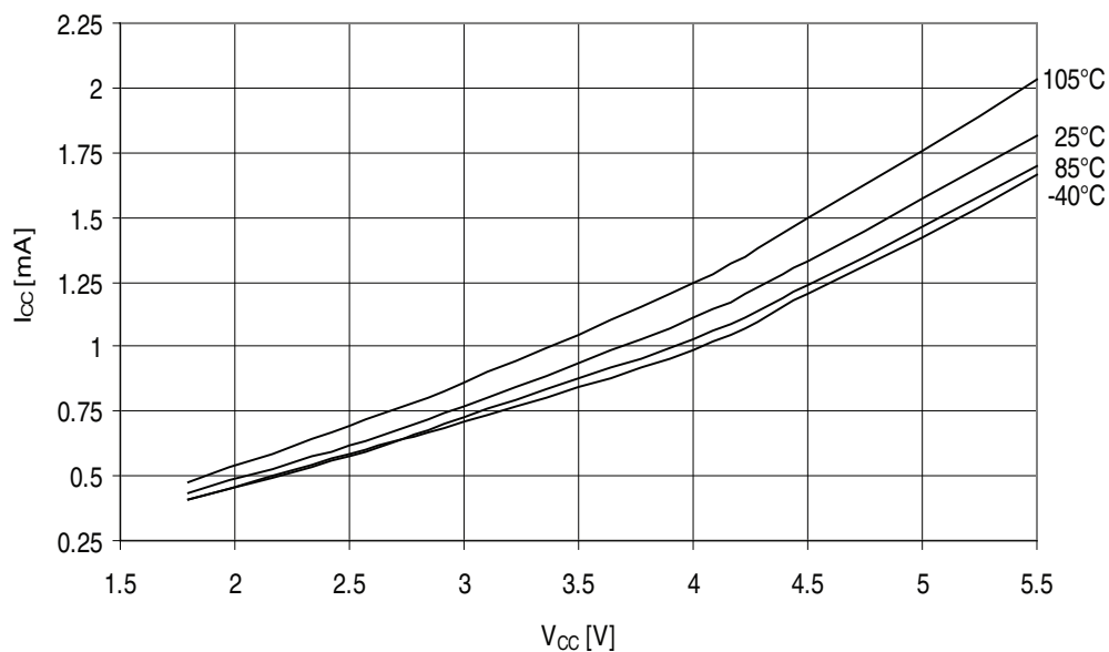
Figure 32-181. ATmega329PA - 105°C: Idle Supply Current vs. V CC (Internal RC Oscillator, 8 MHz)
