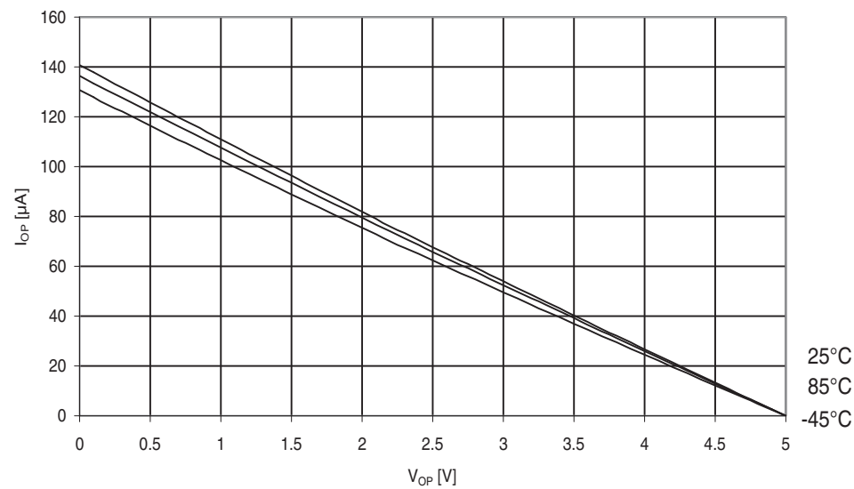
Figure 31-442. Atmel ATmega649P: I/O pin pull-up resistor current vs. input voltage ( V_{CC} = 5V ).
