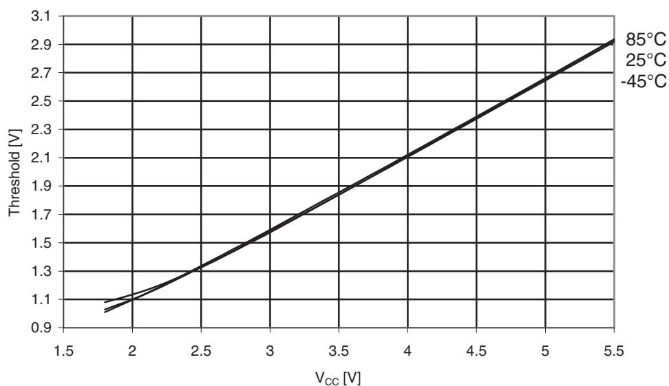
Figure 31-34. ATmega169A: I/O pin input Threshold voltage vs. V_{CC} ( V_{IH} , I/O pin read as “1”).
