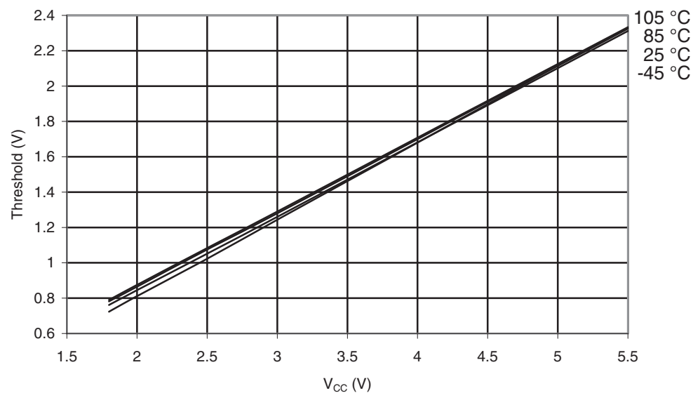
Figure 32-37. ATmega169PA-105°C: Reset Input Threshold Voltage vs. V_{CC} ( V_{IL} , Reset Pin Read as “0”)
