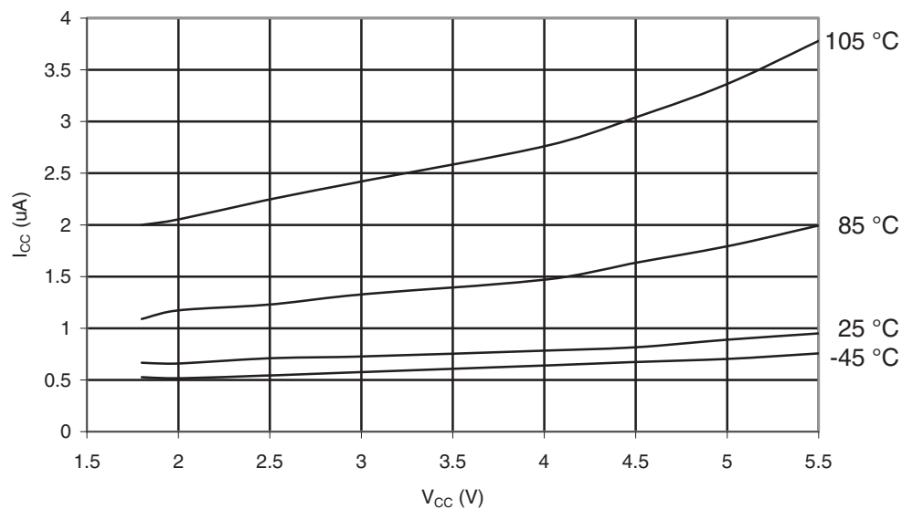
Figure 32-14. ATmega169PA-105°C: Standby Supply Current vs. V_{CC} (32 kHz Watch Crystal, Watchdog Timer Disabled)
