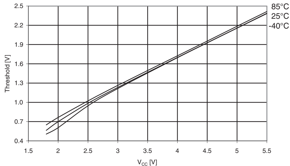
Figure 31-219. Atmel ATmega329PA. I/O pin Input Threshold voltage vs. V_{CC} ( V_{IL} , I/O pin read as “0”).
