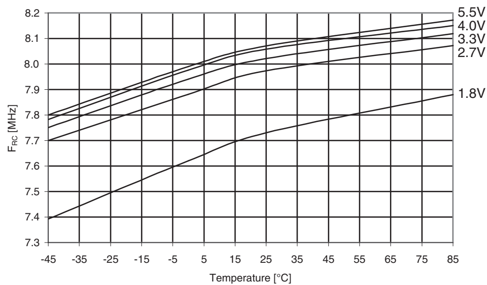
Figure 31-534. ATmega6490A: Calibrated 8MHz RC oscillator frequency vs. temperature.
