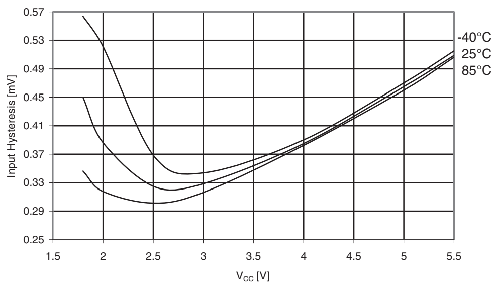
Figure 31-340. Atmel ATmega3290PA: I/O pin Input Hysteresis vs. V_{CC} .
