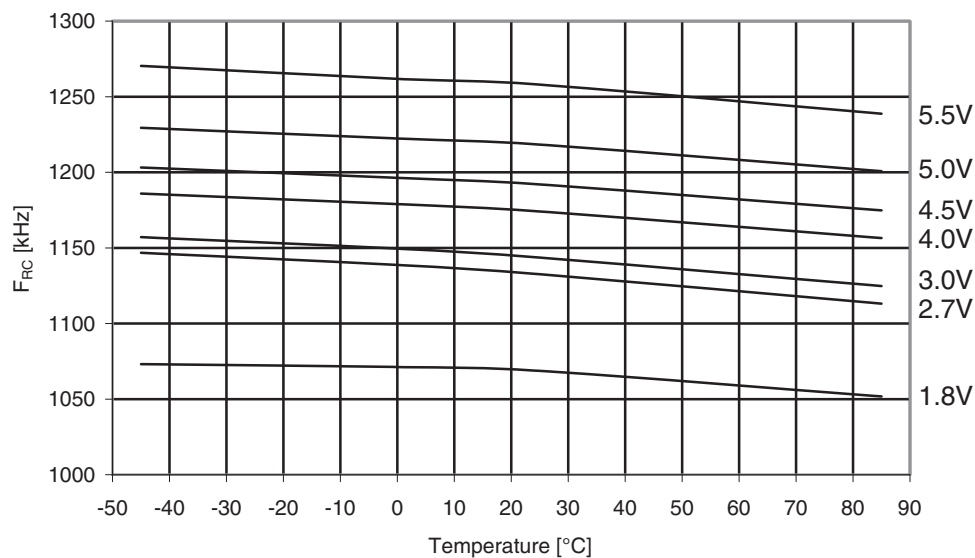
Figure 31-110. ATmega169PA: Watchdog oscillator frequency vs. temperature.
