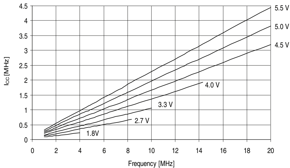
Figure 32-243. ATmega3290A - 105°C: Idle Supply Current vs. Frequency (1 - 20MHz)
