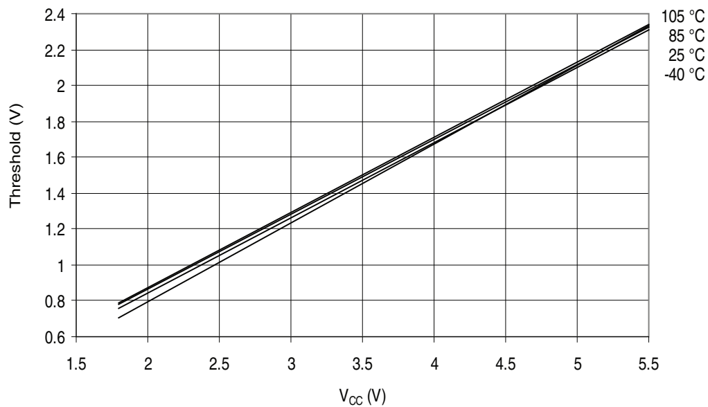
Figure 32-273. ATmega3290A - 105°C: Reset Input Threshold Voltage vs. V_{CC} ( V_{IL} , Reset Pin Read as “0”)
