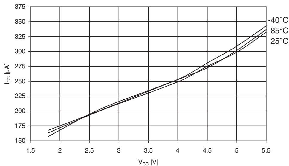
Figure 31-235. Atmel ATmega329PA: Active supply current with ADC at 50kHz vs. V_{CC} .
