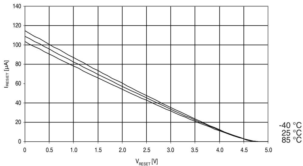
Figure 31-143. Atmel ATmega329A: Reset pull-up resistor current vs. reset pin voltage ( V_{CC} = 5V ).
