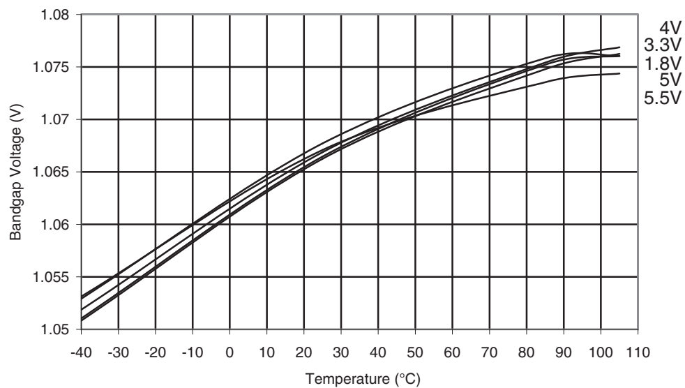
Figure 32-338. ATmega3290PA-105°C: Bandgap Voltage vs. Temperature
