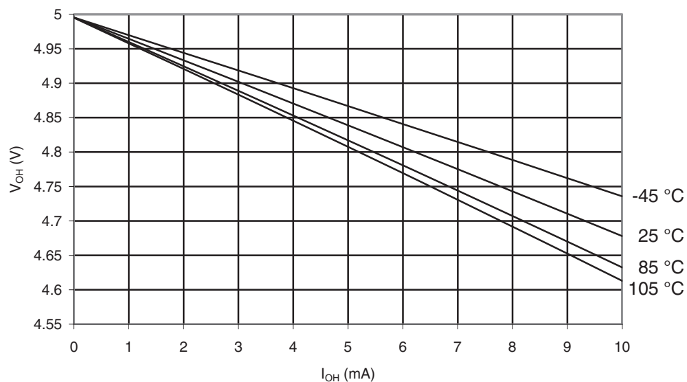
Figure 32-21. ATmega169PA-105°C: I/O Pin Output Voltage vs. Source Current, Ports A, C, D, E, F, G ( V_{CC} = 5V )
