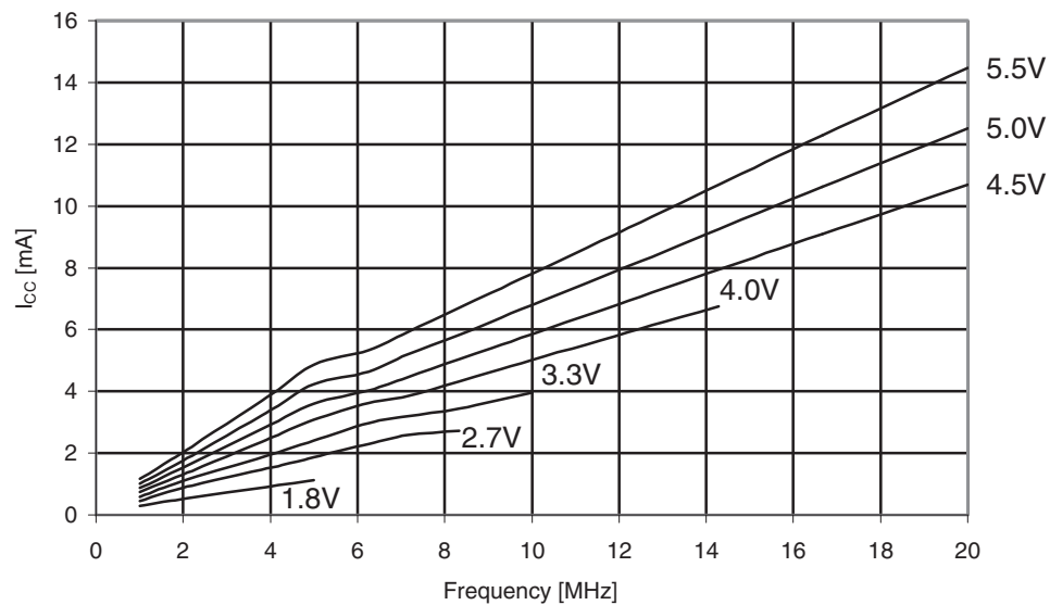
Figure 31-488. ATmega6490A: Active supply current vs. frequency (1 - 20MHz).
