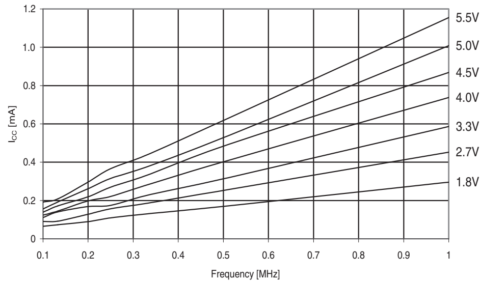
Figure 31-426. ATmega649P: Active supply current vs. low frequency (0.1 - 1.0MHz).
