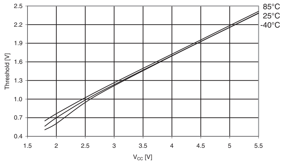
Figure 31-339. ATmega3290PA. I/O pin Input Threshold voltage vs. V_{CC} ( V_{IL} , I/O pin read as “0”).
