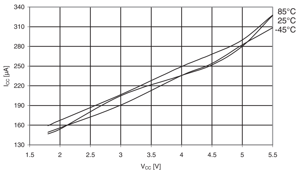
Figure 31-601. ATmega6490P: Active supply current with ADC at 1MHz vs. V_{CC} .
