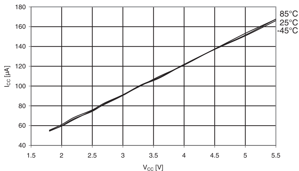
Figure 31-56. ATmega169A: AREF external reference current vs. V_{CC} .
