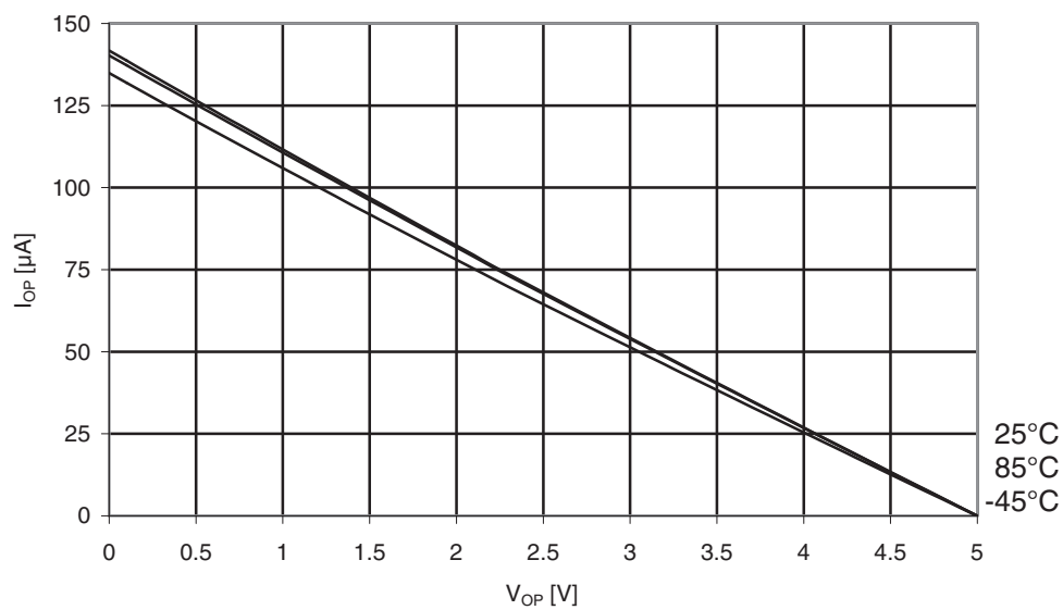
Figure 31-78. ATmega169PA: I/O pin pull-up resistor current vs. input voltage ( V_{CC} = 5V ).
