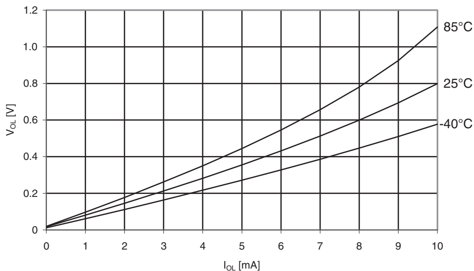
Figure 31-213. Atmel ATmega329PA. I/O pin output voltage vs. sink current, ports A, C, D, E, F, G ( V_{CC} = 2.7V ).
