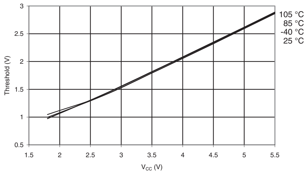
Figure 32-150. ATmega329P-105°C: I/O Pin Input Threshold Voltage vs. V_{CC} ( V_{IH} , I/O Pin Read as “1”)
