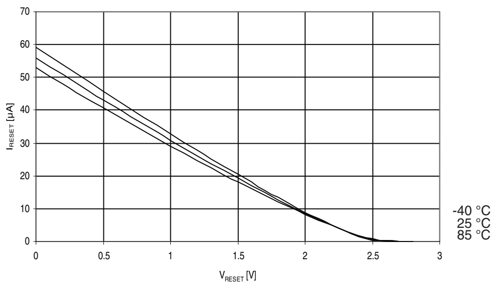
Figure 31-144. ATmega329A: Reset pull-up resistor current vs. reset pin voltage ( V_{CC} = 2.7V ).
