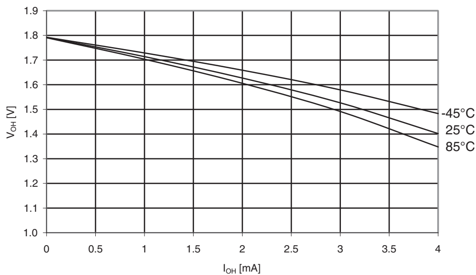
Figure 31-86. ATmega169PA: I/O pin output voltage vs. Source current, ports A, C, D, E, F, G ( V_{CC} = 1.8V ).
