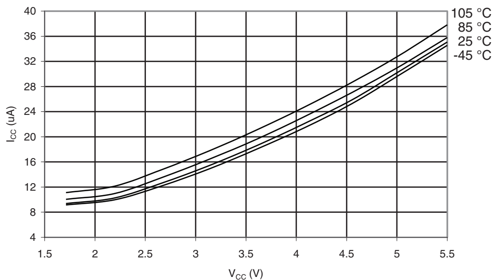
Figure 32-356. ATmega3290PA - 105°C: Active Supply Current vs. V_{CC} (32kHz Watch Crystal)
