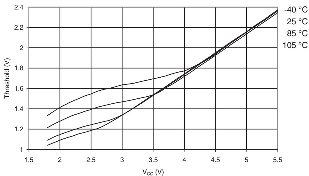
Figure 32-331. ATmega3290PA-105°C: Reset Input Threshold Voltage vs. V_{CC} ( V_{IH} , Reset Pin Read as “1”)
