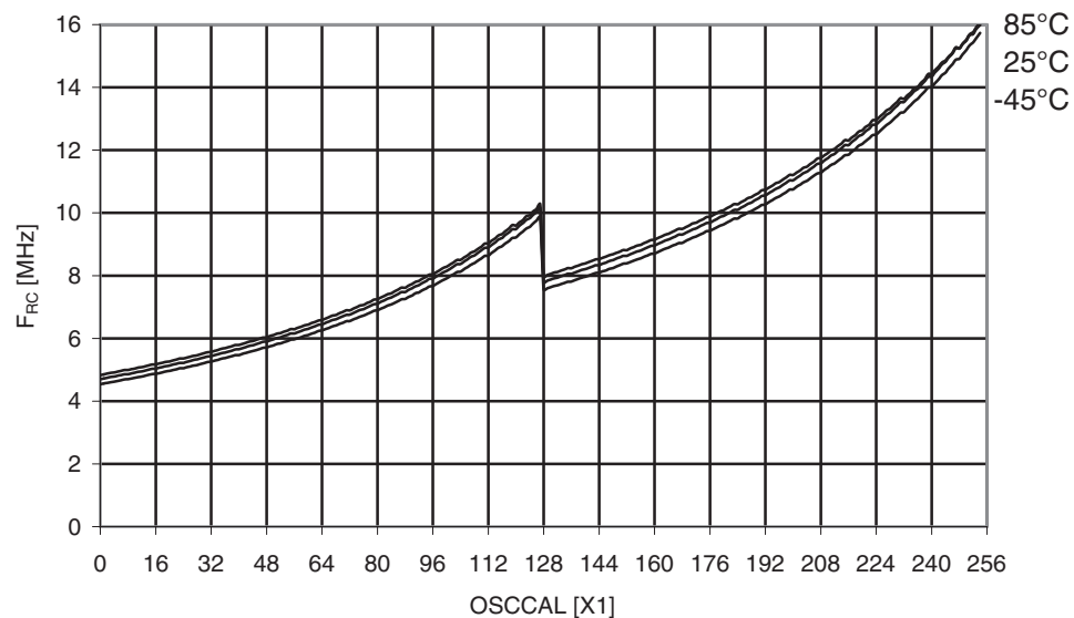
Figure 31-51. Atmel ATmega169A: Calibrated 8MHz RC oscillator frequency vs. Oscscal value.
