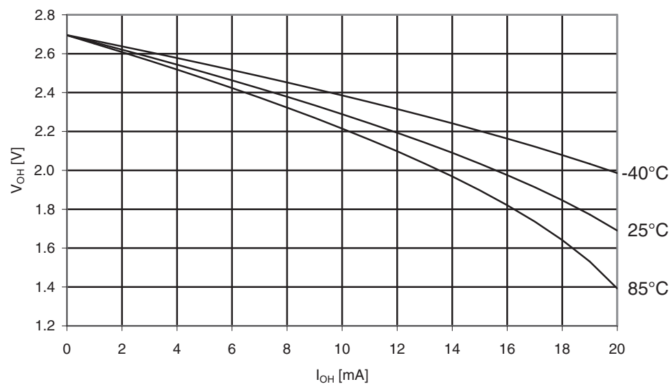
Figure 31-150. ATmega329A: I/O pin output voltage vs. source current, port B ( V_{CC} = 2.7V ).
