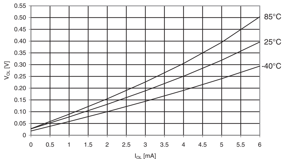
Figure 31-337. ATmega3290PA: I/O pin output voltage vs. sink current, port B ( V_{CC} = 1.8V ).
