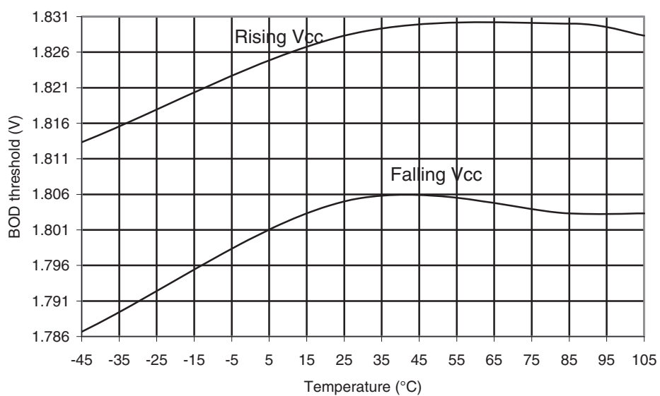
Figure 32-41. ATmega169PA-105°C: BOD Thresholds vs. Temperature (BOD Level is 1.8V)
