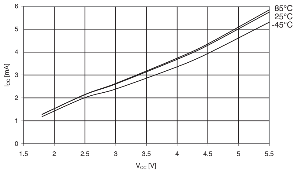
Figure 31-3. ATmega169A: Active supply current vs. V_{CC} (Internal RC oscillator, 8MHz).
