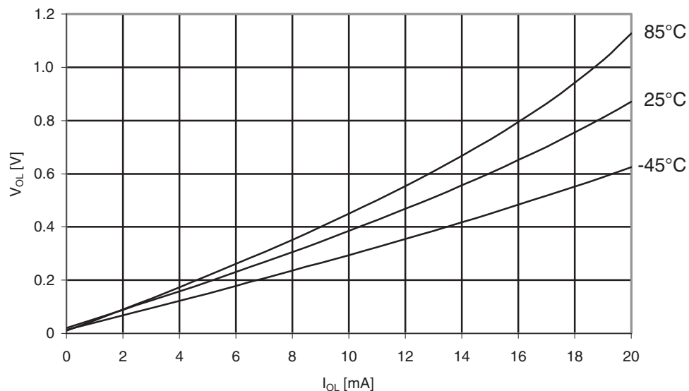
Figure 31-580. Atmel ATmega6490P: I/O pin output voltage vs. sink current, port B ( V_{CC} = 2.7V ).
