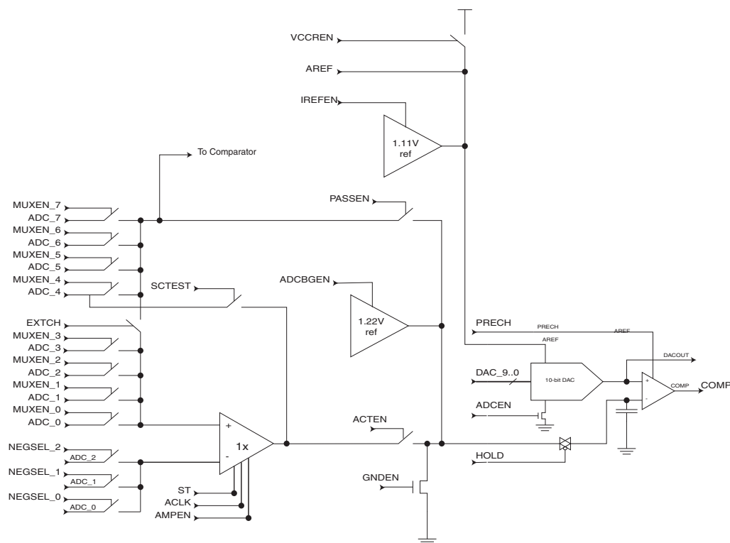
Figure 26-8. Analog to Digital Converter.
