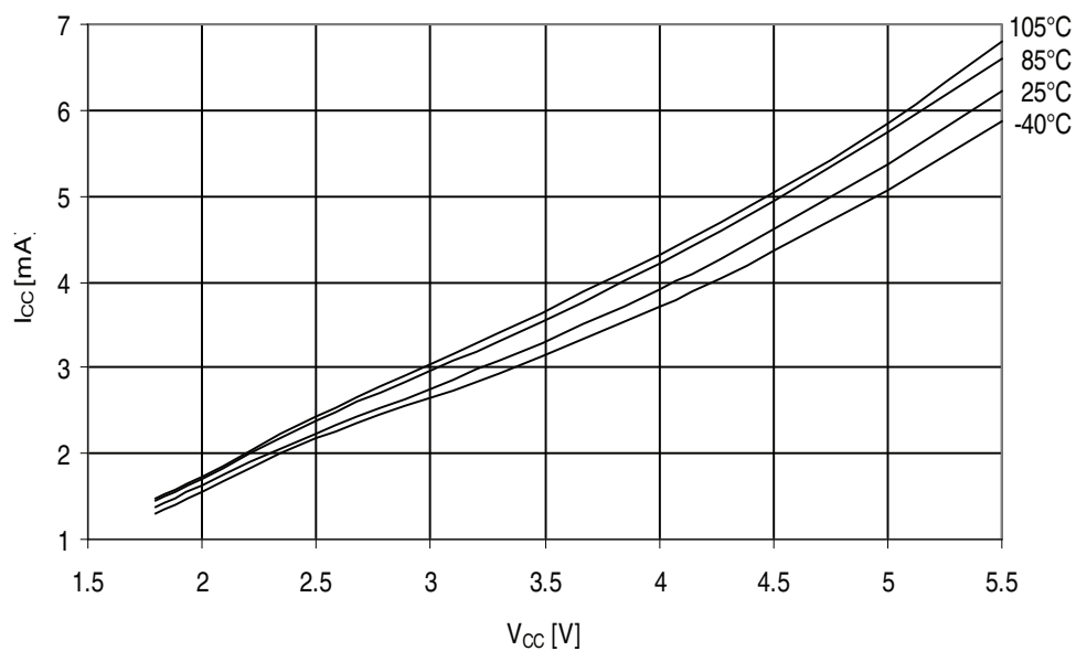
Figure 32-240. ATmega3290A - 105°C: Active Supply Current vs. V_{CC} (Internal RC Oscillator, 1 MHz)
