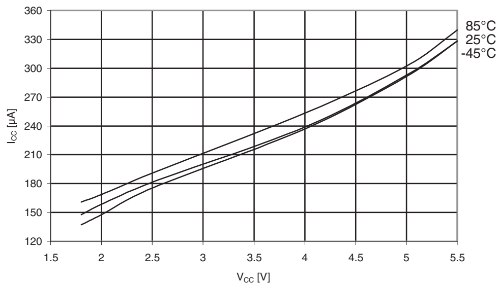
Figure 31-417. Atmel ATmega649A: Active supply current with ADC at 200kHz vs. V_{CC} .
