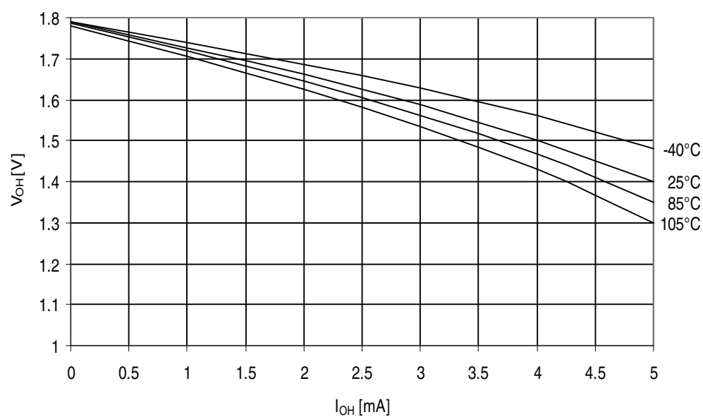
Figure 32-84. ATmega329A - 105°C: I/O Pin Output Voltage vs. Source Current, Port B ( V_{CC} = 1.8V )
