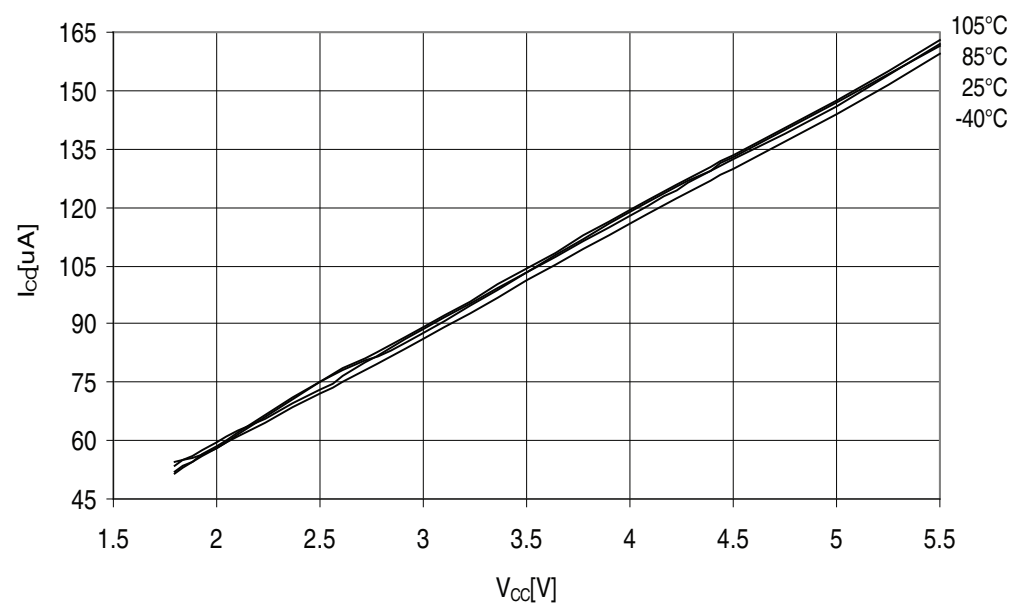
Figure 32-292. ATmega3290A - 105°C: AREF External Reference Current vs. V_{CC}
