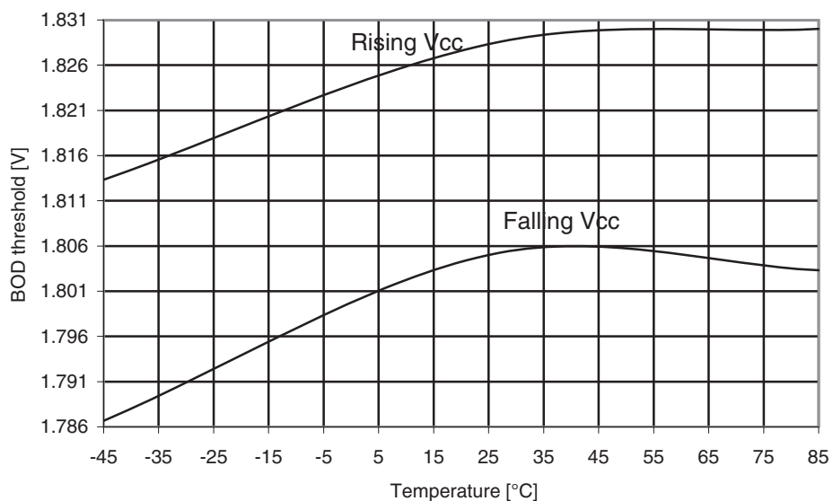
Figure 31-42. ATmega169A: BOD Thresholds vs. temperature (BOD level is 1.8V).
