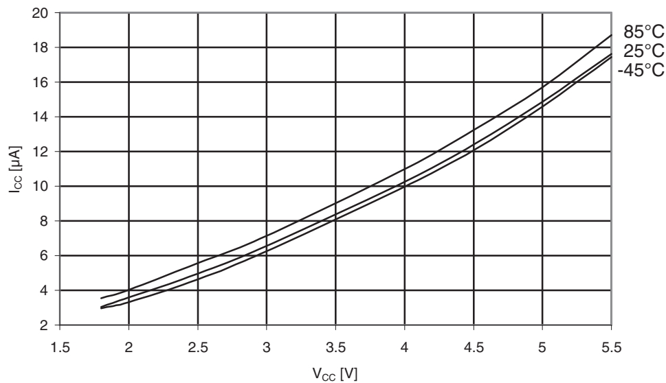
Figure 31-559. ATmega6490P: Power-down supply current vs. V_{CC} (Watchdog Timer enabled).
