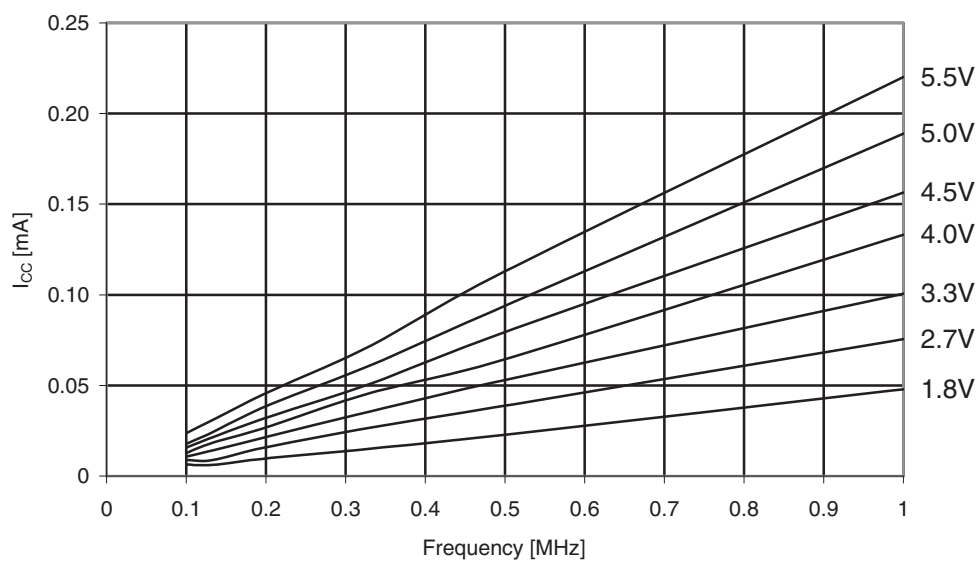
Figure 31-68. ATmega169PA: Idle supply current vs. frequency (0.1 - 1.0MHz).
