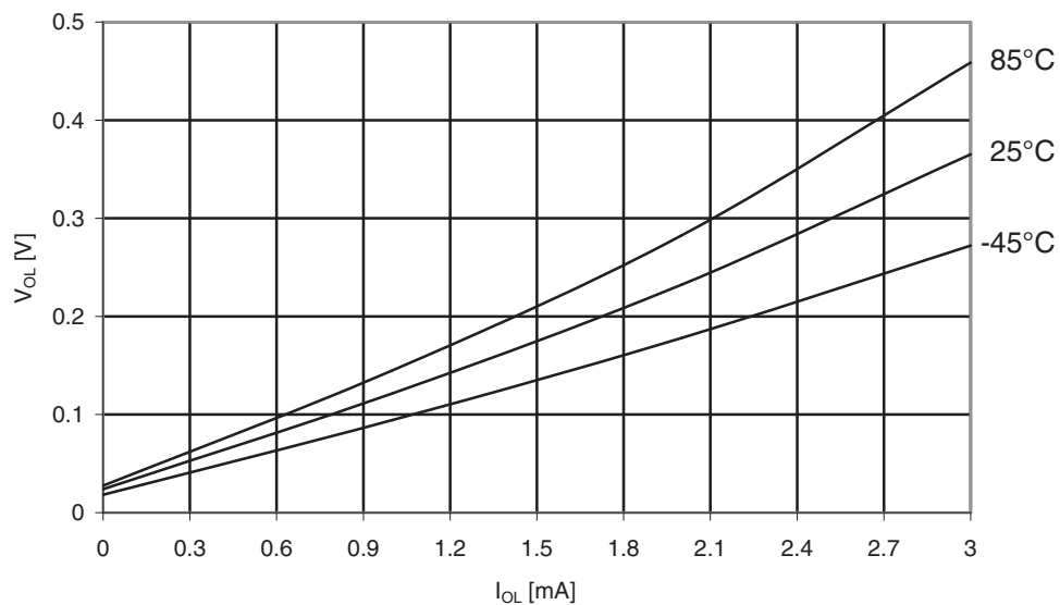
Figure 31-30. ATmega169A: I/O pin output voltage vs. sink current, ports A, C, D, E, F, G ( V_{CC} = 1.8V ).
