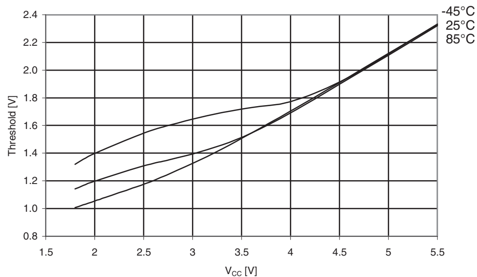
Figure 31-463. ATmega649P: Reset input Threshold voltage vs. V_{CC} ( V_{IH} , reset pin read as "1").
