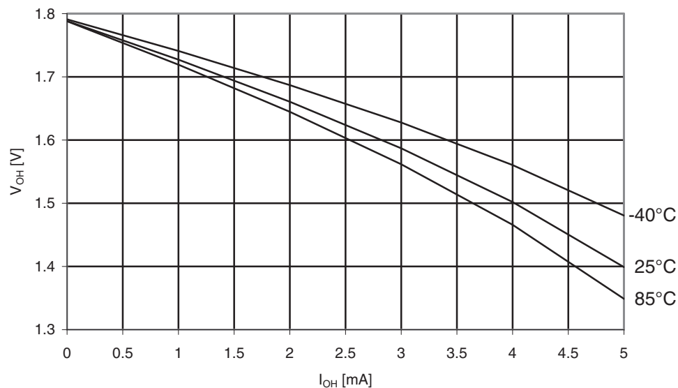
Figure 31-331. ATmega3290PA: I/O pin output voltage vs. source current, port B ( V_{CC} = 1.8V ).
