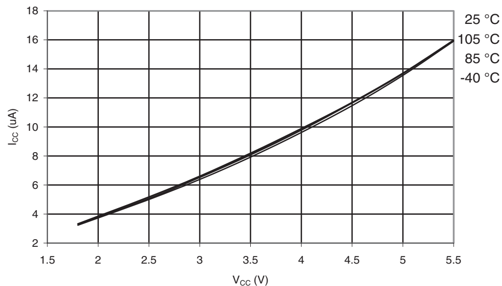
Figure 32-168. ATmega329P-105°C: Watchdog Timer Current vs. V_{CC}
