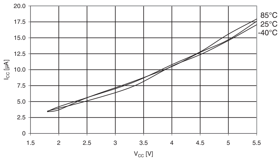
Figure 31-239. Atmel ATmega329PA: Watchdog Timer current vs. V_{CC} .
