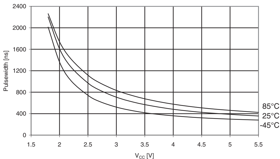
Figure 31-124. ATmega169PA: Minimum reset pulse width vs. V_{CC} .
