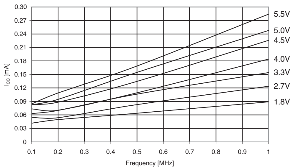
Figure 31-553. ATmega6490P: Idle supply current vs. low frequency (0.1 - 1.0MHz).
