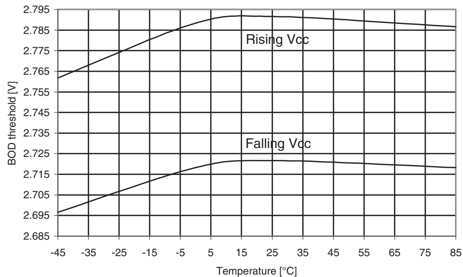
Figure 31-589. ATmega6490P: BOD Thresholds vs. temperature (BOD level is 2.7V).
