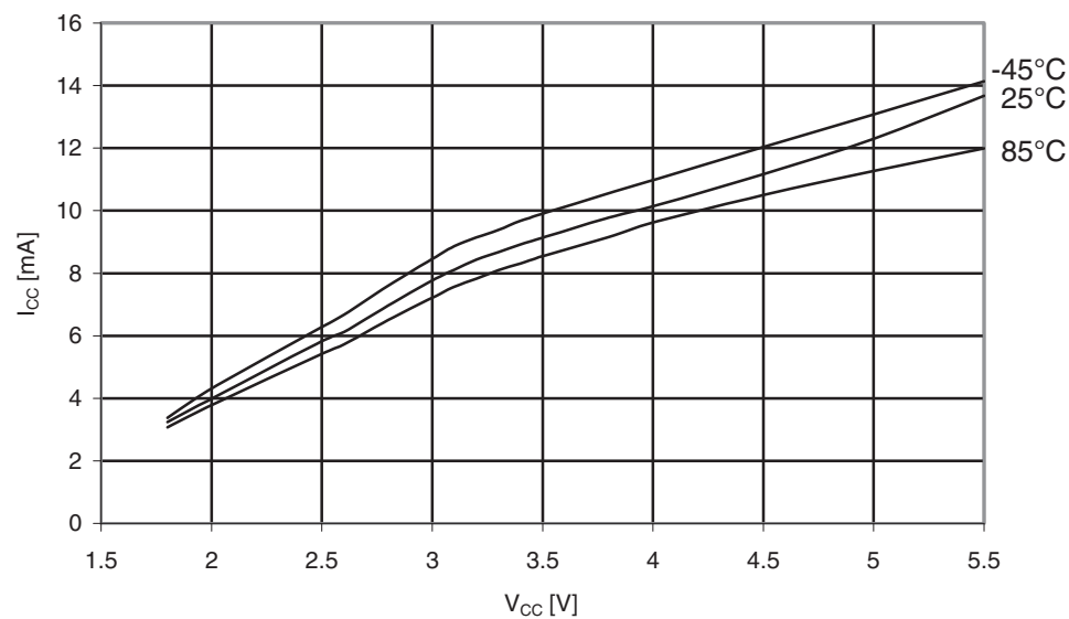
Figure 31-59. Atmel ATmega169A: Programming current vs. V_{CC} .
