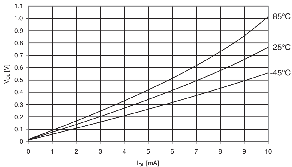
Figure 31-29. Atmel ATmega169A. I/O pin output voltage vs. sink current, ports A, C, D, E, F, G ( V_{CC} = 2.7V ).
