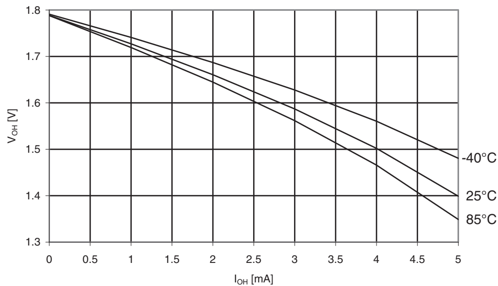
Figure 31-271. Atmel ATmega3290A: I/O pin output voltage vs. source current, port B ( V_{CC} = 1.8V ).
