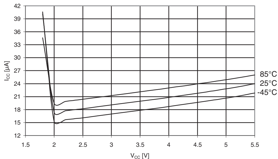
Figure 31-598. Atmel ATmega6490P: Brownout Detector current vs. V_{CC} .
