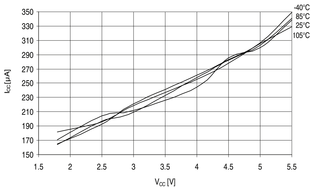
Figure 32-290. ATmega3290A - 105°C: Active Supply Current with ADC at 1MHz vs. V_{CC}
