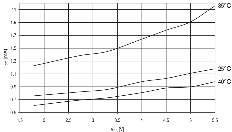
Figure 31-197. Atmel ATmega329PA: Power-save supply current vs. V_{CC} (Watchdog Timer disabled and 32kHz XTAL oscillator running).
