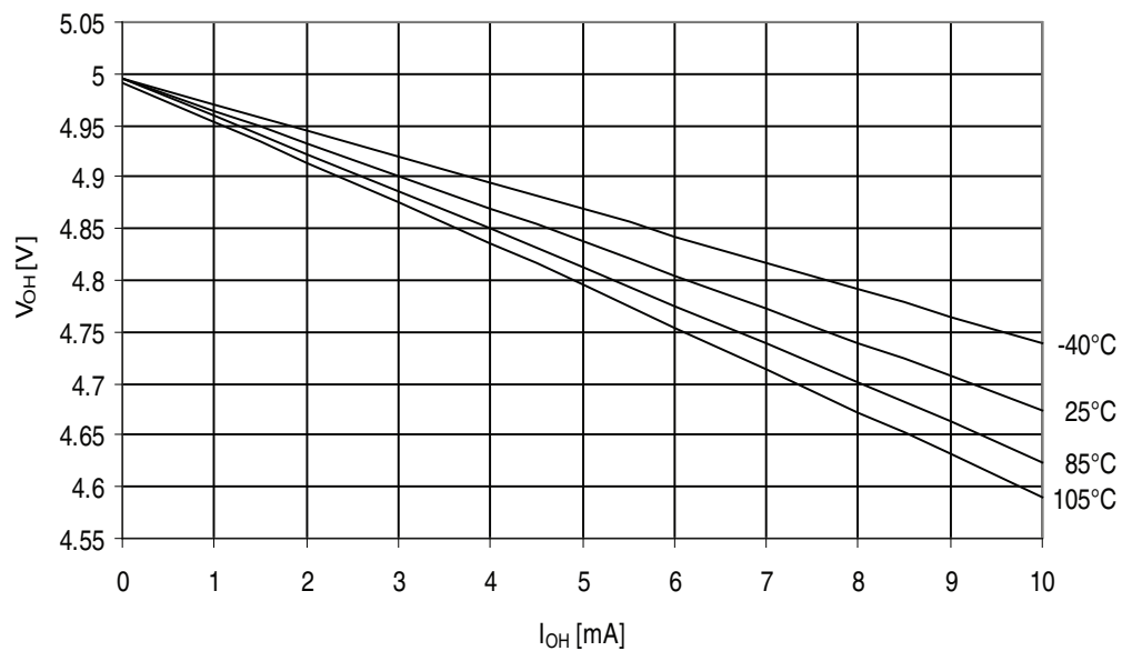
Figure 32-257. ATmega3290A - 105°C: I/O Pin Output Voltage vs. Source Current, Ports A, C, D, E, F, G ( V_{CC} = 5V )
