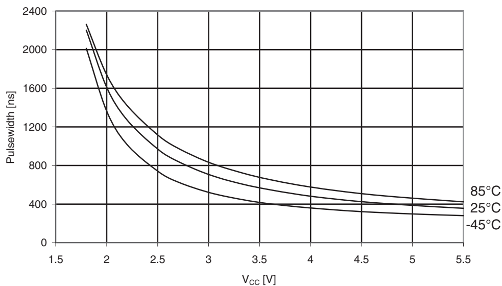
Figure 31-62. ATmega169A: Minimum reset pulse width vs. V_{CC} .
