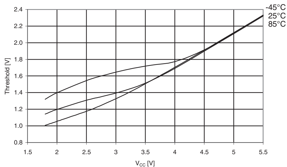
Figure 31-524. ATmega6490A: Reset input Threshold voltage vs. V_{CC} ( V_{IH} , reset pin read as “1”).
