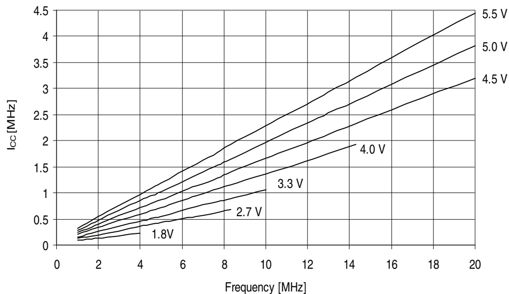
Figure 32-180. ATmega329PA - 105°C: Idle Supply Current vs. Frequency (1 - 20MHz)
