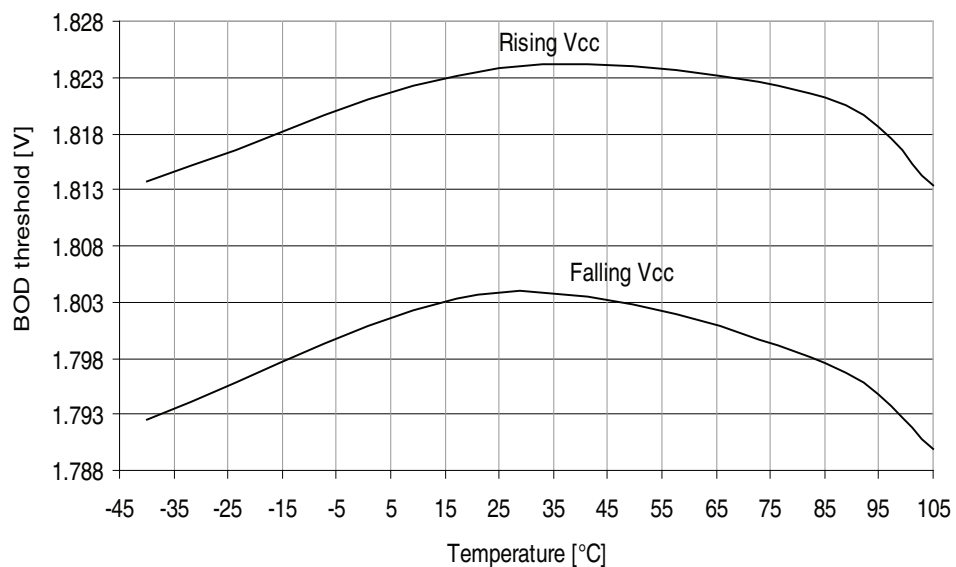
Figure 32-99. ATmega329A - 105°C: BOD Thresholds vs. Temperature (BOD Level is 1.8V)
