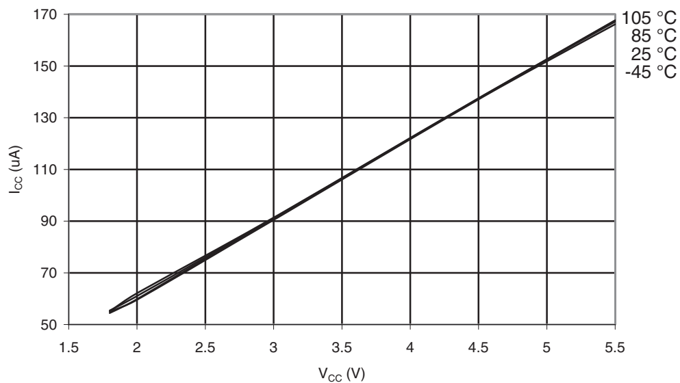
Figure 32-52. ATmega169PA-105°C: AREF External Reference Current vs. V_{CC}
