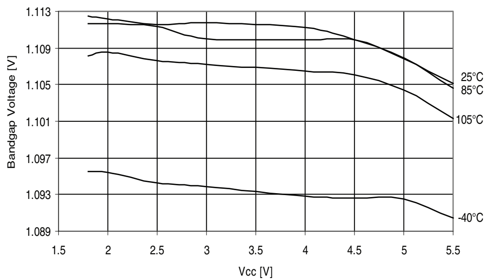
Figure 32-278. ATmega3290A - 105°C: Bandgap Voltage vs. V_{CC}
