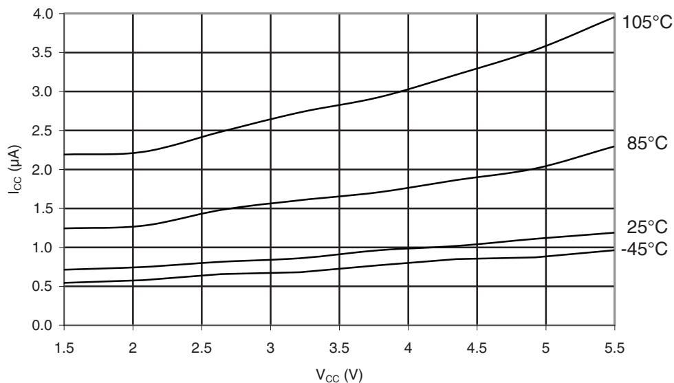
Figure 32-71. ATmega329A - 105°C: Power-save Supply Current vs. V_{CC} (Watchdog Timer Disabled)
