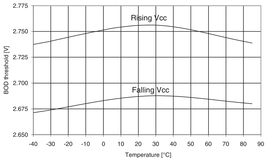
Figure 31-285. Atmel ATmega3290A: BOD Thresholds vs. temperature (BOD level is 2.7V).
