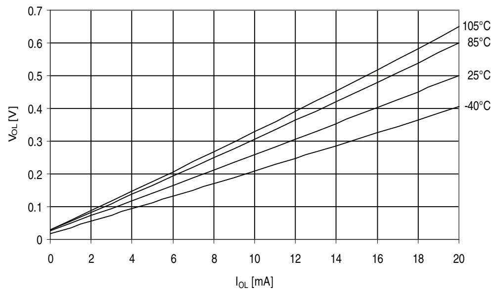
Figure 32-266. ATmega3290A - 105°C: I/O Pin Output Voltage vs. Sink Current, Port B ( V_{CC} = 5V )
