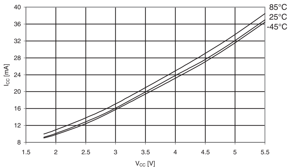
Figure 31-369. Atmel ATmega649A: Active supply current vs. V_{CC} (32kHz watch XTAL).
