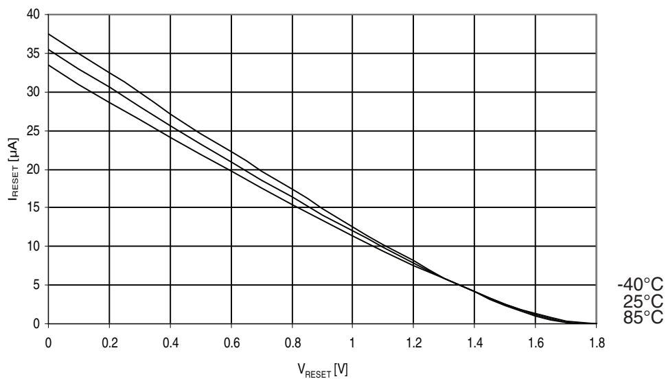
Figure 31-265. Atmel ATmega3290A: Reset pull-up resistor current vs. reset pin voltage ( V_{CC}=1.8V ).
