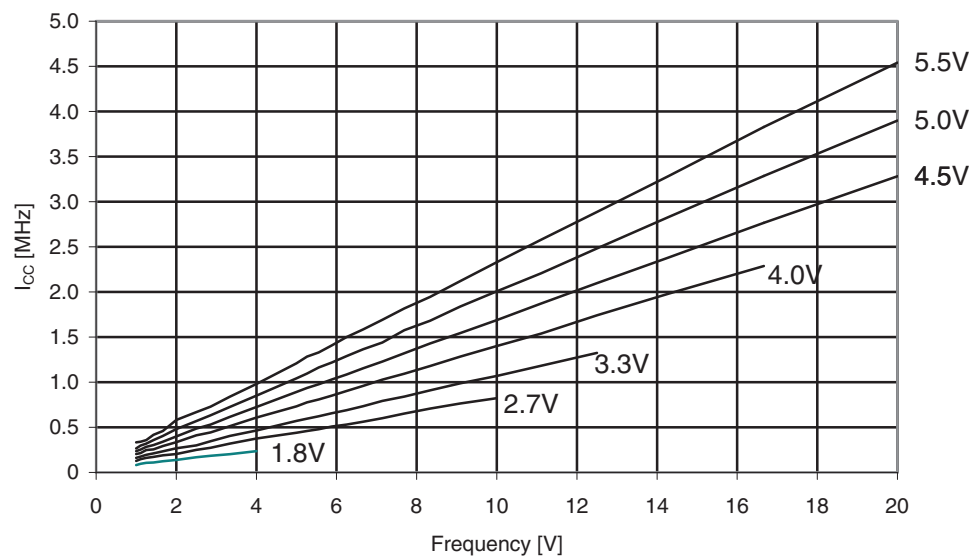
Figure 31-251. Atmel ATmega3290A: Idle supply current vs. frequency (1 - 20MHz).
