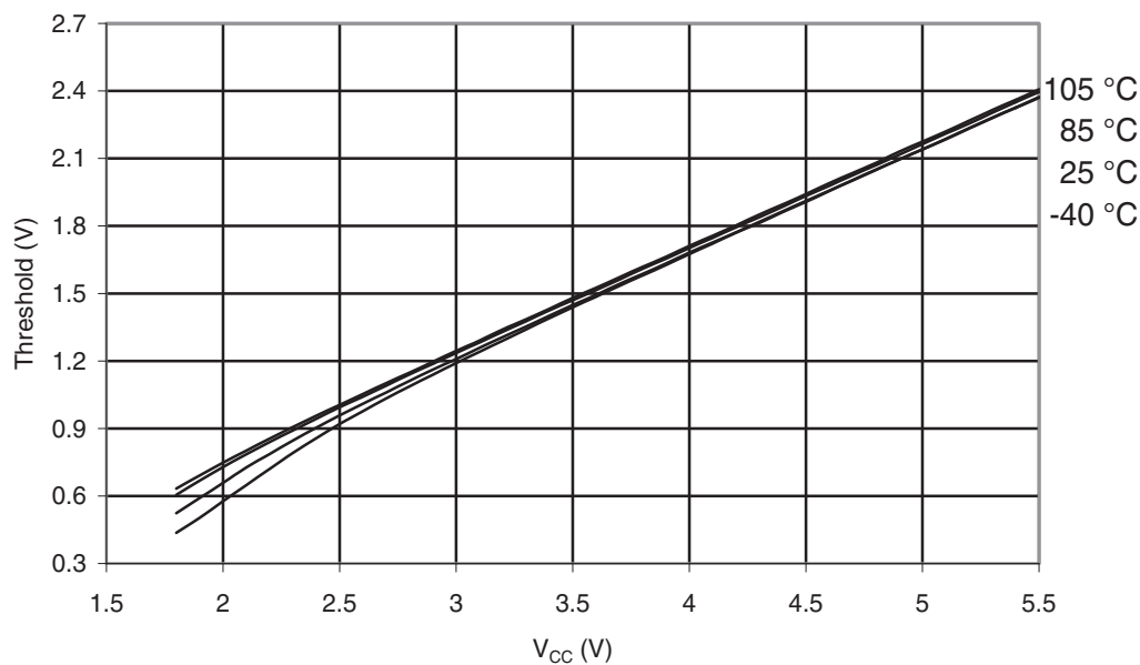
Figure 32-329. ATmega3290PA-105°C: I/O Pin Input Threshold Voltage vs. V_{CC} ( V_{IL} , I/O Pin Read as “0”)
