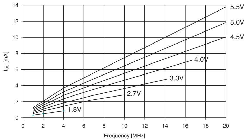
Figure 31-126. ATmega329A: Active supply current vs. frequency (1 - 20MHz).
