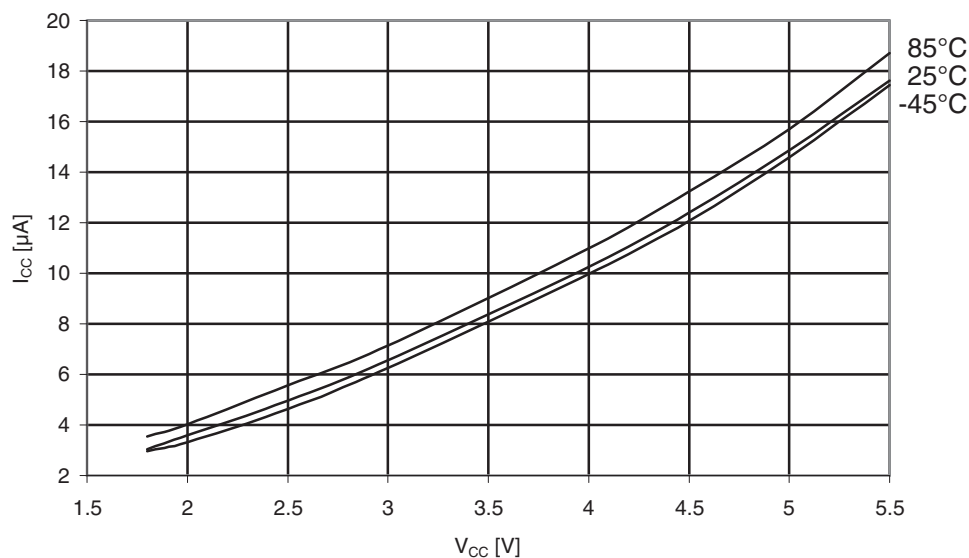
Figure 31-376. ATmega649A: Power-down supply current vs. V_{CC} (Watchdog Timer enabled).
