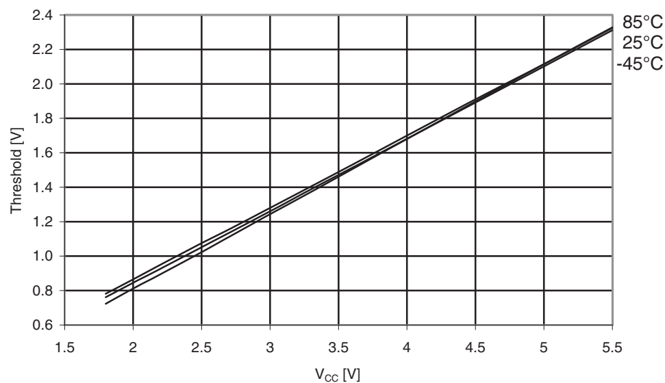
Figure 31-100. ATmega169PA: Reset Input Threshold voltage vs. V_{CC} ( V_{IL} , reset pin read as “0”).
