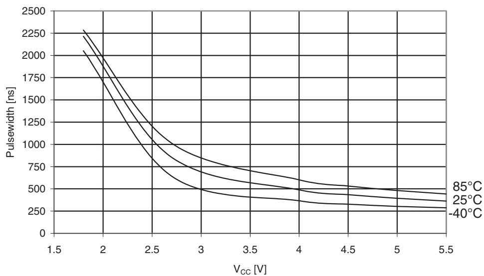
Figure 31-364. Atmel ATmega3290PA: Minimum reset pulse width vs. V_{CC} .
