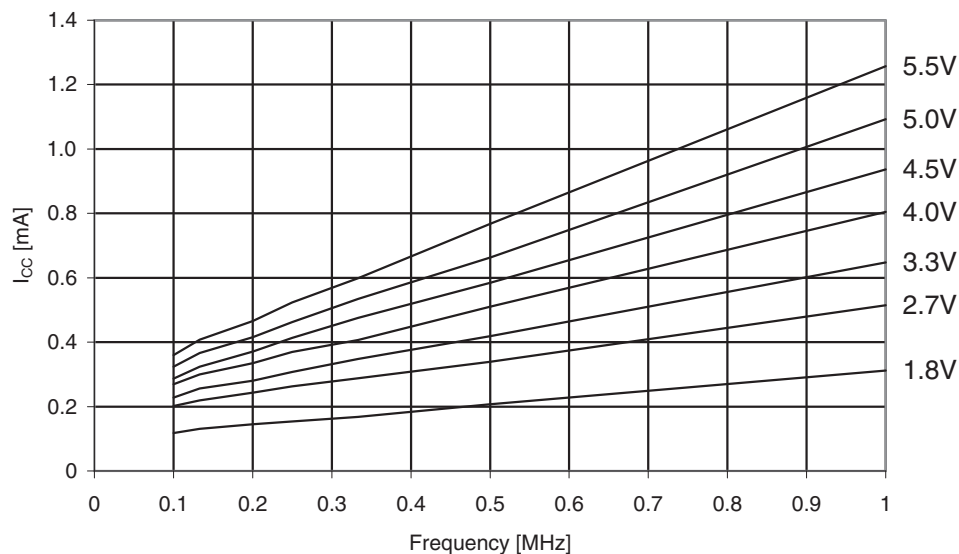
Figure 31-125. ATmega329A: Active supply current vs. low frequency (0.1 - 1.0MHz).
