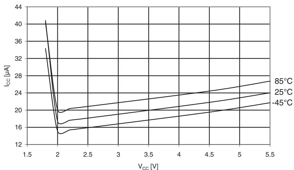
Figure 31-114. ATmega169PA: Brownout Detector current vs. V_{CC} .
