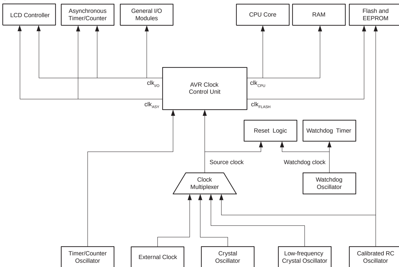
Figure 9-1. Clock distribution.
