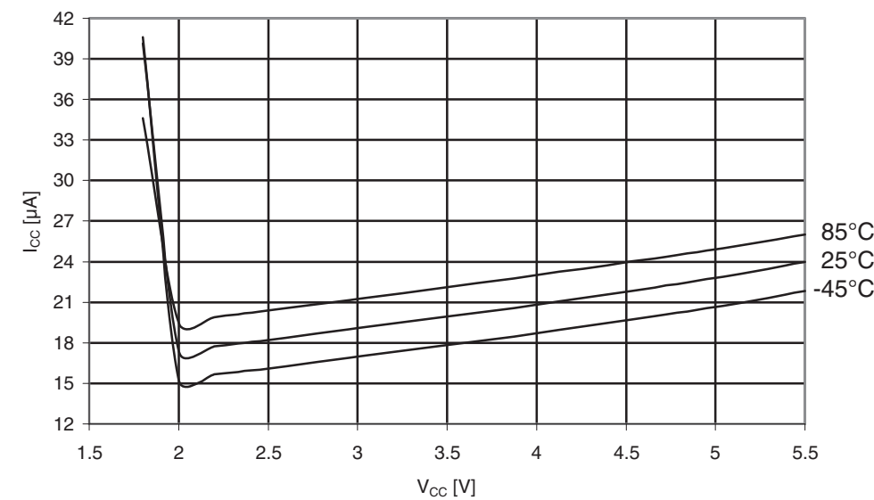
Figure 31-476. Atmel ATmega649P: Brownout Detector current vs. V_{CC} .
