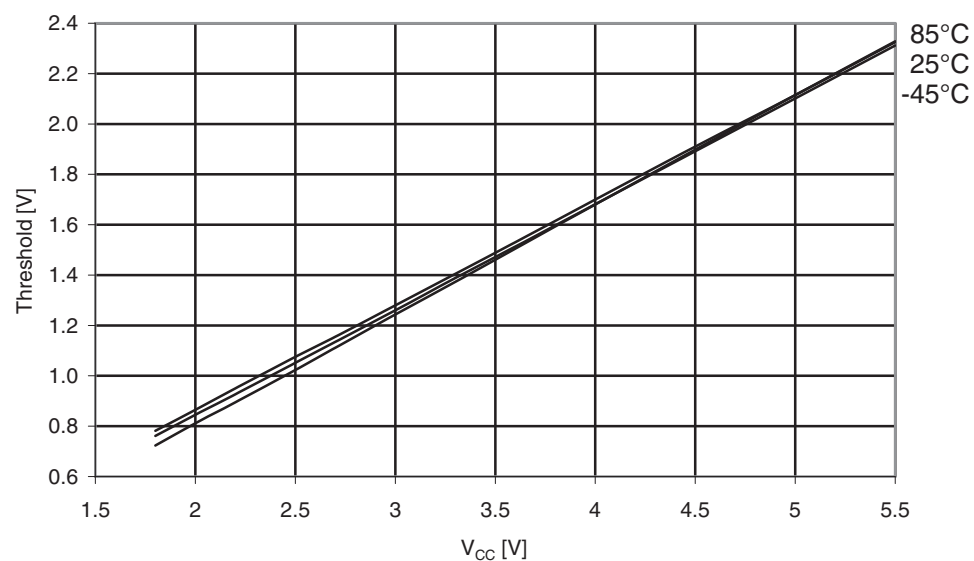
Figure 31-38. ATmega169A: Reset input Threshold voltage vs. V_{CC} ( V_{IL} , reset pin read as “0”).
