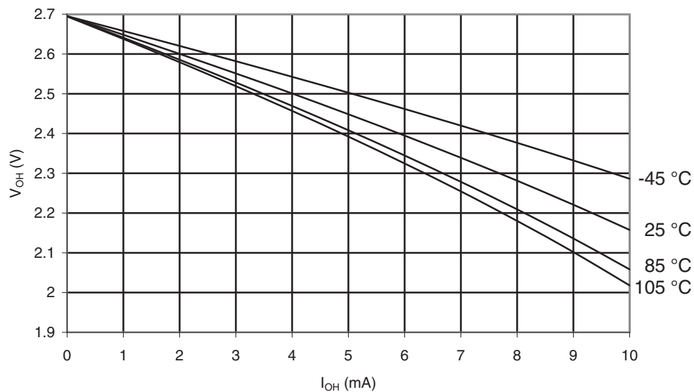
Figure 32-22. ATmega169PA-105°C: I/O Pin Output Voltage vs. Source Current, Ports A, C, D, E, F, G ( V_{CC} = 2.7V )
