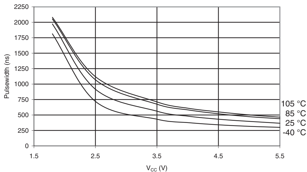
Figure 32-173. ATmega329P-105°C: Minimum Reset Pulse Width vs. V_{CC}
