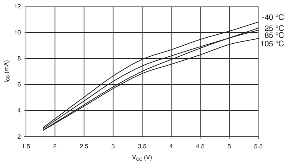
Figure 32-348. ATmega3290PA-105°C: Programming Current vs. V_{CC}
