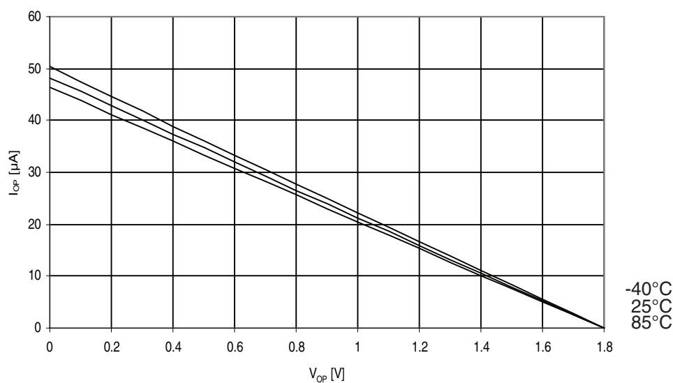
Figure 31-262. ATmega3290A: I/O pin pull-up resistor current vs. input voltage ( V_{CC} = 1.8V ).
