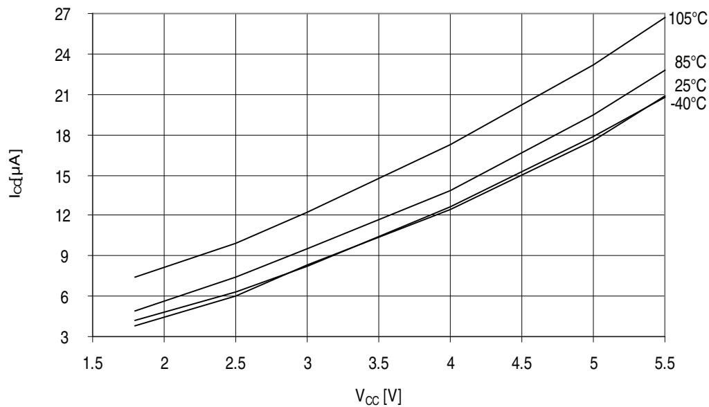
Figure 32-235. ATmega329PA - 105°C: Reset Current vs. V_{CC} (1 - 20MHz, Excluding Current Through The Reset Pull-up and No Clock)
