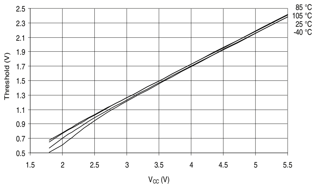
Figure 32-386. ATmega3290PA - 105°C: I/O Pin Input Threshold Voltage vs. V_{CC} ( V_{IL} , I/O Pin Read as “0”)
