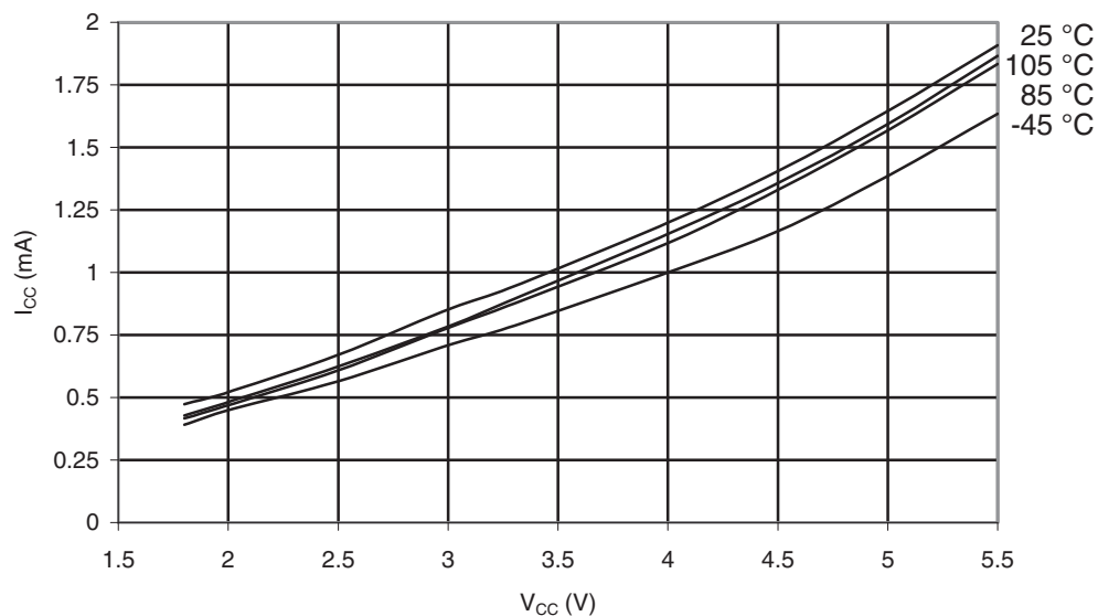
Figure 32-8. ATmega169PA-105°C: Idle Supply Current vs. V_{CC} (Internal RC Oscillator, 8MHz)
