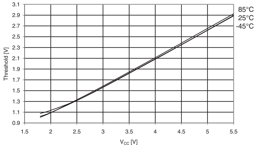
Figure 31-521. Atmel ATmega6490A: I/O pin input Threshold voltage vs. V_{CC} ( V_{IH} , I/O pin read as “1”).
