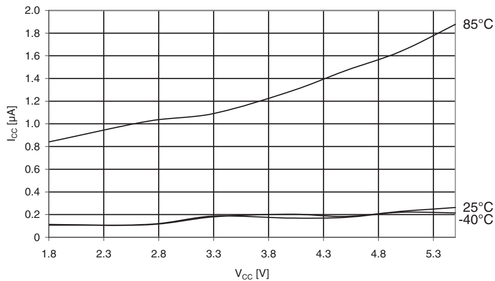
Figure 31-315. Atmel ATmega3290PA Power-down Supply current vs. V_{CC} (Watchdog Timer disabled).
