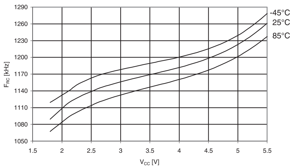
Figure 31-532. ATmega6490A: Watchdog Oscillator frequency vs. V_{CC} .
