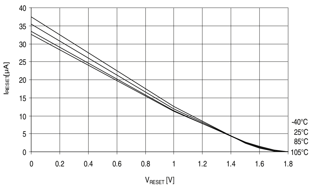
Figure 32-78. ATmega329A - 105°C: Reset Pull-up Resistor Current vs. Reset Pin Voltage ( V_{CC} = 1.8V )
