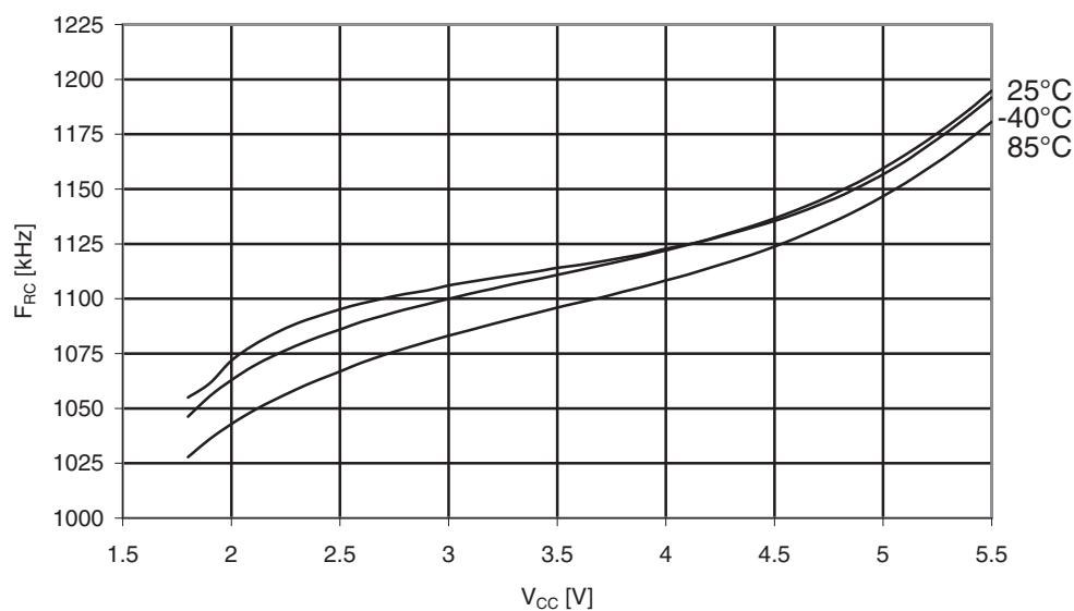
Figure 31-229. Atmel ATmega329PA: Watchdog Oscillator frequency vs. V_{CC} .
