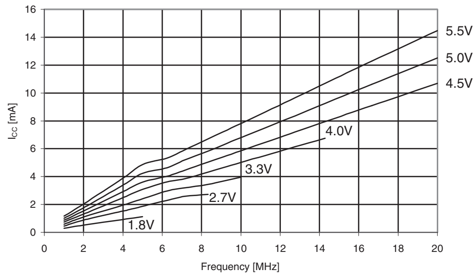
Figure 31-366. ATmega649A: Active supply current vs. frequency (1 - 20MHz).
