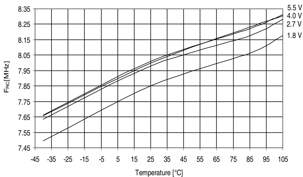
Figure 32-284. AATmega3290A - 105°C: Calibrated 8MHz RC Oscillator Frequency vs. Temperature
