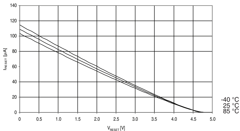
Figure 31-263. Atmel ATmega3290A: Reset pull-up resistor current vs. reset pin voltage ( V_{CC} = 5V ).
