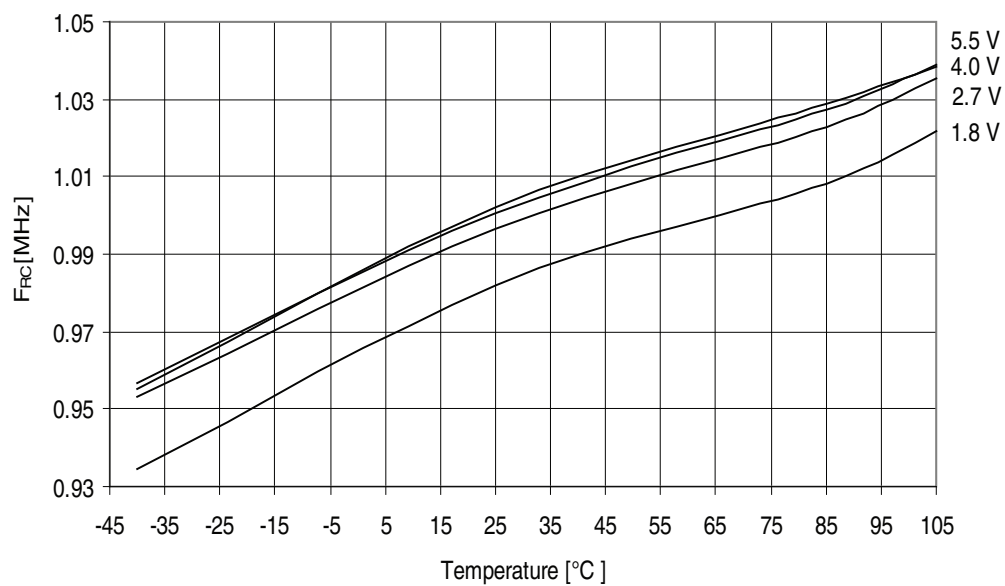
Figure 32-219. AATmega329PA - 105°C: Calibrated 1MHz RC Oscillator Frequency vs. Temperature
