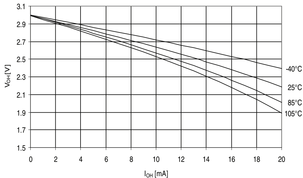
Figure 32-83. ATmega329A - 105°C: I/O Pin Output Voltage vs. Source Current, Port B ( V_{CC} = 3V )
