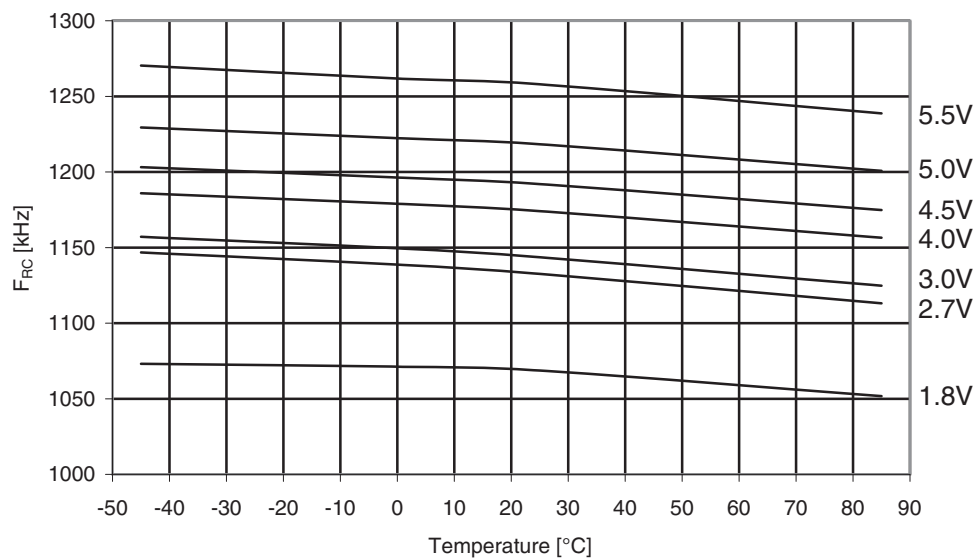
Figure 31-48. ATmega169A: Watchdog oscillator frequency vs. temperature.
