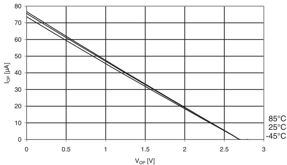
Figure 31-79. Atmel ATmega169PA: I/O pin pull-up resistor current vs. input voltage ( V_{CC} = 2.7V ).
