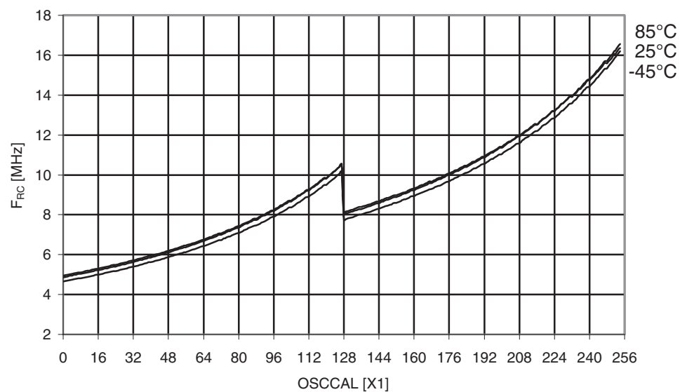
Figure 31-414. ATmega649A: Calibrated 8MHz RC oscillator frequency vs. Oscal value.
