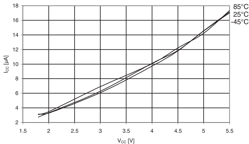
Figure 31-603. ATmega6490P: Watchdog Timer current vs. V_{CC} .
