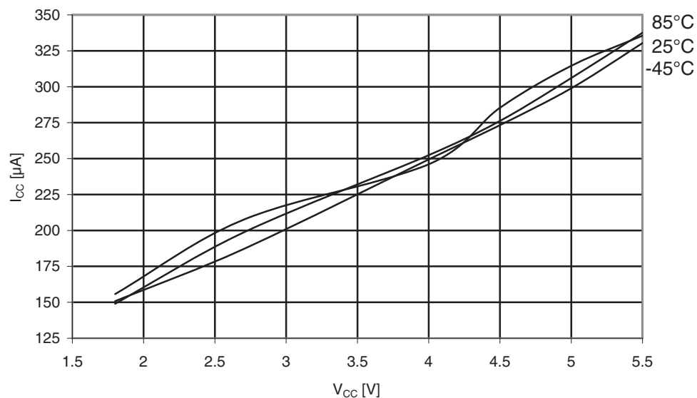
Figure 31-55. Atmel ATmega169A: Active supply current with ADC at 1MHz vs. V_{CC} .
