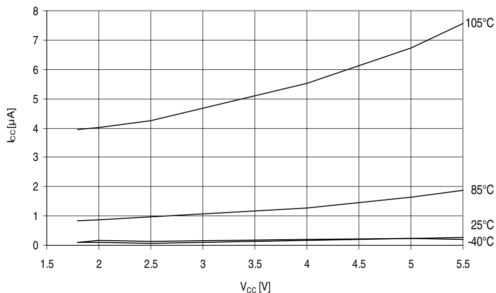
Figure 32-184. ATmega329PA - 105°C: Power-down Supply Current vs. V_{CC} (Watchdog Timer Disabled)
