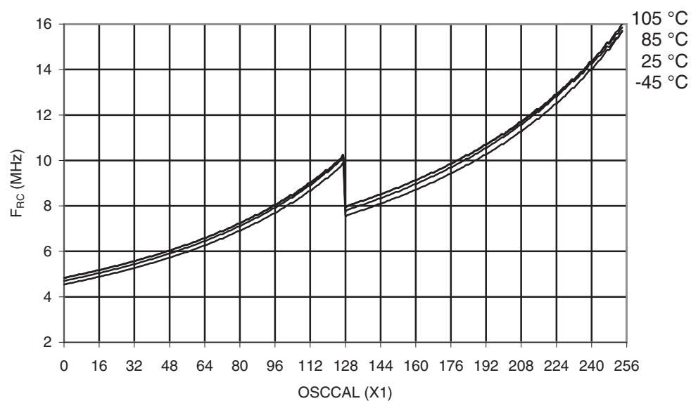
Figure 32-47. ATmega169PA-105°C: Calibrated 8MHz RC Oscillator Frequency vs. Oscal Value
