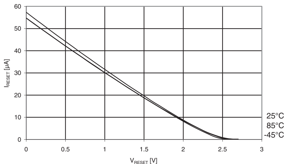
Figure 31-82. ATmega169PA: Reset pull-up resistor current vs. Reset pin voltage ( V_{CC} = 2.7V ).
