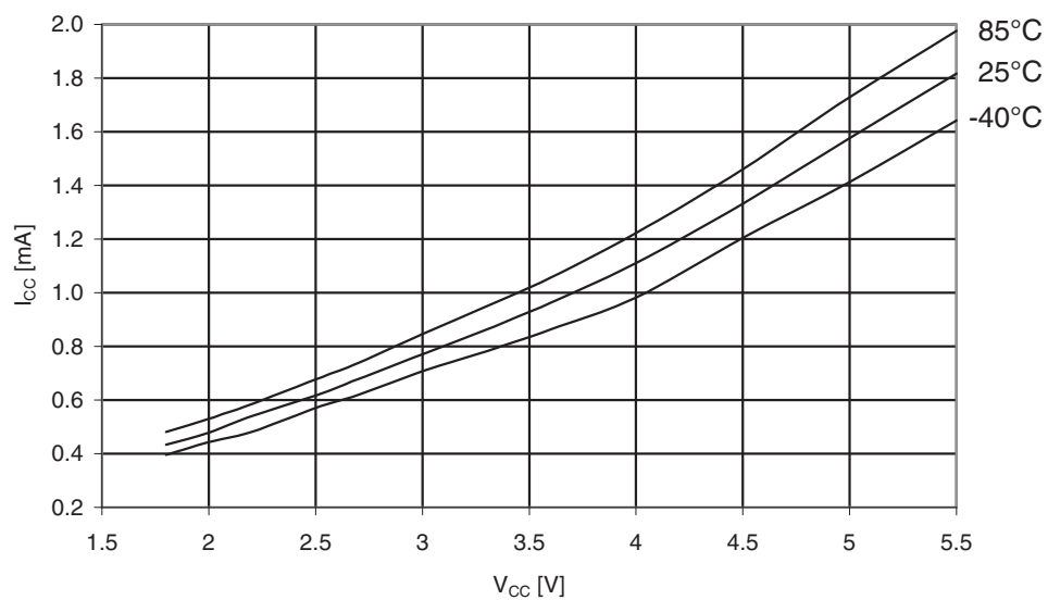
Figure 31-252. ATmega3290A: Idle supply current vs. V_{CC} (Internal RC oscillator, 8MHz).
