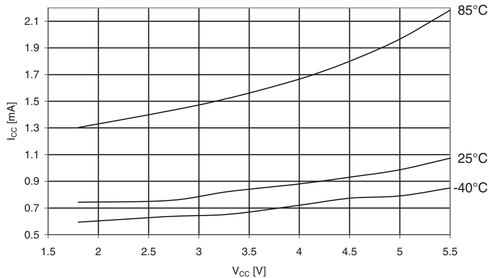
Figure 31-138. ATmega329A Standby supply current vs. V_{CC} (32kHz watch XTAL, Watchdog Timer disabled).
