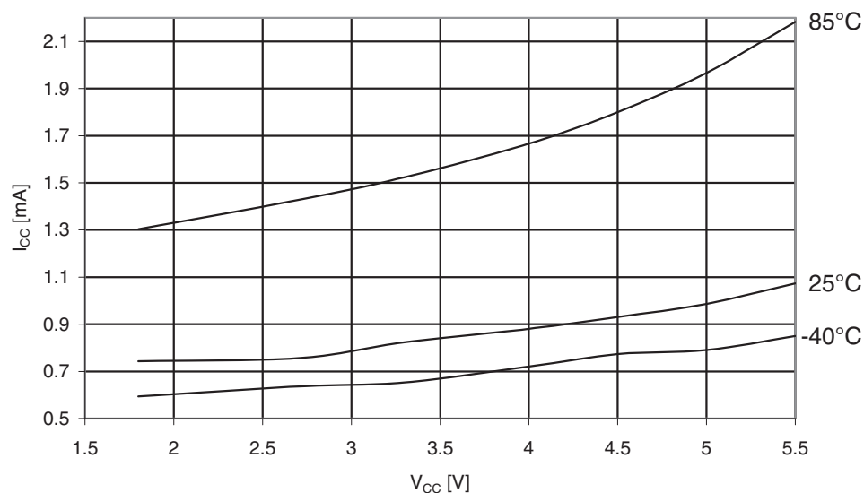
Figure 31-198. ATmega329PA standby supply current vs. V_{CC} (32kHz watch XTAL, Watchdog Timer disabled).
