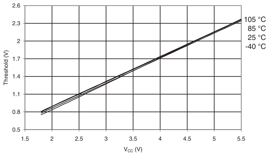
Figure 32-154. ATmega329P-105°C: Reset Input Threshold Voltage vs. V_{CC} ( V_{IL} , Reset Pin Read as “0”)
