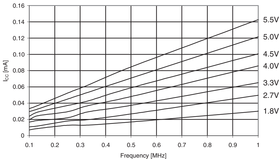
Figure 31-423. Atmel ATmega649A: Reset supply current vs. V_{CC} (0.1 - 1.0MHz, excluding current through the reset pull-up).
