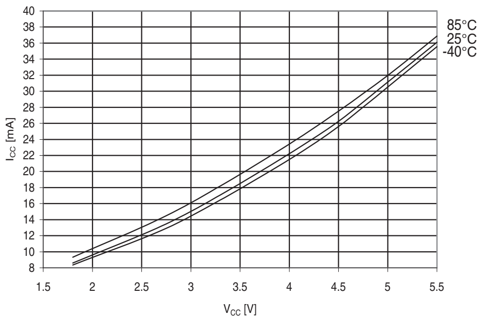
Figure 31-189. Atmel ATmega329PA: Active supply current vs. V_{CC} (32kHz watch XTAL).
