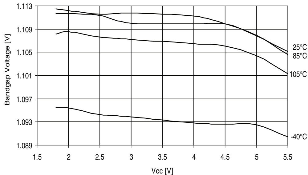
Figure 32-394. ATmega3290PA - 105°C: Bandgap Voltage vs. V_{CC}
