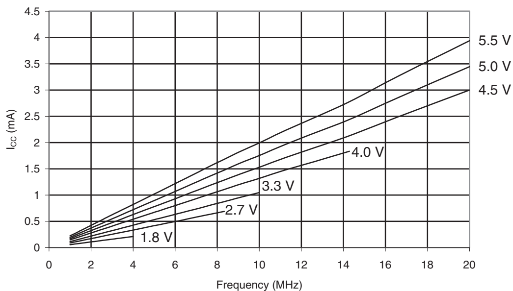
Figure 32-172. ATmega329P-105°C: Reset Supply Current vs. V_{CC} (1 - 20MHz, Excluding Current Through The Reset Pull-up)
