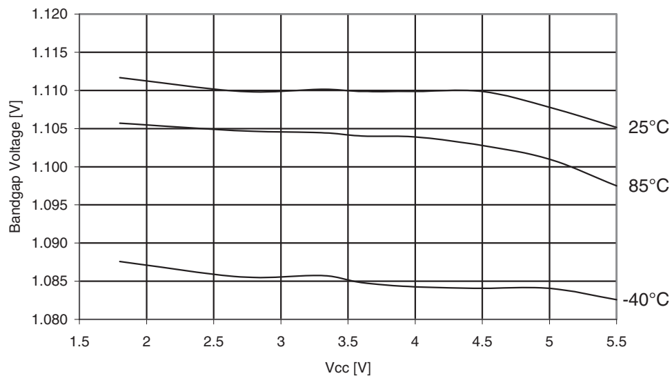
Figure 31-227. Atmel ATmega329PA: Bandgap voltage vs. V_{CC} .
