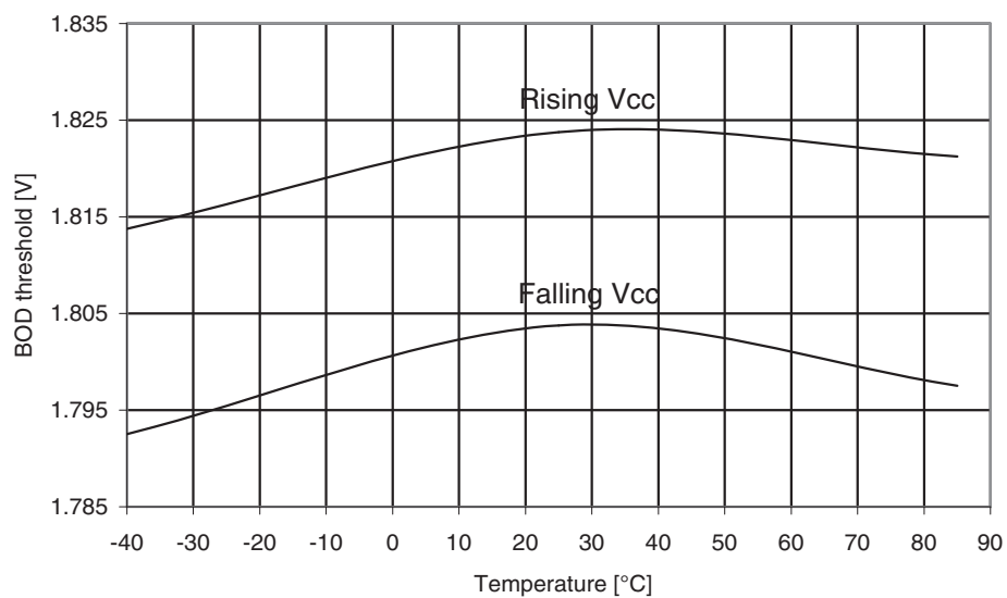
Figure 31-226. ATmega329PA: BOD Thresholds vs. temperature (BOD level is 1.8V).
