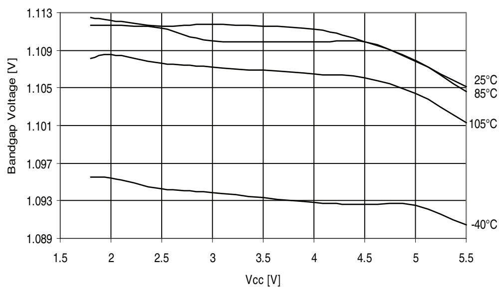
Figure 32-215. ATmega329PA - 105°C: Bandgap Voltage vs. V_{CC}
