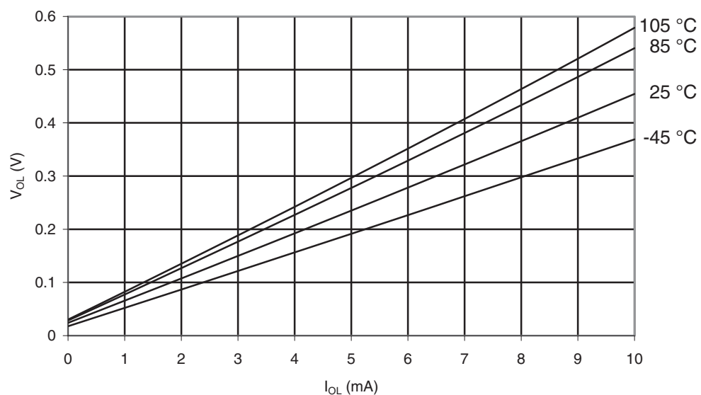
Figure 32-27. ATmega169PA-105°C: I/O Pin Output Voltage vs. Sink Current, Ports A, C, D, E, F, G ( V_{CC} = 5V )
