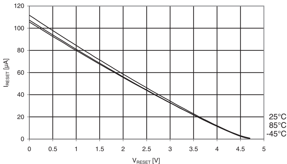
Figure 31-81. Atmel ATmega169PA: Reset pull-up resistor current vs. Reset pin voltage ( V_{CC} = 5V ).
