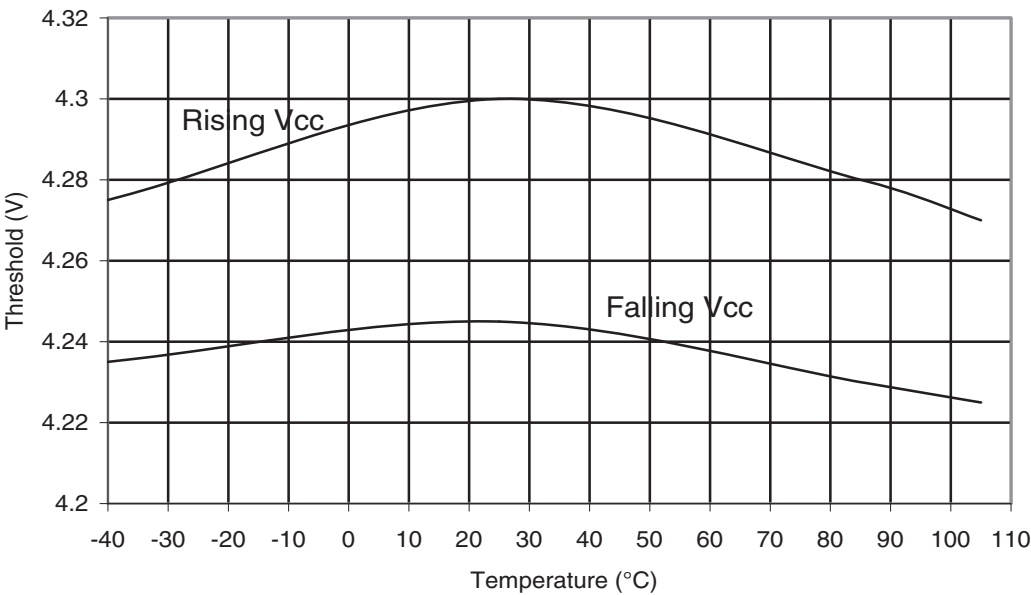
Figure 32-334. ATmega3290PA-105°C: BOD Thresholds vs. Temperature (BOD Level is 4.3V)
