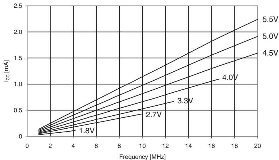
Figure 31-363. ATmega3290PA: Reset supply current vs. V_{CC} (1 - 20MHz, excluding current through the reset pull-up).
