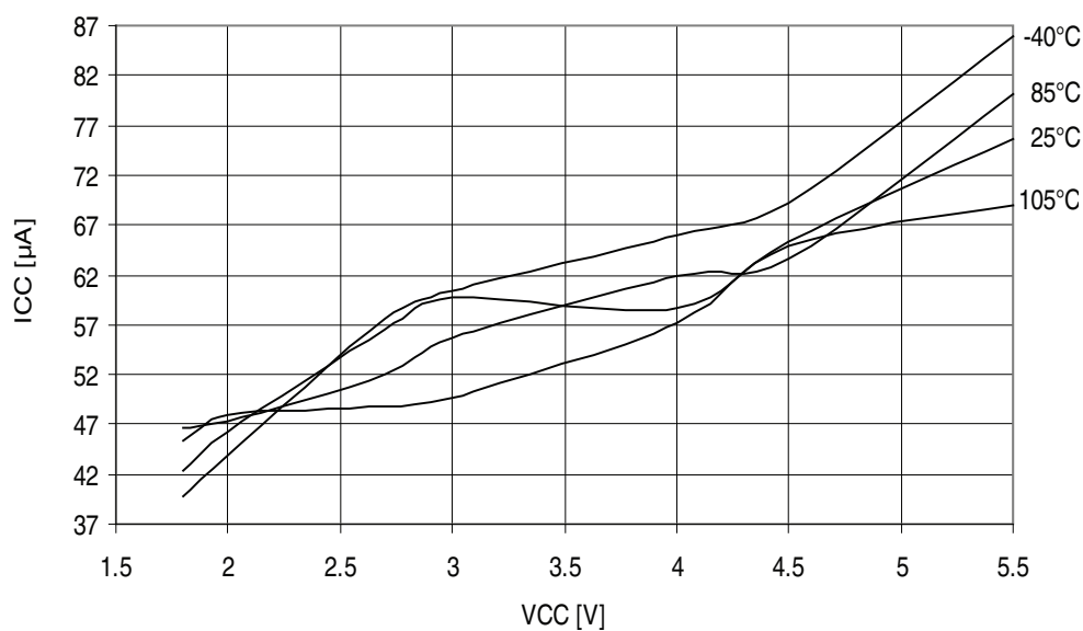
Figure 32-294. ATmega3290A - 105°C: Analog Comparator Current vs. V_{CC}
