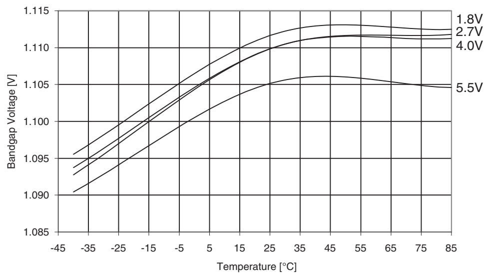
Figure 31-168. ATmega329A: Bandgap voltage vs. temperature.
