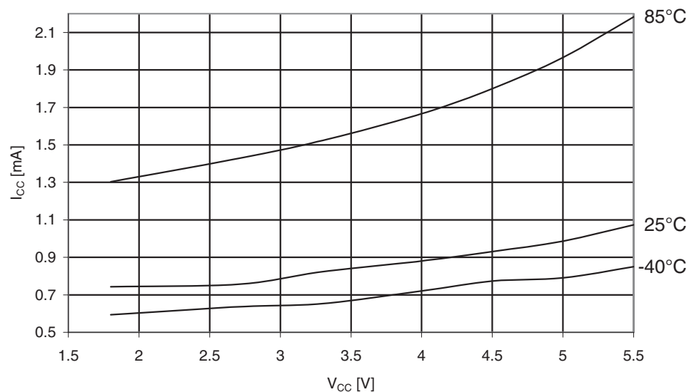
Figure 31-258. ATmega3290A: Standby supply current vs. V_{CC} (32kHz watch XTAL, Watchdog Timer disabled).
