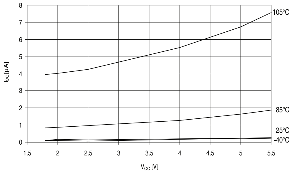
Figure 32-69. ATmega329A - 105°C: Power-down Supply Current vs. V CC (Watchdog Timer Disabled)
