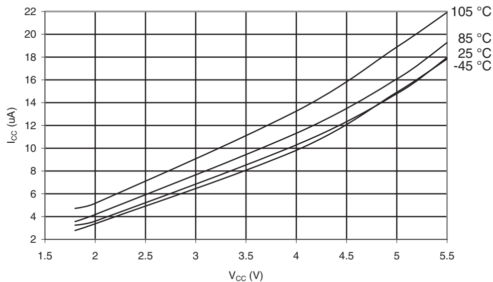
Figure 32-12. ATmega169PA-105°C: Power-down Supply Current vs. V_{CC} (Watchdog Timer Enabled)
