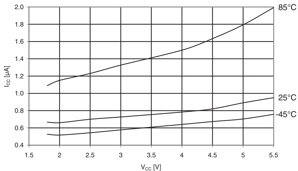
Figure 31-76. ATmega169PA: Standby supply current vs. V_{CC} (32kHz watch XTAL, Watchdog Timer disabled).
