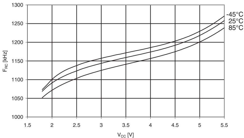
Figure 31-47. Atmel ATmega169A: Watchdog oscillator frequency vs. V_{CC} .
