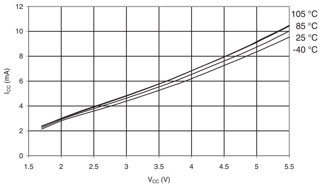
Figure 32-302. ATmega3290PA-105°C: Active Supply Current vs. V_{CC} (Internal RC Oscillator, 8MHz)
