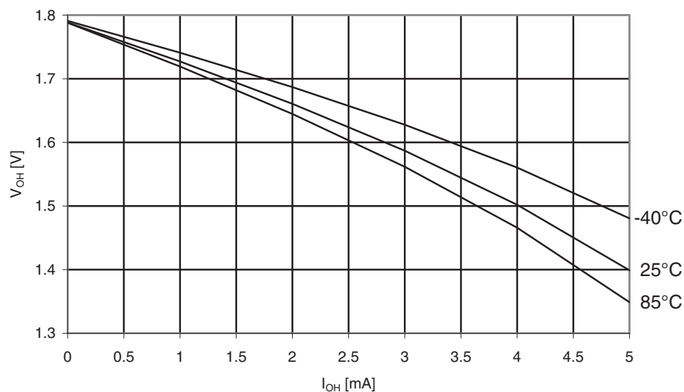
Figure 31-211. Atmel ATmega329PA: I/O pin output voltage vs. source current, port B ( V_{CC} = 1.8V ).
