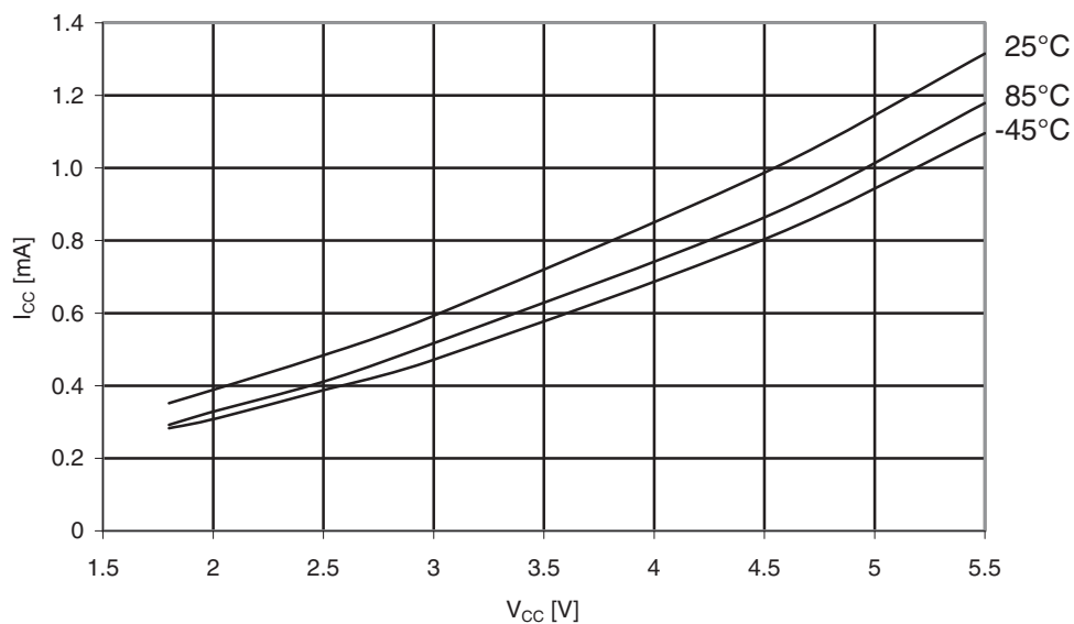
Figure 31-66. ATmega169PA: Active supply current vs. V_{CC} (Internal RC oscillator, 1MHz).
