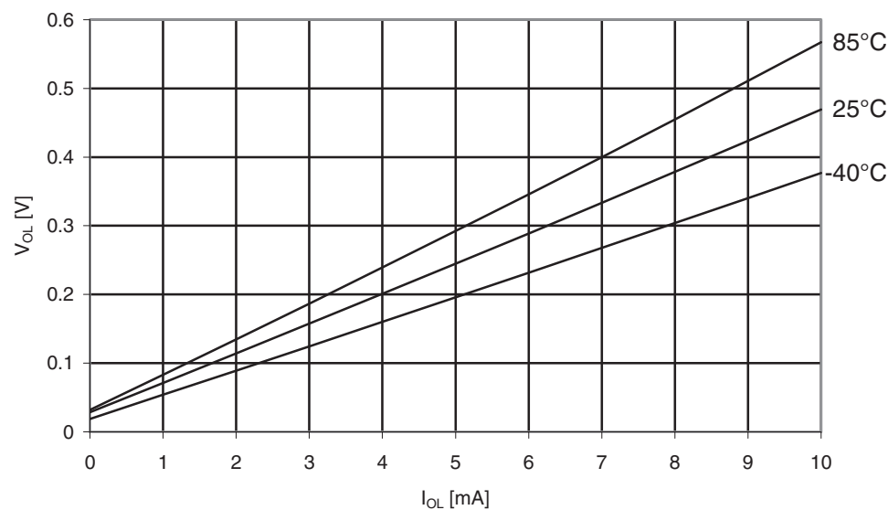
Figure 31-212. ATmega329PA: I/O pin output voltage vs. sink current, ports A, C, D, E, F, G ( V_{CC} = 5V ).
