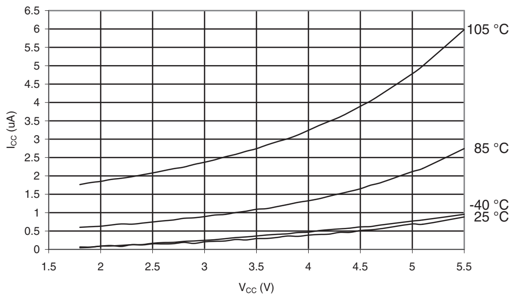
Figure 32-310. ATmega3290PA-105°C: Power-down Supply Current vs. V_{CC} (Watchdog Timer Disabled)
