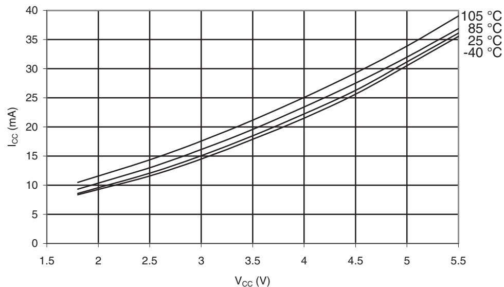
Figure 32-304. ATmega3290PA-105°C: Active Supply Current vs. V_{CC} (32kHz Watch Crystal)
