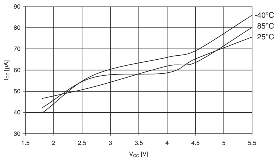
Figure 31-180. ATmega329A: Analog Comparator current vs. V_{CC} .
