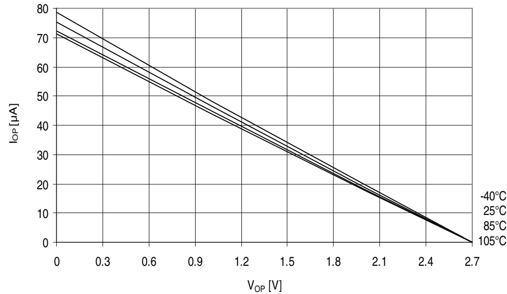
Figure 32-74. ATmega329A - 105°C: I/O Pin Pull-up Resistor Current vs. Input Voltage ( V_{CC} = 2.7V )
