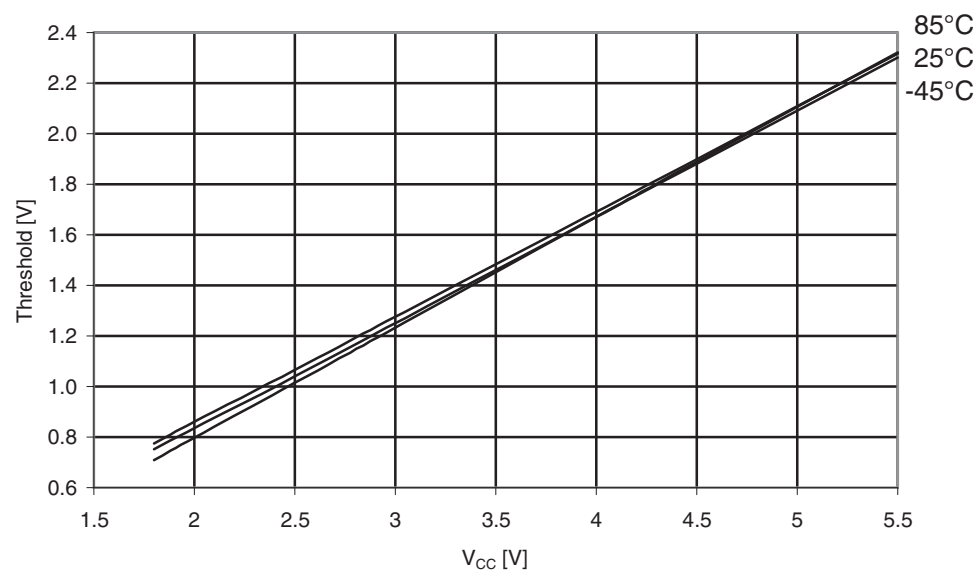
Figure 31-464. Atmel ATmega649P: Reset input Threshold voltage vs. V_{CC} ( V_{IL} , reset pin read as “0”).
