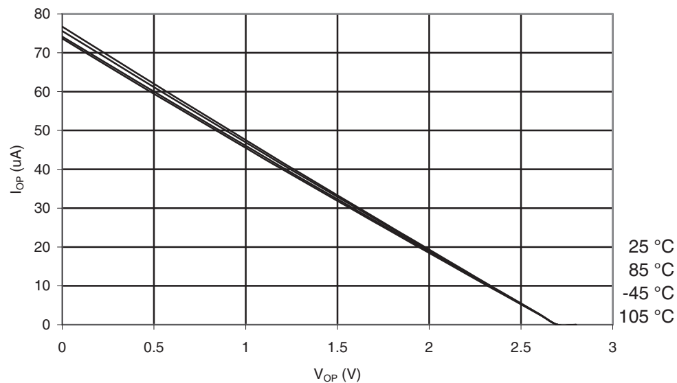
Figure 32-16. ATmega169PA-105°C: I/O Pin Pull-up Resistor Current vs. Input Voltage ( V_{CC} = 2.7V )
