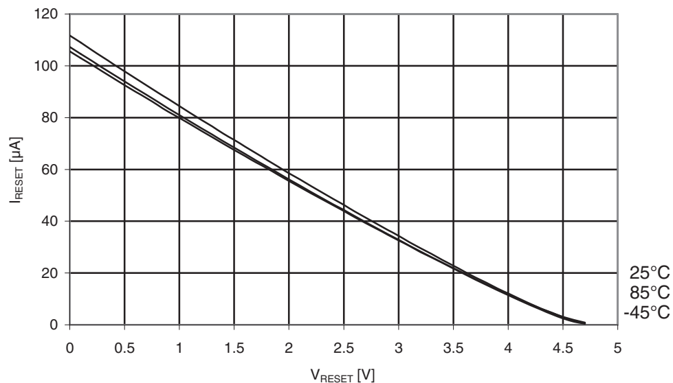
Figure 31-19. Atmel ATmega169A: Reset pull-up resistor current vs. reset pin voltage ( V_{CC} = 5V ).
