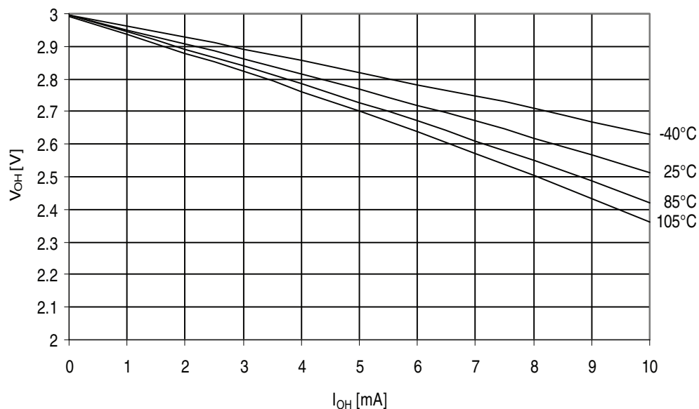
Figure 32-374. ATmega3290PA - 105°C: I/O Pin Output Voltage vs. Source Current, Ports A, C, D, E, F, G, H ( V_{CC} = 3V )
