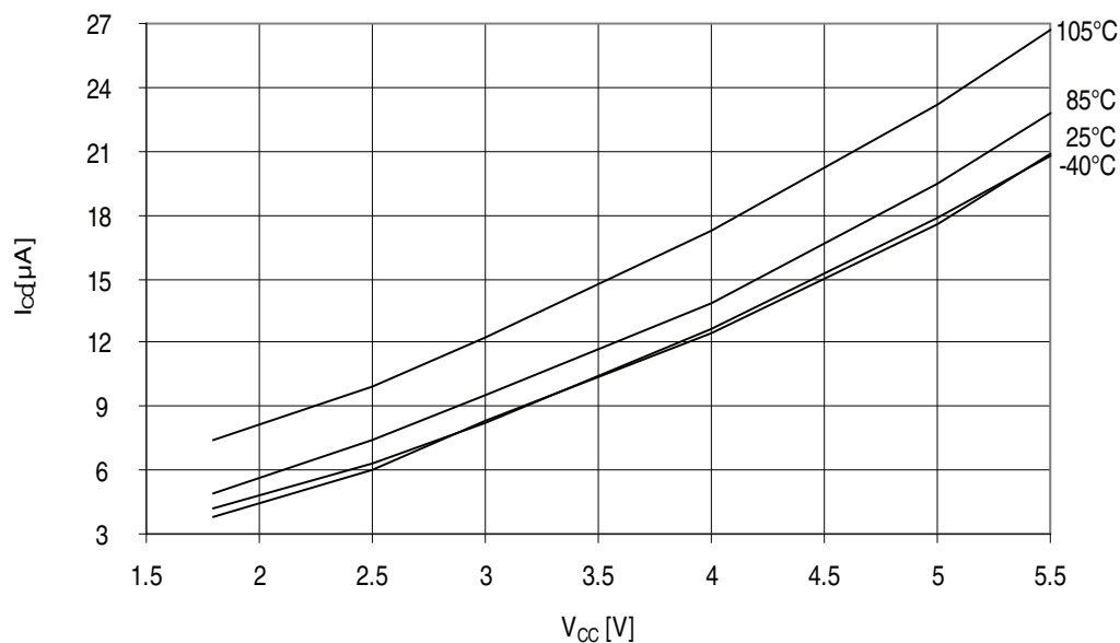
Figure 32-298. ATmega3290A - 105°C: Reset Current vs. V_{CC} (1 - 20MHz, Excluding Current Through The Reset Pull-up and No Clock)
