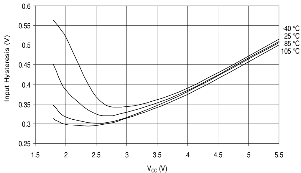
Figure 32-271. ATmega3290A - 105°C: I/O Pin Input Hysteresis vs. V_{CC}
