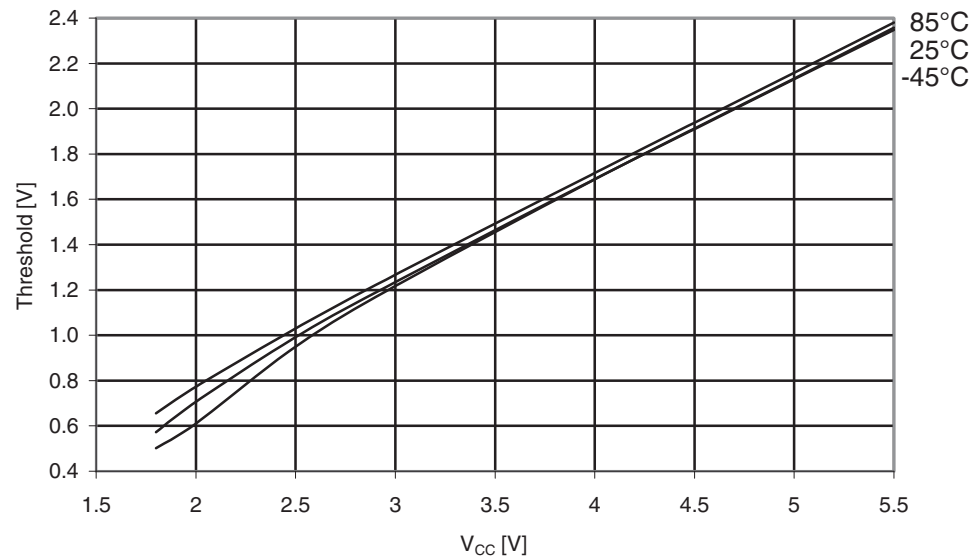
Figure 31-400. ATmega649A: I/O pin Input Threshold voltage vs. V_{CC} ( V_{IL} , I/O pin read as “0”).
