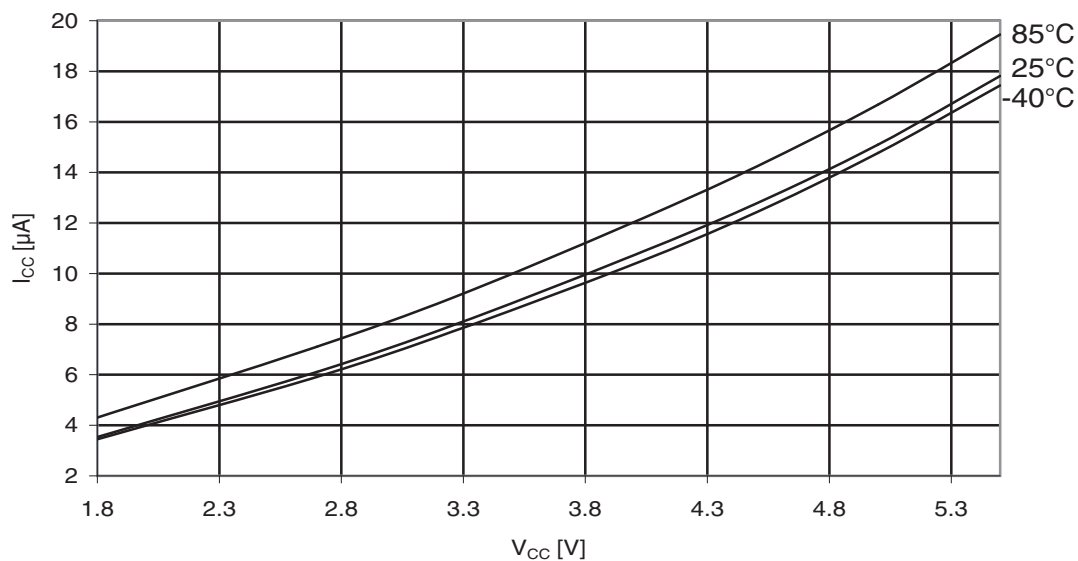
Figure 31-136. ATmega329A: Power-down supply current vs. V_{CC} (Watchdog Timer enabled).
