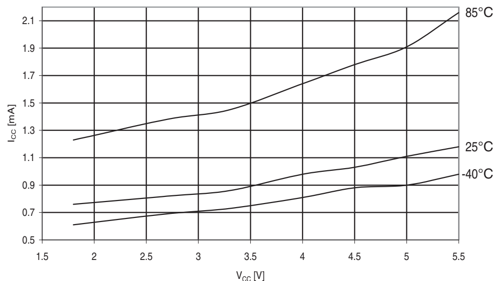
Figure 31-137. Atmel ATmega329A: Power-save supply current vs. V_{CC} (Watchdog Timer disabled and 32kHz XTAL oscillator running).
