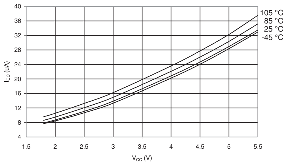
Figure 32-5. ATmega169PA-105°C: Active Supply Current vs. V_{CC} (32kHz Watch Crystal)
