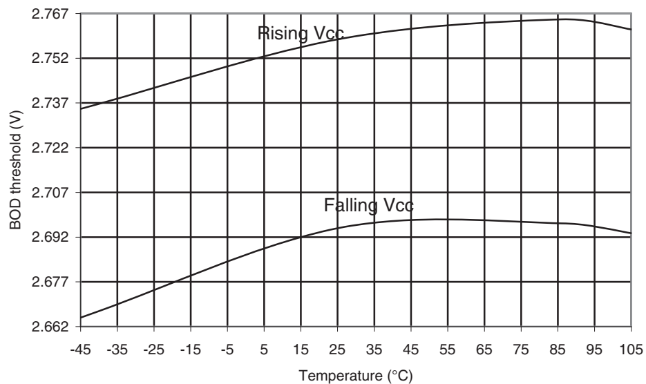
Figure 32-40. ATmega169PA-105°C: BOD Thresholds vs. Temperature (BOD Level is 2.7V)
