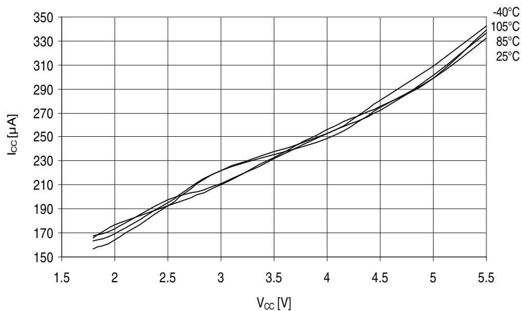
Figure 32-404. ATmega3290PA - 105°C: Active Supply Current with ADC at 50kHz vs. V_{CC}
