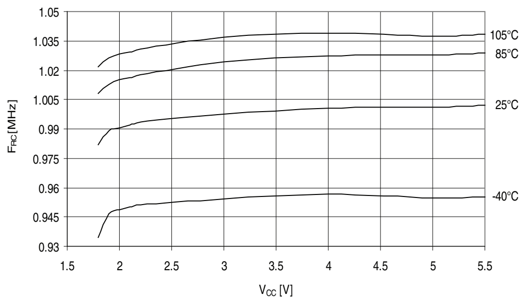
Figure 32-399. ATmega3290PA - 105°C: Calibrated 1MHz RC Oscillator Frequency vs. V_{CC}
