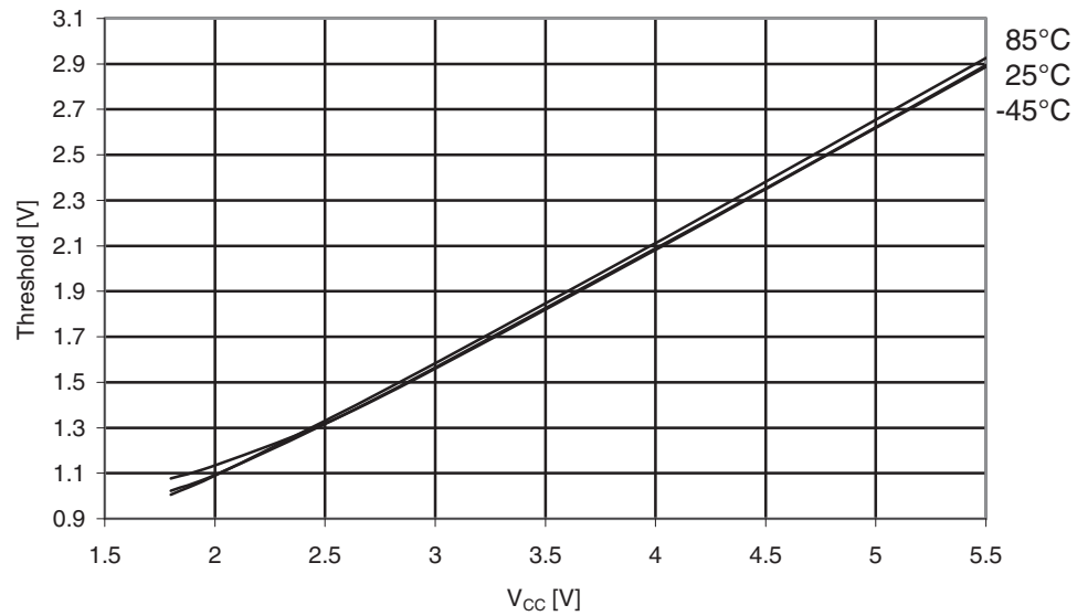
Figure 31-399. Atmel ATmega649A: I/O pin Input Threshold voltage vs. V_{CC} ( V_{IH} , I/O pin read as “1”).
