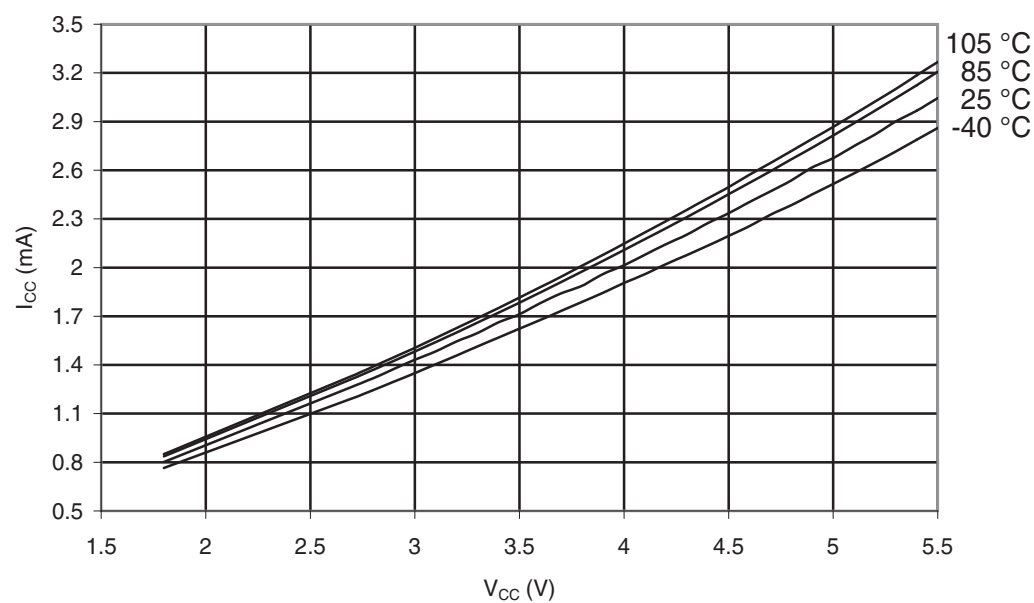
Figure 32-129. ATmega329P-105°C: Idle Supply Current vs. V_{CC} (Internal RC Oscillator, 8MHz)
