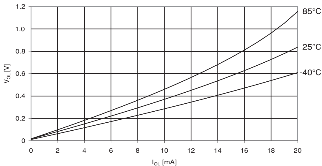
Figure 31-276. ATmega3290A: I/O pin output voltage vs. sink current, port B ( V_{CC} = 2.7V ).
