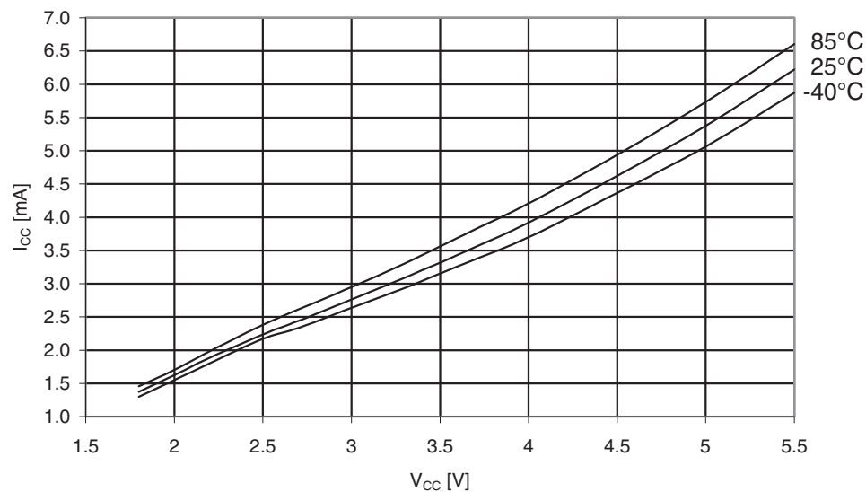
Figure 31-127. Atmel ATmega329A: Active supply current vs. V_{CC} (Internal RC oscillator, 8MHz).
