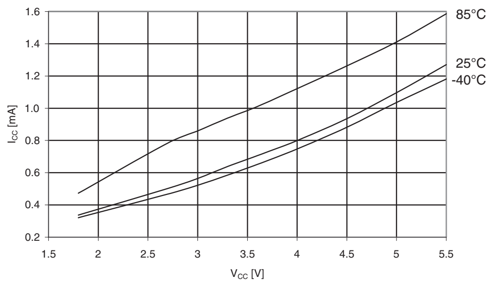
Figure 31-308. ATmega3290PA: Active supply current vs. V_{CC} (Internal RC oscillator, 1MHz).
