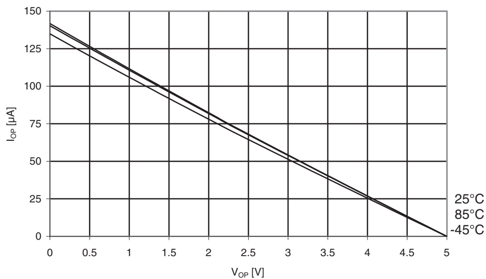
Figure 31-16. ATmega169A: I/O pin pull-up resistor current vs. input voltage ( V_{CC} = 5V ).
