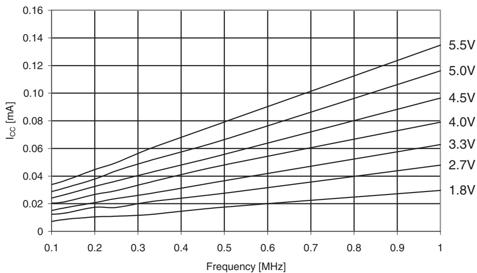
Figure 31-362. Atmel ATmega3290PA: Reset supply current vs. V_{CC} (0.1 - 1.0MHz, excluding current through the reset pull-up).
