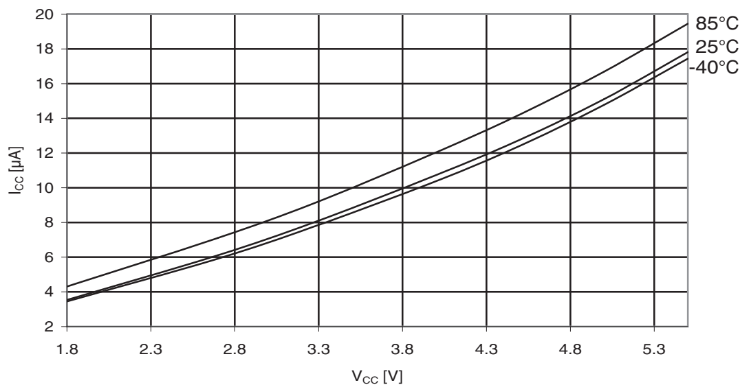
Figure 31-256. ATmega3290A: Power-down supply current vs. V_{CC} (Watchdog Timer enabled).
