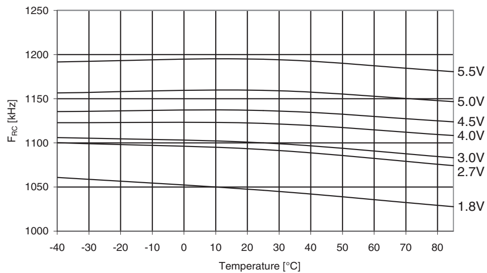
Figure 31-290. ATmega3290A: Watchdog Oscillator frequency vs. temperature.
