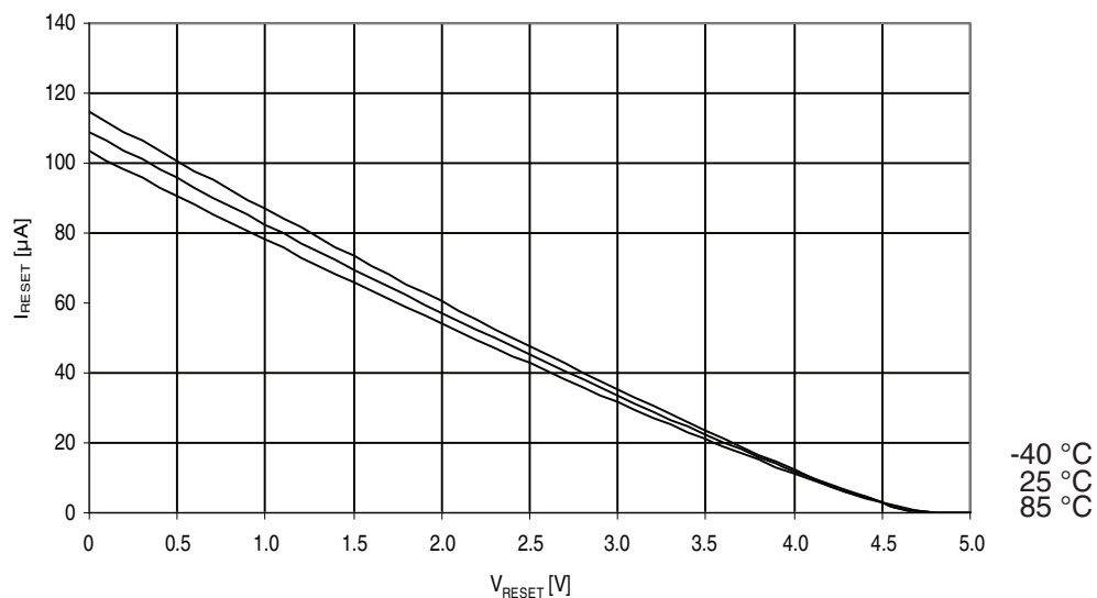
Figure 31-323. ATmega3290PA: Reset pull-up resistor current vs. reset pin voltage ( V_{CC}=5V ).
