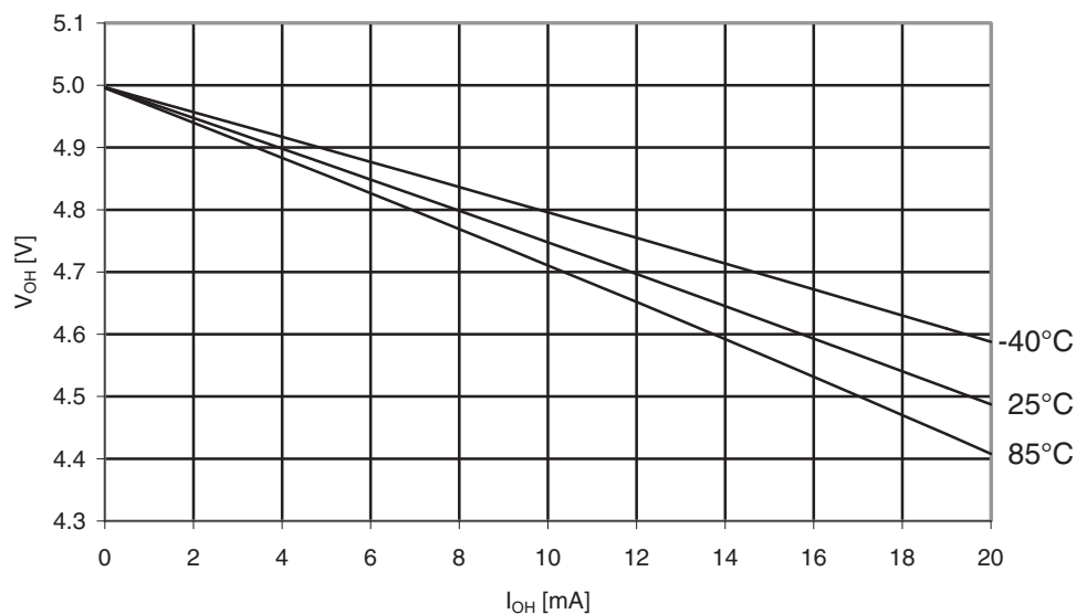
Figure 31-269. Atmel ATmega3290A: I/O pin output voltage vs. source current, port B ( V_{CC} = 5V ).
