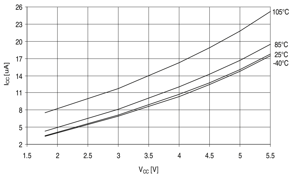
Figure 32-185. ATmega329PA - 105°C: Power-down Supply Current vs. V_{CC} (Watchdog Timer Enabled)
