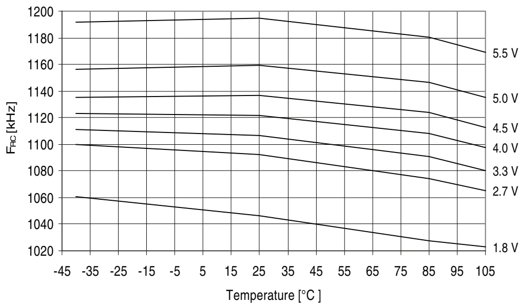
Figure 32-396. ATmega3290PA - 105°C: Watchdog Oscillator Frequency vs. Temperature
