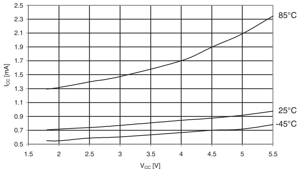
Figure 31-563. ATmega6490P: Standby supply current vs. V_{CC} (XTAL and resonator, Watchdog Timer disabled).
