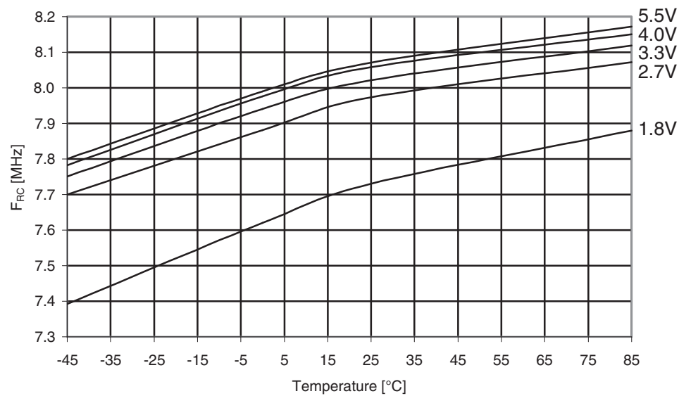
Figure 31-473. ATmega649P: Calibrated 8MHz RC oscillator frequency vs. temperature.
