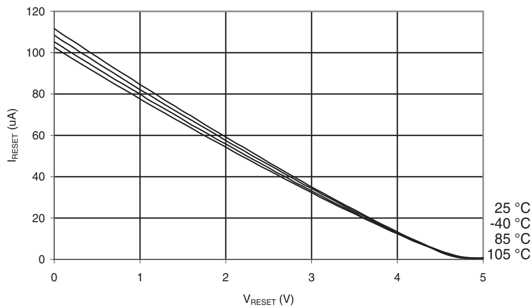
Figure 32-139. ATmega329P-105°C: Reset Pull-up Resistor Current vs. Reset Pin Voltage ( V_{CC} = 5V )
