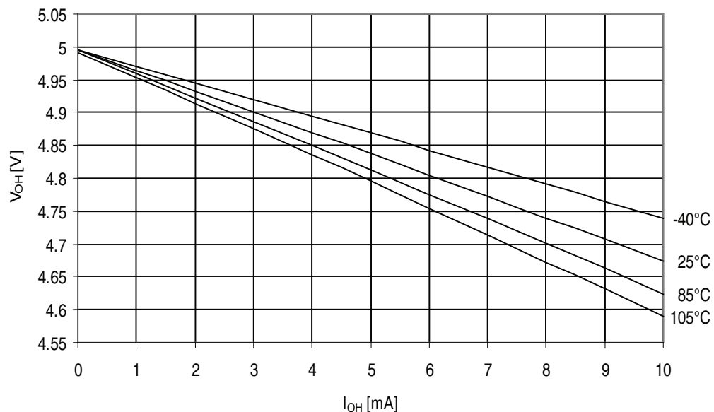
Figure 32-194. ATmega329PA - 105°C: I/O Pin Output Voltage vs. Source Current, Ports A, C, D, E, F, G ( V_{CC} = 5V )
