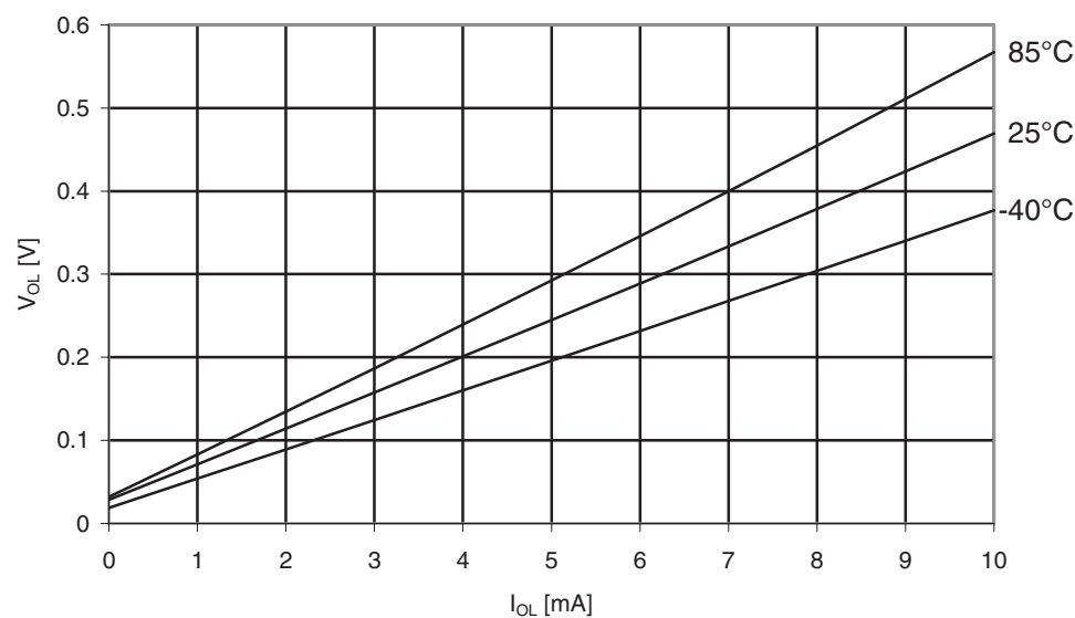
Figure 31-272. ATmega3290A: I/O pin output voltage vs. sink current, ports A, C, D, E, F, G ( V_{CC} = 5V ).
