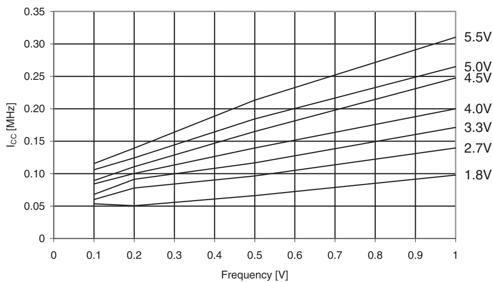
Figure 31-130. ATmega329A: Idle supply current vs. low frequency (0.1 - 1.0MHz).
