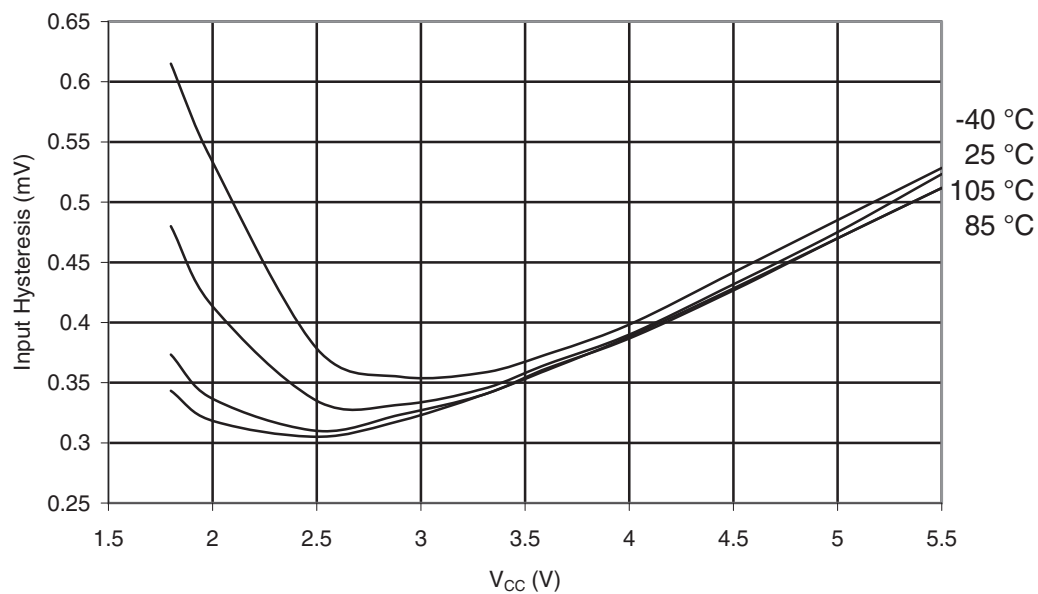
Figure 32-152. ATmega329P-105°C: I/O Pin Input Hysteresis vs. V_{CC}
