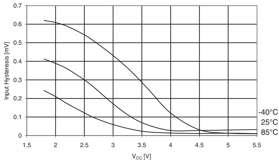
Figure 31-343. ATmega3290PA: Reset input pin Hysteresis vs. V_{CC} .
