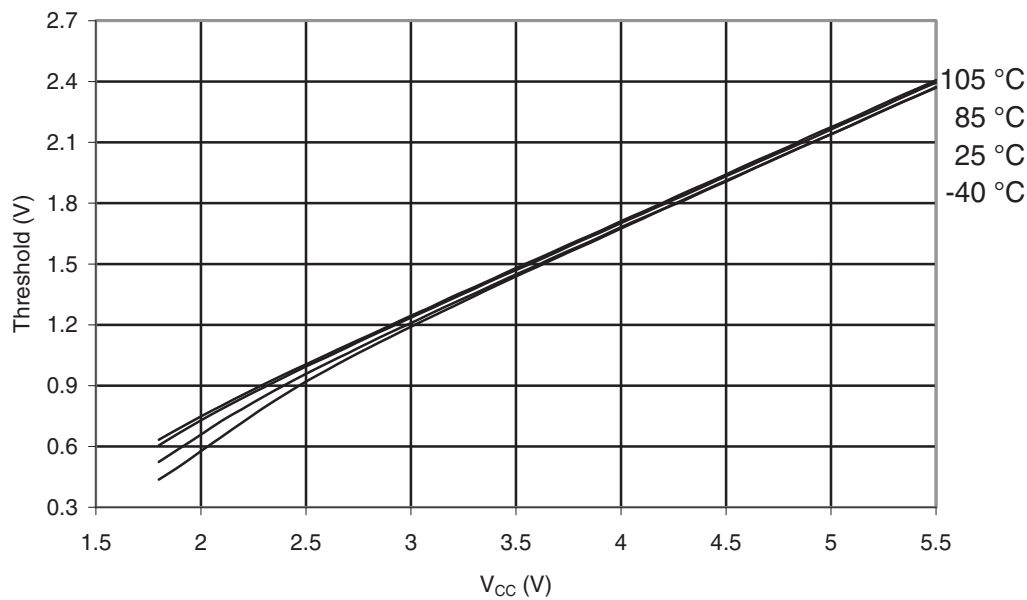
Figure 32-151. ATmega329P-105°C: I/O Pin Input Threshold Voltage vs. V_{CC} ( V_{IL} , I/O Pin Read as “0”)
