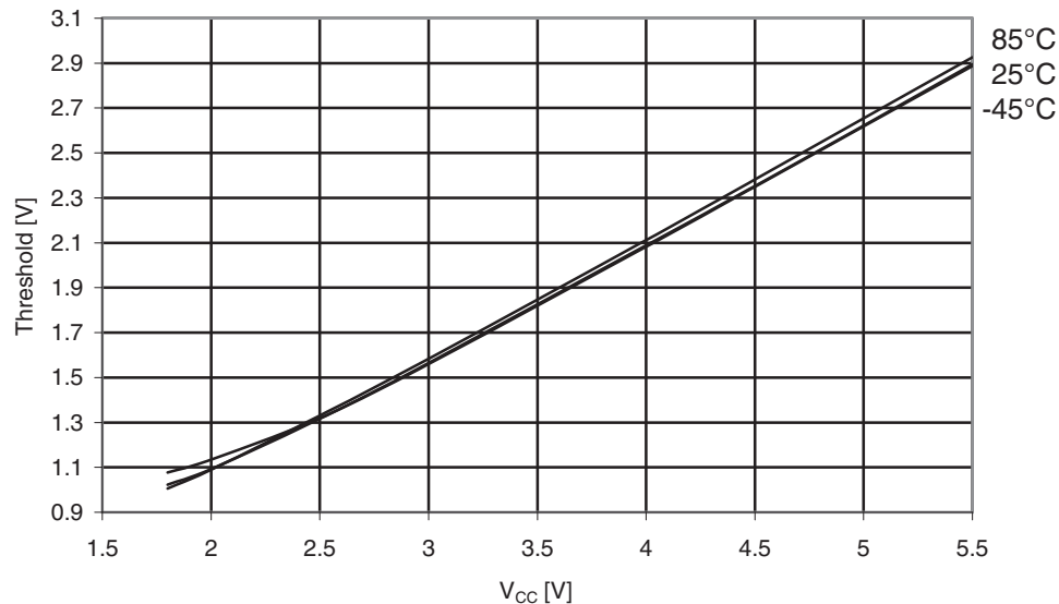
Figure 31-582. Atmel ATmega6490P: I/O pin input Threshold voltage vs. V_{CC} ( V_{IH} , I/O pin read as “1”).
