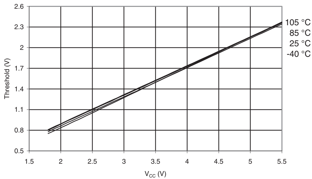
Figure 32-332. ATmega3290PA-105°C: Reset Input Threshold Voltage vs. V_{CC} ( V_{IL} , Reset Pin Read as “0”)
