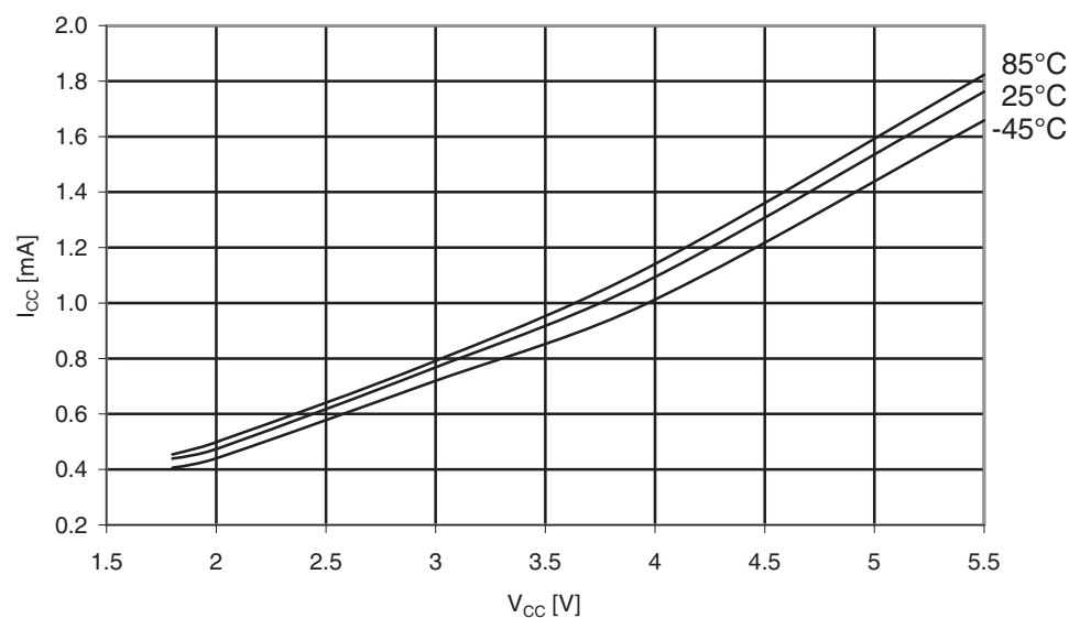
Figure 31-433. ATmega649P: Idle supply current vs. V_{CC} (Internal RC oscillator, 8MHz).
