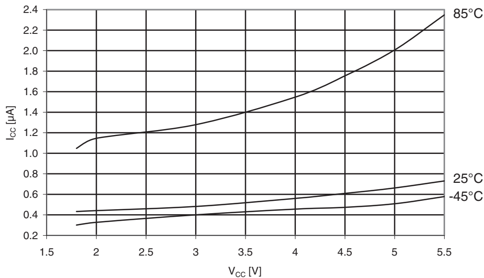
Figure 31-436. Atmel ATmega649P: Power-down supply current vs. V CC (Watchdog Timer disabled).
