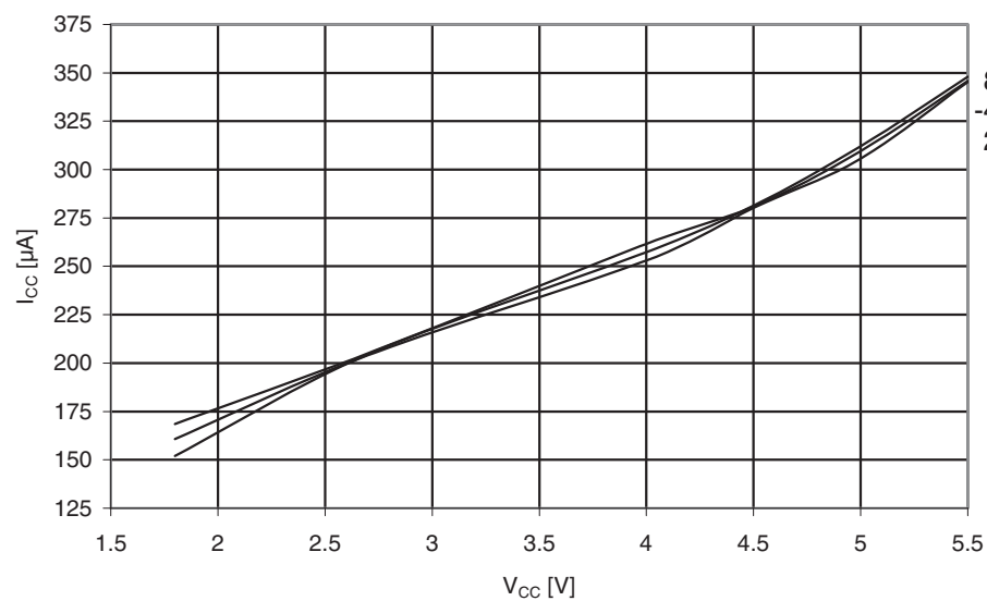
Figure 31-236. ATmega329PA: Active supply current with ADC at 200kHz vs. V_{CC} .
