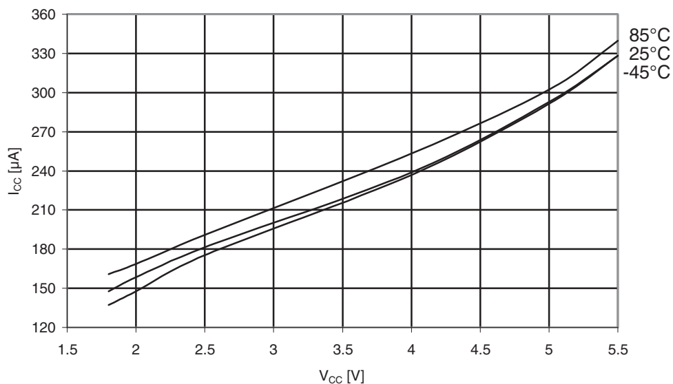
Figure 31-600. Atmel ATmega6490P: Active supply current with ADC at 200kHz vs. V_{CC} .
