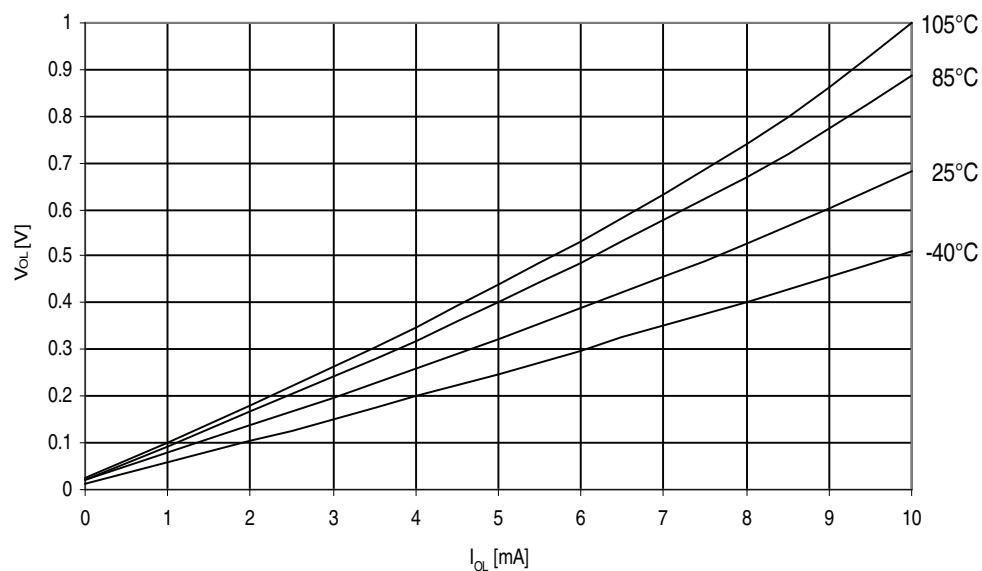
Figure 32-380. ATmega3290PA - 105°C: I/O Pin Output Voltage vs. Sink Current, Ports A, C, D, E, F, G ( V_{CC} = 3V )
