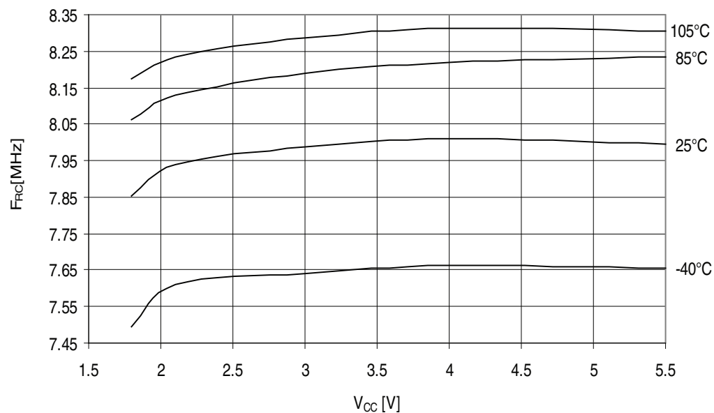
Figure 32-222. ATmega329PA - 105°C: Calibrated 8MHz RC Oscillator Frequency vs. V_{CC}
