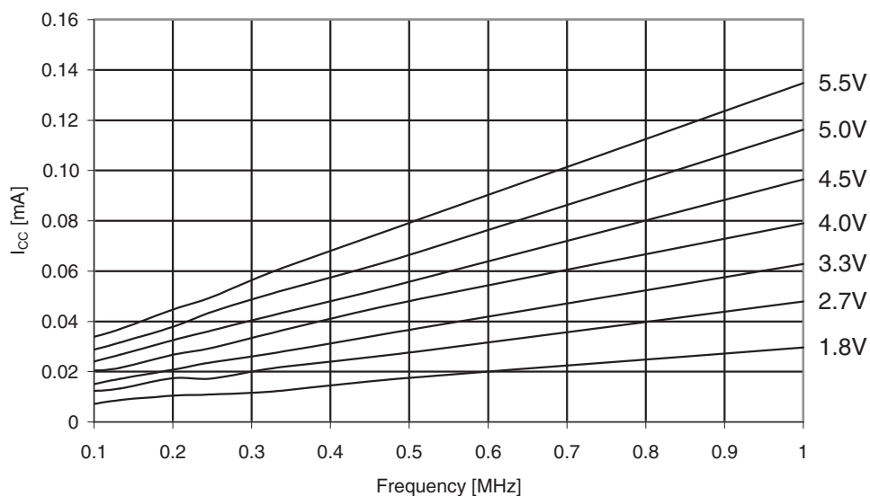
Figure 31-242. ATmega329PA: Reset supply current vs. V_{CC} (0.1 - 1.0MHz, excluding current through the reset pull-up).
