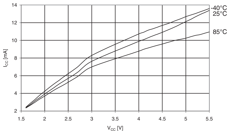
Figure 31-181. Atmel ATmega329A: Programming current vs. V_{CC} .
