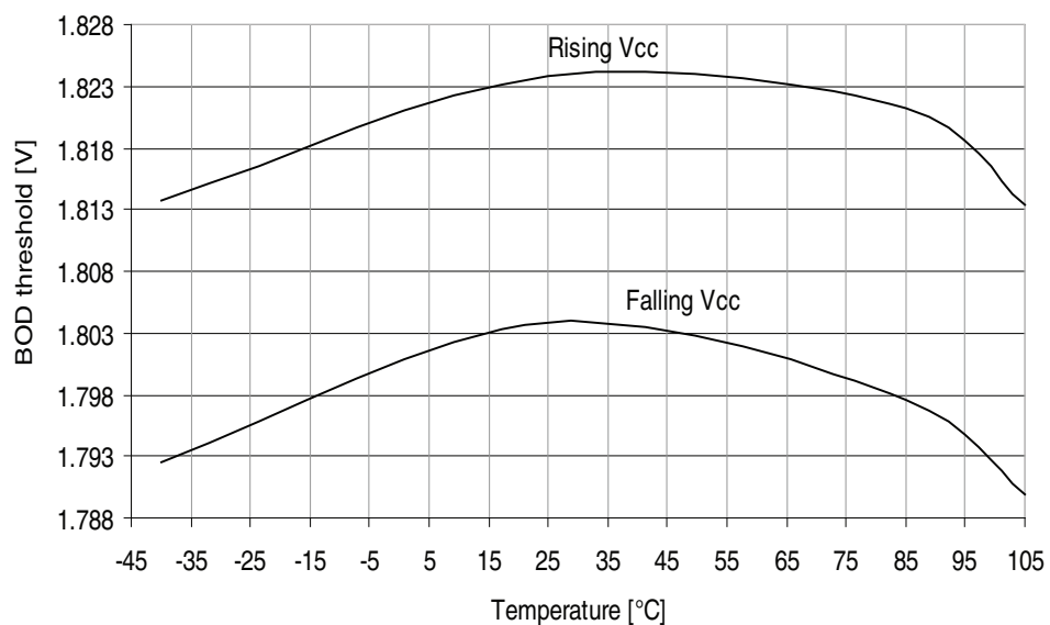
Figure 32-393. ATmega3290PA - 105°C: BOD Thresholds vs. Temperature (BOD Level is 1.8V)
