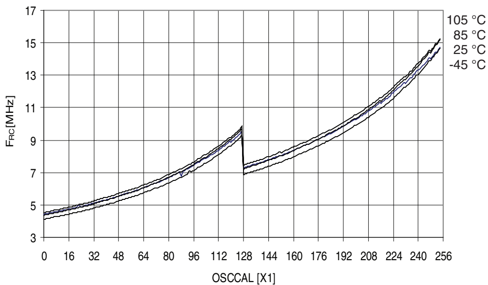
Figure 32-108. ATmega329A - 105°C: Calibrated 8MHz RC Oscillator Frequency vs. Oscal Value
