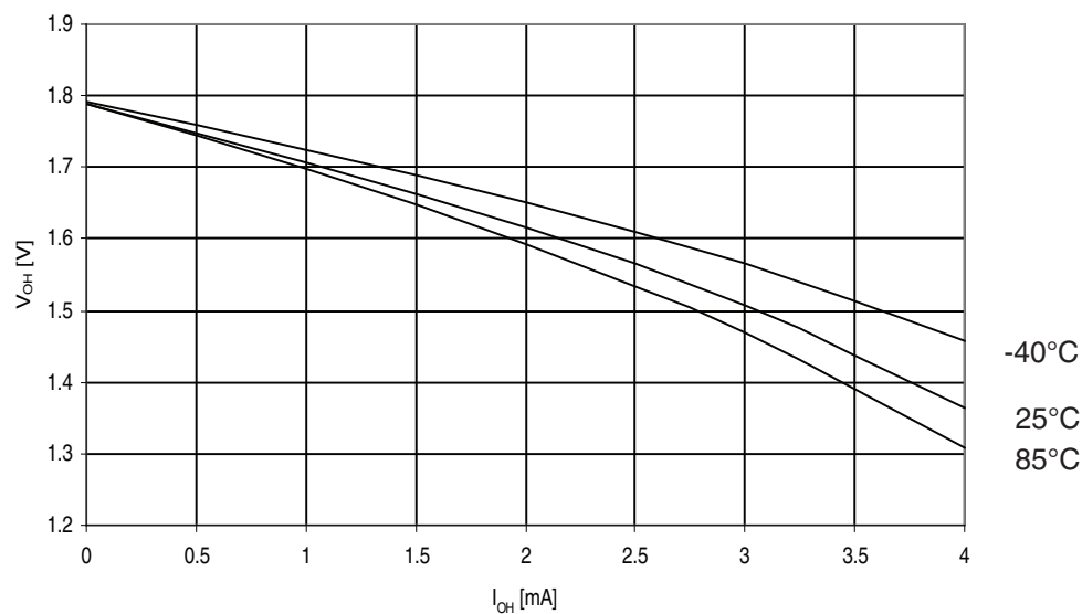
Figure 31-328. Atmel ATmega3290PA: I/O pin output voltage vs. source current, ports A, C, D, E, F, G ( V_{CC} = 1.8V ).
