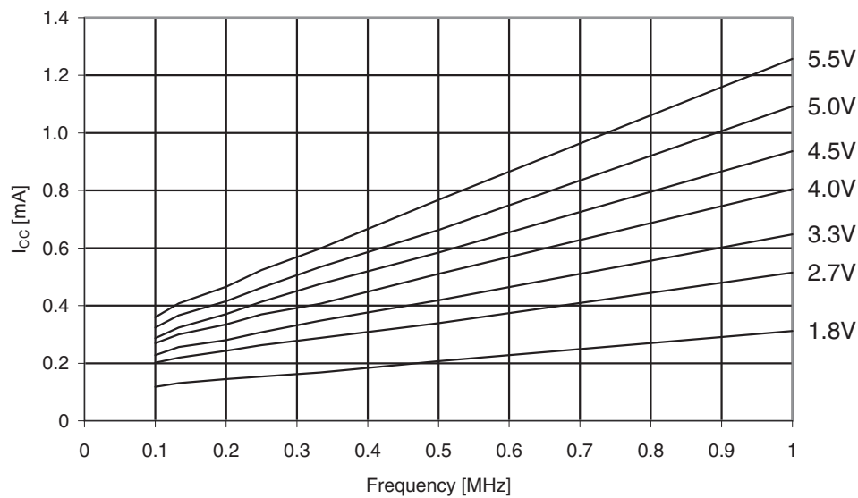
Figure 31-185. ATmega329PA: Active supply current vs. low frequency (0.1 - 1.0MHz).
