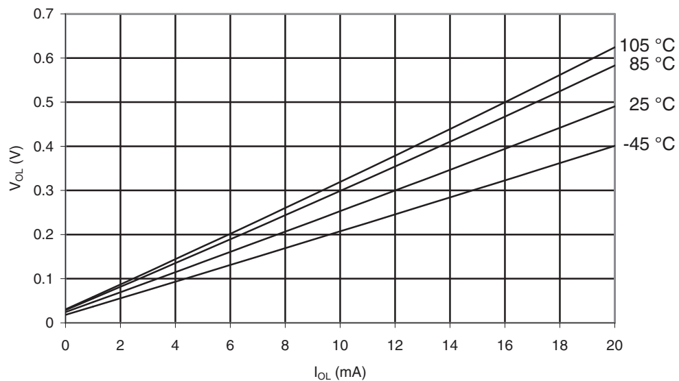
Figure 32-30. ATmega169PA-105°C: I/O Pin Output Voltage vs. Sink Current, PortB ( V_{CC}=5V )
