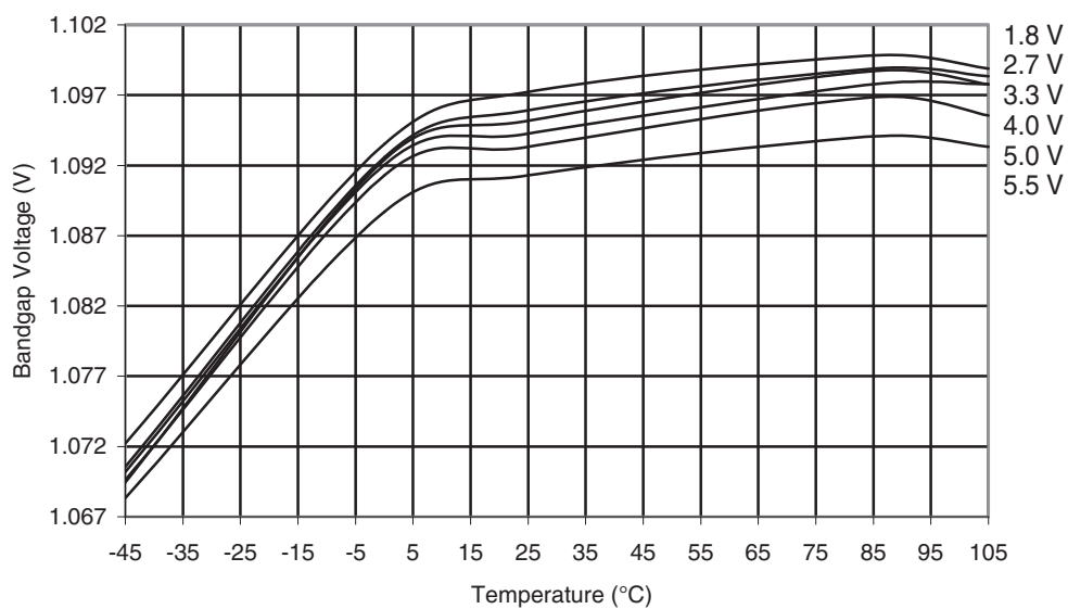
Figure 32-43. ATmega169PA-105°C: Bandgap Voltage vs. Temperature
