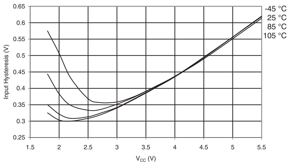
Figure 32-35. ATmega169PA-105°C: I/O Pin Input Hysteresis vs. V_{CC}
