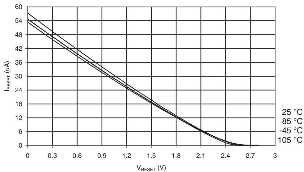
Figure 32-19. ATmega169PA-105°C: Reset Pull-up Resistor Current vs. Reset Pin Voltage ( V_{CC} = 2.7V )
