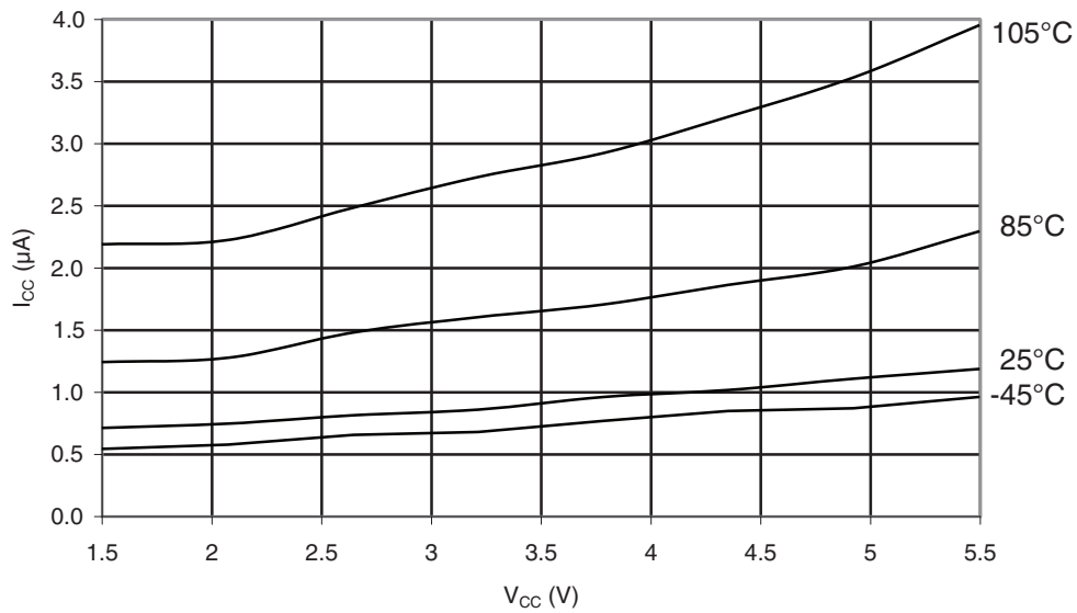
Figure 32-364. ATmega3290PA - 105°C: Power-save Supply Current vs. V_{CC} (Watchdog Timer Disabled)
