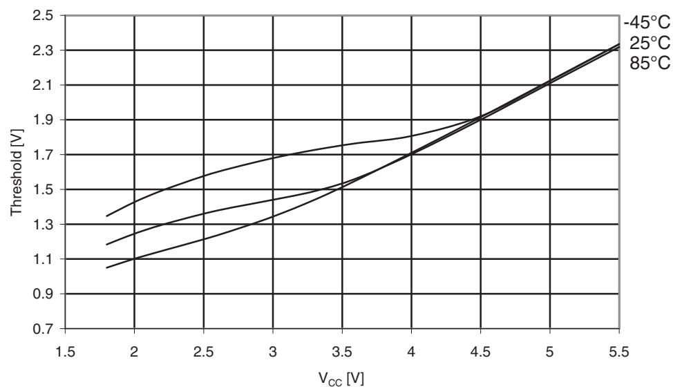
Figure 31-99. Atmel ATmega169PA: Reset Input Threshold voltage vs. V_{CC} ( V_{IH} , reset pin read as “1”).
