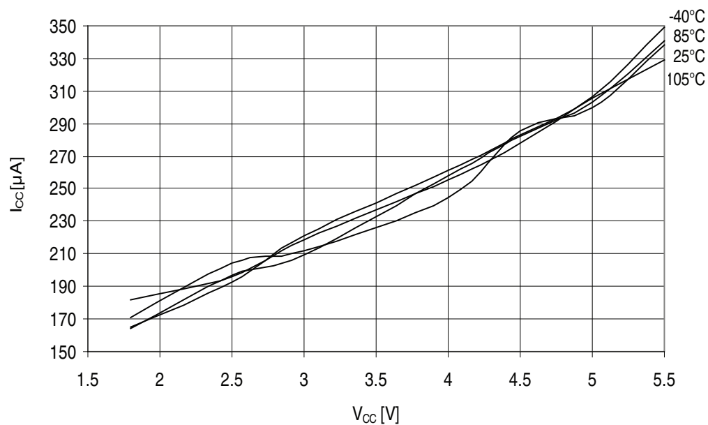
Figure 32-113. ATmega329A - 105°C: Active Supply Current with ADC at 2MHz vs. V_{CC} )
