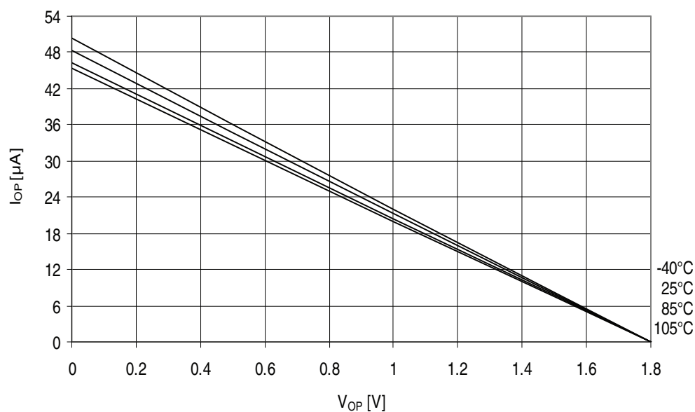
Figure 32-369. ATmega3290PA - 105°C: I/O Pin Pull-up Resistor Current vs. Input Voltage ( V_{CC} = 1.8V )
