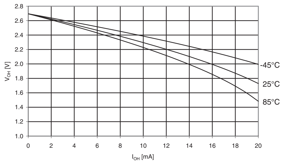
Figure 31-88. ATmega169PA: I/O pin output voltage vs. Source current, port B ( V_{CC} = 2.7V ).
