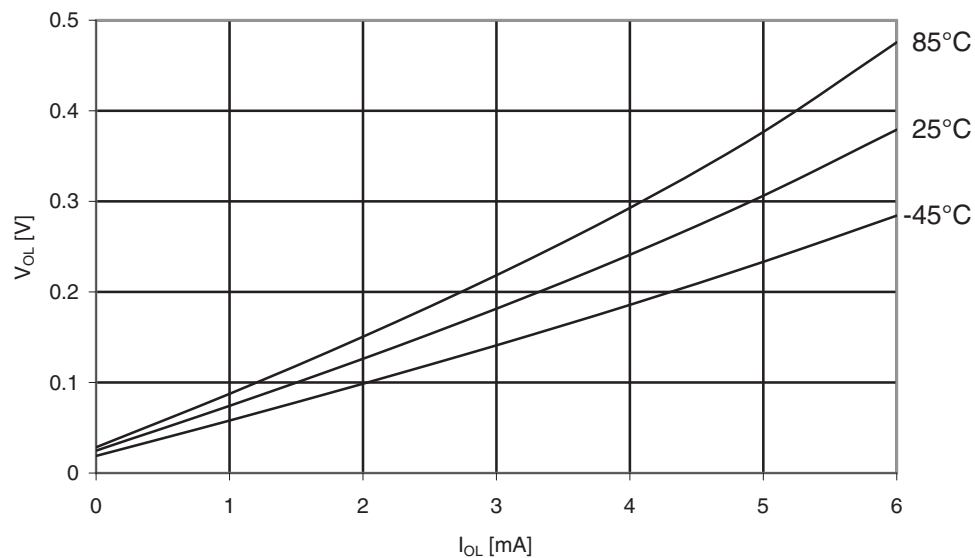
Figure 31-95. Atmel ATmega169PA: I/O pin output voltage vs. Sink current, port B ( V_{CC} = 1.8V ).
