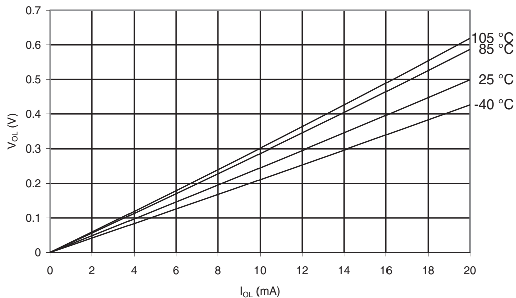
Figure 32-146. ATmega329P-105°C: I/O Pin Output Voltage vs. Sink Current, Ports A, C, D, E, F, G ( V_{CC} = 5V )
