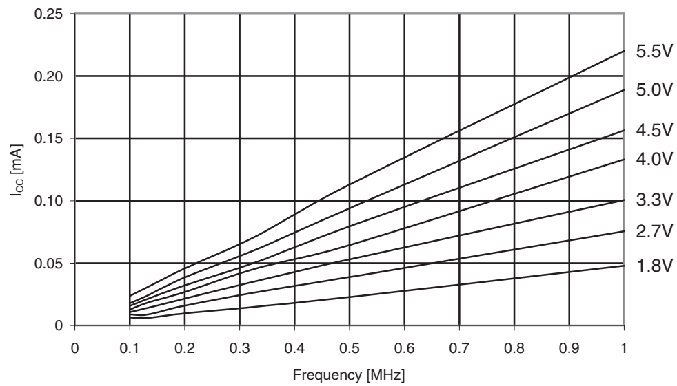
Figure 31-6. Atmel ATmega169A: Idle supply current vs. low frequency (0.1 - 1.0MHz).
