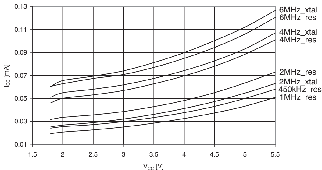
Figure 31-319. ATmega3290PA: Standby Supply current vs. V_{CC} (XTAL and resonator, Watchdog Timer disabled).
