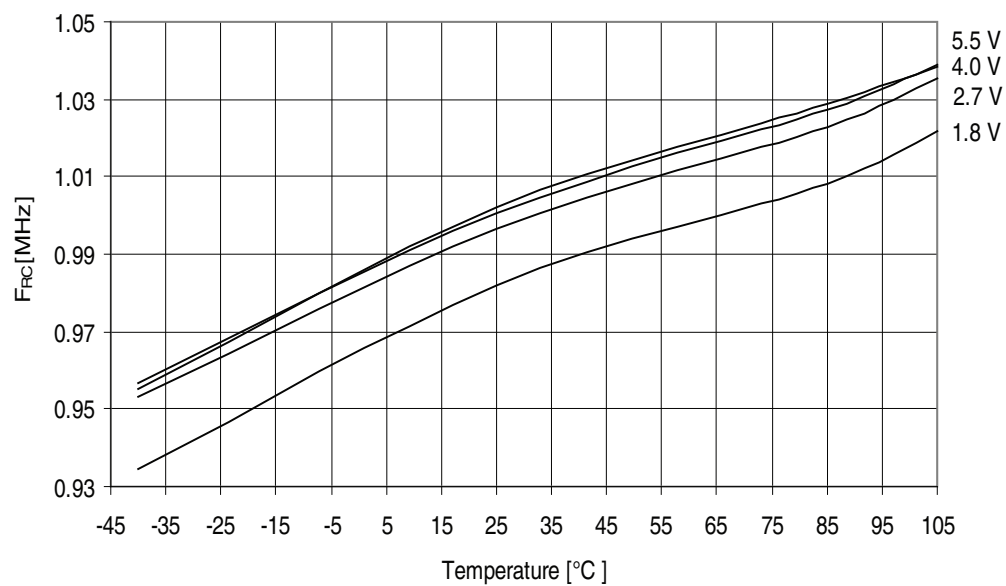
Figure 32-104. AATmega329A - 105°C: Calibrated 1MHz RC Oscillator Frequency vs. Temperature
