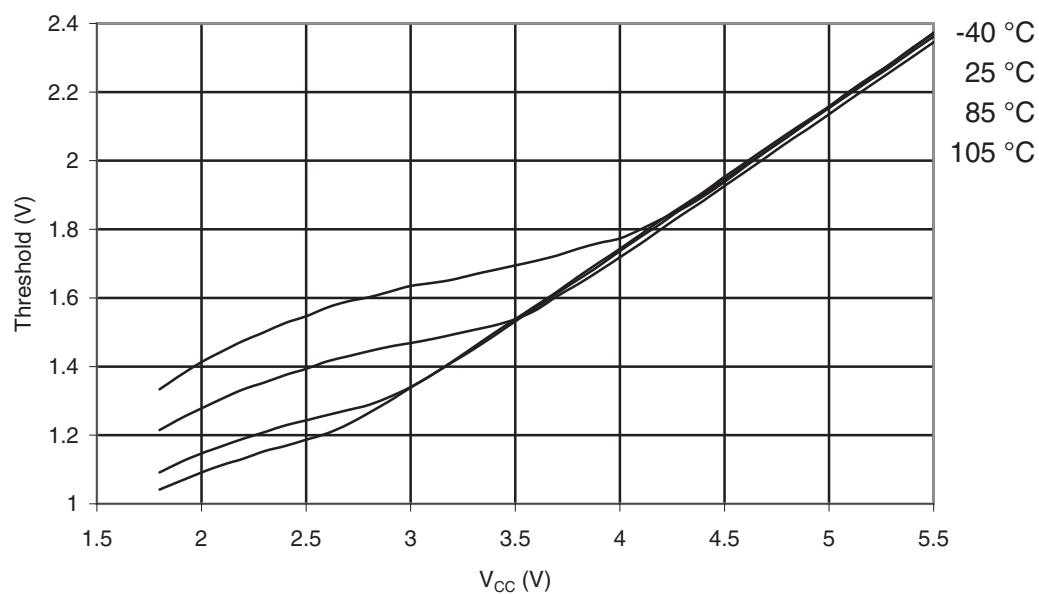
Figure 32-153. ATmega329P-105°C: Reset Input Threshold Voltage vs. V_{CC} ( V_{IH} , Reset Pin Read as “1”)
