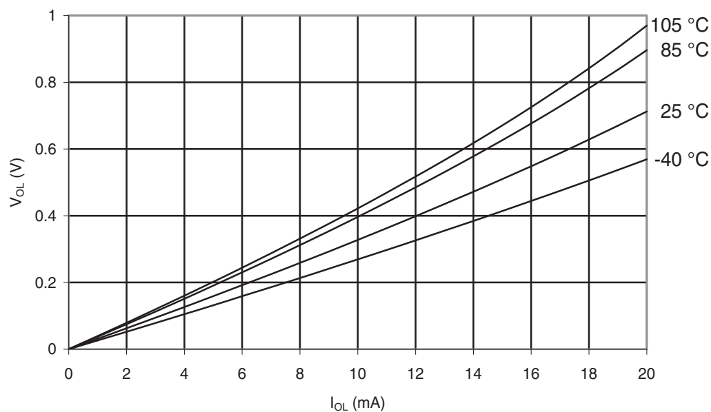
Figure 32-325. ATmega3290PA-105°C: I/O Pin Output Voltage vs. Sink Current, Ports A, C, D, E, F, G ( V_{CC} = 3V )
