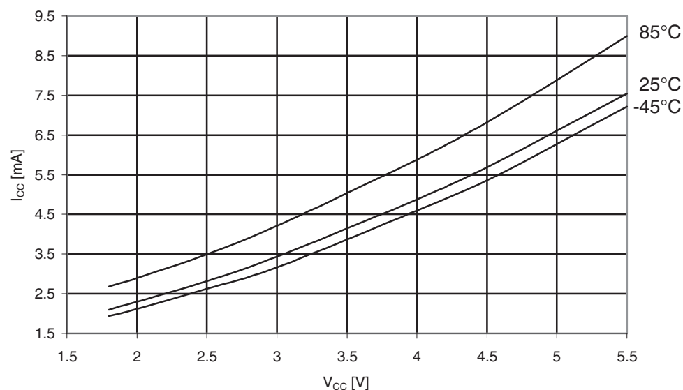
Figure 31-557. ATmega6490P: Idle supply current vs. V_{CC} (32kHz watch XTAL).
