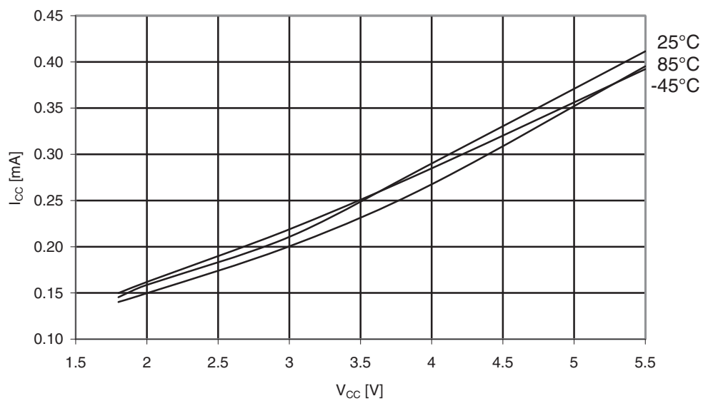
Figure 31-551. ATmega6490P: Active supply current vs. V_{CC} (Internal RC oscillator, 1MHz).
