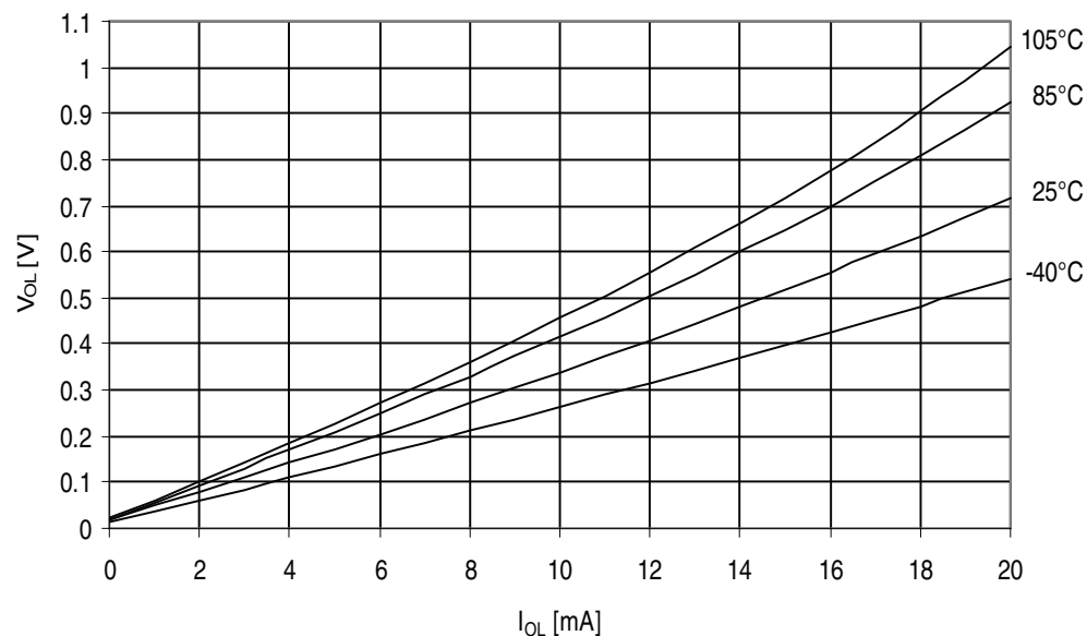
Figure 32-268. ATmega3290A - 105°C: I/O Pin Output Voltage vs. Sink Current, Port B ( V_{CC} = 1.8V )
