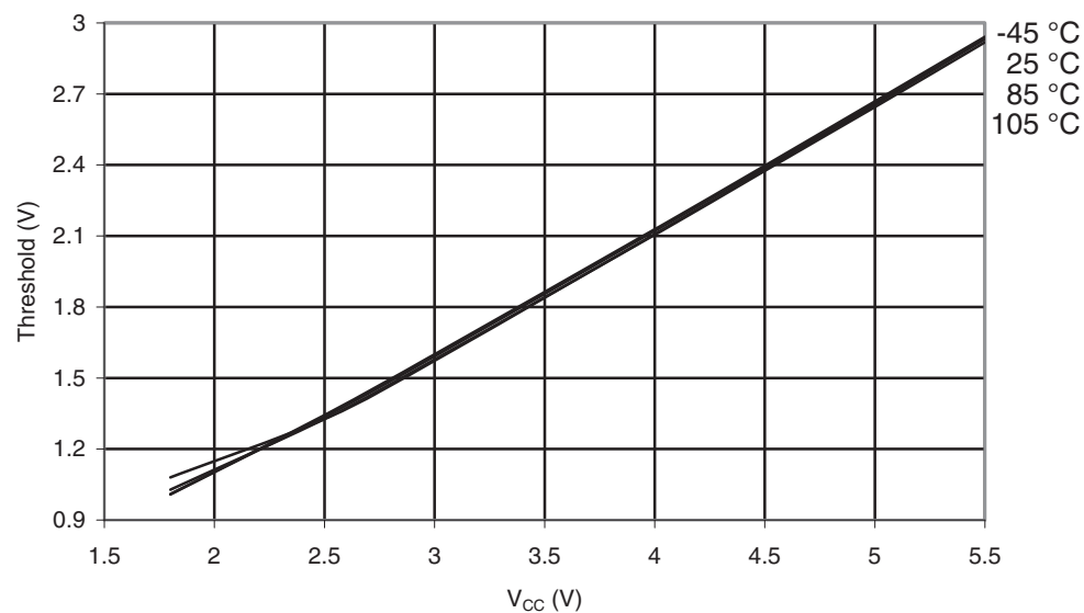
Figure 32-33. ATmega169PA-105°C: I/O Pin Input Threshold Voltage vs. V_{CC} ( V_{IH} , I/O Pin Read as “1”)
