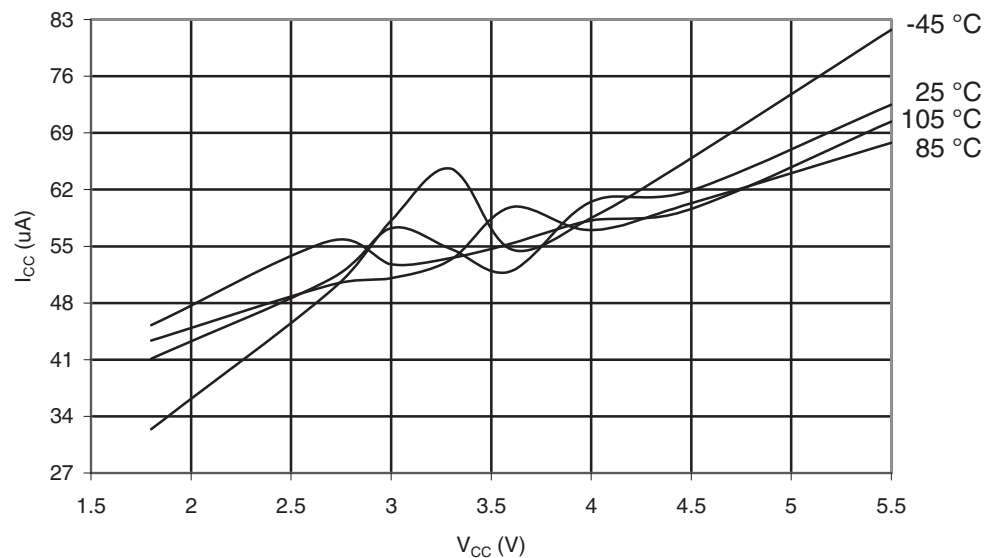
Figure 32-54. ATmega169PA-105°C: Analog Comparator Current vs. V_{CC}
