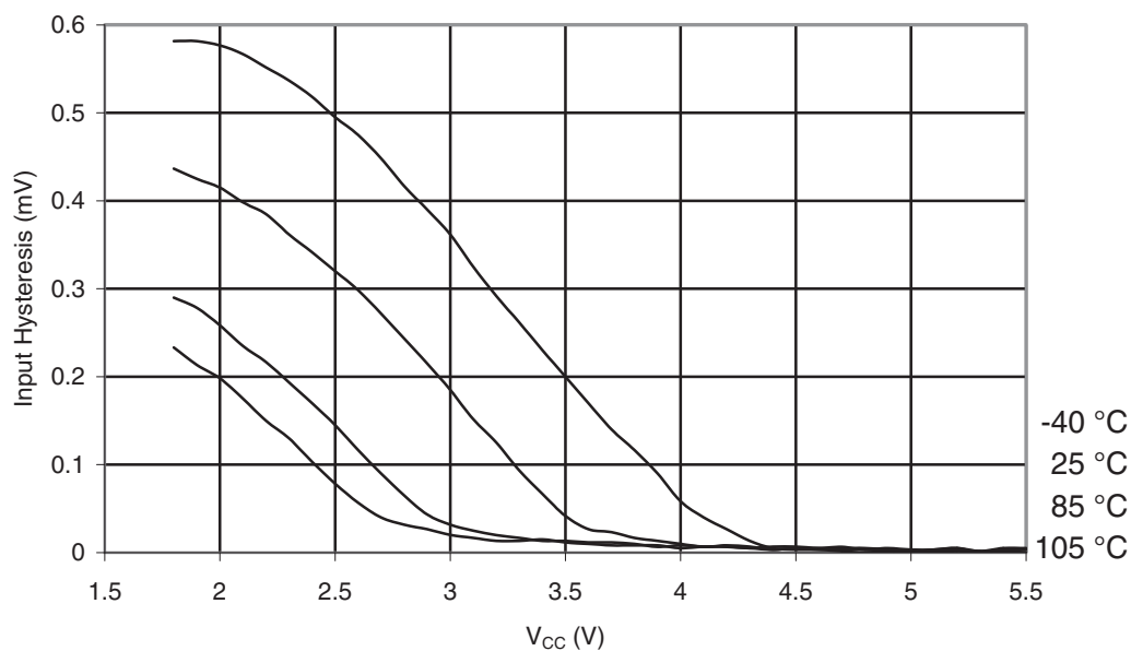
Figure 32-155. ATmega329P-105°C: Reset Input Pin Hysteresis vs. V_{CC}
