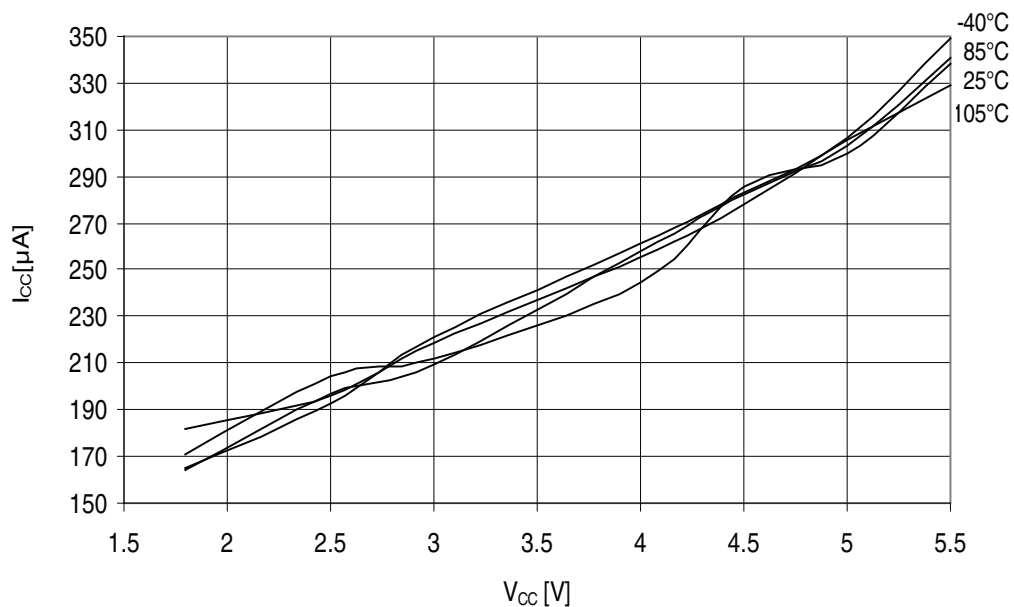
Figure 32-406. ATmega3290PA - 105°C: Active Supply Current with ADC at 1MHz vs. V_{CC} )
