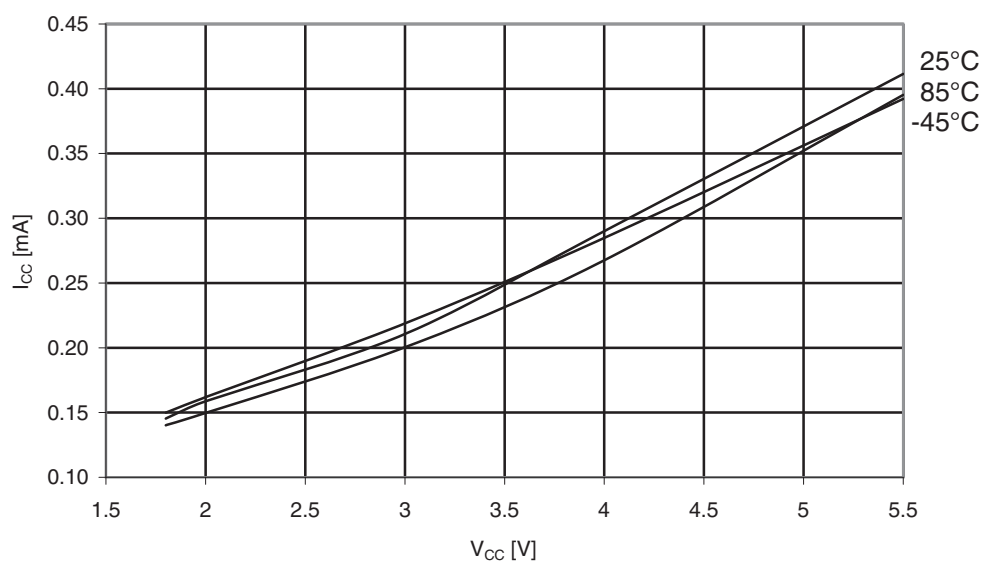
Figure 31-490. ATmega6490A: Active supply current vs. V_{CC} (Internal RC oscillator, 1MHz).
