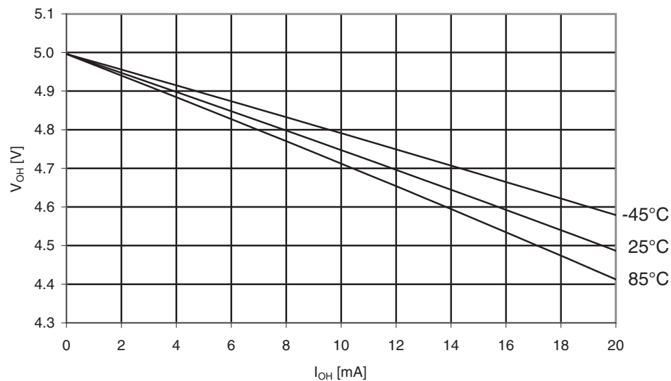
Figure 31-87. Atmel ATmega169PA: I/O pin output voltage vs. Source current, Port B ( V_{CC} = 5V ).
