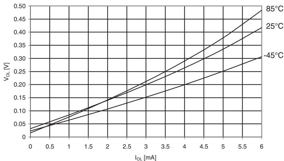
Figure 31-581. ATmega6490P: I/O pin output voltage vs. sink current, port B ( V_{CC} = 1.8V ).
