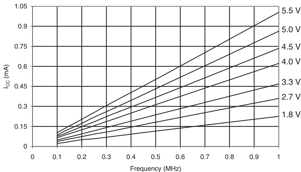
Figure 32-1. ATmega169PA-105°C: Active Supply Current vs. Frequency (0.1 - 1.0MHz)
