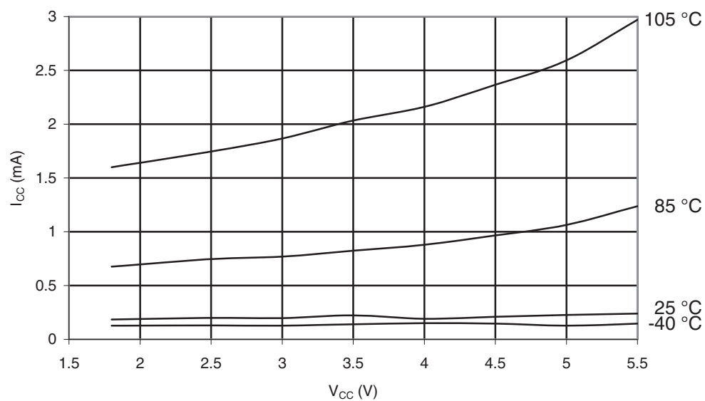
Figure 32-131. ATmega329P-105°C: Idle Supply Current vs. V_{CC} (32kHz Watch Crystal)
