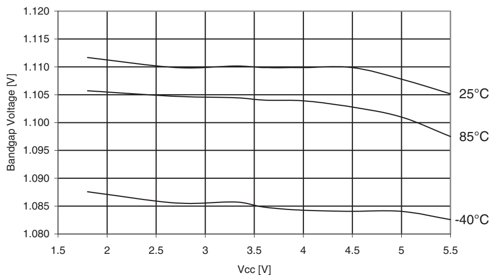
Figure 31-347. ATmega3290PA: Bandgap voltage vs. V_{CC} .
