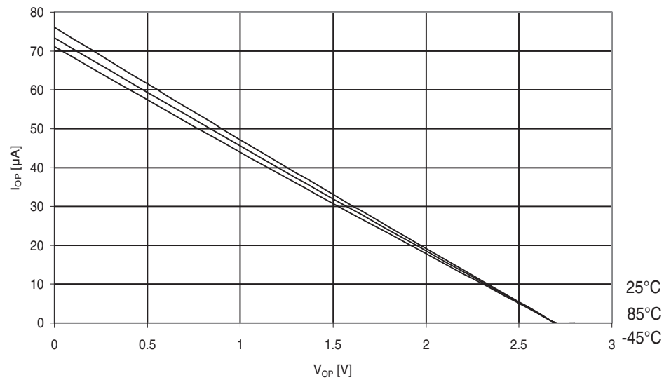
Figure 31-504. ATmega6490A: I/O pin pull-up resistor current vs. input voltage ( V_{CC} = 2.7V ).
