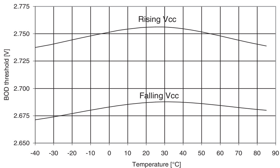
Figure 31-345. ATmega3290PA: BOD Thresholds vs. temperature (BOD level is 2.7V).
