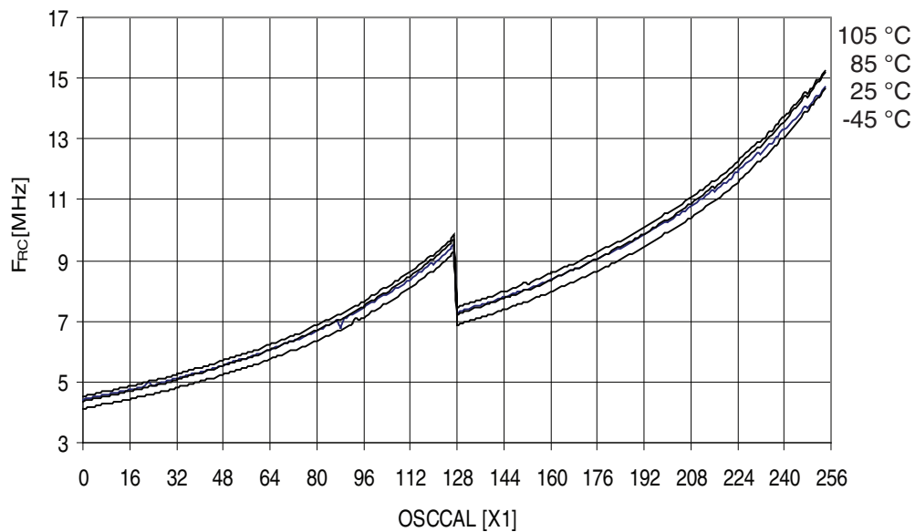
Figure 32-402. ATmega3290PA - 105°C: Calibrated 8MHz RC Oscillator Frequency vs. Oscal Value
