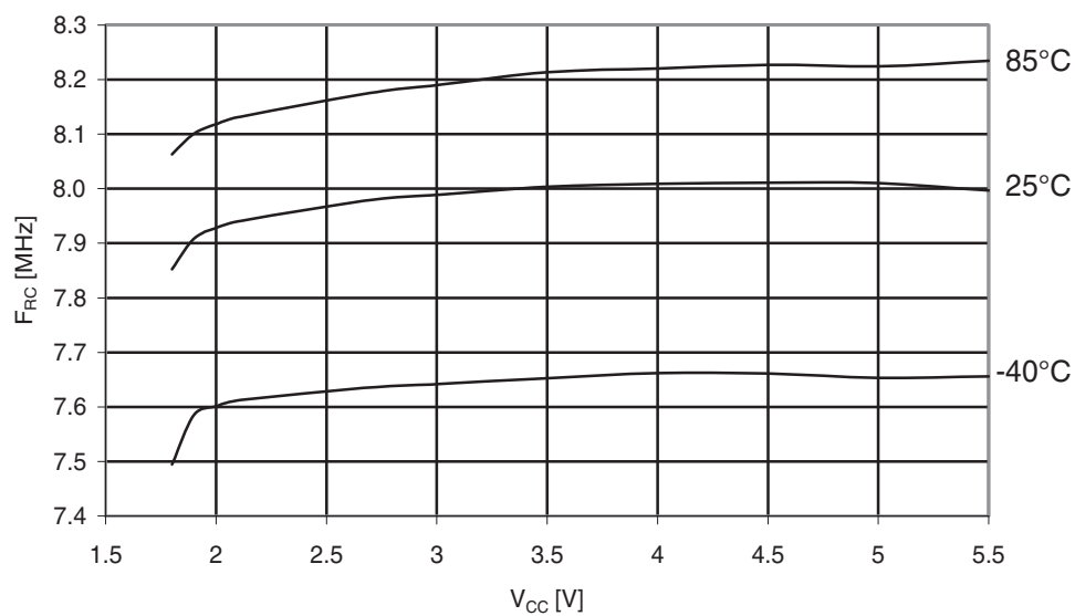
Figure 31-172. ATmega329A: Calibrated 8MHz RC oscillator frequency vs. V_{CC} .
