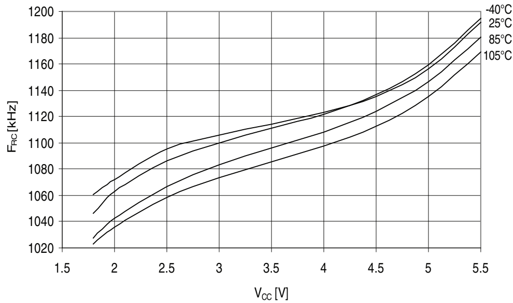
Figure 32-397. ATmega3290PA - 105°C: Watchdog Oscillator Frequency vs. V CC
