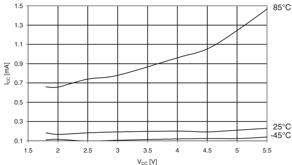
Figure 31-438. Atmel ATmega649P: Power-down supply current vs. V_{CC} (32kHz watch XTAL).
