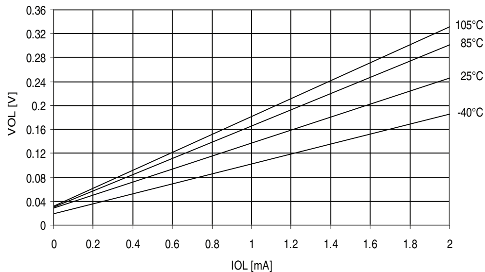
Figure 32-202. ATmega329PA - 105°C: I/O Pin Output Voltage vs. Sink Current, Ports A, C, D, E, F, G ( V_{CC} = 1.8V )
