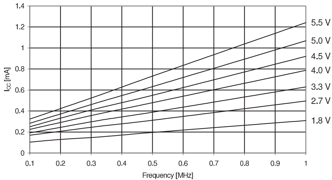
Figure 32-174. ATmega329PA - 105°C: Active Supply Current vs. Frequency (0.1 - 1.0MHz)
