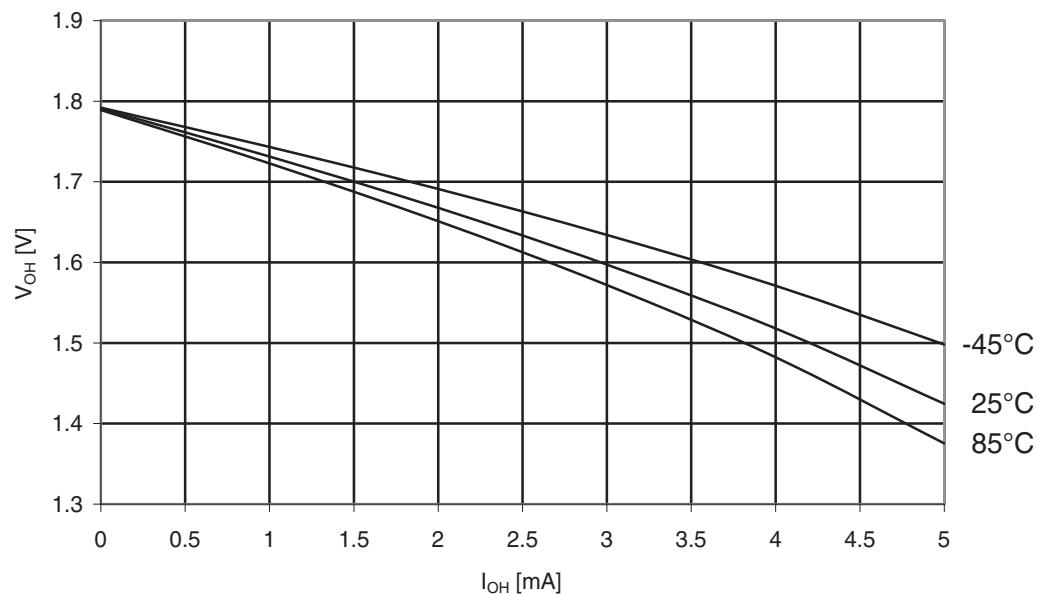
Figure 31-89. Atmel ATmega169PA: I/O pin output voltage vs. Source current, port B ( V_{CC} = 1.8V ).
