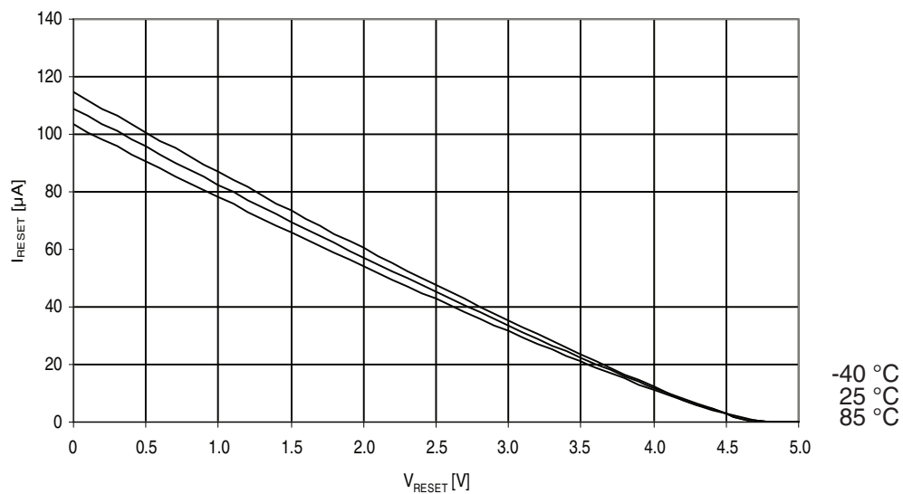
Figure 31-203. Atmel ATmega329PA: Reset pull-up resistor current vs. reset pin voltage ( V_{CC} = 5V ).
