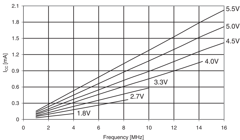
Figure 31-61. Atmel ATmega169A: Reset supply current vs. V_{CC} (1 - 16MHz, excluding current through the reset pull-up).
