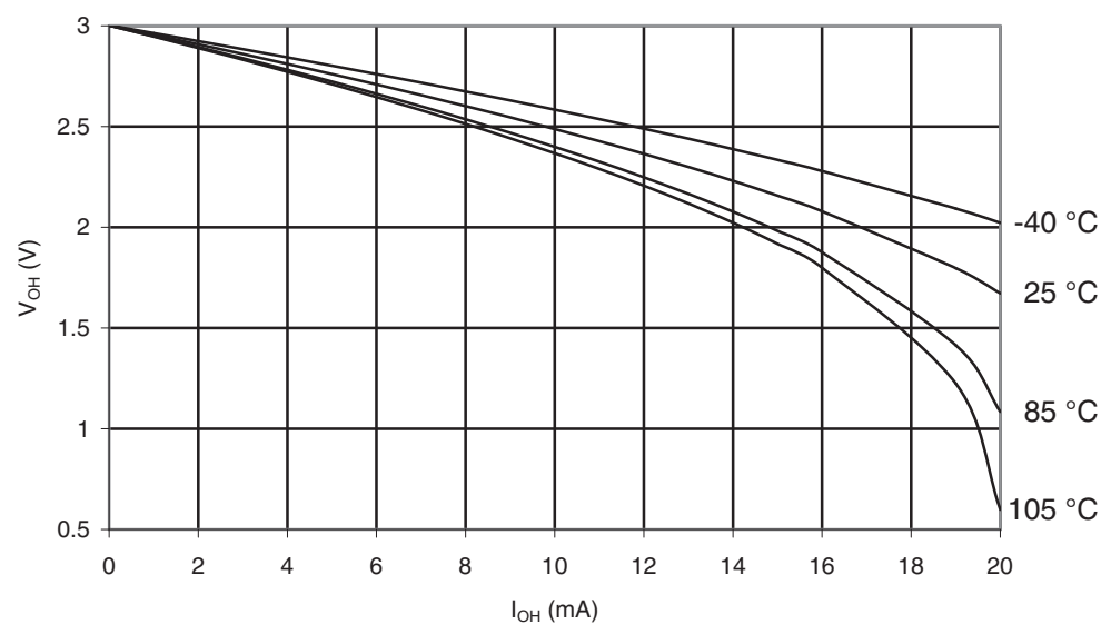
Figure 32-323. ATmega3290PA-105°C: I/O Pin Output Voltage vs. Source Current, Port B ( V_{CC} = 3V )
