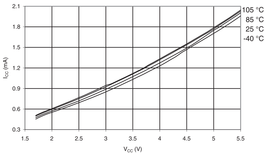
Figure 32-125. ATmega329P-105°C: Active Supply Current vs. V_{CC} (Internal RC Oscillator, 1MHz)
