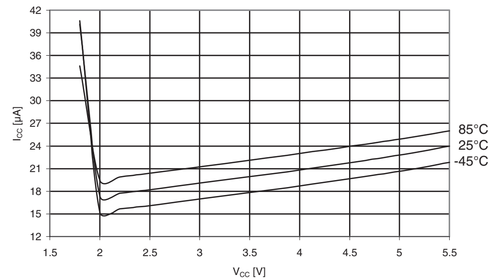
Figure 31-537. Atmel ATmega6490A: Brownout Detector current vs. V_{CC} .
