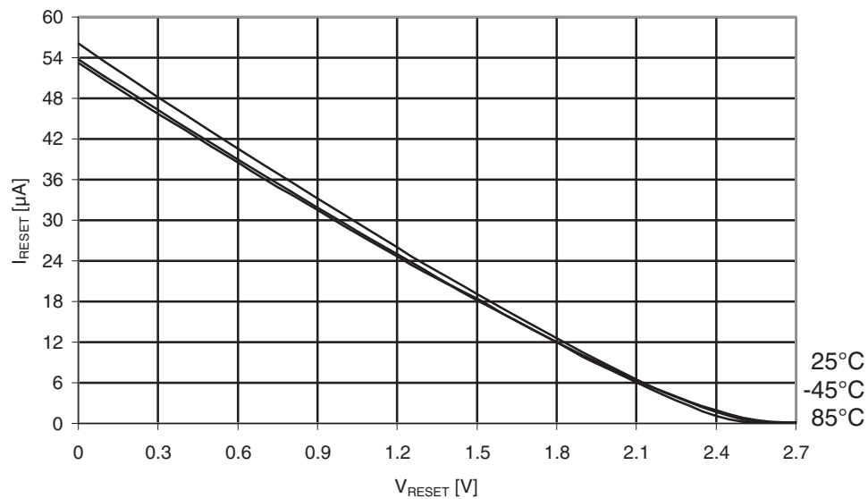
Figure 31-507. Atmel ATmega6490A: Reset pull-up resistor current vs. reset pin voltage ( V_{CC} = 2.7V ).
