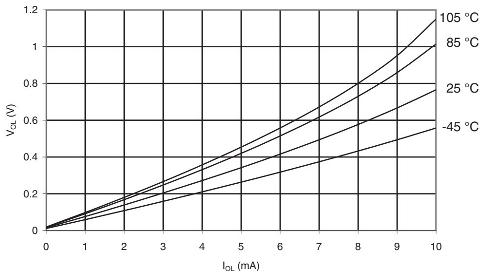
Figure 32-28. ATmega169PA-105°C: I/O Pin Output Voltage vs. Sink Current, Ports A, C, D, E, F, G ( V_{CC} = 2.7V )
