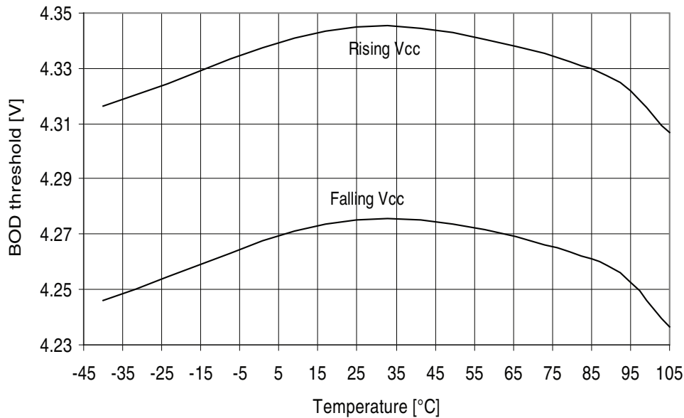
Figure 32-97. ATmega329A - 105°C: BOD Thresholds vs. Temperature (BOD Level is 4.3V)
