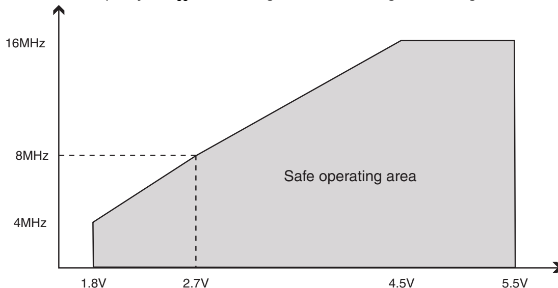
Figure 29-1. Maximum frequency vs. V_{CC} , Atmel ATmega169A/169PA/ATmega649A/ATmega649P.
