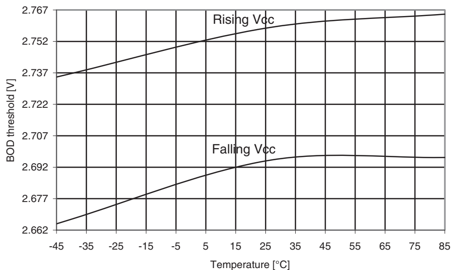
Figure 31-41. Atmel ATmega169A: BOD Thresholds vs. temperature (BOD level is 2.7V).
