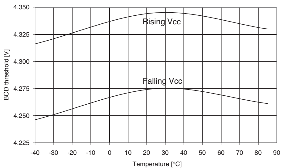
Figure 31-344. Atmel ATmega3290PA: BOD Thresholds vs. temperature (BOD level is 4.3V).
