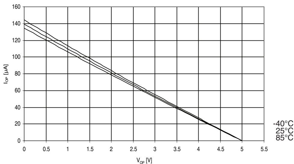
Figure 31-260. ATmega3290A: I/O pin pull-up resistor current vs. input voltage ( V_{CC} = 5V ).
