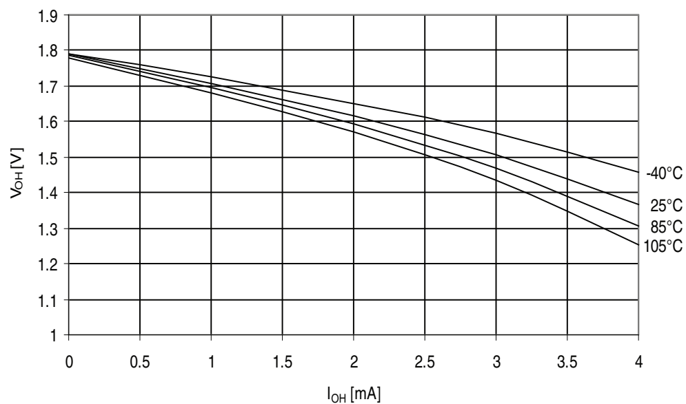
Figure 32-375. ATmega3290PA - 105°C: I/O Pin Output Voltage vs. Source Current, Ports A, C, D, E, F, G ( V_{CC} = 1.8V )
