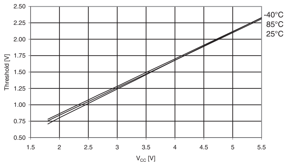
Figure 31-222. ATmega329PA: Reset Input Threshold voltage vs. V_{CC} ( V_{IL} , reset pin read as “0”).
