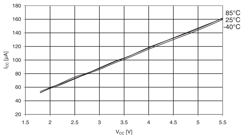
Figure 31-178. ATmega329A: AREF external reference current vs. V_{CC} .
