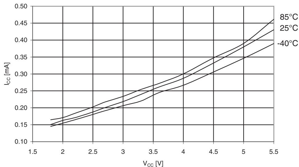
Figure 31-253. ATmega3290A: Idle Supply Current vs. V_{CC} (Internal RC Oscillator, 1MHz)
