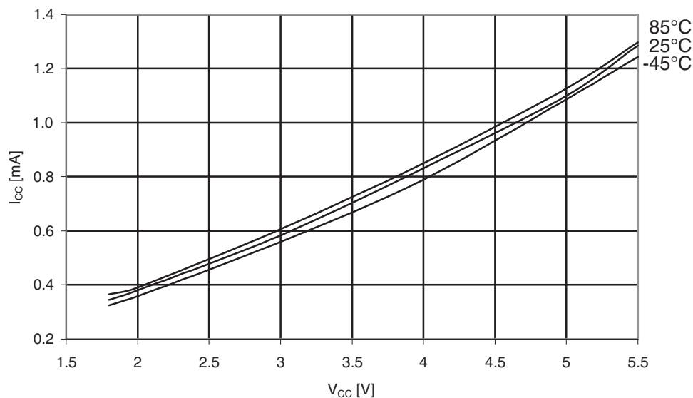
Figure 31-373. Atmel ATmega649A: Idle supply current vs. V_{CC} (Internal RC oscillator, 1MHz).
