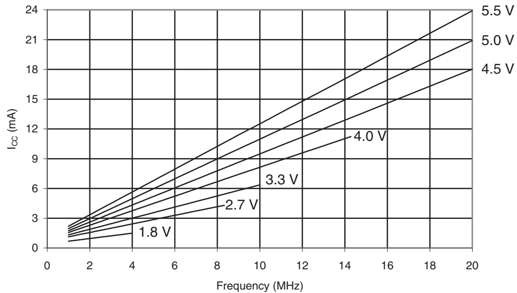
Figure 32-123. ATmega329P-105°C: Active Supply Current vs. Frequency (1 - 20MHz)
