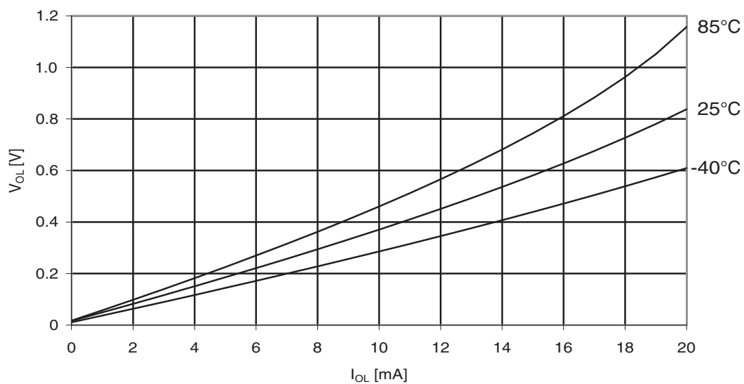
Figure 31-216. ATmega329PA: I/O pin output voltage vs. sink current, port B ( V_{CC} = 2.7V ).
