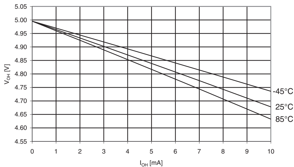
Figure 31-84. ATmega169PA: I/O pin output voltage vs. Source current, ports A, C, D, E, F, G ( V_{CC} = 5V ).
