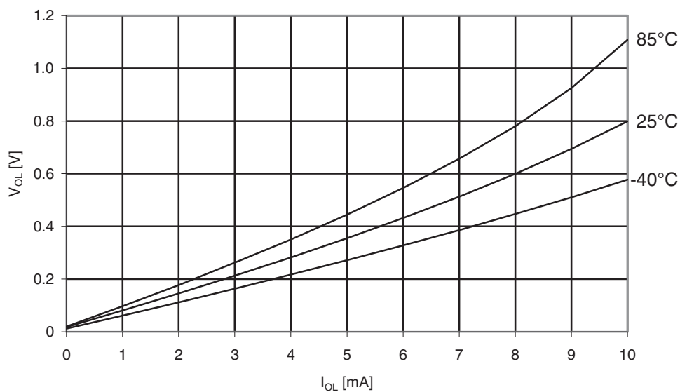
Figure 31-153. Atmel ATmega329A. I/O pin output voltage vs. sink current, ports A, C, D, E, F, G ( V_{CC} = 2.7V ).
