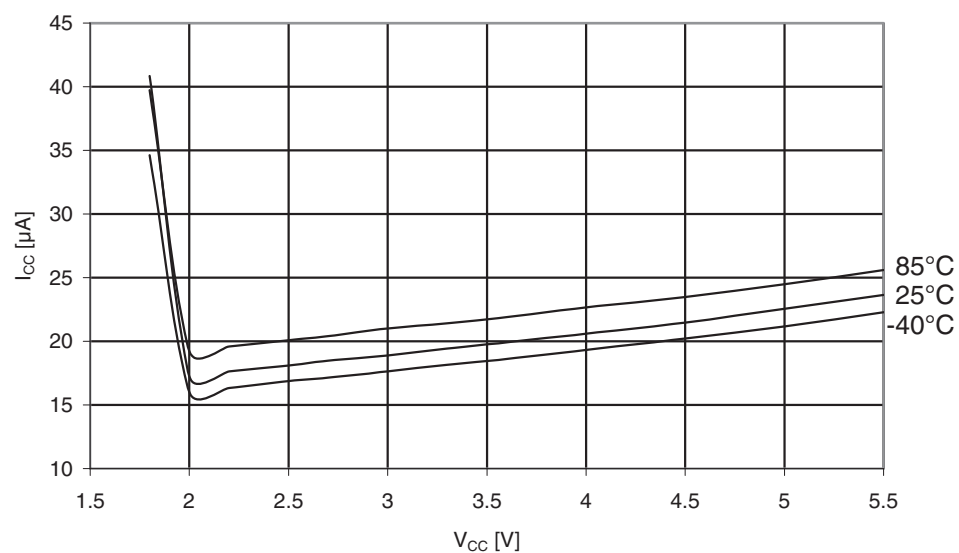
Figure 31-234. ATmega329PA: Brownout Detector current vs. V_{CC} .
