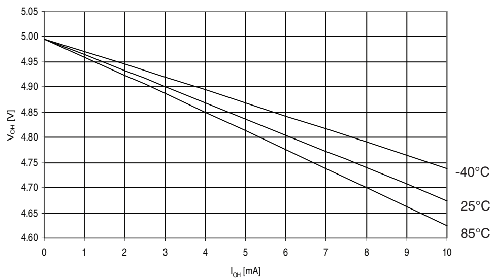
Figure 31-266. ATmega3290A: I/O pin output voltage vs. source current, ports A, C, D, E, F, G ( V_{CC} = 5V ).
