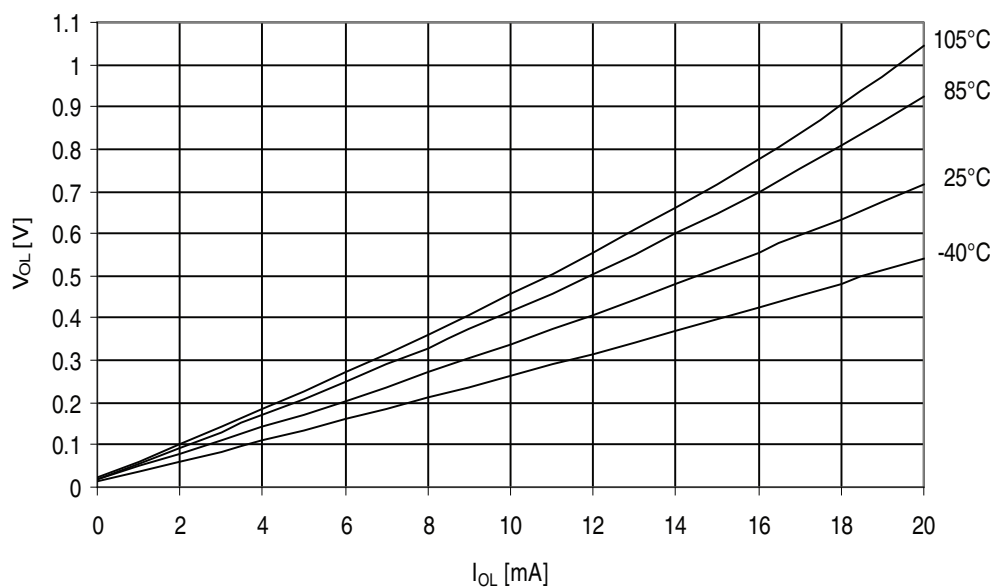
Figure 32-383. ATmega3290PA - 105°C: I/O Pin Output Voltage vs. Sink Current, Port B ( V_{CC} = 3V )
