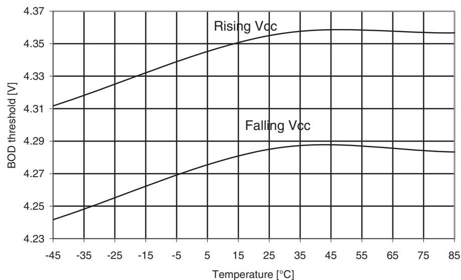
Figure 31-102. ATmega169PA: BOD Thresholds vs. temperature (BOD level is 4.3V).
