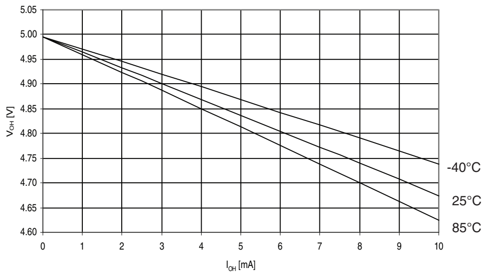
Figure 31-146. ATmega329A: I/O pin output voltage vs. source current, ports A, C, D, E, F, G ( V_{CC} = 5V ).
