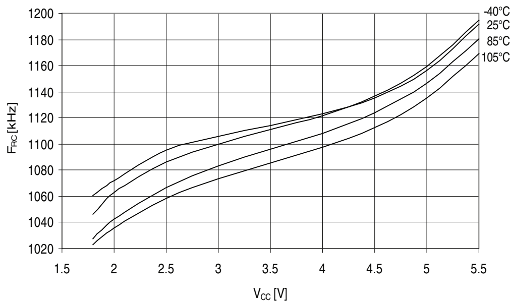
Figure 32-218. ATmega329PA - 105°C: Watchdog Oscillator Frequency vs. V_{CC}
