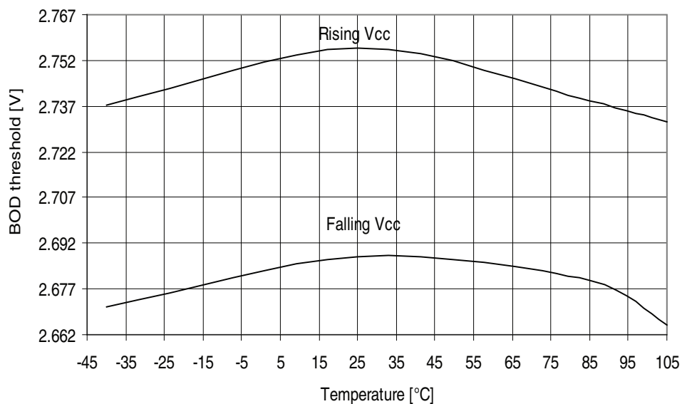
Figure 32-392. ATmega3290PA - 105°C: BOD Thresholds vs. Temperature (BOD Level is 2.7V)
