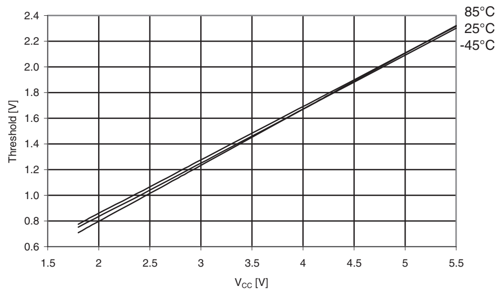
Figure 31-525. Atmel ATmega6490A: Reset input Threshold voltage vs. V_{CC} ( V_{IL} , reset pin read as “0”).
