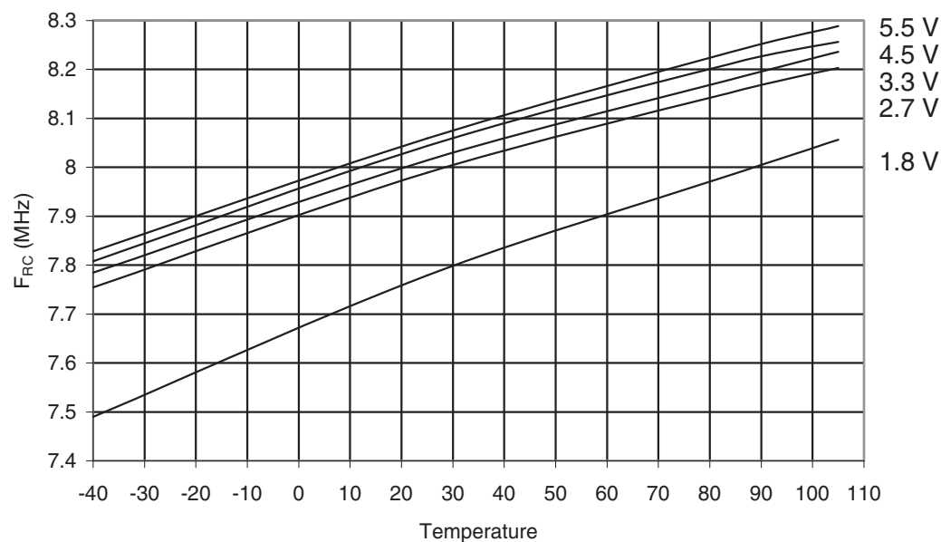
Figure 32-340. ATmega3290PA-105°C: Calibrated RC Oscillator Frequency vs. Temperature
