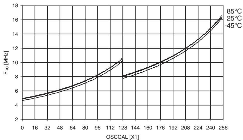
Figure 31-475. ATmega649P: Calibrated 8MHz RC oscillator frequency vs. Oscal value.
