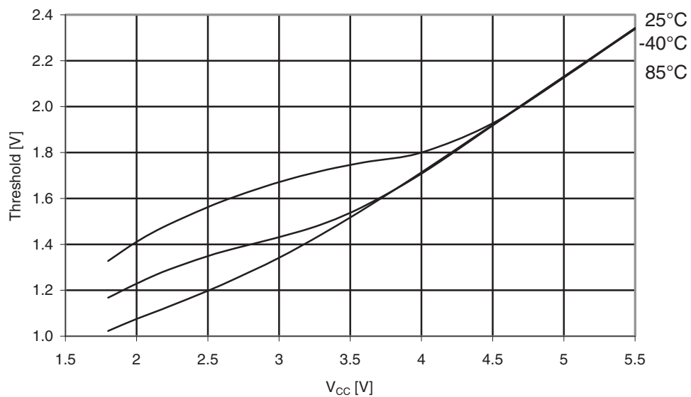
Figure 31-281. Atmel ATmega3290A: Reset Input Threshold voltage vs. V_{CC} ( V_{IH} , reset pin read as “1”).
