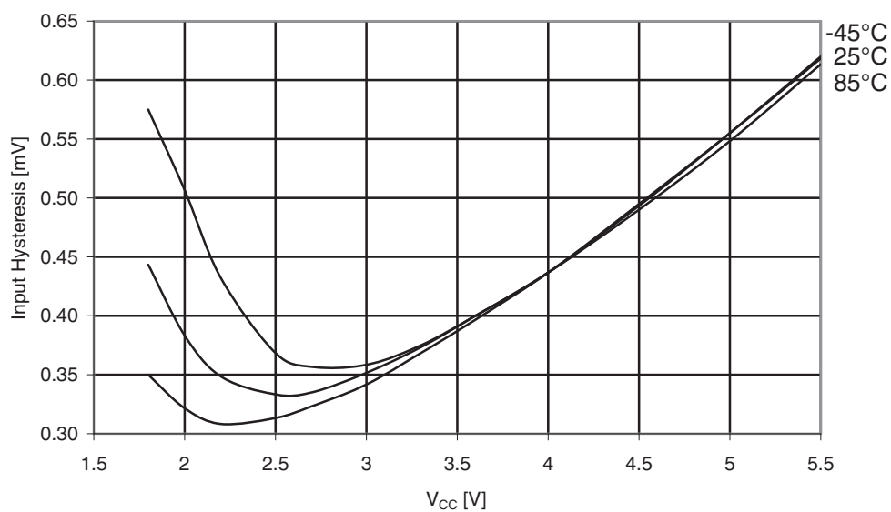
Figure 31-36. ATmega169A: I/O pin input Hysteresis vs. V_{CC} .
