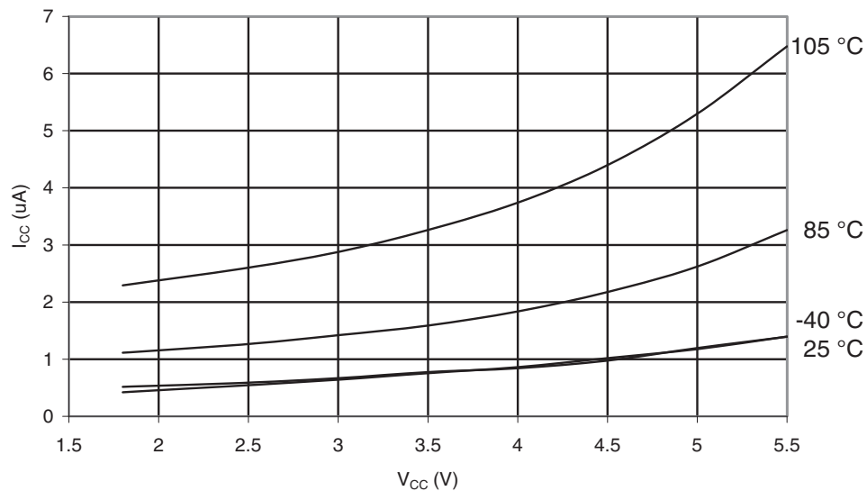
Figure 32-134. ATmega329P -105°C: Power-save Supply Current vs. V_{CC} (Watchdog Timer Disabled)
