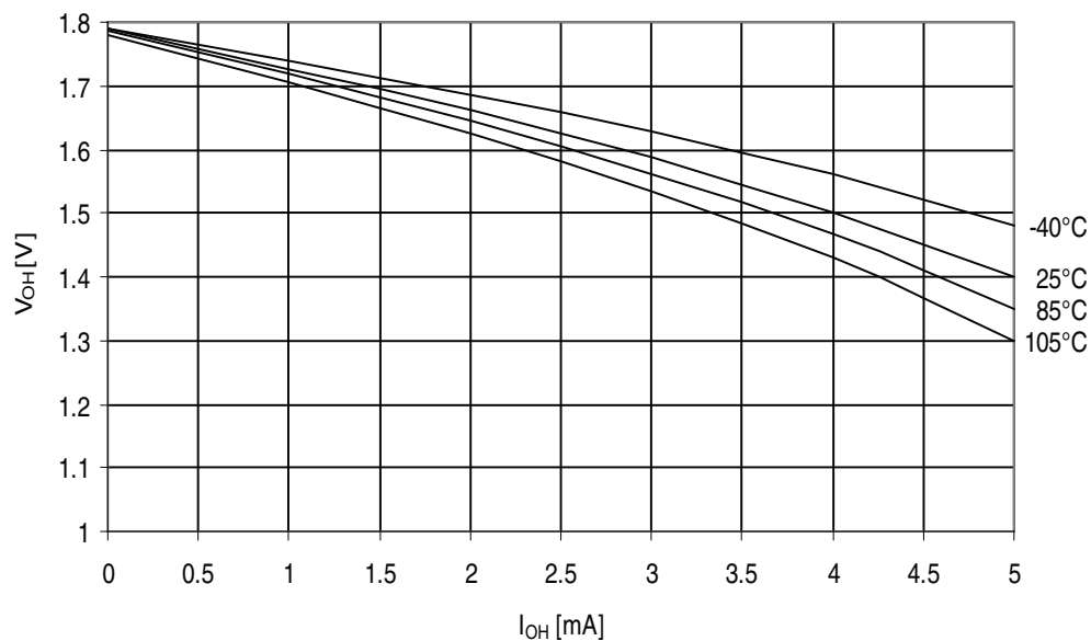
Figure 32-378. ATmega3290PA - 105°C: I/O Pin Output Voltage vs. Source Current, Port B ( V_{CC} = 1.8V )
