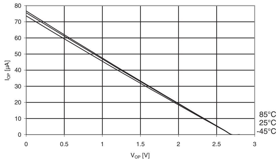
Figure 31-17. Atmel ATmega169A: I/O pin pull-up resistor current vs. input voltage ( V_{CC} = 2.7V ).
