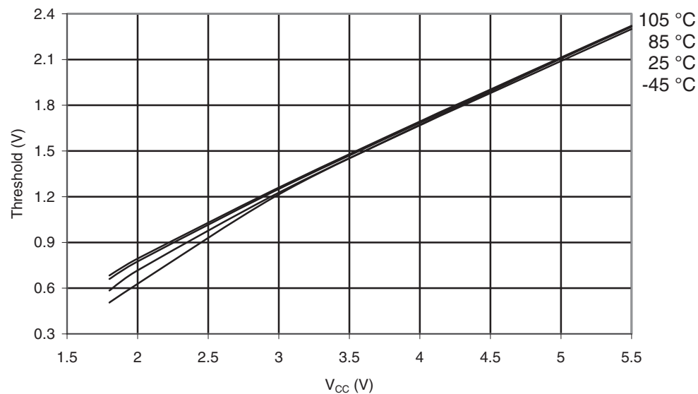
Figure 32-34. ATmega169PA-105°C: I/O Pin Input Threshold Voltage vs. V_{CC} ( V_{IL} , I/O Pin Read as “0”)
