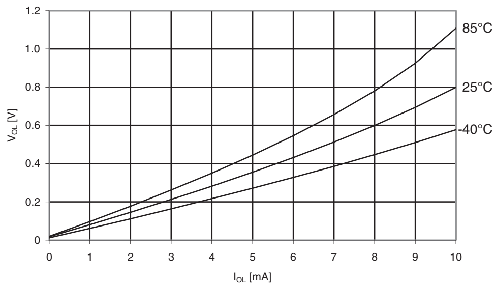
Figure 31-273. Atmel ATmega3290A. I/O pin output voltage vs. sink current, ports A, C, D, E, F, G ( V_{CC} = 2.7V ).
