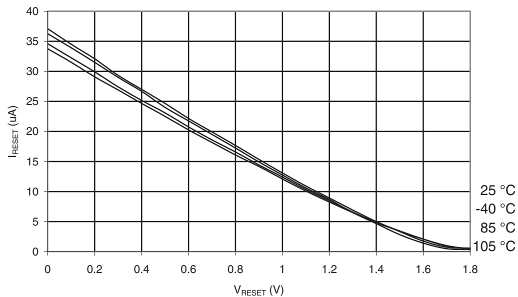
Figure 32-319. ATmega3290PA-105°C: Reset Pull-up Resistor Current vs. Reset Pin Voltage ( V_{CC} = 1.8V )
