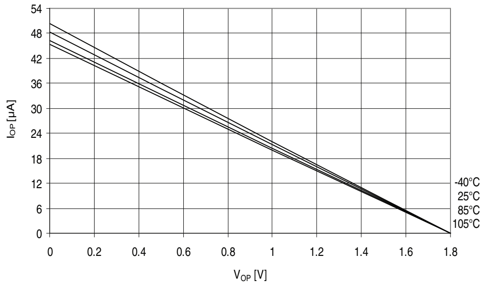
Figure 32-191. ATmega329PA - 105°C: Reset Pull-up Resistor Current vs. Reset Pin Voltage ( V_{CC} = 5V )
