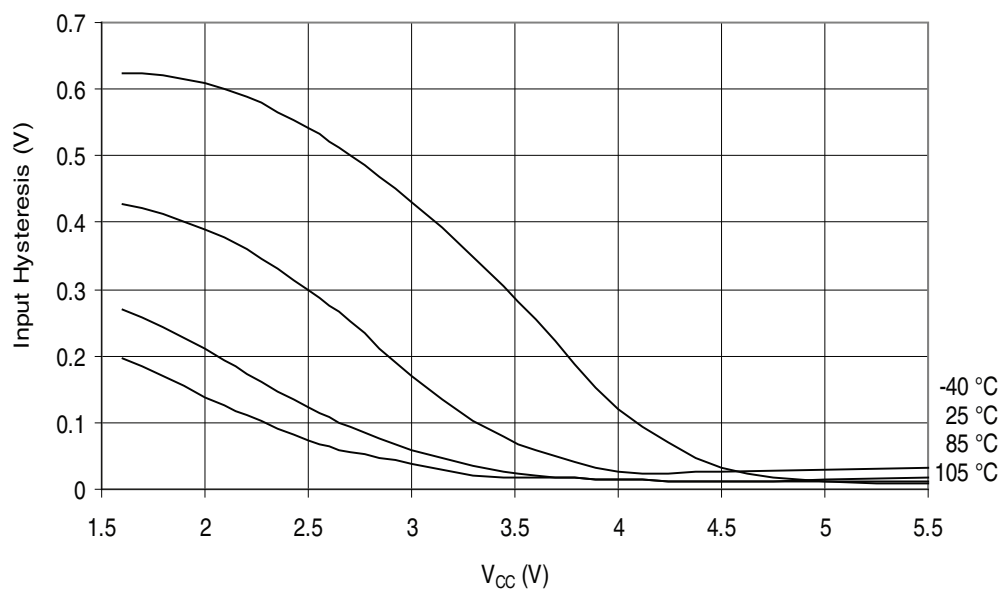
Figure 32-211. ATmega329PA - 105°C: Reset Input Pin Hysteresis vs. V_{CC}
