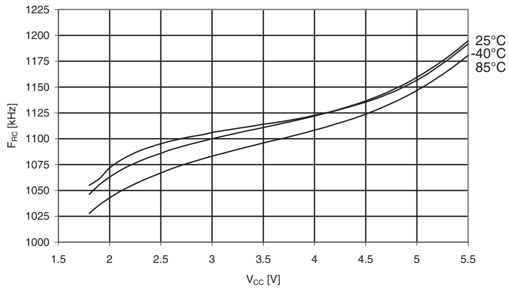
Figure 31-289. Atmel ATmega3290A: Watchdog Oscillator frequency vs. V_{CC} .
