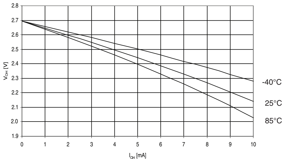
Figure 31-267. Atmel ATmega3290A: I/O pin output voltage vs. source current, ports A, C, D, E, F, G ( V_{CC} = 2.7V ).
