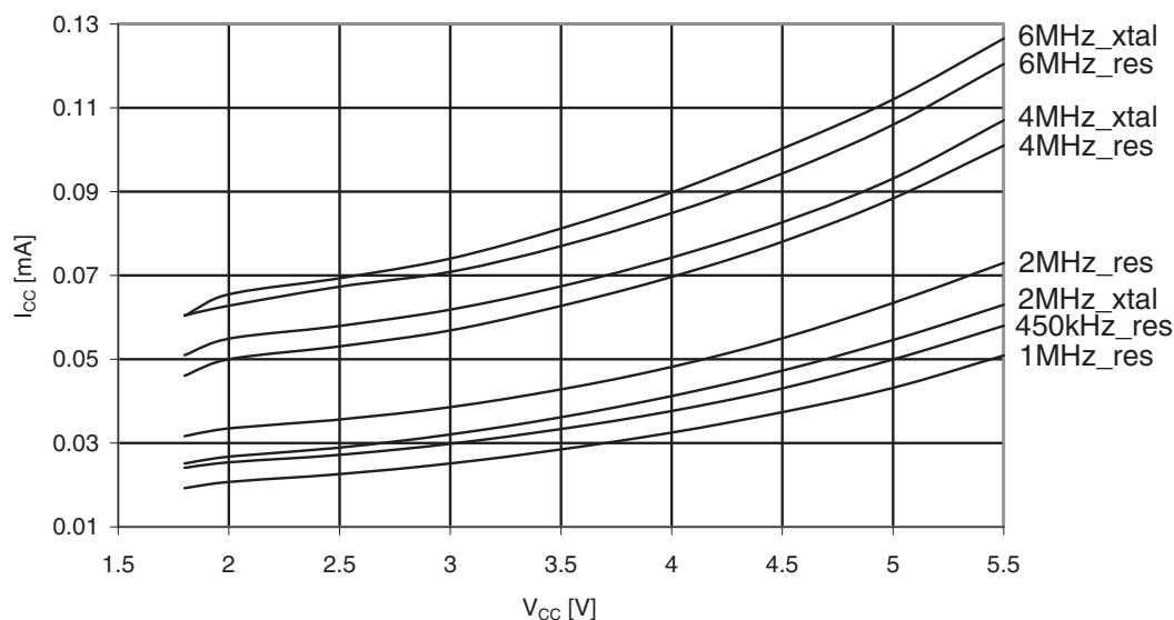
Figure 31-259. Atmel ATmega3290A: Standby supply current vs. V_{CC} (XTAL and resonator, Watchdog Timer disabled).
