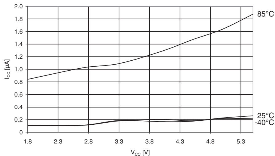
Figure 31-256. ATmega3290A: Power-down supply current vs. V_{CC} (Watchdog Timer enabled).
