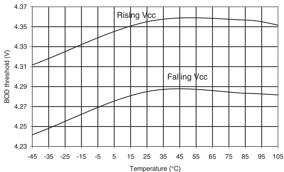
Figure 32-39. ATmega169PA-105°C: BOD Thresholds vs. Temperature (BOD Level is 4.3V)
