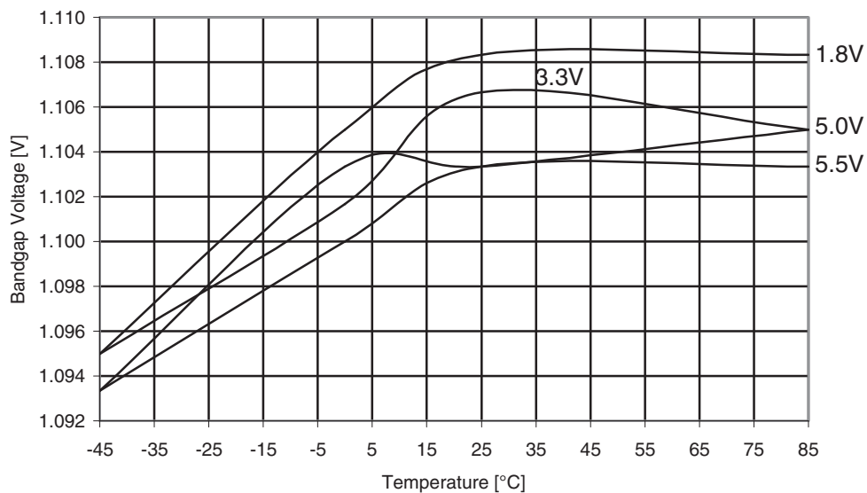
Figure 31-409. Atmel ATmega649A: Bandgap voltage vs. temperature.
