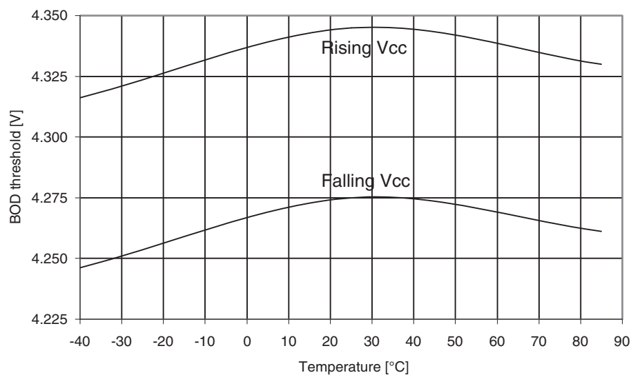
Figure 31-164. ATmega329A: BOD Thresholds vs. temperature (BOD level is 4.3V).
