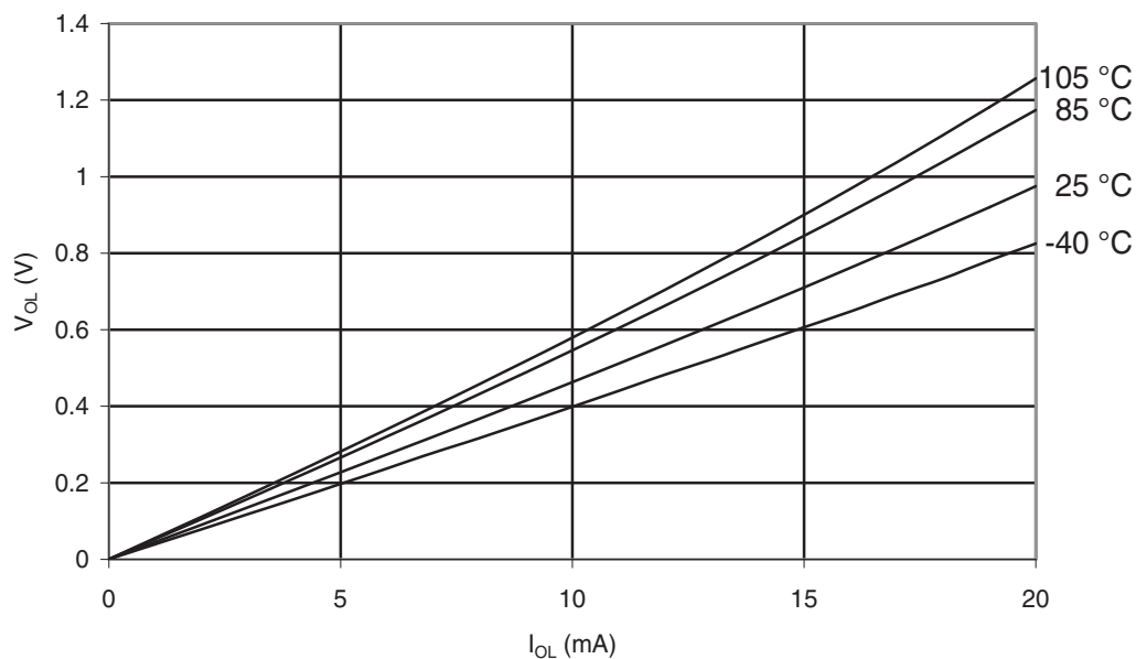
Figure 32-148. ATmega329P-105°C: I/O Pin Output Voltage vs. Sink Current, Port B ( V_{CC} = 5V )
