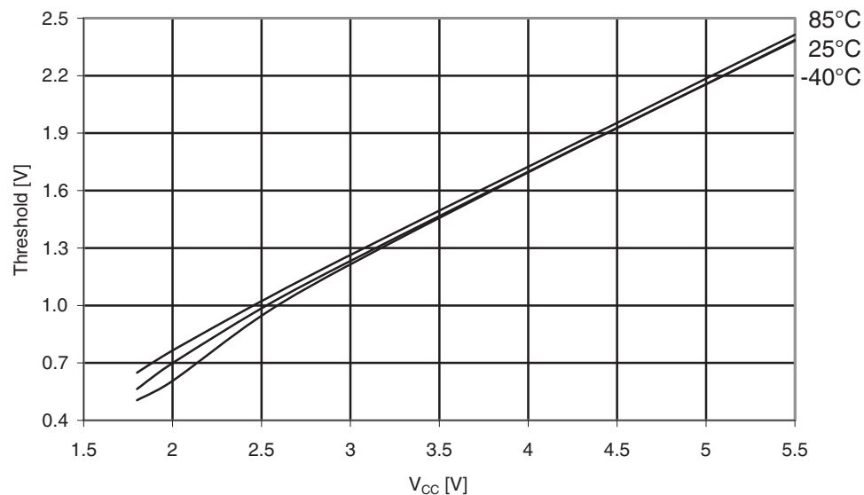
Figure 31-279. Atmel ATmega3290A: I/O pin Input Threshold voltage vs. V_{CC} ( V_{IL} , I/O pin read as “0”).
