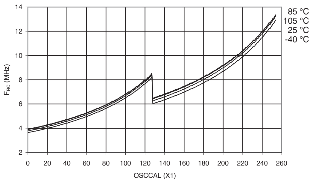
Figure 32-342. ATmega3290PA-105°C: Calibrated RC Oscillator Frequency vs. Oscal Value
