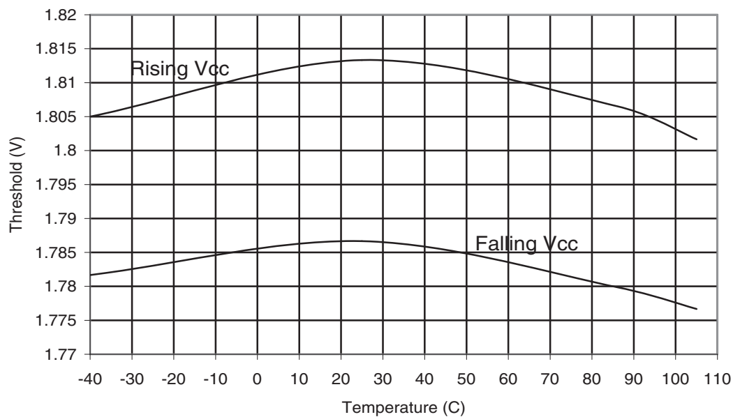
Figure 32-336. ATmega3290PA-105°C: BOD Thresholds vs. Temperature (BOD Level is 1.8V)
