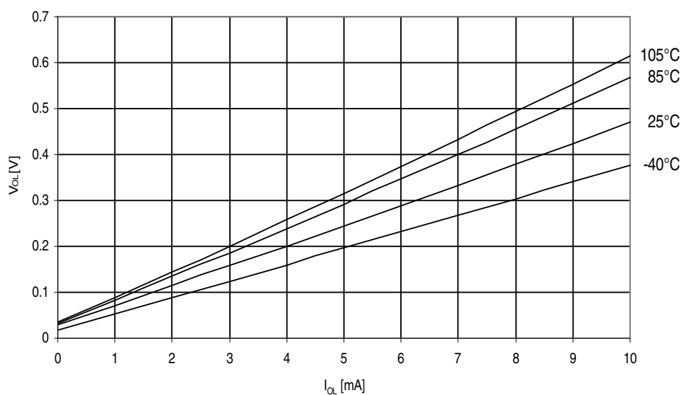
Figure 32-379. ATmega3290PA - 105°C: I/O Pin Output Voltage vs. Sink Current, Ports A, C, D, E, F, G ( V_{CC} = 5V )
