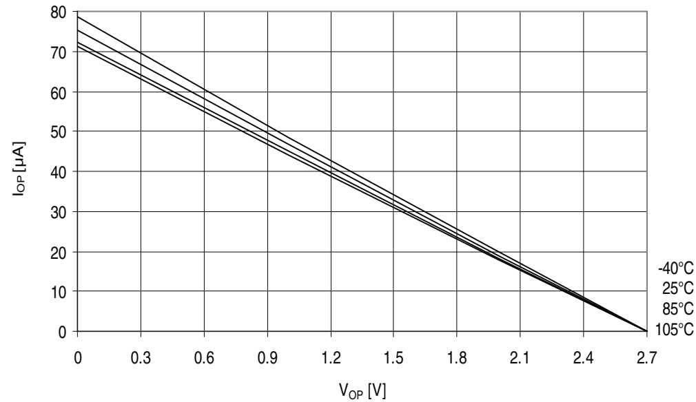
Figure 32-189. ATmega329PA - 105°C: I/O Pin Pull-up Resistor Current vs. Input Voltage ( V_{CC} = 2.7V )
