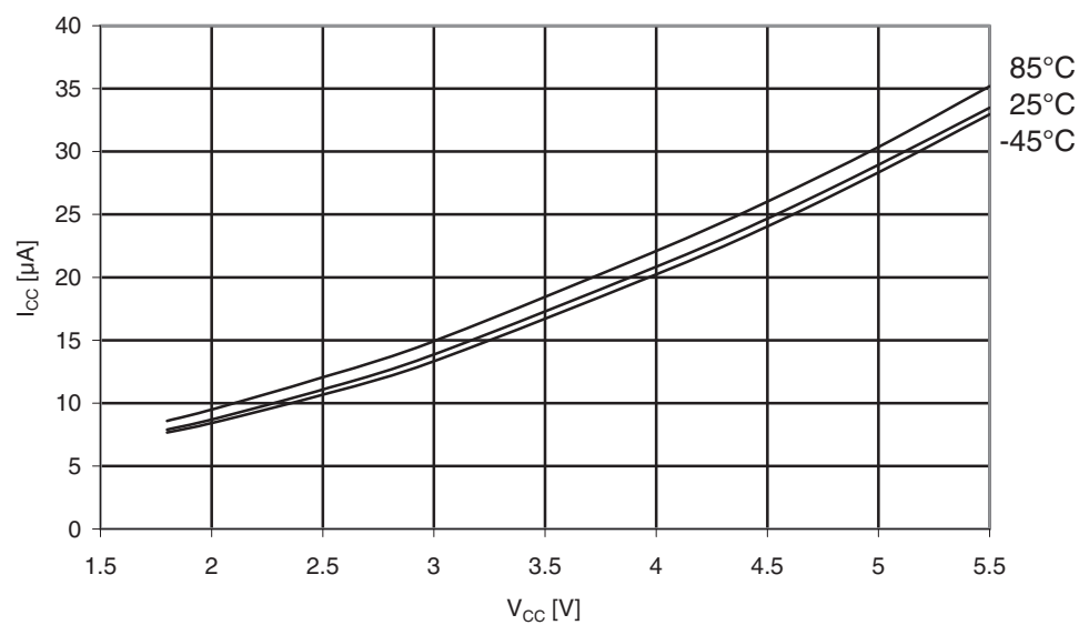
Figure 31-5. ATmega169A: Active supply current vs. V_{CC} (32kHz watch XTAL).
