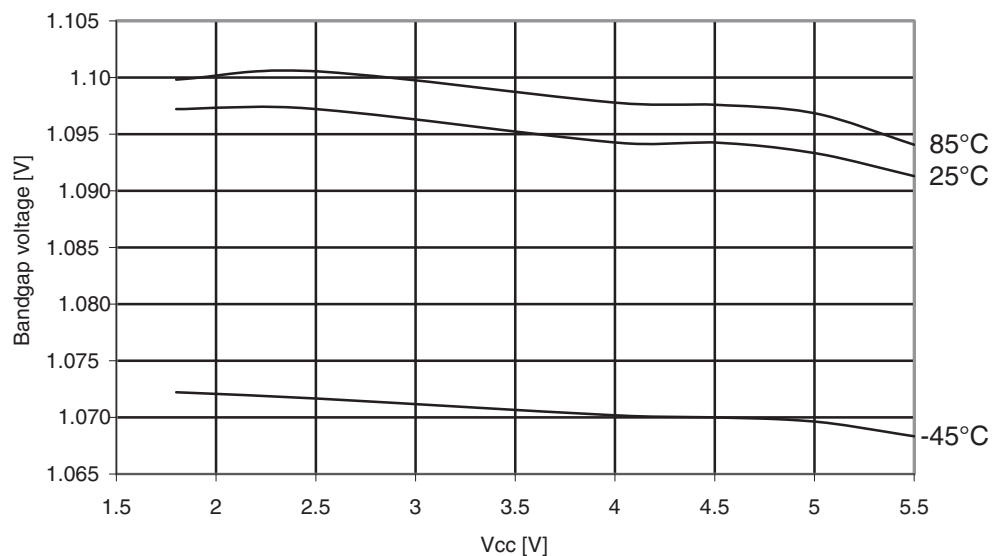
Figure 31-43. Atmel ATmega169A: Bandgap voltage vs. V_{CC} .
