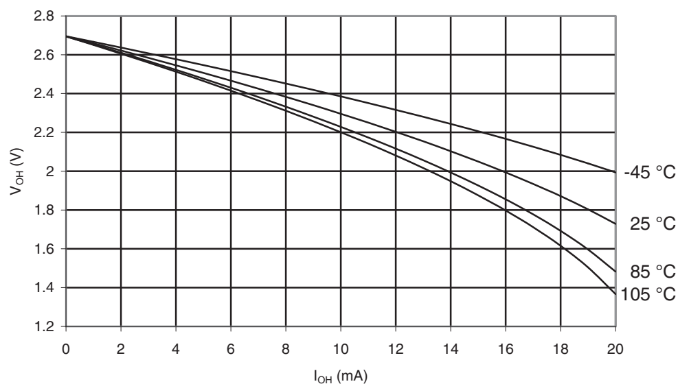
Figure 32-25. ATmega169PA-105°C: I/O Pin Output Voltage vs. Source Current, Port B ( V_{CC} = 2.7V )
