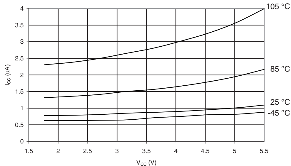
Figure 32-187. ATmega329PA - 105°C: Standby Supply Current vs. V_{CC} (32kHz Watch Crystal, Watchdog Timer Disabled)
