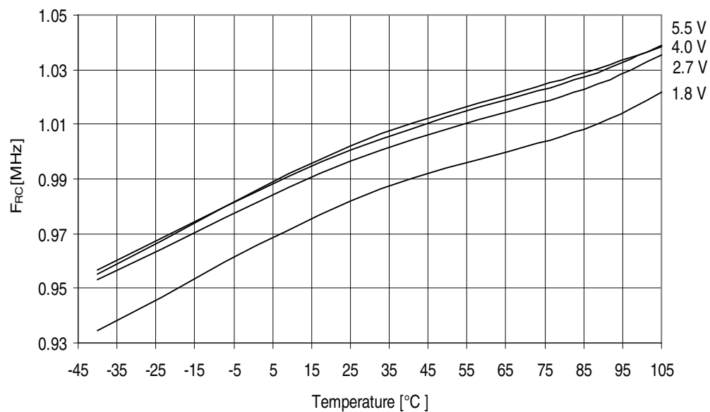
Figure 32-398. ATmega3290PA - 105°C: Calibrated 1MHz RC Oscillator Frequency vs. Temperature
