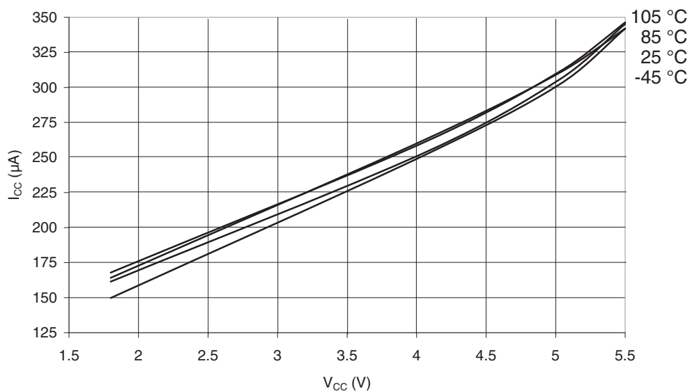
Figure 32-49. ATmega169PA-105°C: Active Supply Current with ADC at 50kHz vs. V_{CC}
