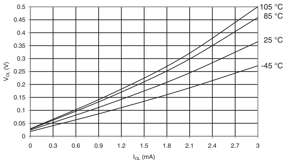
Figure 32-29. ATmega169PA-105°C: I/O Pin Output Voltage vs. Sink Current, Ports A, C, D, E, F, G ( V_{CC} = 1.8V )
