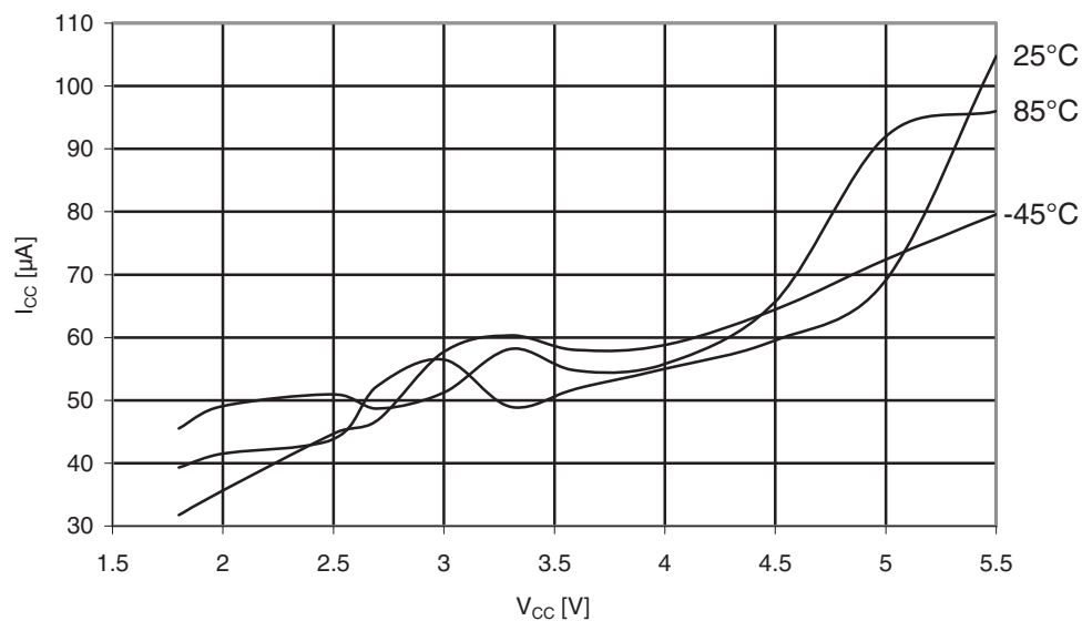
Figure 31-604. Atmel ATmega6490P: Analog Comparator current vs. V_{CC} .
