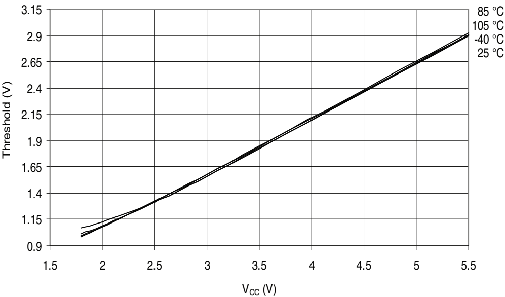
Figure 32-269. ATmega3290A - 105°C: I/O Pin Input Threshold Voltage vs. V_{CC} ( V_{IH} , I/O Pin Read as “1”)
