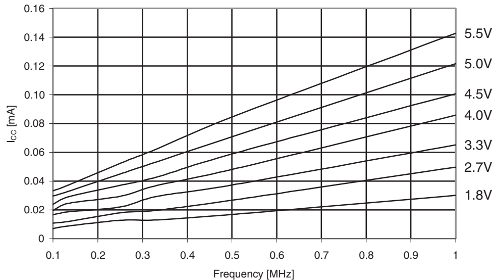
Figure 31-545. Atmel ATmega6490A: Reset supply current vs. V_{CC} (0.1 - 1.0MHz, excluding current through the reset pull-up).
