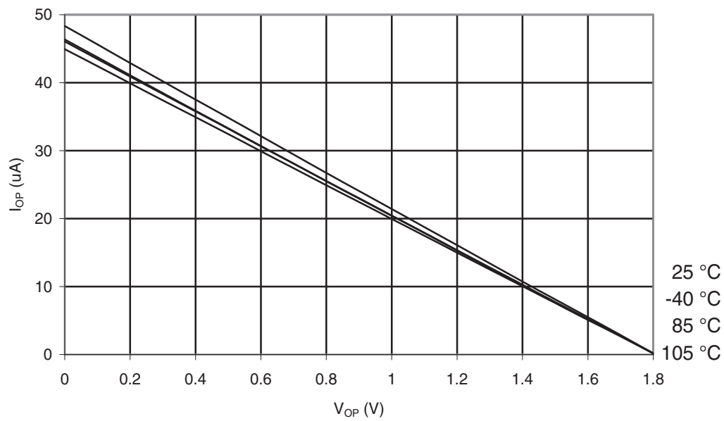
Figure 32-138. ATmega329P-105°C: I/O Pin Pull-up Resistor Current vs. Input Voltage ( V_{CC} = 1.8V )
