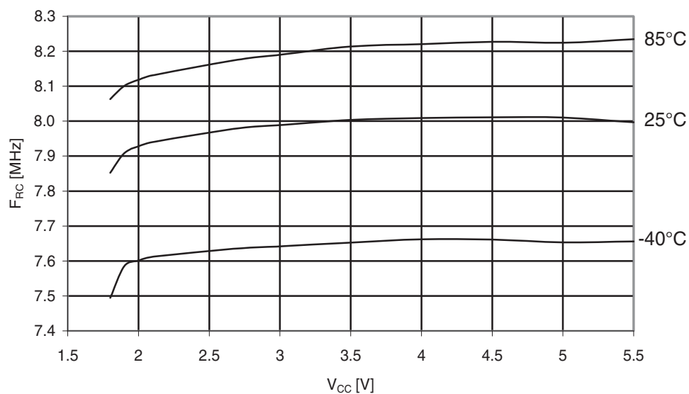
Figure 31-292. ATmega3290A: Calibrated 8MHz RC oscillator frequency vs. V_{CC} .
