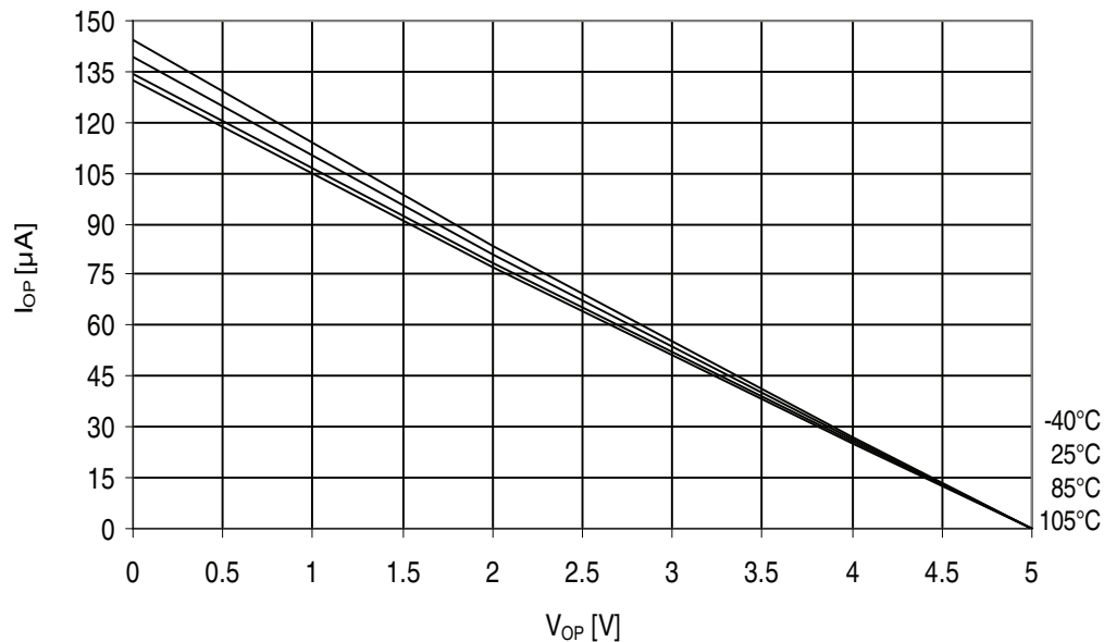
Figure 32-188. ATmega329PA - 105°C: I/O Pin Pull-up Resistor Current vs. Input Voltage ( V_{CC} = 5V )
