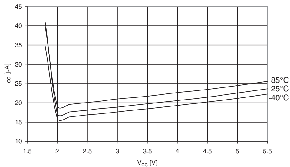
Figure 31-294. ATmega3290A: Brownout Detector current vs. V_{CC} .
