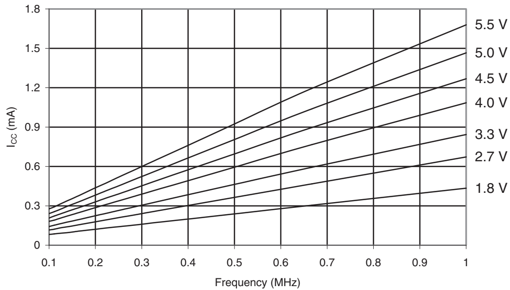
Figure 32-122. ATmega329P-105°C: Active Supply Current vs. Frequency (0.1 - 1.0 MHz)
