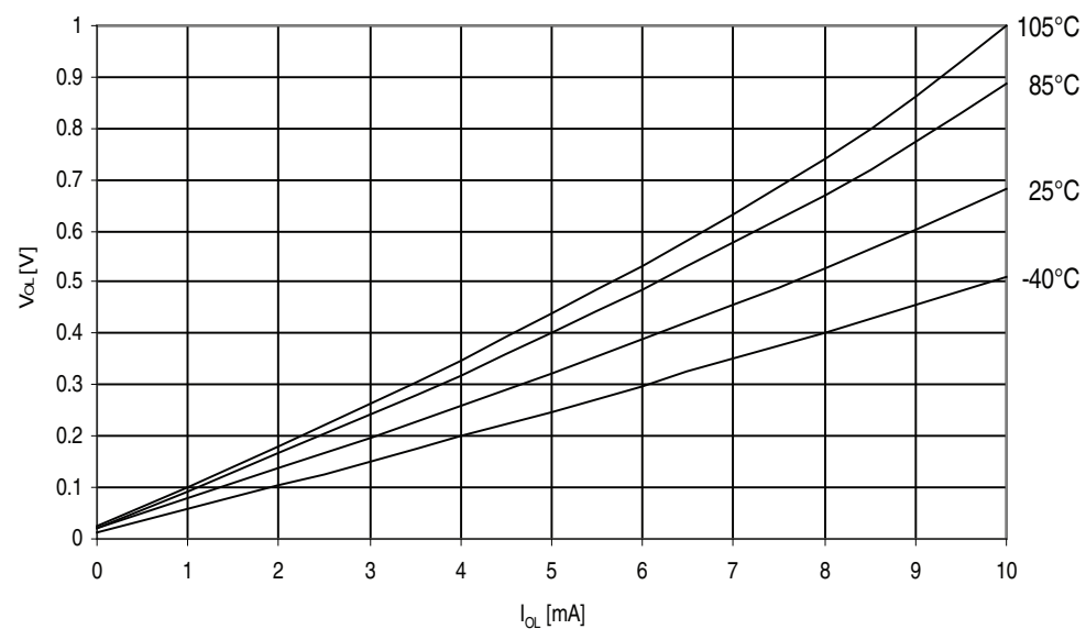
Figure 32-201. ATmega329PA - 105°C: I/O Pin Output Voltage vs. Sink Current, Ports A, C, D, E, F, G ( V_{CC} = 3V )
