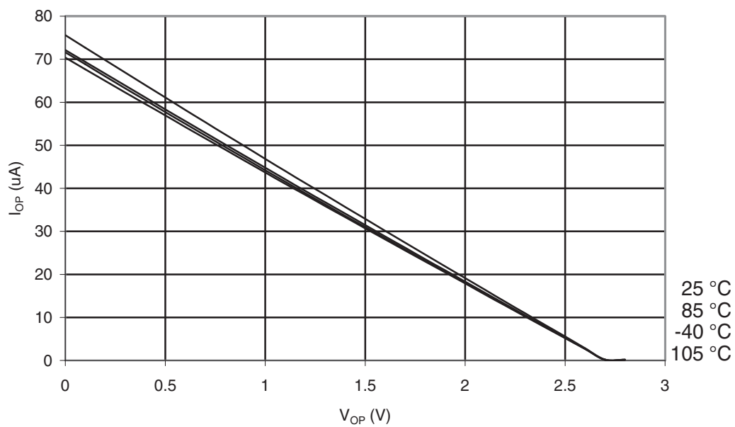
Figure 32-137. ATmega329P-105°C: I/O Pin Pull-up Resistor Current vs. Input Voltage ( V_{CC} = 2.7V )
