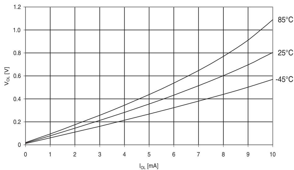
Figure 31-455. ATmega649P: I/O pin output voltage vs. sink current, ports A, C, D, E, F, G ( V_{CC} = 2.7V ).
