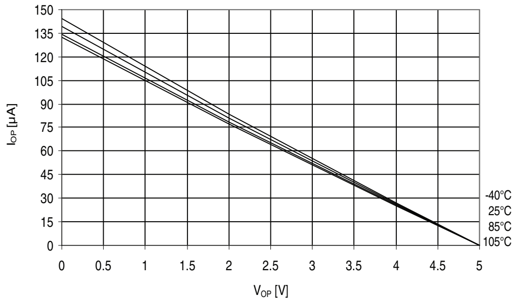
Figure 32-251. ATmega3290A - 105°C: I/O Pin Pull-up Resistor Current vs. Input Voltage ( V_{CC} = 5V )
