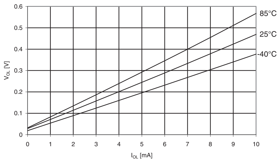
Figure 31-152. ATmega329A: I/O pin output voltage vs. sink current, ports A, C, D, E, F, G ( V_{CC} = 5V ).
