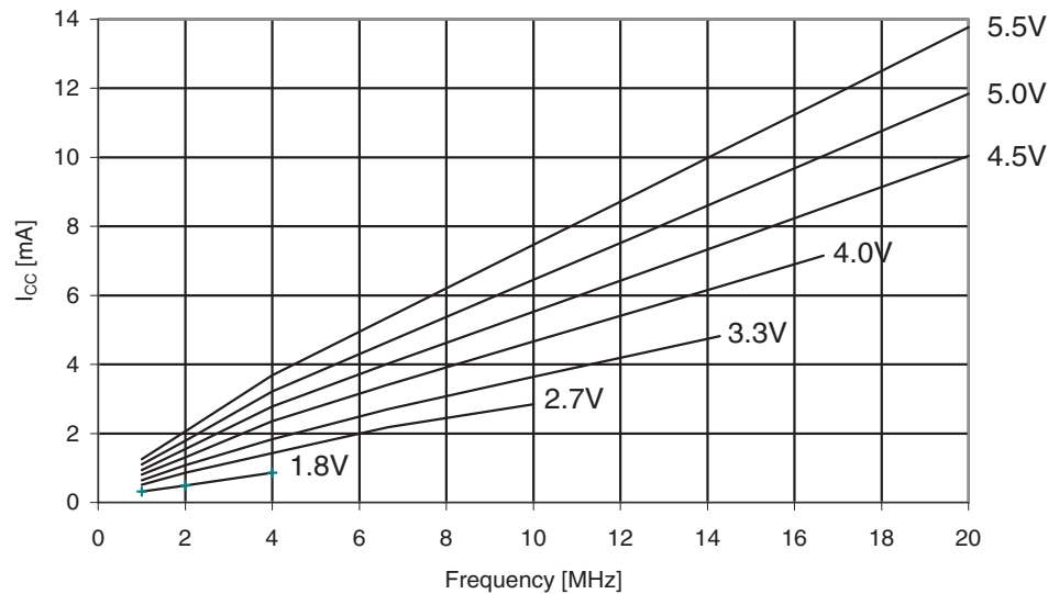
Figure 31-186. ATmega329PA: Active supply current vs. frequency (1 - 20MHz).
