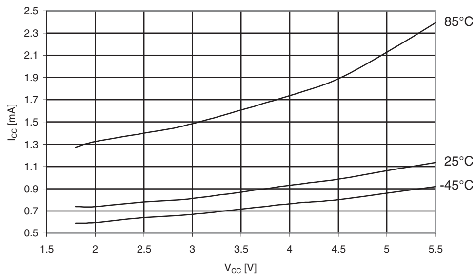
Figure 31-439. ATmega649P: Power-save supply current vs. V_{CC} (Watchdog Timer disabled and 32kHz XTAL oscillator running).
