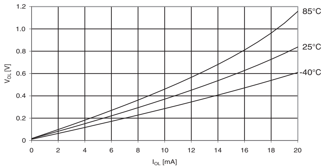
Figure 31-156. ATmega329A: I/O pin output voltage vs. sink current, port B ( V_{CC} = 2.7V ).
