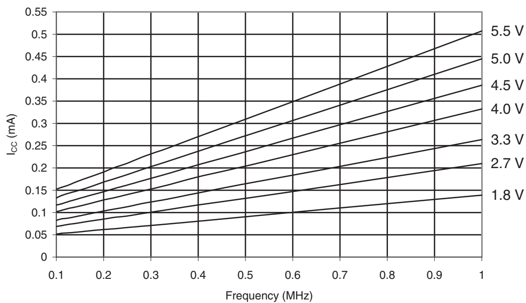
Figure 32-127. ATmega329P-105°C: Idle Supply Current vs. Frequency (0.1 - 1.0MHz)
