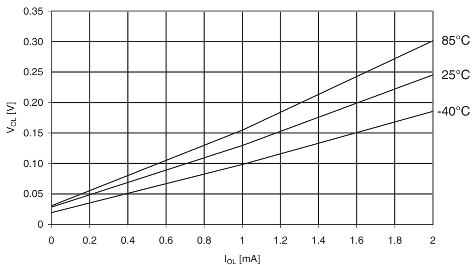
Figure 31-274. ATmega3290A: I/O pin output voltage vs. sink current, ports A, C, D, E, F, G ( V_{CC} = 1.8V ).
