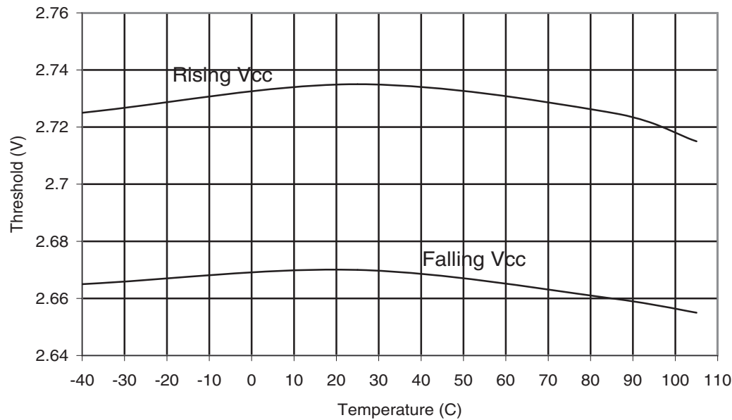
Figure 32-157. ATmega329P-105°C: BOD Thresholds vs. Temperature (BOD Level is 2.7V)
