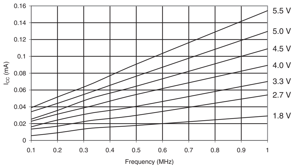
Figure 32-56. ATmega169PA-105°C: Reset Supply Current vs. V_{CC} (0.1 - 1.0 MHz, Excluding Current Through The Reset Pull-up)
