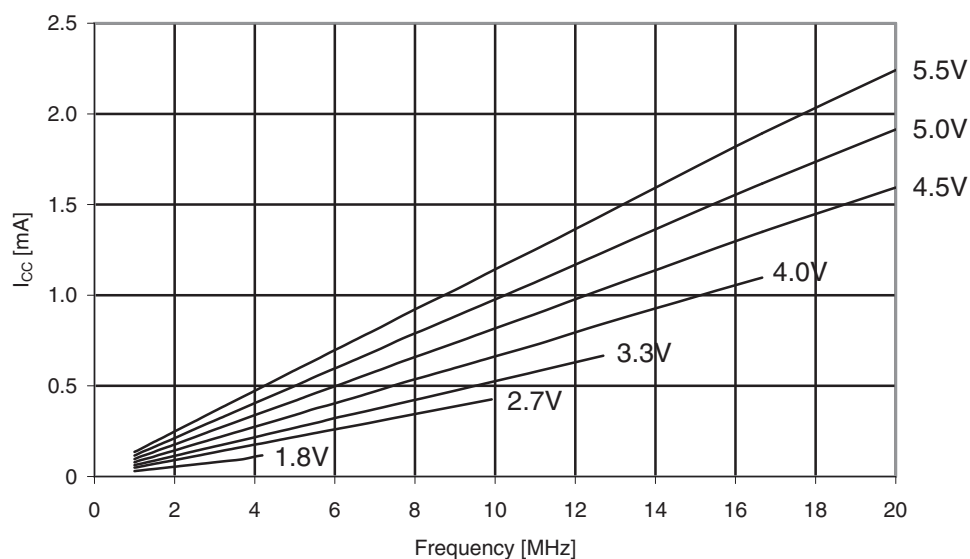
Figure 31-243. Atmel ATmega329PA: Reset supply current vs. V_{CC} (1 - 20MHz, excluding current through the reset pull-up).
