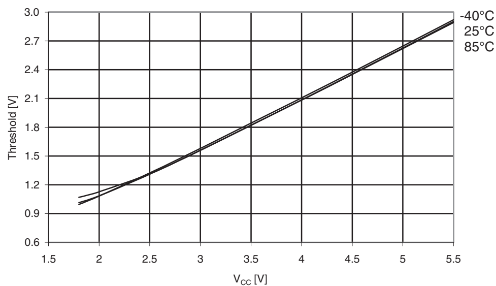
Figure 31-218. ATmega329PA: I/O pin Input Threshold voltage vs. V_{CC} ( V_{IH} , I/O pin read as "1").
