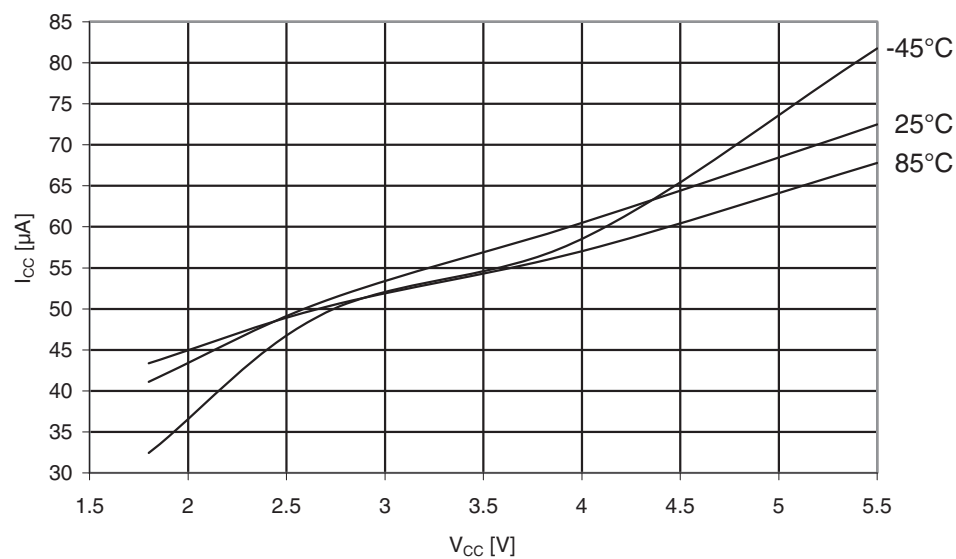
Figure 31-58. ATmega169A: Analog Comparator current vs. V_{CC} .
