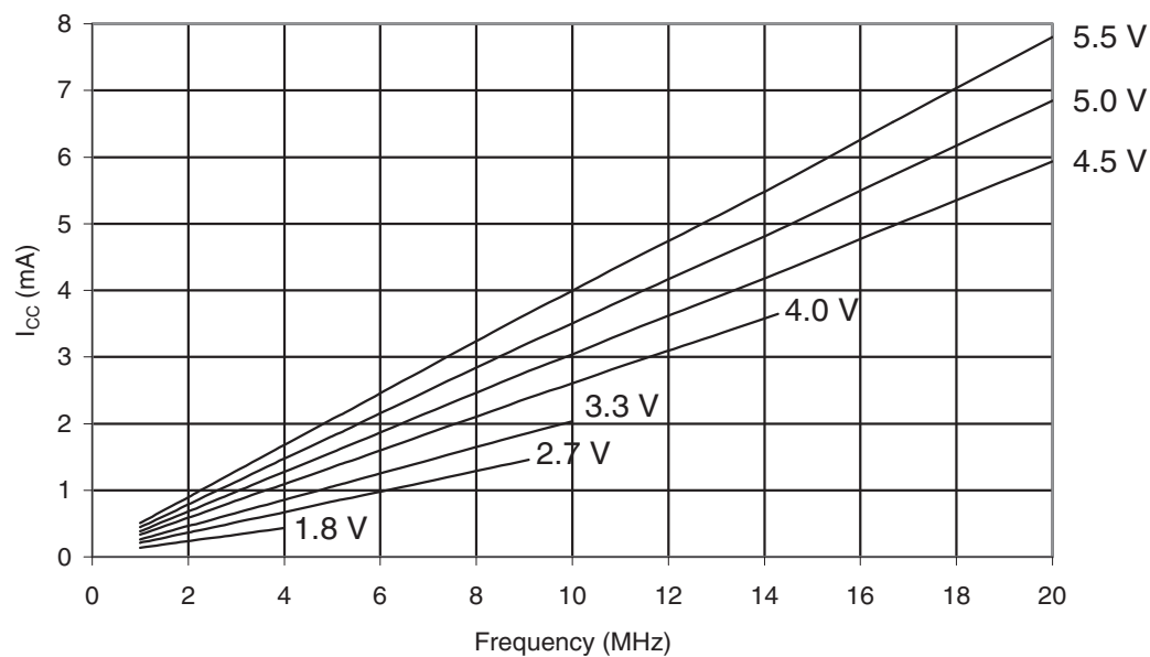
Figure 32-128. ATmega329P-105°C: Idle Supply Current vs. Frequency (1 - 20MHz)
