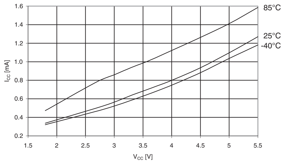
Figure 31-188. ATmega329PA: Active supply current vs. V_{CC} (Internal RC oscillator, 1MHz).
