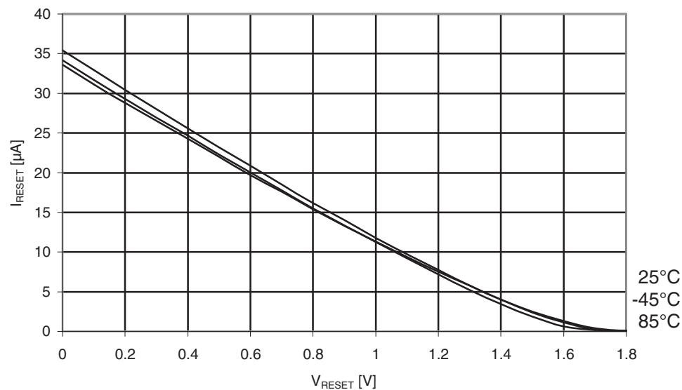
Figure 31-386. ATmega649A: Reset pull-up resistor current vs. reset pin voltage ( V_{CC} = 1.8V ).
