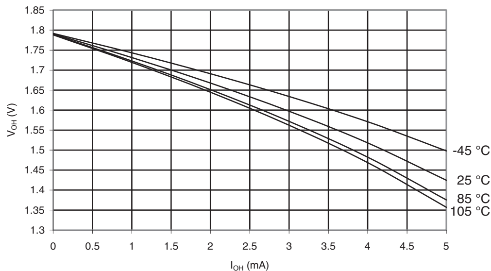
Figure 32-26. ATmega169PA-105°C: I/O Pin Output Voltage vs. Source Current, Port B ( V_{CC} = 1.8V )
