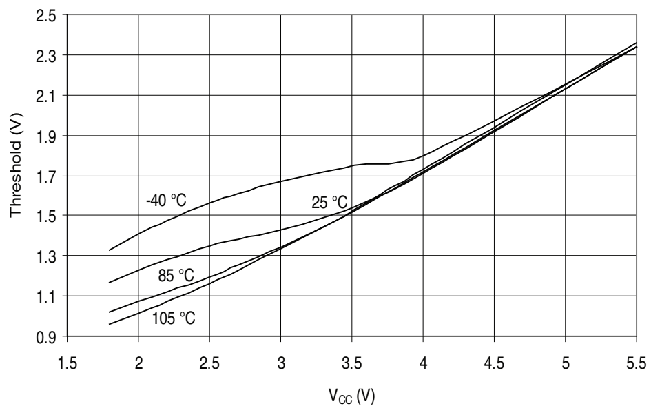
Figure 32-388. ATmega3290PA - 105°C: Reset Input Threshold Voltage vs. V_{CC} ( V_{IH} , Reset Pin Read as “1”)
