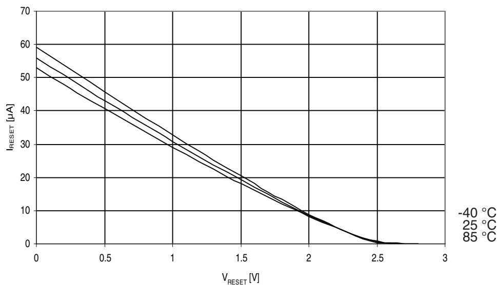
Figure 31-324. Atmel ATmega3290PA: Reset pull-up resistor current vs. reset pin voltage ( V_{CC} = 2.7V ).
