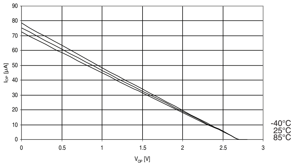
Figure 31-141. Atmel ATmega329A: I/O pin pull-up resistor current vs. input voltage ( V_{CC} = 2.7V ).
