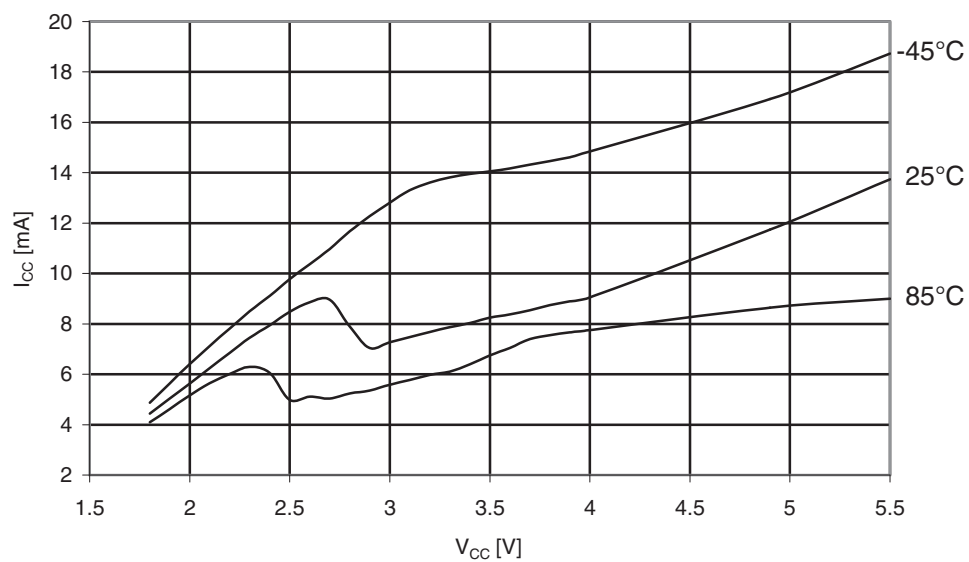
Figure 31-483. ATmega649P: Programming current vs. V_{CC} .
