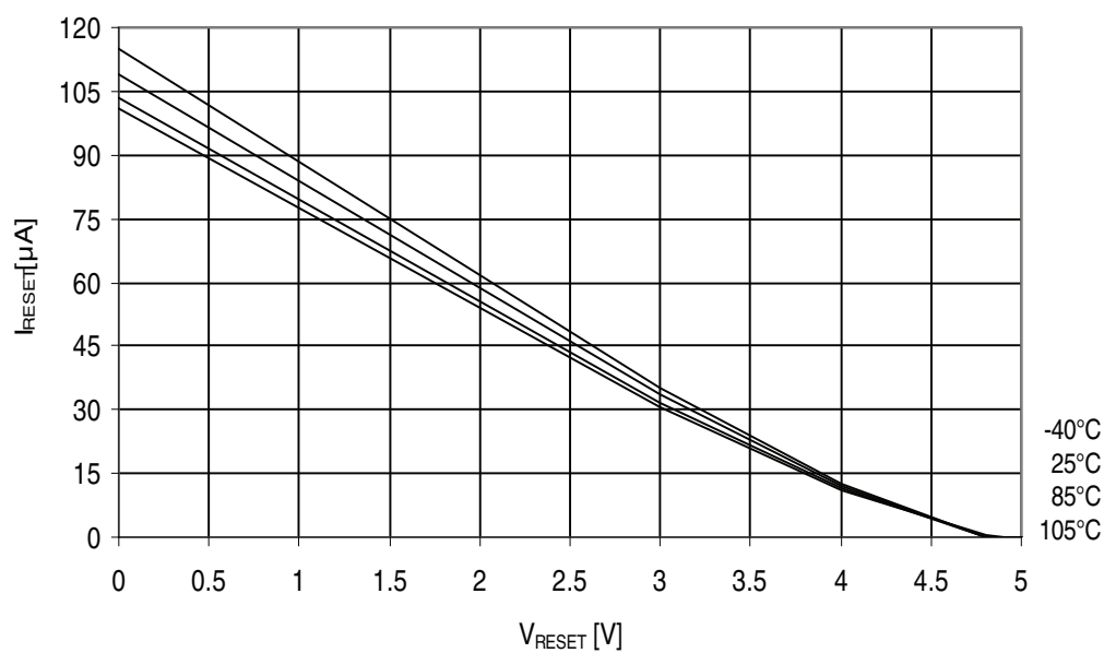
Figure 32-254. ATmega3290A - 105°C: Reset Pull-up Resistor Current vs. Reset Pin Voltage ( V_{CC} = 5V )
