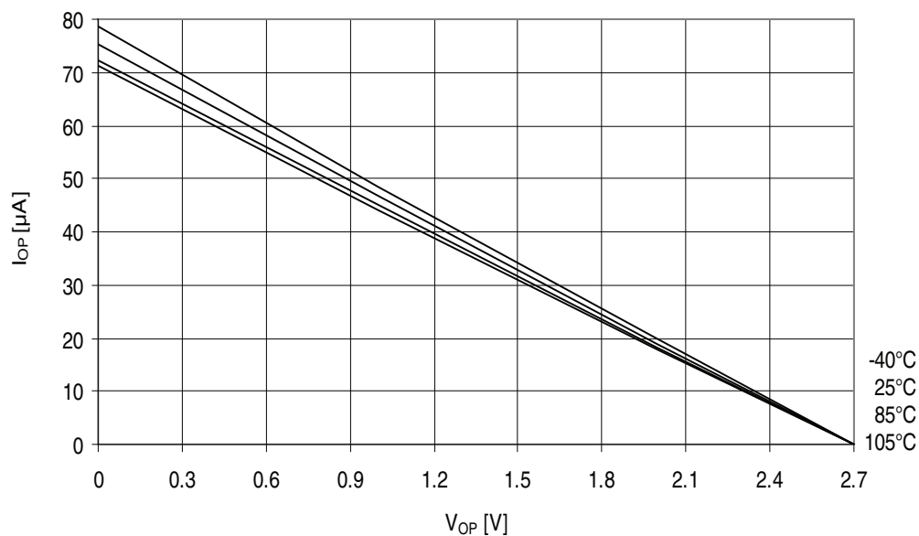
Figure 32-368. ATmega3290PA - 105°C: I/O Pin Pull-up Resistor Current vs. Input Voltage ( V_{CC} = 2.7V )
