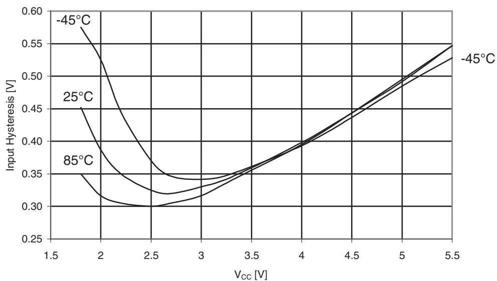
Figure 31-584. Atmel ATmega6490P: I/O pin input Hysteresis vs. V_{CC} .
