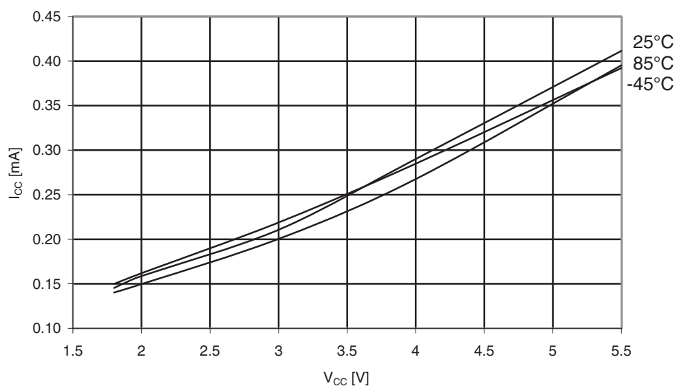
Figure 31-368. ATmega649A: Active supply current vs. V_{CC} (Internal RC oscillator, 1MHz).
