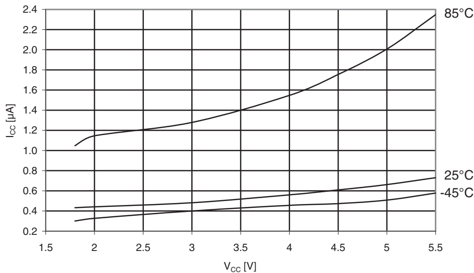
Figure 31-558. Atmel ATmega6490P: Power-down supply current vs. V_{CC} (Watchdog Timer disabled).
