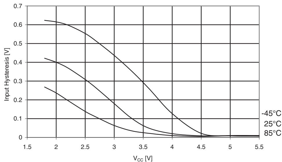
Figure 31-101. Atmel ATmega169PA: Reset input pin Hysteresis vs. V_{CC} .
