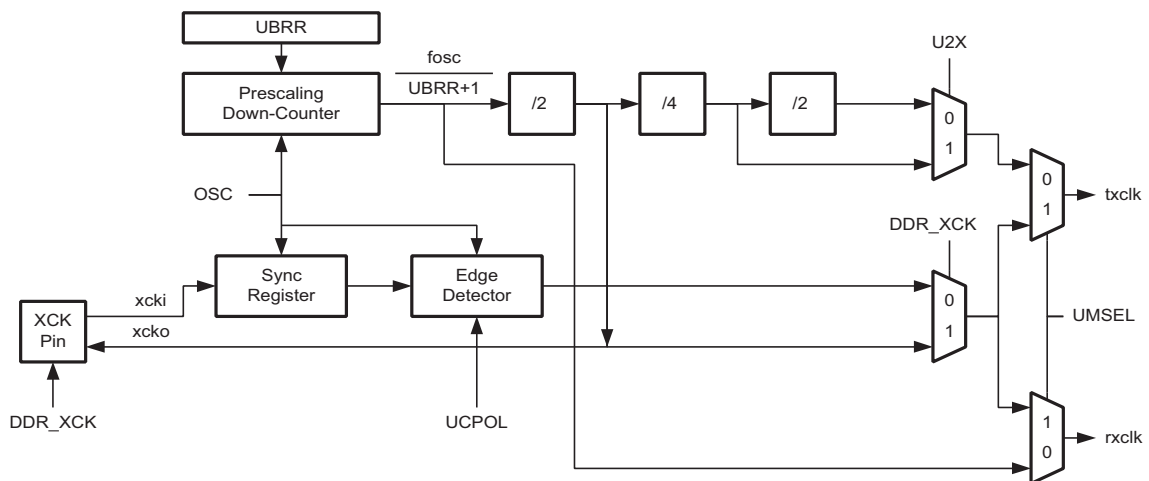
Figure 20-2. Clock Generation Logic, block diagram.
