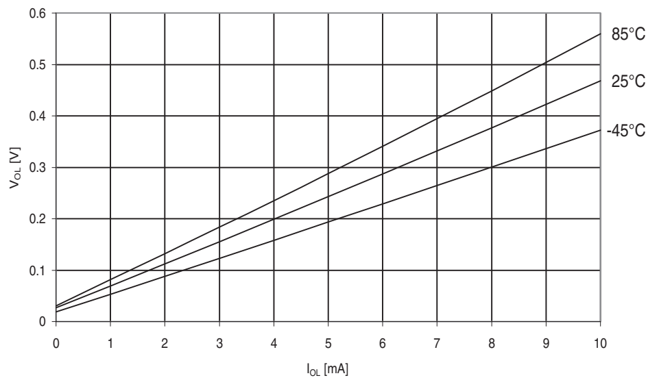
Figure 31-394. ATmega649A: I/O pin output voltage vs. sink current, ports A, C, D, E, F, G ( V_{CC} = 2.7V ).
