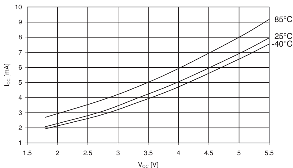
Figure 31-194. ATmega329PA: Idle supply current vs. V_{CC} (32kHz watch XTAL).
