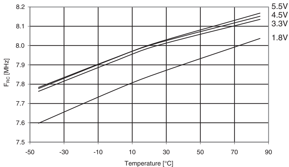
Figure 31-49. Atmel ATmega169A: Calibrated 8MHz RC oscillator frequency vs. temperature.
