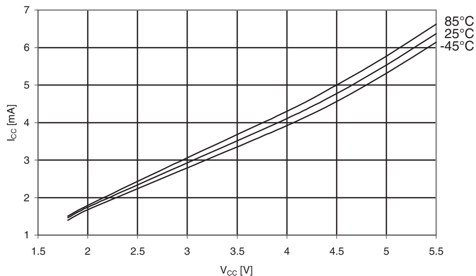
Figure 31-428. Atmel ATmega649P: Active supply current vs. V_{CC} (Internal RC oscillator, 8MHz).
