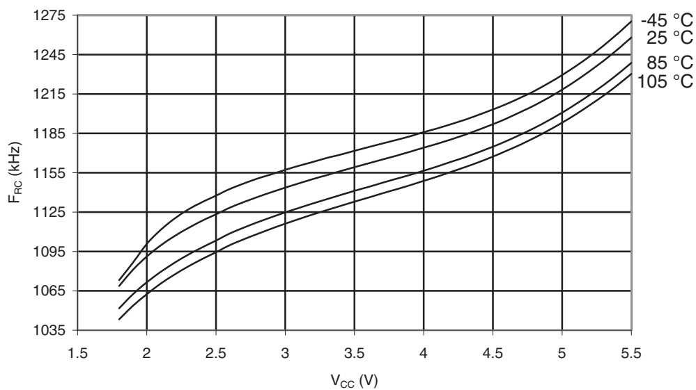
Figure 32-44. ATmega169PA-105°C: Watchdog Oscillator Frequency vs. V_{CC}
