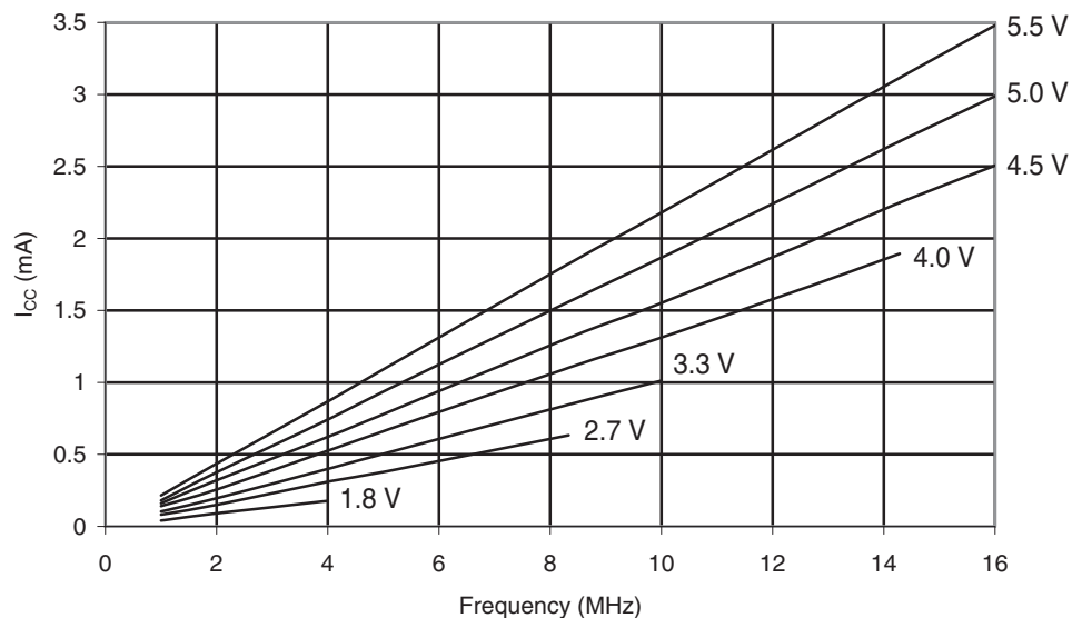
Figure 32-7. ATmega169PA-105°C: Idle Supply Current vs. Frequency (1 - 16MHz)
