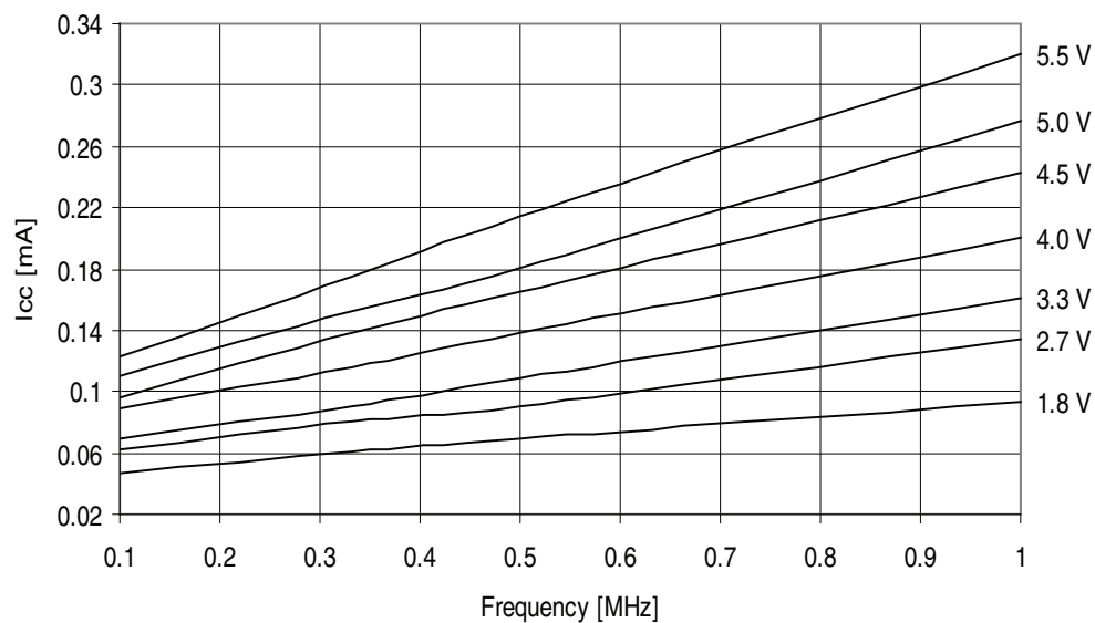
Figure 32-242. ATmega3290A - 105°C: Idle Supply Current vs. Frequency (0.1 - 1.0MHz)
