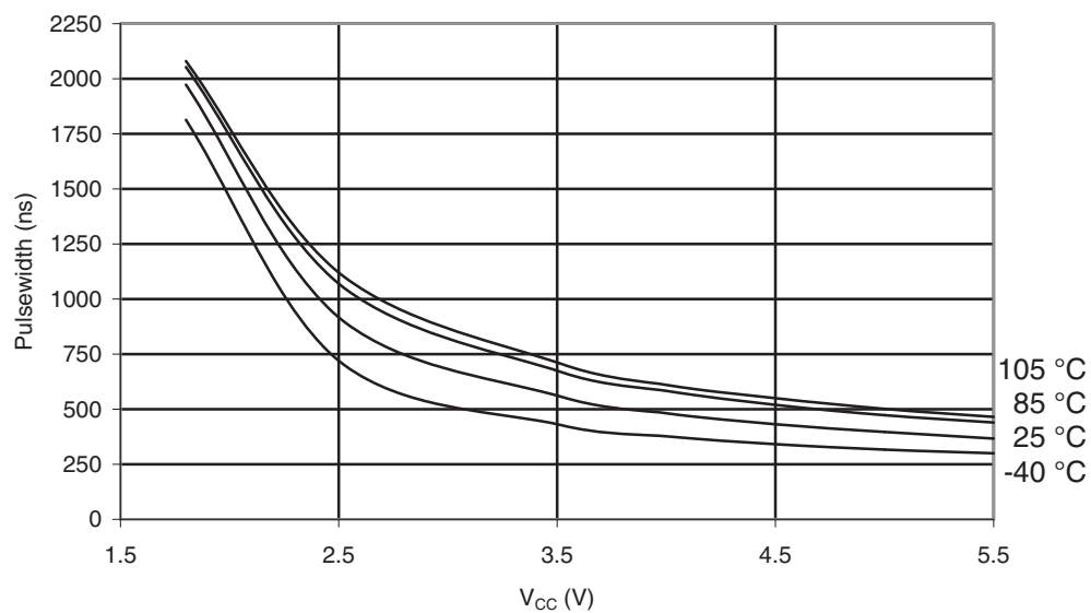
Figure 32-351. ATmega3290PA-105°C: Minimum Reset Pulse Width vs. V_{CC}
