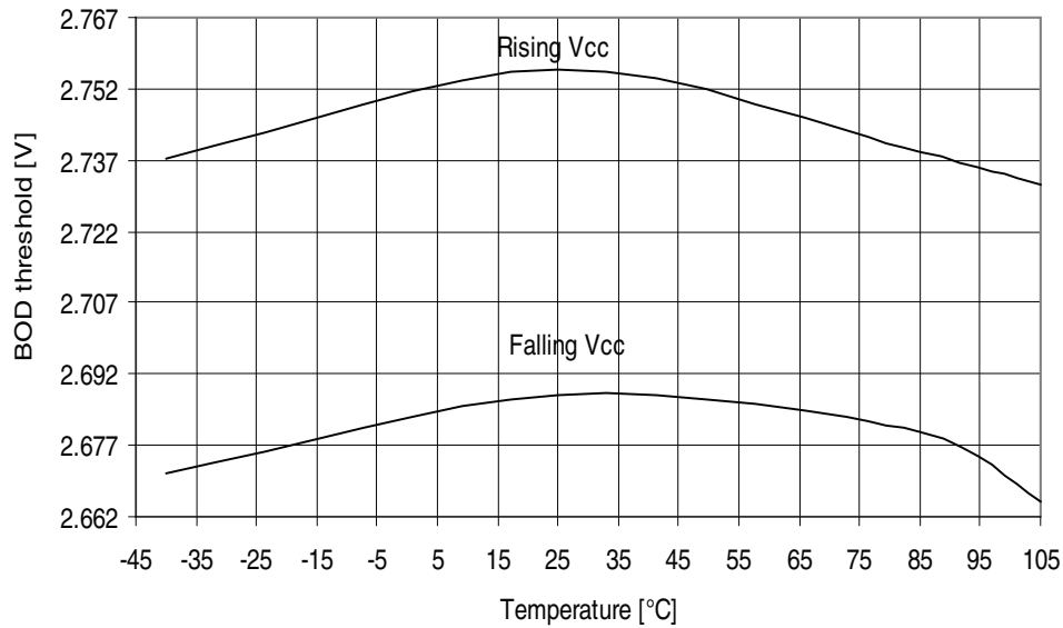
Figure 32-98. ATmega329A - 105°C: BOD Thresholds vs. Temperature (BOD Level is 2.7V)
