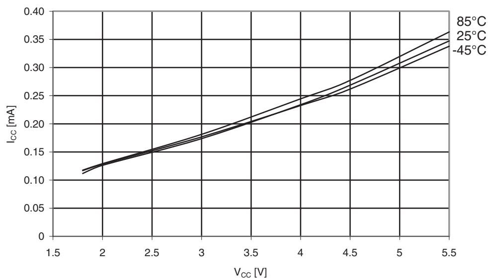
Figure 31-9. ATmega169A: Idle supply current vs. V_{CC} (Internal RC oscillator, 1MHz).
