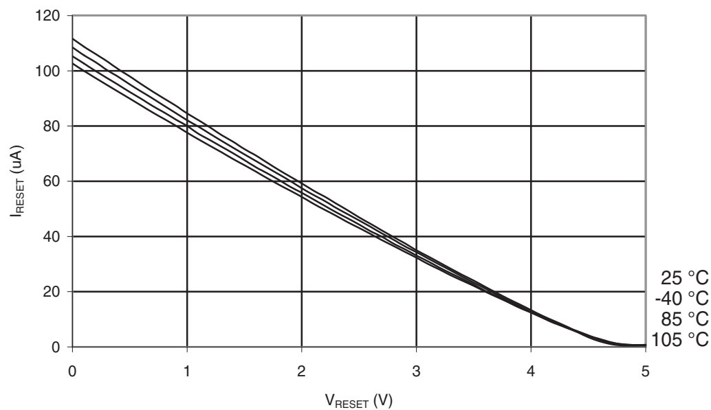
Figure 32-317. ATmega3290PA-105°C: Reset Pull-up Resistor Current vs. Reset Pin Voltage ( V_{CC} = 5V )
