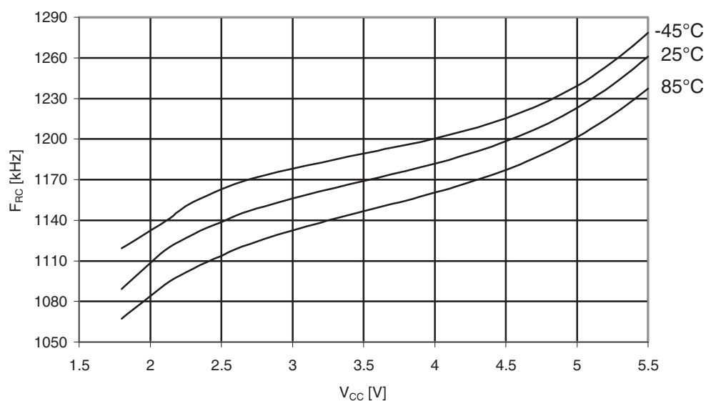
Figure 31-410. ATmega649A: Watchdog Oscillator frequency vs. V_{CC} .
