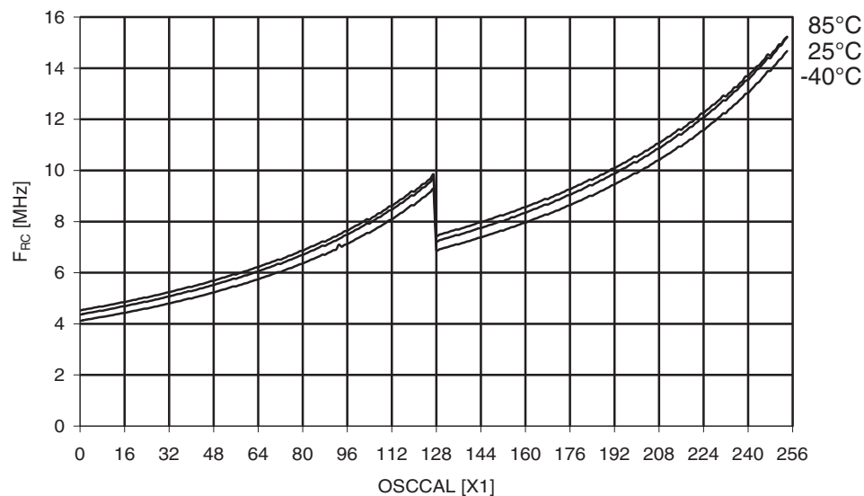
Figure 31-293. Atmel ATmega3290A: Calibrated 8MHz RC oscillator frequency vs. Oscscal value.
