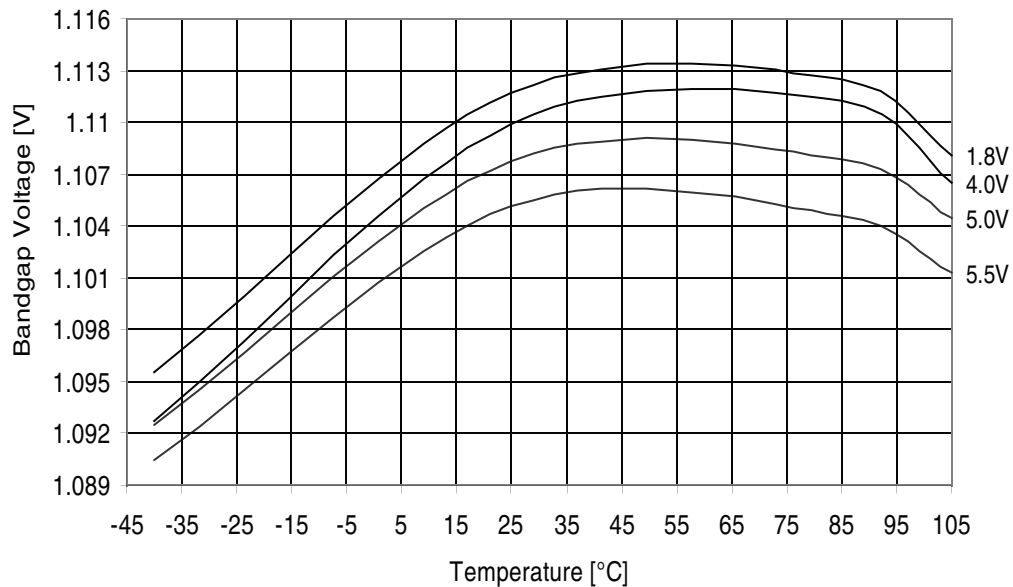
Figure 32-216. ATmega329PA - 105°C: Bandgap Voltage vs. Temperature
