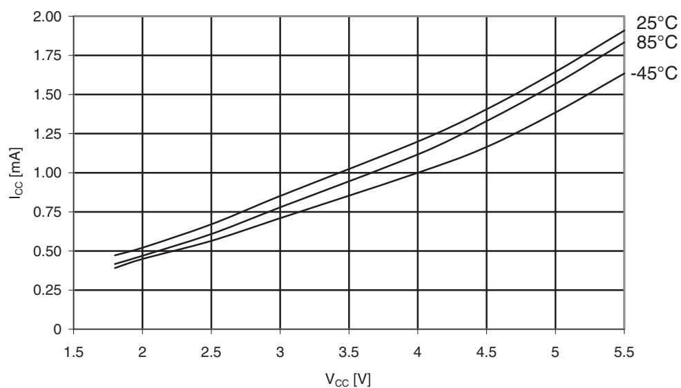
Figure 31-8. Atmel ATmega169A: Idle supply current vs. V_{CC} (Internal RC oscillator, 8MHz).
