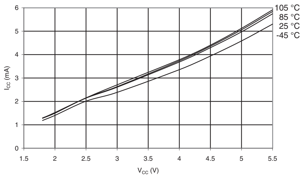
Figure 32-3. ATmega169PA-105°C: Active Supply Current vs. V_{CC} (Internal RC Oscillator, 8MHz)
