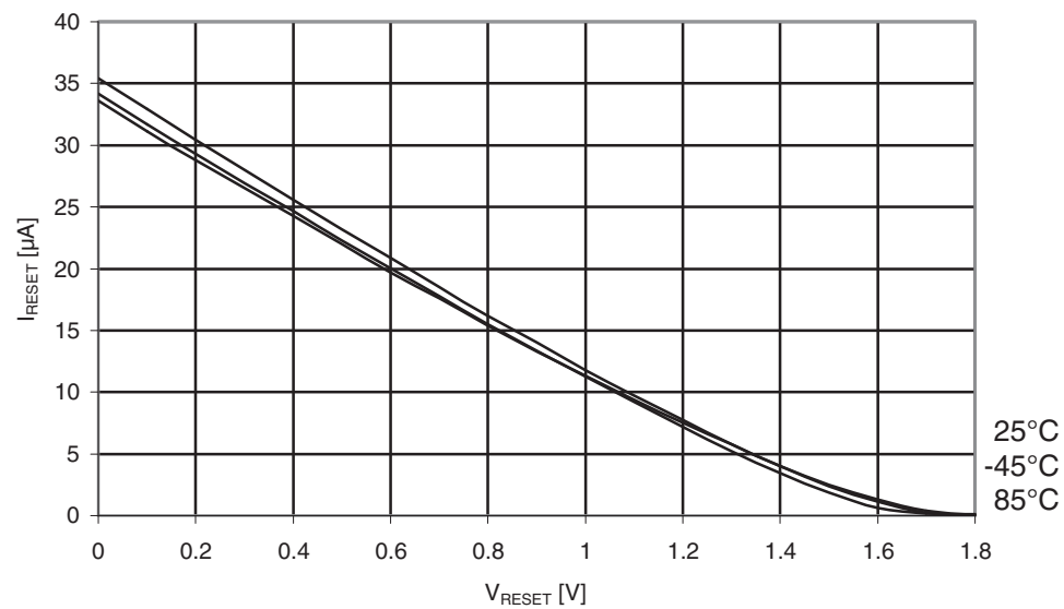
Figure 31-569. ATmega6490P: Reset pull-up resistor current vs. reset pin voltage ( V_{CC} = 1.8V ).
