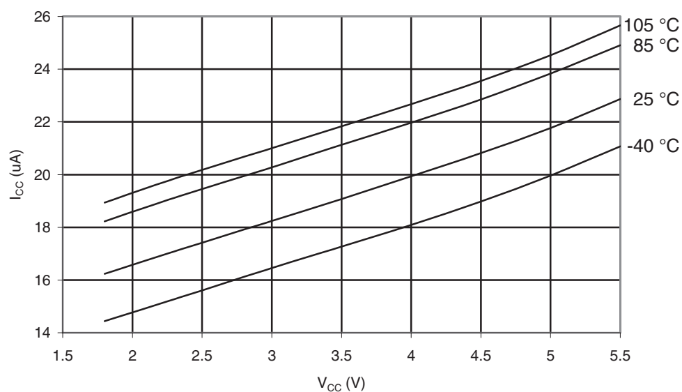
Figure 32-343. ATmega3290PA-105°C: Brownout Detector Current vs. V_{CC}
