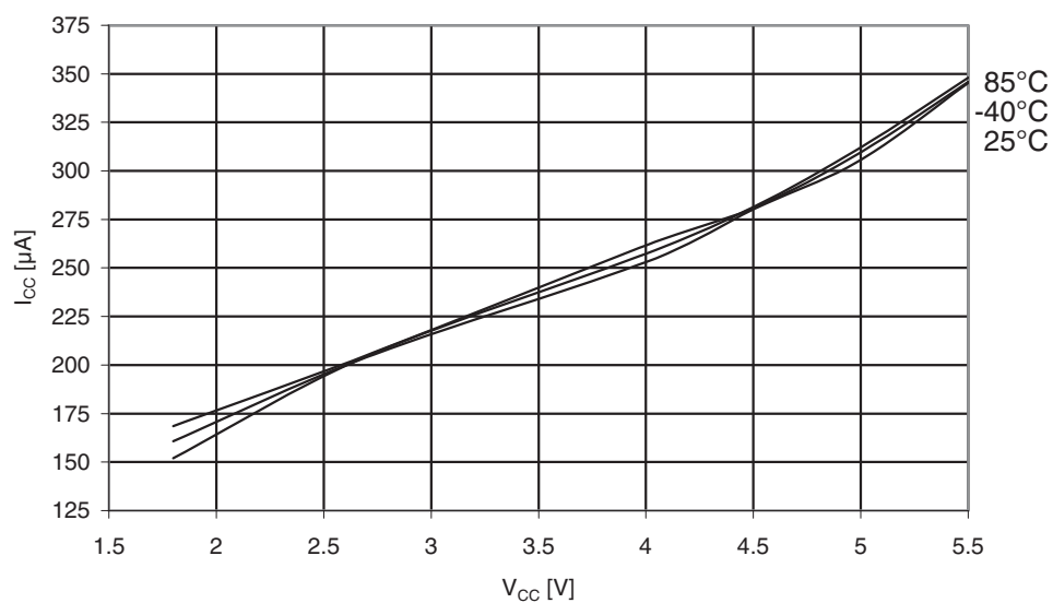
Figure 31-176. ATmega329A: Active supply current with ADC at 200kHz vs. V_{CC} .
