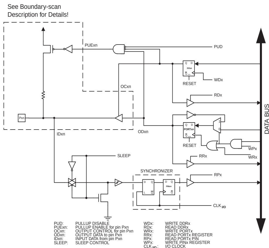
Figure 26-3. General Port Pin, schematic diagram.
