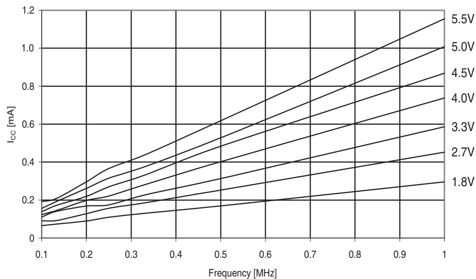
Figure 31-487. ATmega6490A: Active supply current vs. low frequency (0.1 - 1.0MHz).
