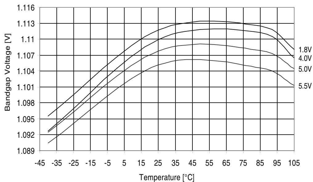
Figure 32-279. ATmega3290A: Bandgap Voltage vs. Temperature
