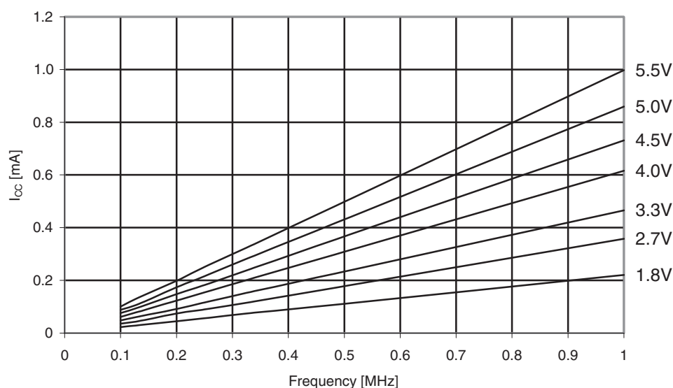
Figure 31-1. ATmega169A: Active supply current vs. low frequency (0.1 - 1.0MHz).
