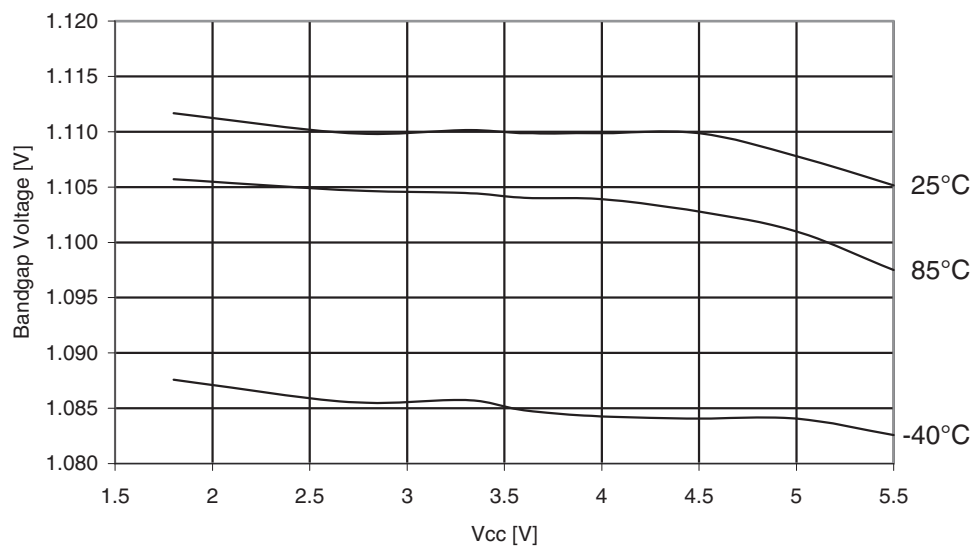
Figure 31-167. Atmel ATmega329A: Bandgap voltage vs. V_{CC} .
