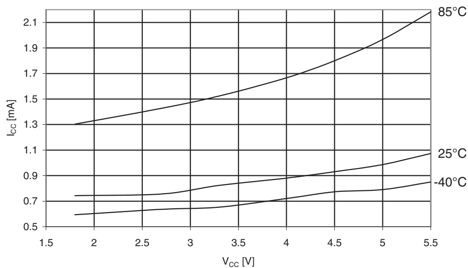
Figure 31-318. Atmel ATmega3290PA Standby Supply current vs. V_{CC} (32kHz watch XTAL, Watchdog Timer disabled).
