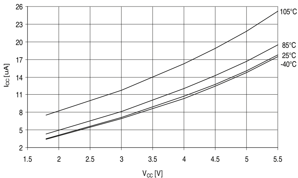
Figure 32-363. ATmega3290PA - 105°C: Power-down Supply Current vs. V_{CC} (Watchdog Timer Enabled)
