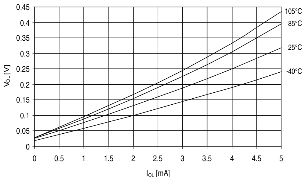
Figure 32-384. ATmega3290PA - 105°C: I/O Pin Output Voltage vs. Sink Current, Port B ( V_{CC} = 1.8V )
