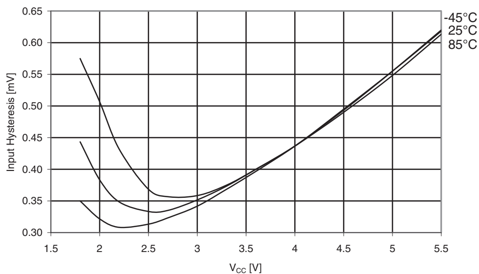
Figure 31-98. ATmega169PA: I/O pin Input Hysteresis vs. V_{CC} .
