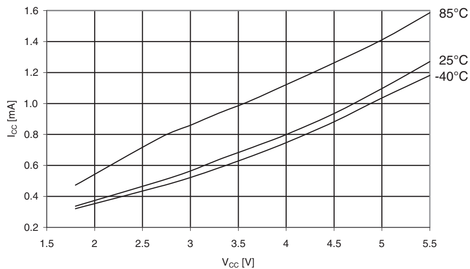
Figure 31-248. ATmega3290A: Active supply current vs. V_{CC} (Internal RC oscillator, 1MHz).
