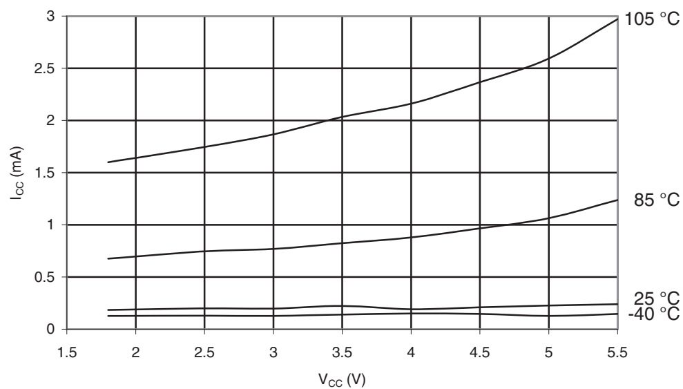
Figure 32-309. ATmega3290PA-105°C: Idle Supply Current vs. V_{CC} (32kHz Watch Crystal)
