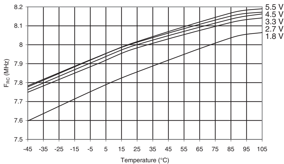
Figure 32-45. ATmega169PA-105°C: Calibrated 8MHz RC Oscillator Frequency vs. Temperature
