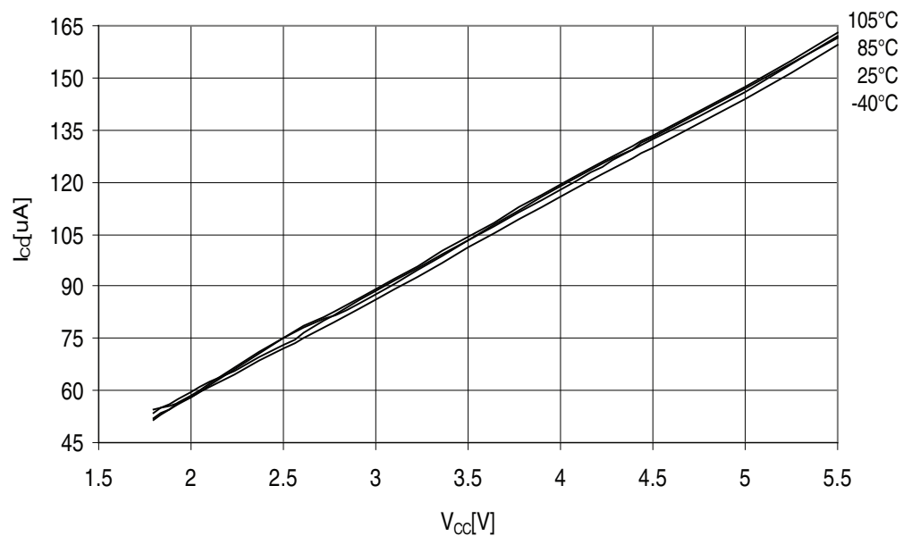
Figure 32-408. ATmega3290PA - 105°C: AREF External Reference Current vs. V_{CC}
