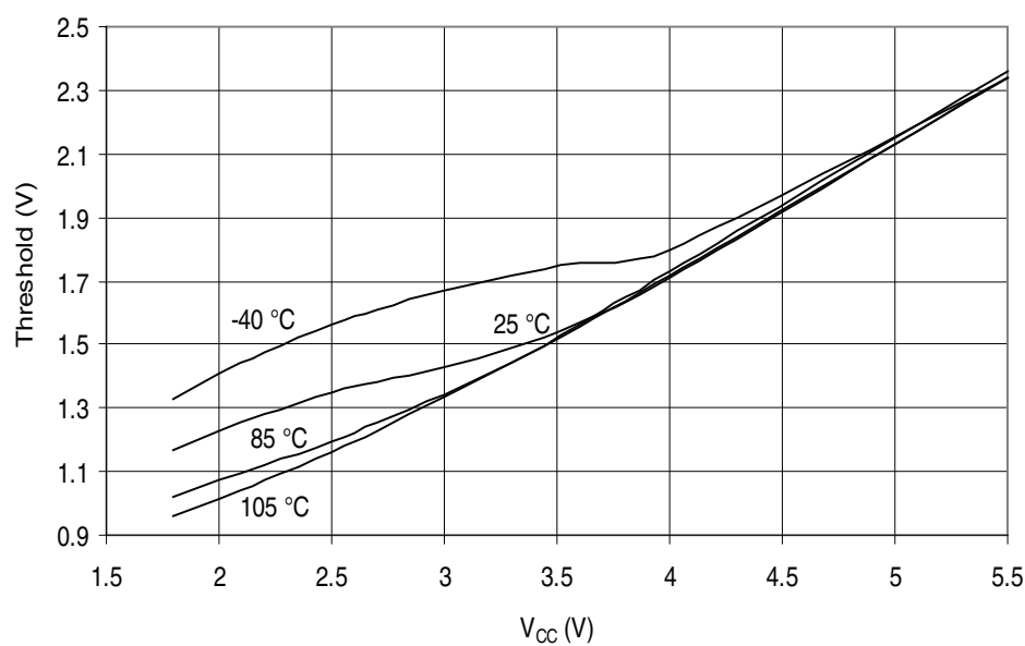
Figure 32-209. ATmega329PA - 105°C: Reset Input Threshold Voltage vs. V_{CC} ( V_{IH} , Reset Pin Read as “1”)
