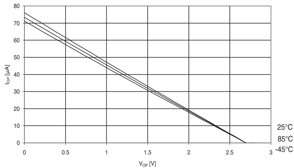
Figure 31-443. ATmega649P: I/O pin pull-up resistor current vs. input voltage ( V_{CC} = 2.7V ).
