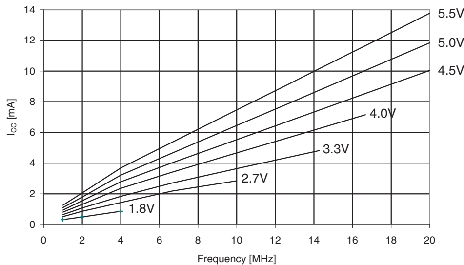
Figure 31-246. ATmega3290A: Active supply current vs. frequency (1 - 20MHz).
