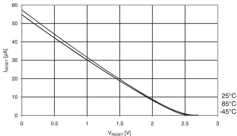
Figure 31-20. ATmega169A: Reset pull-up resistor current vs. reset pin voltage ( V_{CC} = 2.7V ).
