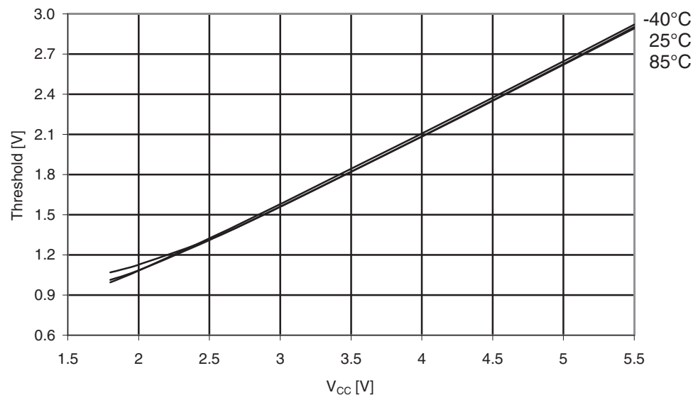
Figure 31-278. ATmega3290A: I/O pin Input Threshold voltage vs. V_{CC} ( V_{IH} , I/O pin read as "1").
