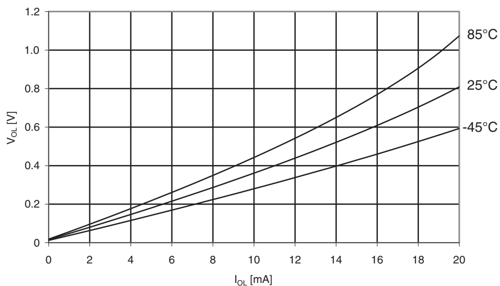
Figure 31-32. ATmega169A: I/O pin output voltage vs. sink current, port B ( V_{CC} = 2.7V ).
