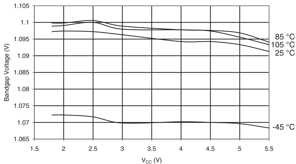
Figure 32-42. ATmega169PA-105°C: Bandgap Voltage vs. V_{CC}
