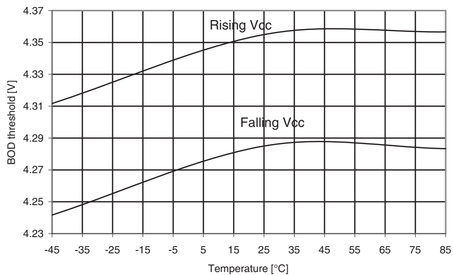
Figure 31-40. ATmega169A: BOD Thresholds vs. temperature (BOD level is 4.3V).
