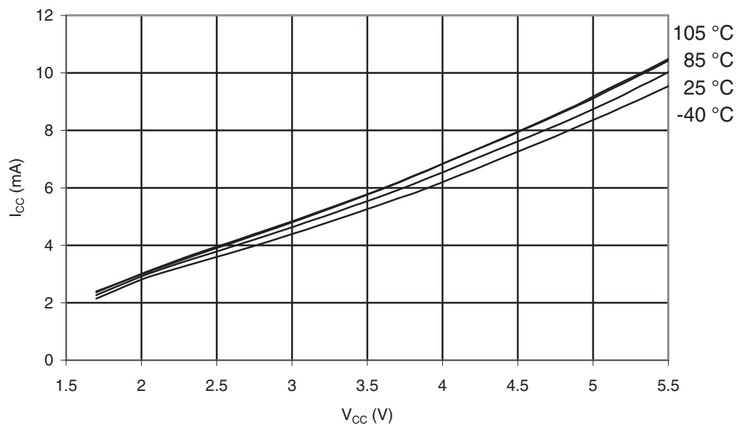
Figure 32-124. ATmega329P-105°C: Active Supply Current vs. V_{CC} (Internal RC Oscillator, 8MHz)
