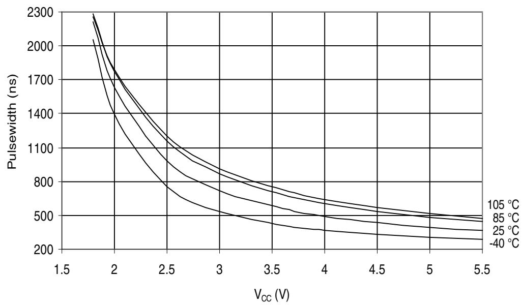
Figure 32-236. ATmega329PA - 105°C: Minimum Reset Pulse Width vs. V_{CC}
