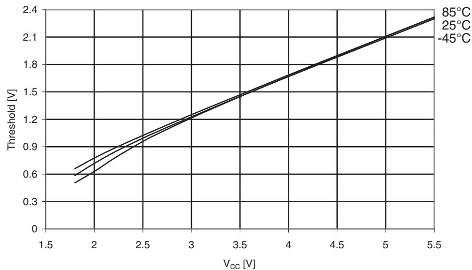
Figure 31-35. Atmel ATmega169A: I/O pin inputThreshold voltage vs. V_{CC} ( V_{IL} , I/O pin read as “0”).
