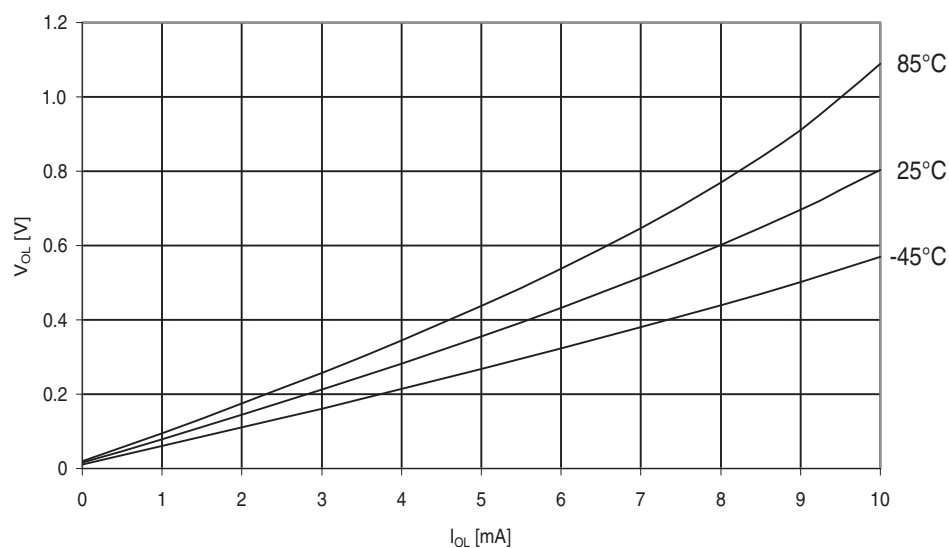
Figure 31-577. ATmega6490P: I/O pin output voltage vs. sink current, ports A, C, D, E, F, G ( V_{CC} = 2.7V ).
