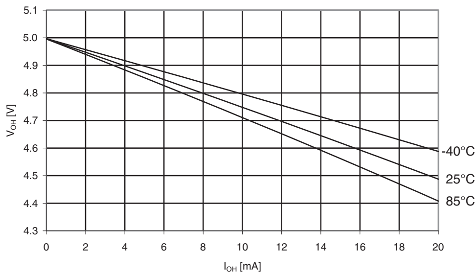
Figure 31-329. ATmega3290PA: I/O pin output voltage vs. source current, port B ( V_{CC} = 5V ).
