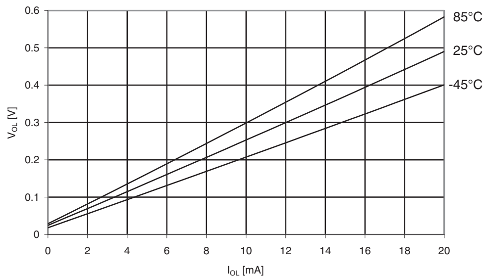
Figure 31-93. Atmel ATmega169PA: I/O pin output voltage vs. Sink current, port B ( V_{CC} = 5V ).
