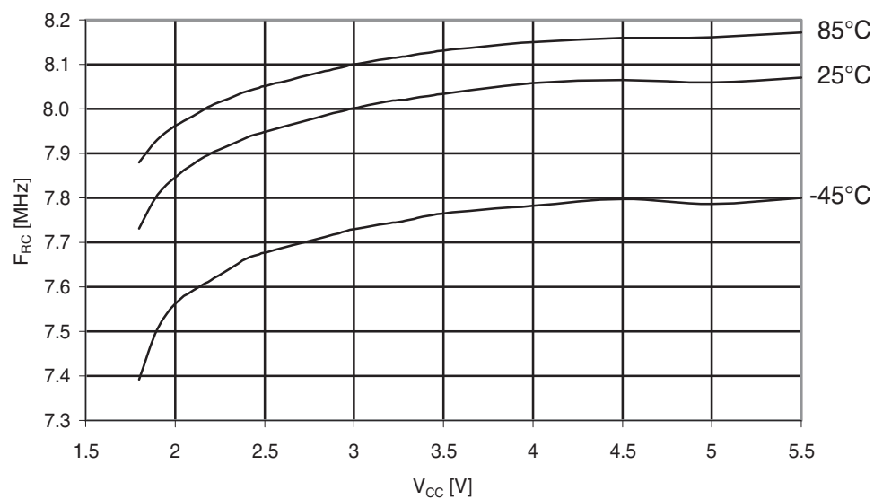
Figure 31-413. Atmel ATmega649A: Calibrated 8MHz RC oscillator frequency vs. V_{CC} .
