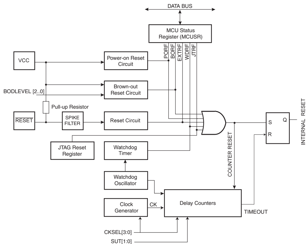
Figure 11-1. Reset logic.
