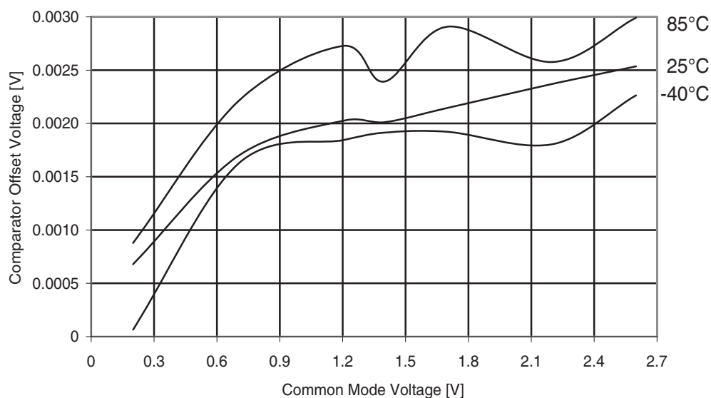
Figure 31-46. ATmega169A: Analog Comparator offset voltage vs. Common Mode voltage ( V_{CC} = 2.7V ).
