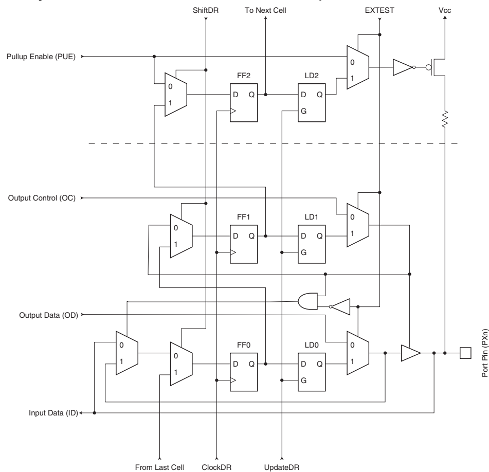
Figure 26-2. Boundary-scan cell for bi-directional Port Pin with Pull-up function.
