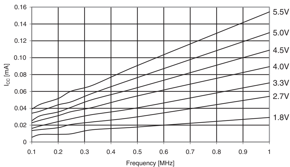
Figure 31-122. ATmega169PA: Reset supply current vs. V_{CC} (0.1 - 1.0MHz, excluding current through the reset pull-up).
