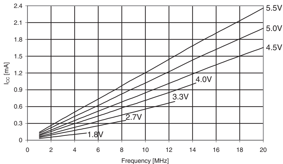
Figure 31-607. ATmega6490P: Reset supply current vs. V_{CC} (1 - 20MHz, excluding current through the reset pull-up).
