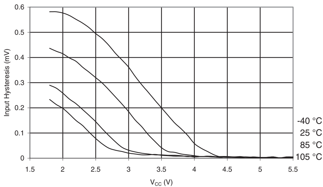
Figure 32-333. ATmega3290PA-105°C: Reset Input Pin Hysteresis vs. V_{CC}
