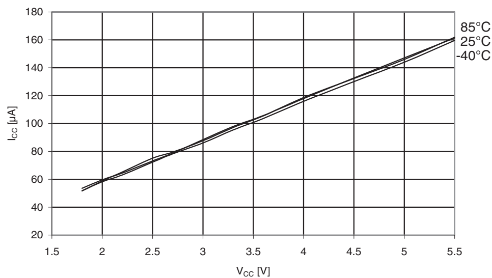
Figure 31-238. ATmega329PA: AREF external reference current vs. V_{CC} .
