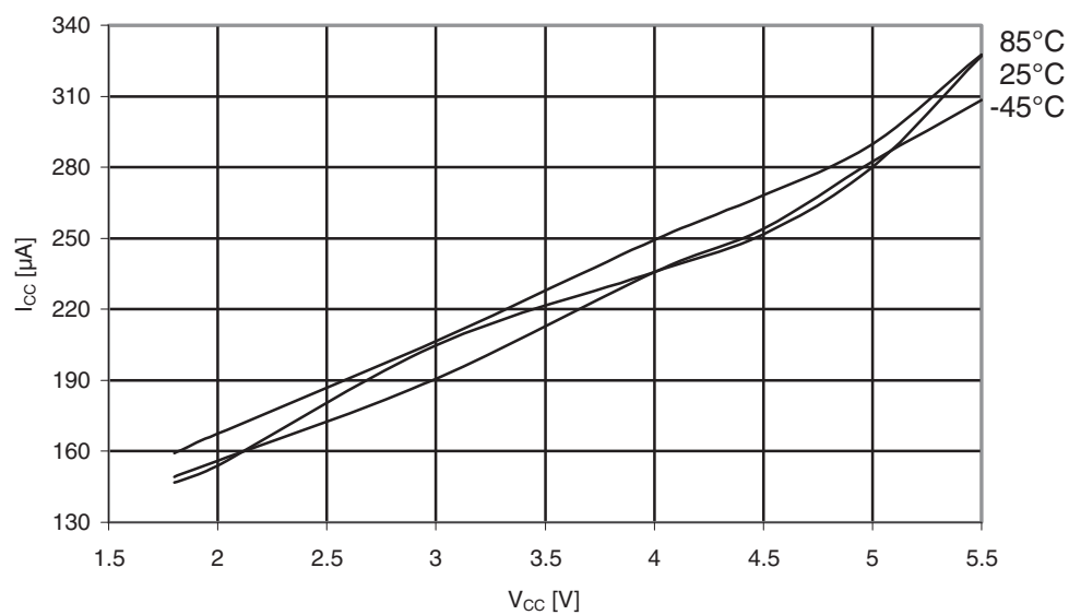
Figure 31-418. ATmega649A: Active supply current with ADC at 1MHz vs. V_{CC} .
