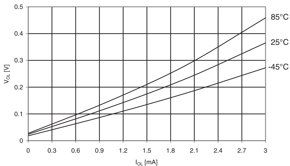
Figure 31-92. ATmega169PA: I/O pin output voltage vs. Sink current, ports A, C, D, E, F, G ( V_{CC} = 1.8V ).
