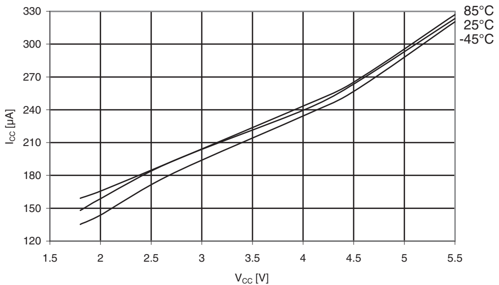
Figure 31-538. ATmega6490A: Active supply current with ADC at 50kHz vs. V_{CC} .
