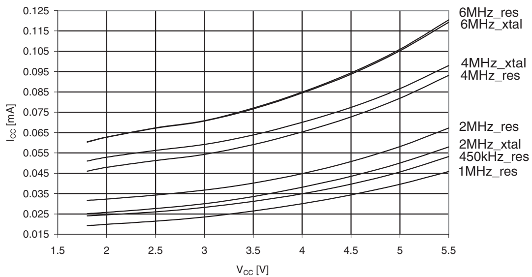
Figure 31-441. ATmega649P: Standby supply current vs. V_{CC} (XTAL and resonator, Watchdog Timer disabled).
