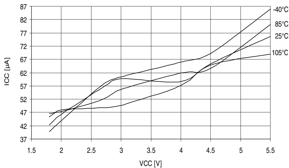
Figure 32-410. ATmega3290PA - 105°C: Analog Comparator Current vs. V_{CC}
