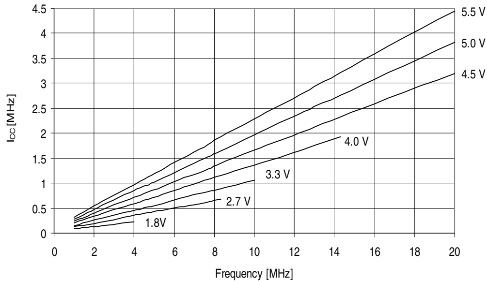
Figure 32-65. ATmega329A - 105°C: Idle Supply Current vs. Frequency (1 - 20MHz)
