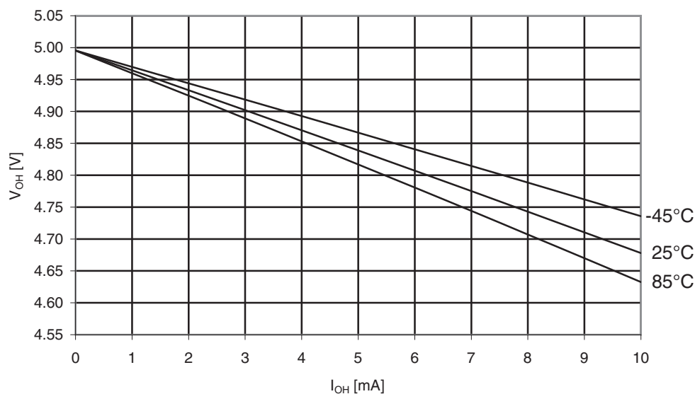
Figure 31-22. ATmega169A: I/O pin output voltage vs. source current, ports A, C, D, E, F, G ( V_{CC} = 5V ).
