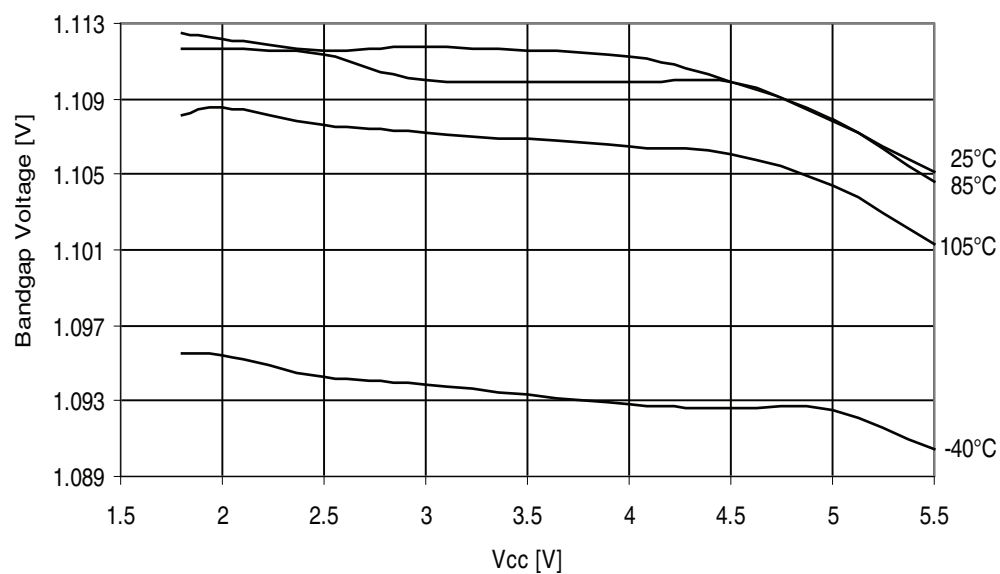
Figure 32-100. ATmega329A - 105°C: Bandgap Voltage vs. V_{CC}
