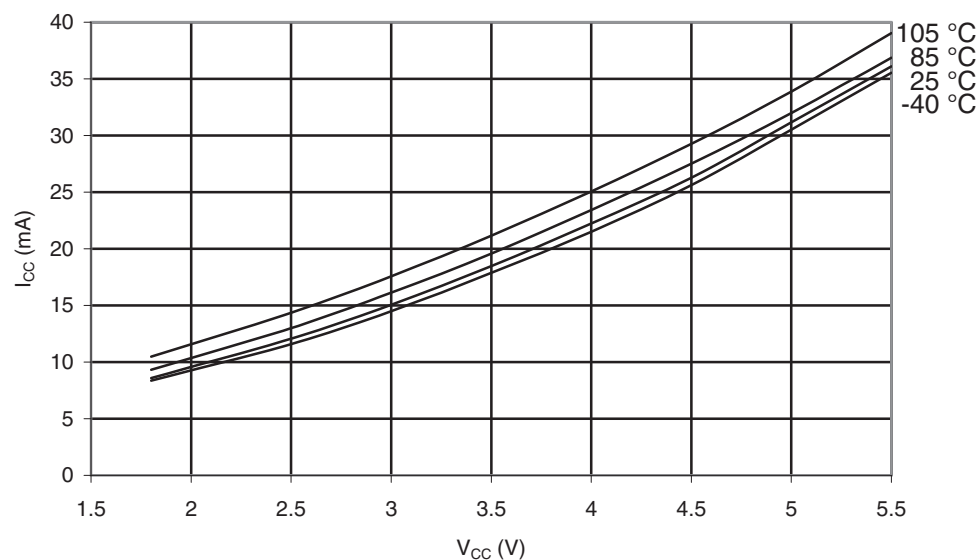
Figure 32-126. ATmega329P-105°C: Active Supply Current vs. V_{CC} (32kHz Watch Crystal)
