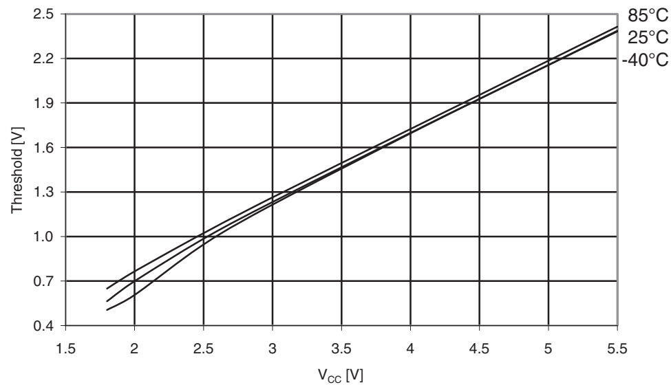
Figure 31-159. Atmel ATmega329A. I/O pin Input Threshold voltage vs. V_{CC} ( V_{IL} , I/O pin read as “0”).
