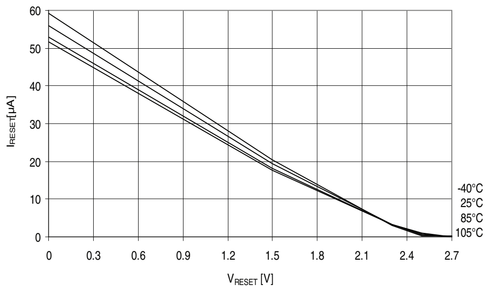
Figure 32-77. ATmega329A - 105°C: Reset Pull-up Resistor Current vs. Reset Pin Voltage ( V_{CC} = 2.7V )
