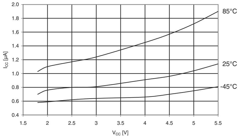
Figure 31-13. Atmel ATmega169A: Power-save supply current vs. V_{CC} (Watchdog Timer disabled and 32kHz XTAL oscillator running).
