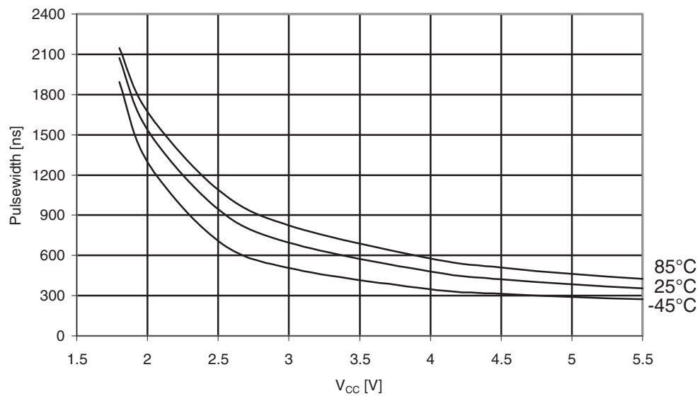
Figure 31-547. Atmel ATmega6490A: Minimum reset pulse width vs. V_{CC} .
