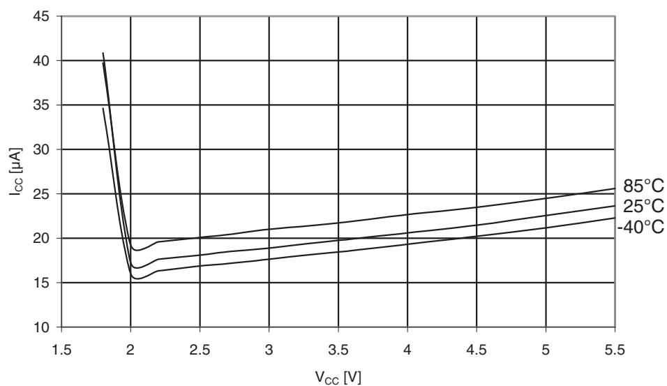
Figure 31-174. ATmega329A: Brownout Detector current vs. V_{CC} .
