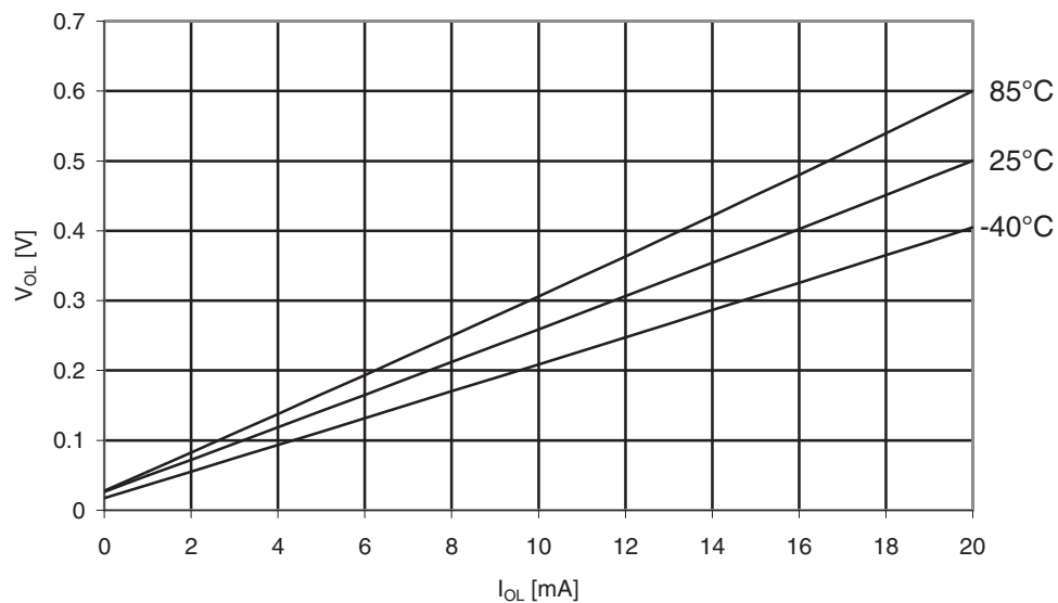
Figure 31-155. Atmel ATmega329A: I/O pin output voltage vs. sink current, port B ( V_{CC} = 5V ).
