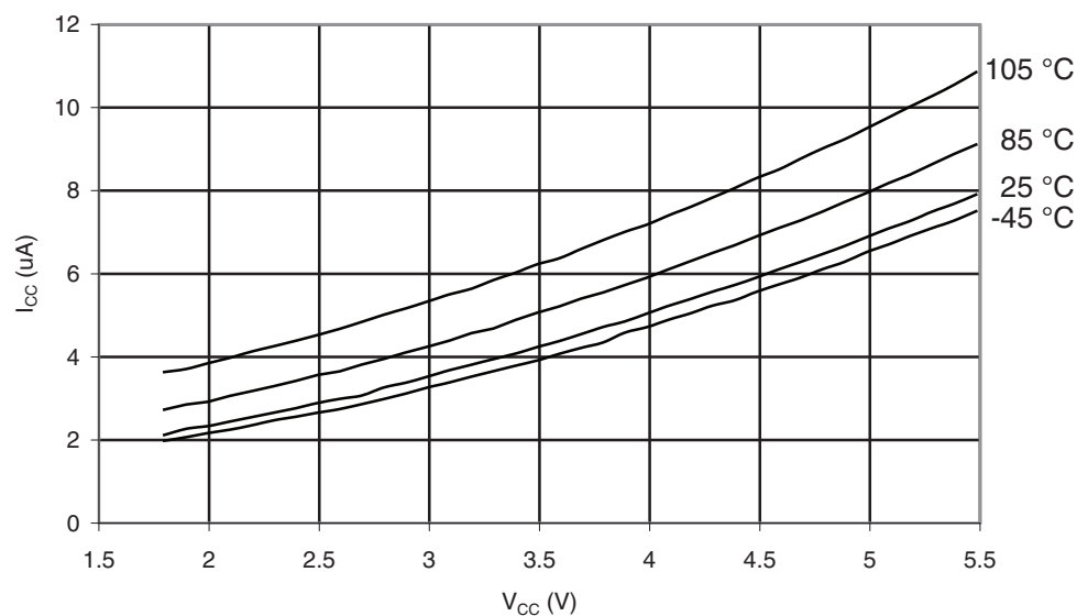
Figure 32-183. ATmega329PA - 105°C: Idle Supply Current vs. V_{CC} (32kHz Watch Crystal)
