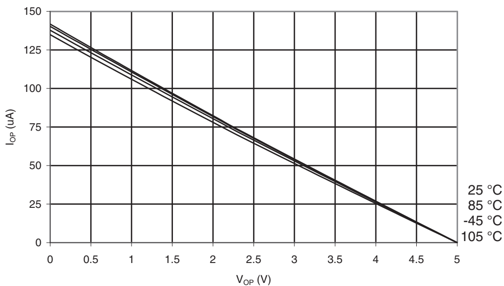
Figure 32-15. ATmega169PA-105°C: I/O Pin Pull-up Resistor Current vs. Input Voltage ( V_{CC} = 5V )
