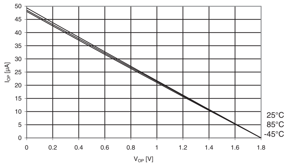
Figure 31-80. ATmega169PA: I/O pin pull-up resistor current vs. input voltage ( V_{CC} = 1.8V ).
