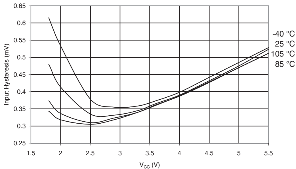
Figure 32-330. ATmega3290PA-105°C: I/O Pin Input Hysteresis vs. V_{CC}
