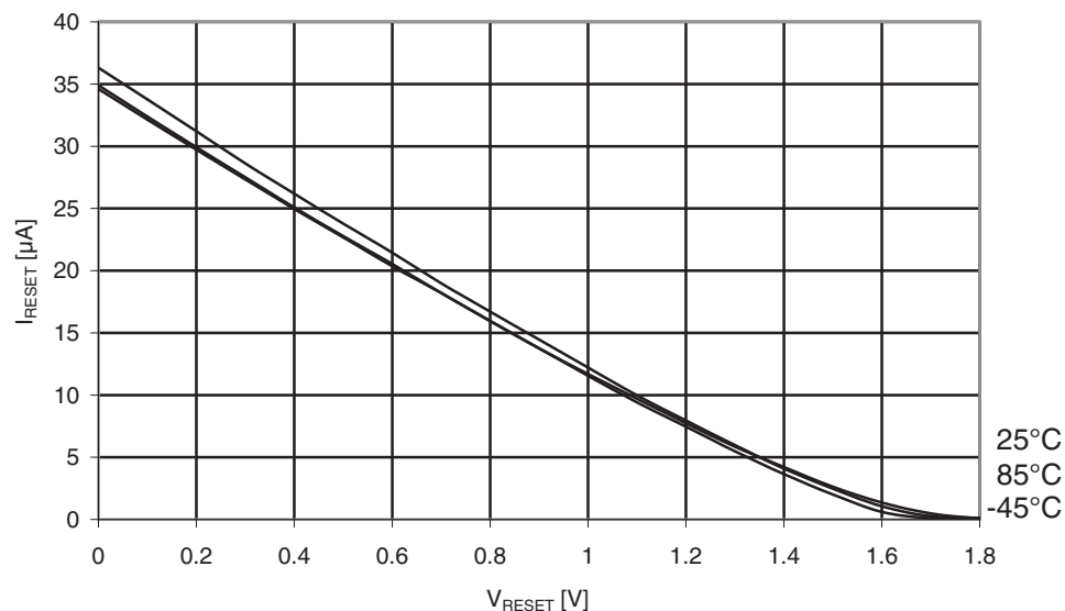
Figure 31-21. Atmel ATmega169A: Reset pull-up resistor current vs. reset pin voltage ( V_{CC} = 1.8V ).
