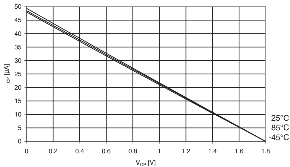
Figure 31-18. ATmega169A: I/O pin pull-up resistor current vs. input voltage ( V_{CC} = 1.8V ).
