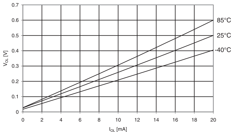
Figure 31-215. Atmel ATmega329PA: I/O pin output voltage vs. sink current, port B ( V_{CC} = 5V ).
