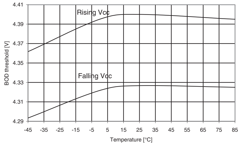
Figure 31-405. Atmel ATmega649A: BOD Thresholds vs. temperature (BOD level is 4.3V).
