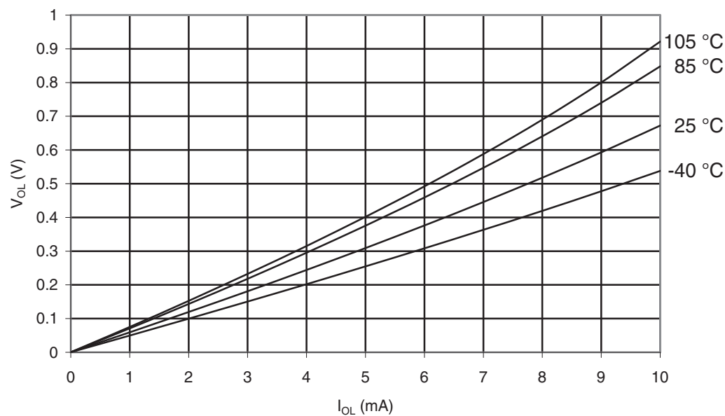
Figure 32-149. ATmega329P-105°C: I/O Pin Output Voltage vs. Sink Current, Port B ( V_{CC} = 3V )
