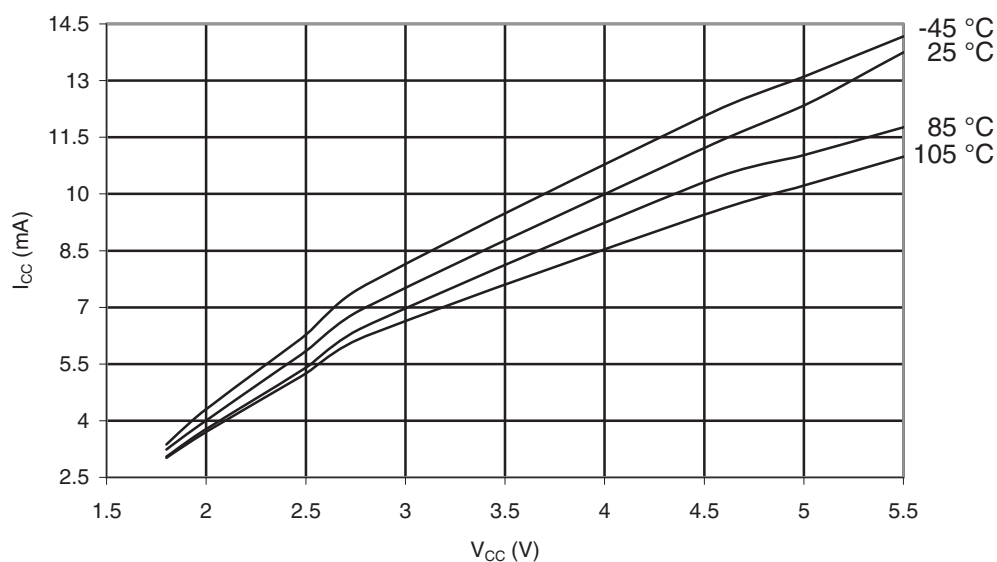
Figure 32-55. ATmega169PA-105°C: Programming Current vs. V_{CC}
