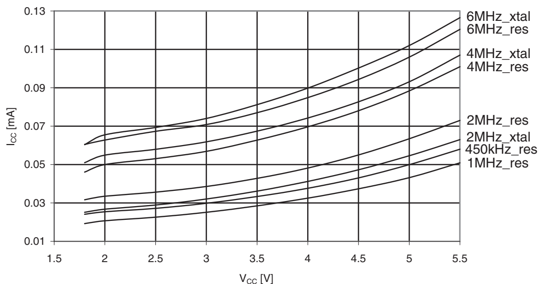
Figure 31-199. Atmel ATmega329PA standby supply current vs. V_{CC} (XTAL and resonator, Watchdog Timer disabled).
