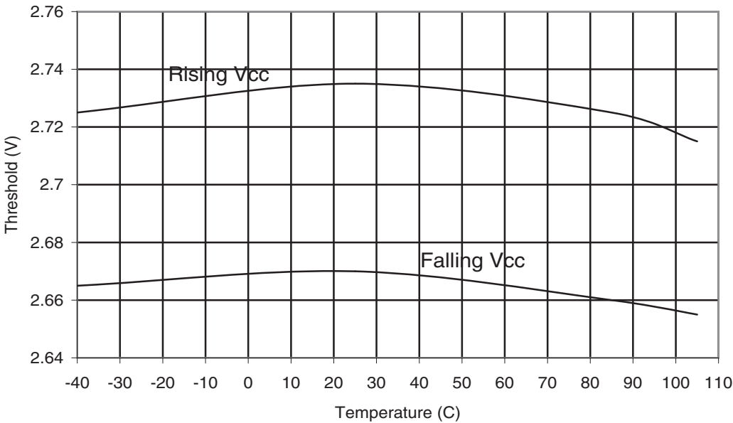
Figure 32-335. ATmega3290PA-105°C: BOD Thresholds vs. Temperature (BOD Level is 2.7V)
