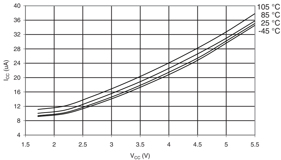
Figure 32-241. ATmega3290A - 105°C: Active Supply Current vs. V_{CC} (32kHz Watch Crystal)
