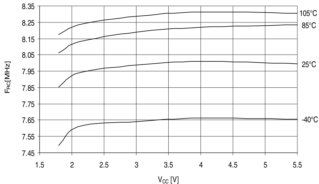
Figure 32-107. ATmega329A - 105°C: Calibrated 8MHz RC Oscillator Frequency vs. V_{CC}
