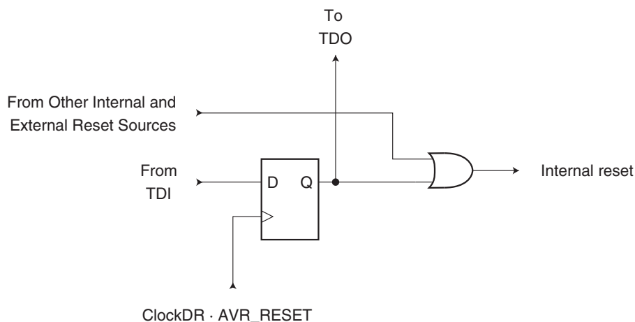
Figure 26-1. Reset register.
