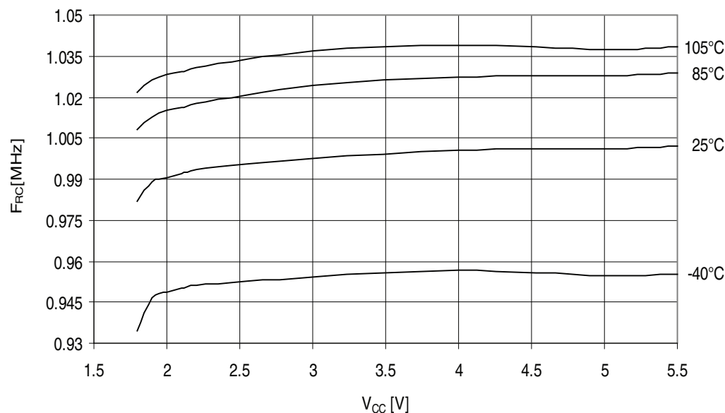
Figure 32-220. ATmega329PA - 105°C: Calibrated 1MHz RC Oscillator Frequency vs. V_{CC}
