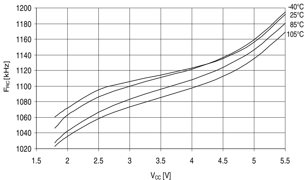
Figure 32-103. ATmega329A - 105°C: Watchdog Oscillator Frequency vs. V_{CC}
