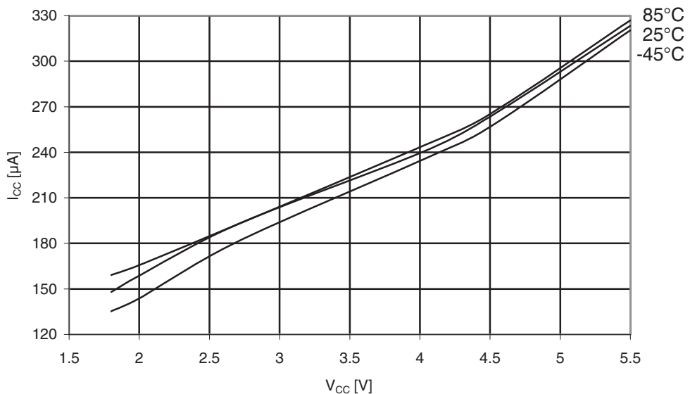
Figure 31-477. ATmega649P: Active supply current with ADC at 50kHz vs. V_{CC} .
