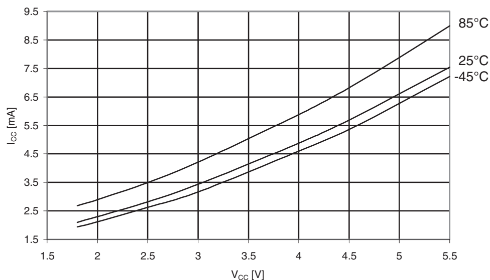
Figure 31-496. ATmega6490A: Idle supply current vs. V_{CC} (32kHz watch XTAL).
