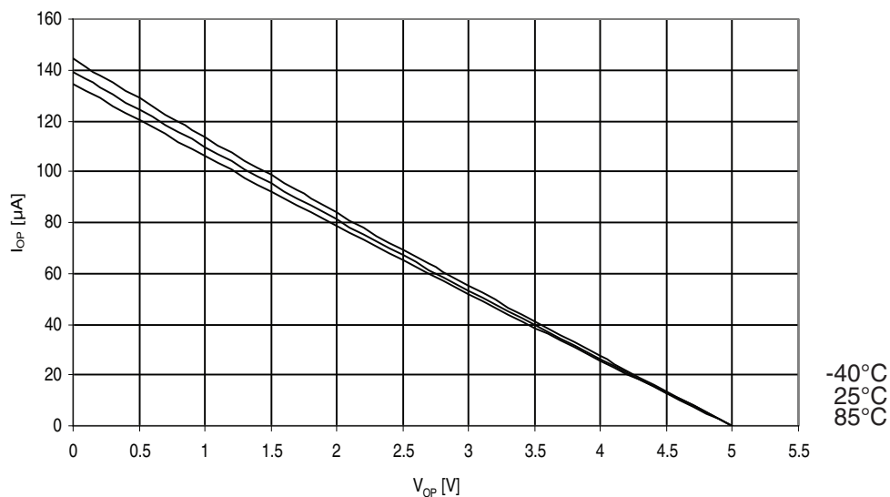
Figure 31-200. ATmega329PA: I/O pin pull-up resistor current vs. input voltage ( V_{CC} = 5V ).
