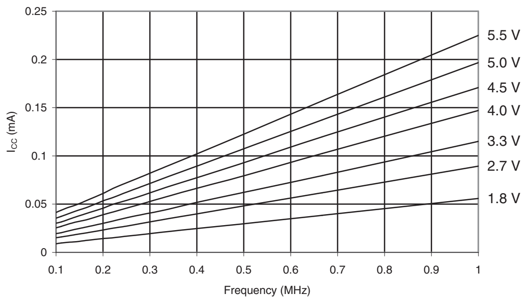
Figure 32-171. ATmega329P-105°C: Reset Supply Current vs. V_{CC} (0.1 - 1.0MHz, Excluding Current Through The Reset Pull-up)
