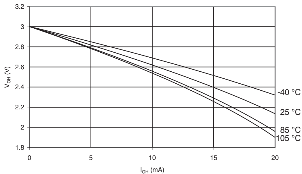
Figure 32-321. ATmega3290PA-105°C: I/O Pin Output Voltage vs. Source Current, Ports A,C,D,E,G,G ( V_{CC} = 3V )
