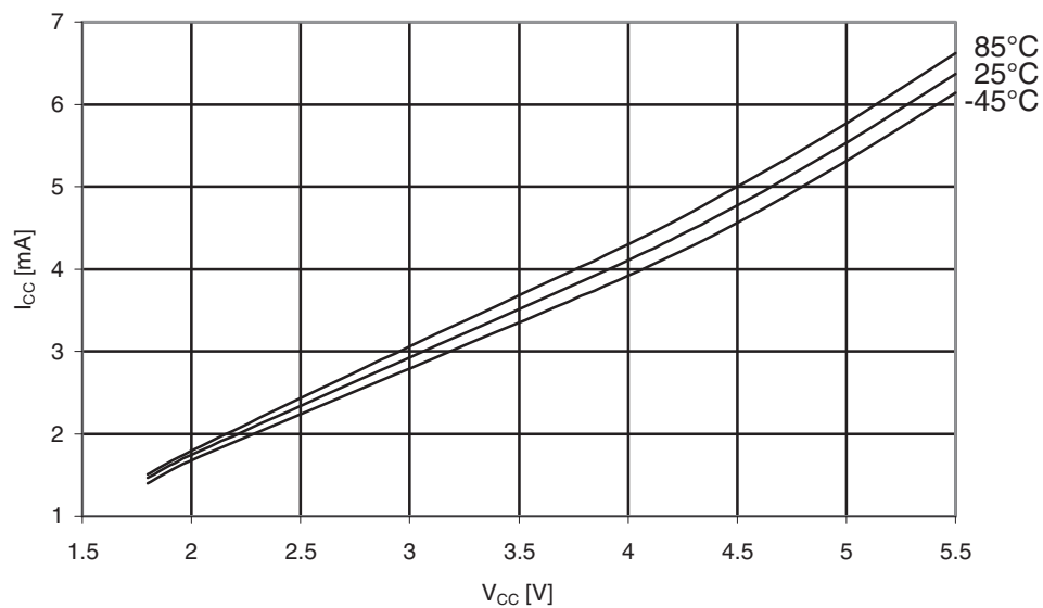
Figure 31-367. Atmel ATmega649A: Active supply current vs. V_{CC} (Internal RC oscillator, 8MHz).
