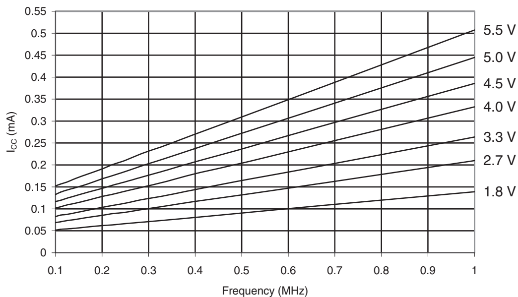
Figure 32-305. ATmega3290PA-105°C: Idle Supply Current vs. Frequency (0.1 - 1.0MHz)
