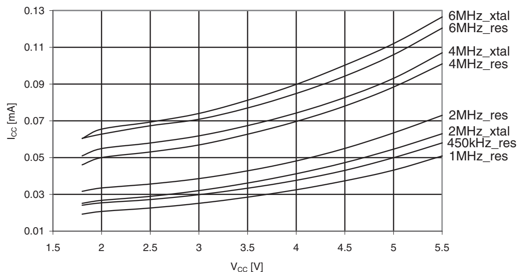
Figure 31-139. Atmel ATmega329A: Standby supply current vs. V_{CC} (XTAL and resonator, Watchdog Timer disabled).
