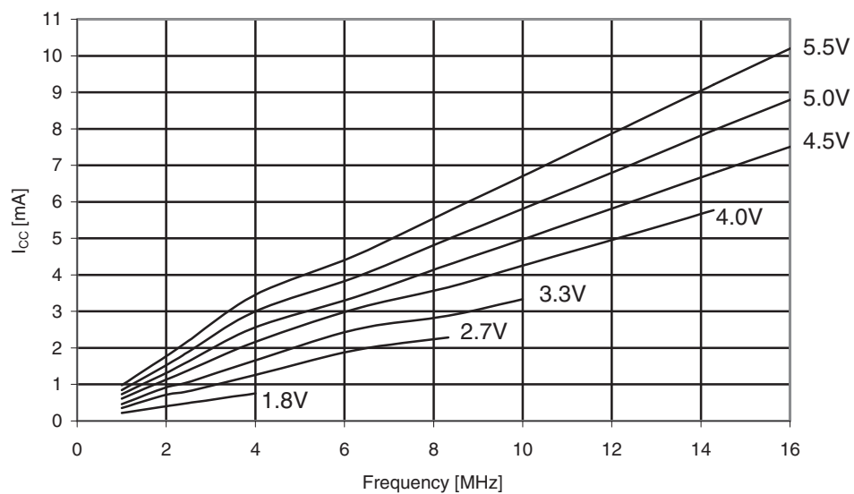
Figure 31-64. ATmega169PA: Active supply current vs. frequency (1 - 16MHz).
