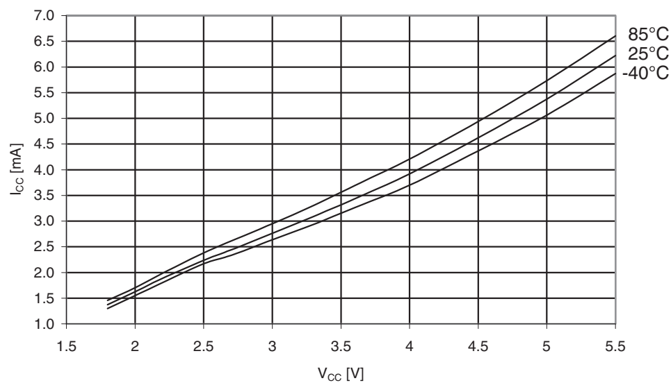
Figure 31-307. Atmel ATmega3290PA: Active supply current vs. V_{CC} (Internal RC oscillator, 8MHz).
