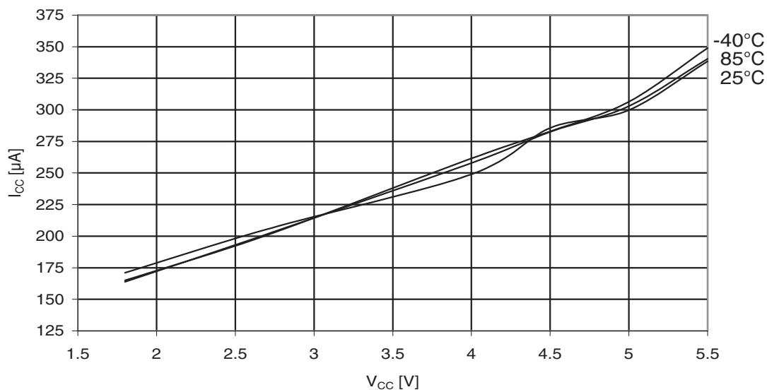
Figure 31-357. ATmega3290PA: Active supply current with ADC at 1MHz vs. V_{CC} .
