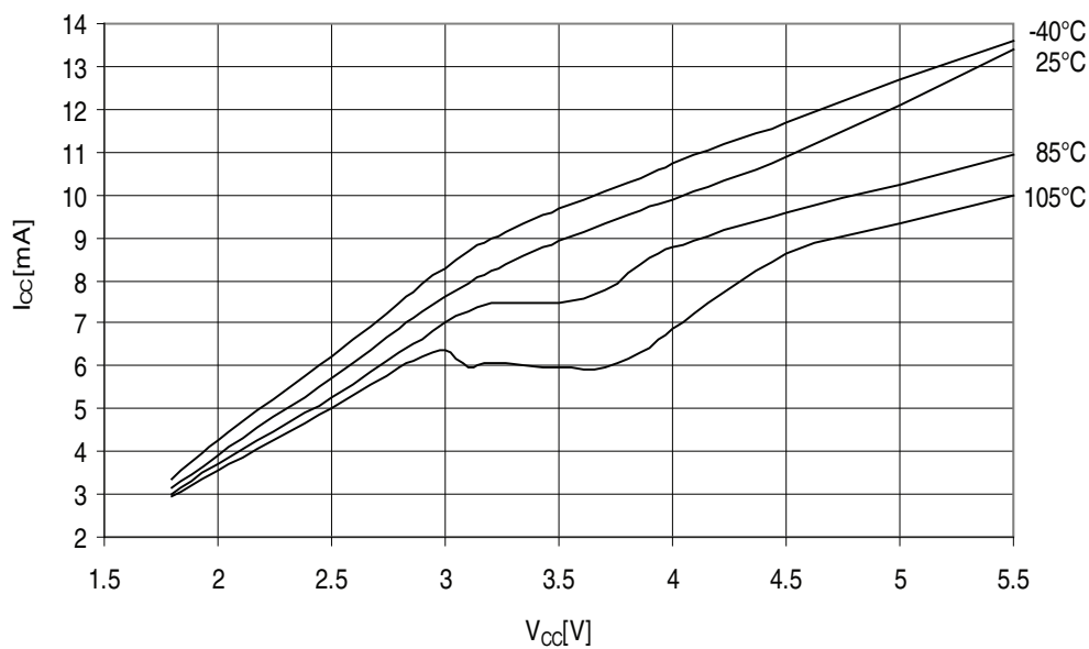
Figure 32-411. ATmega3290PA - 105°C: Programming Current vs. V_{CC}
