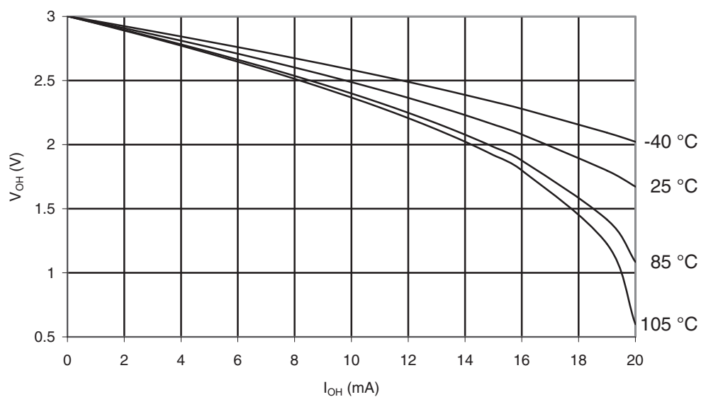
Figure 32-145. ATmega329P-105°C: I/O Pin Output Voltage vs. Source Current, Port B ( V_{CC} = 3V )
