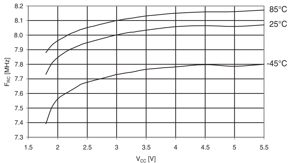
Figure 31-535. Atmel ATmega6490A: Calibrated 8MHz RC oscillator frequency vs. V_{CC} .
