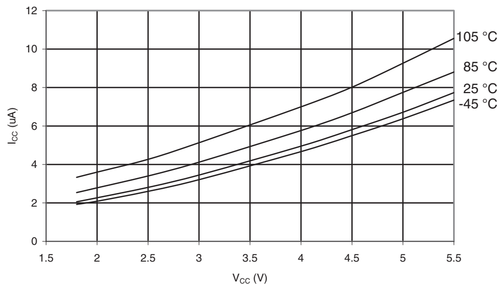
Figure 32-10. ATmega169PA-105°C: Idle Supply Current vs. V_{CC} (32kHz Watch Crystal)
