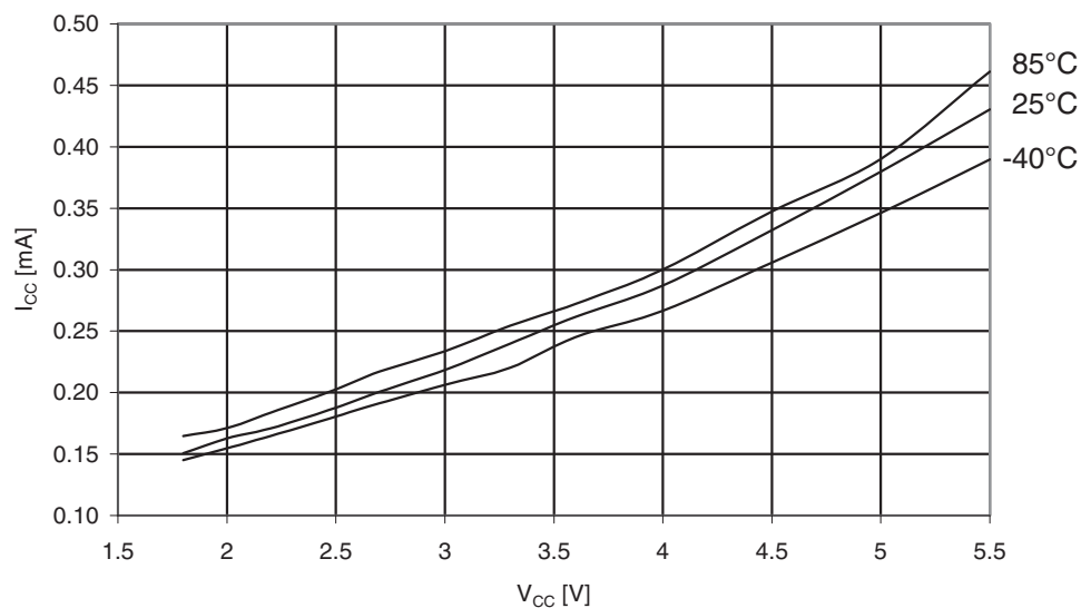
Figure 31-313. Atmel ATmega3290PA: Idle supply current vs. V_{CC} (Internal RC oscillator, 1MHz).
