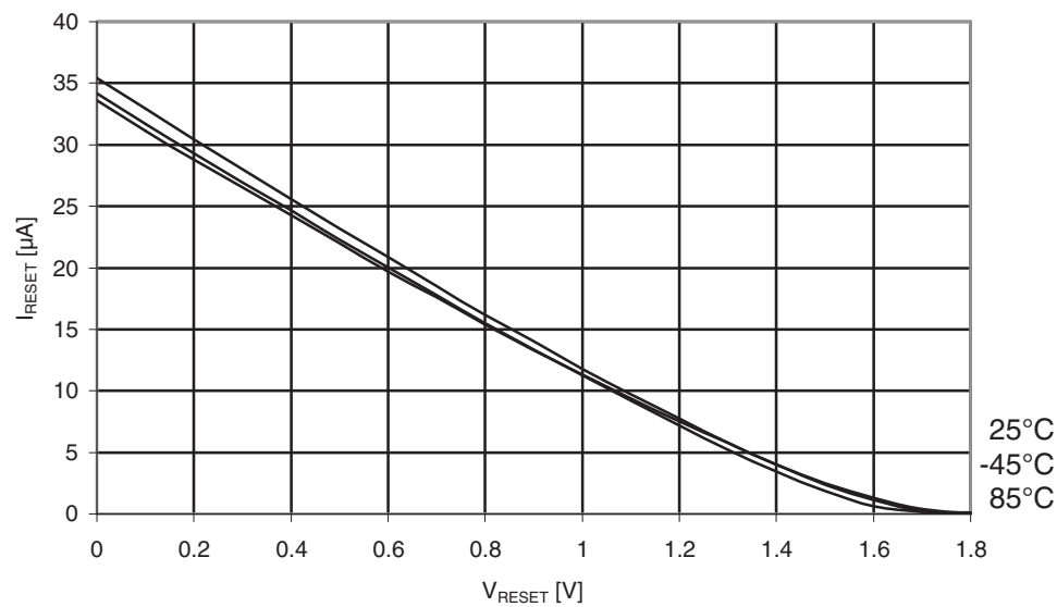
Figure 31-508. ATmega6490A: Reset pull-up resistor current vs. reset pin voltage ( V_{CC} = 1.8V ).
