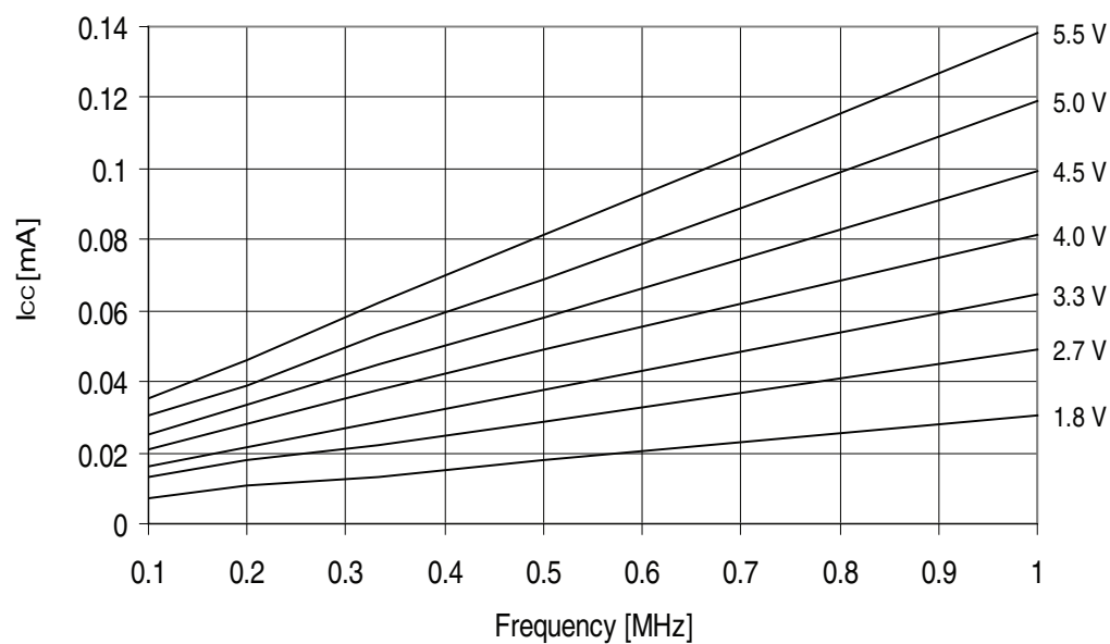
Figure 32-296. ATmega3290A - 105°C: Reset Supply Current vs. V_{CC} (0.1 - 1.0MHz, Excluding Current Through The Reset Pull-up)
