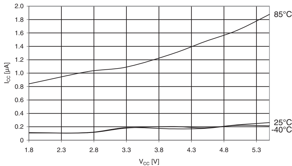
Figure 31-196. ATmega329PA: Power-down supply current vs. V_{CC} (Watchdog Timer enabled).
