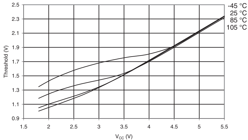
Figure 32-36. ATmega169PA-105°C: Reset Input Threshold Voltage vs. V_{CC} ( V_{IH} , Reset Pin Read as “1”)
