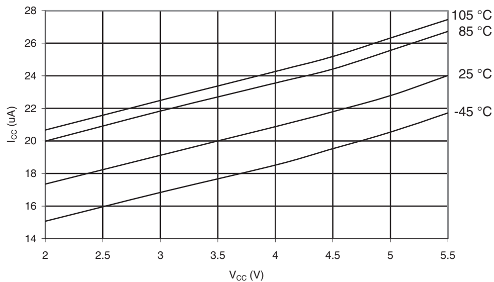
Figure 32-48. ATmega169PA-105°C: Brownout Detector Current vs. V_{CC}
