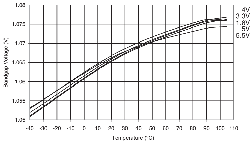
Figure 32-160. ATmega329P-105°C: Bandgap Voltage vs. Temperature
