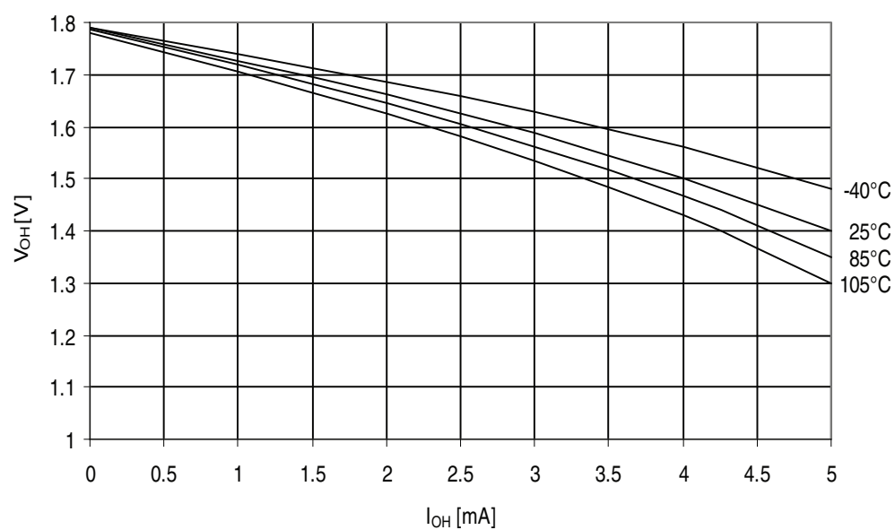
Figure 32-262. ATmega3290A - 105°C: I/O Pin Output Voltage vs. Source Current, Port B ( V_{CC} = 1.8V )
