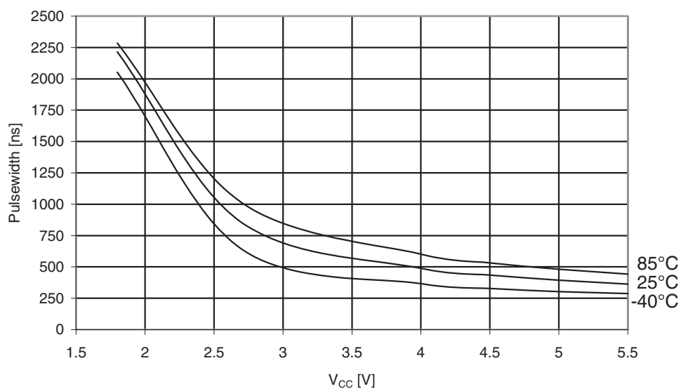
Figure 31-184. ATmega329A: Minimum reset pulse width vs. V_{CC} .
