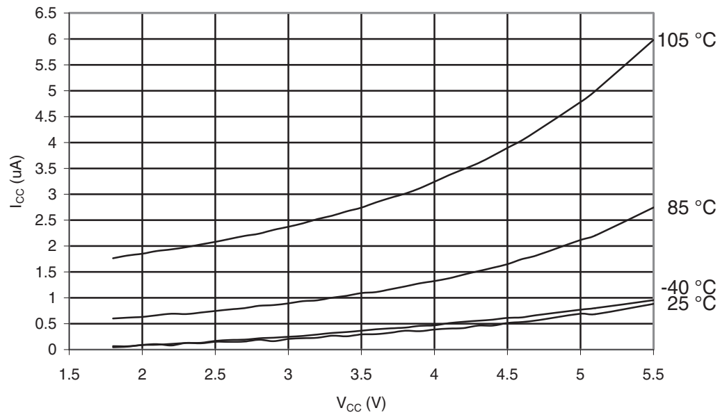
Figure 32-132. ATmega329P-105°C: Power-down Supply Current vs. V_{CC} (Watchdog Timer Disabled)
