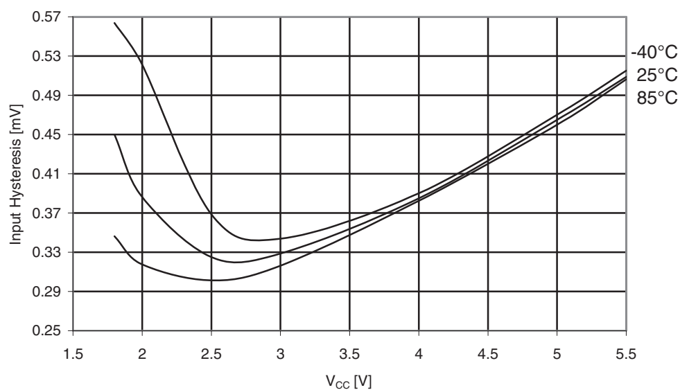
Figure 31-280. ATmega3290A: I/O pin Input Hysteresis vs. V_{CC} .
