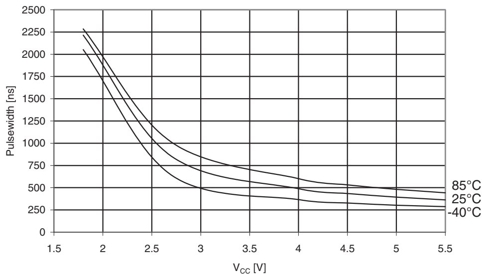
Figure 31-244. ATmega329PA: Minimum reset pulse width vs. V_{CC} .
