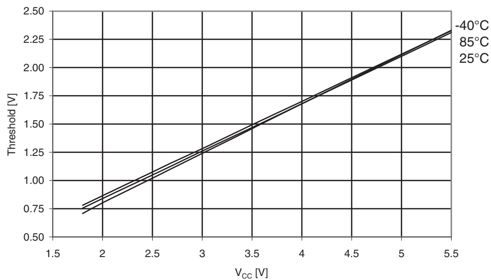
Figure 31-282. ATmega3290A: Reset Input Threshold voltage vs. V_{CC} ( V_{IL} , reset pin read as “0”).
