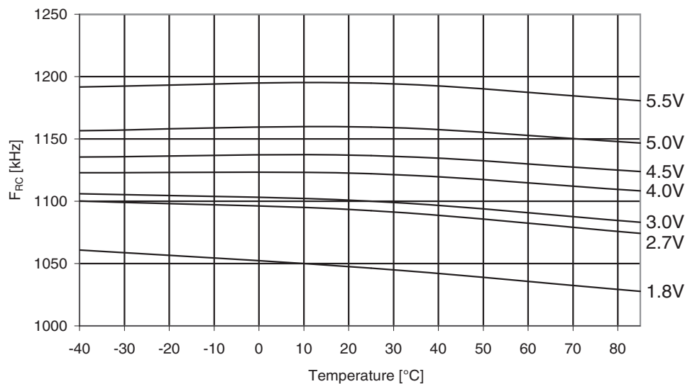
Figure 31-170. ATmega329A: Watchdog oscillator frequency vs. temperature.
