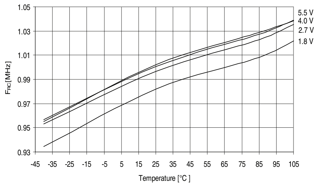
Figure 32-282. ATmega3290A - 105°C: Calibrated 1MHz RC Oscillator Frequency vs. Temperature
