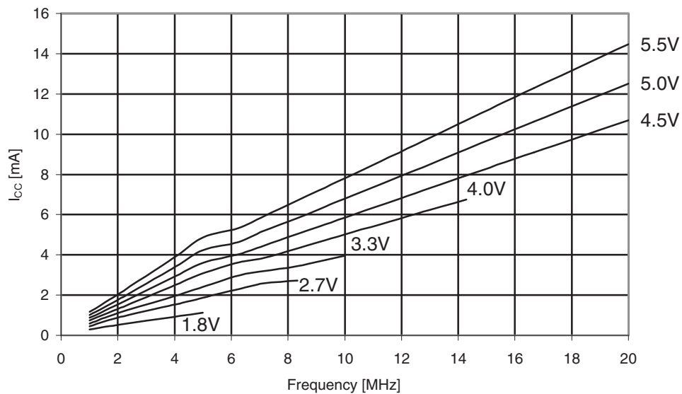
Figure 31-549. ATmega6490P: Active supply current vs. frequency (1 - 20MHz).
