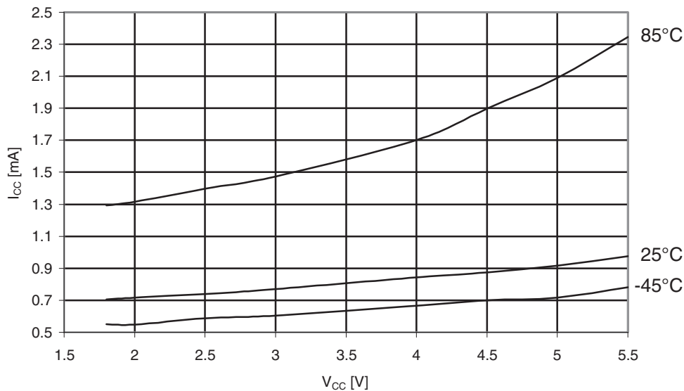
Figure 31-380. ATmega649A: Standby supply current vs. V_{CC} (XTAL and resonator, Watchdog Timer disabled).
