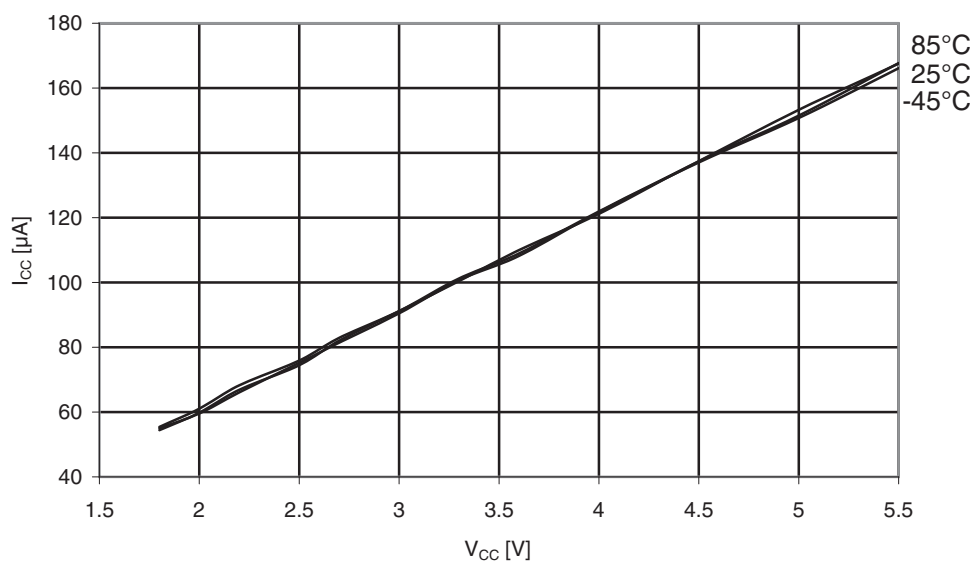
Figure 31-118. ATmega169PA: AREF external reference current vs. V_{CC} .
