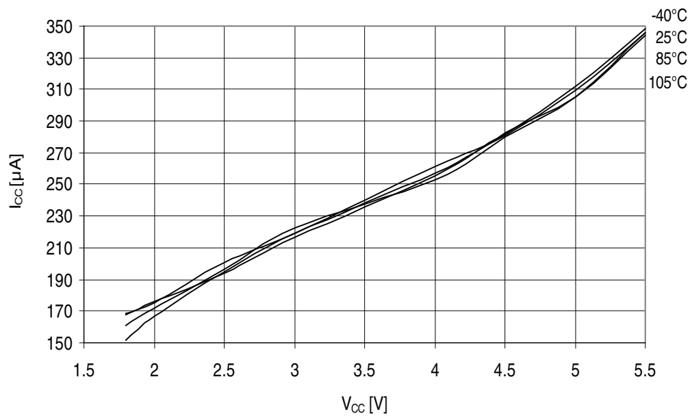
Figure 32-405. ATmega3290PA - 105°C: Active Supply Current with ADC at 200kHz vs. V_{CC}
