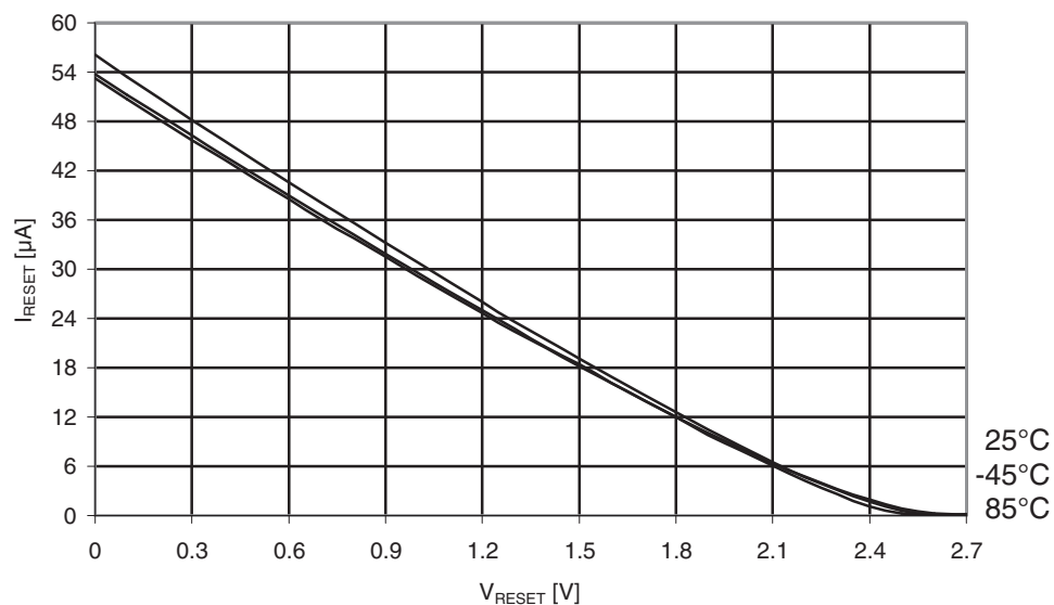
Figure 31-385. Atmel ATmega649A: Reset pull-up resistor current vs. reset pin voltage ( V_{CC} = 2.7V ).
