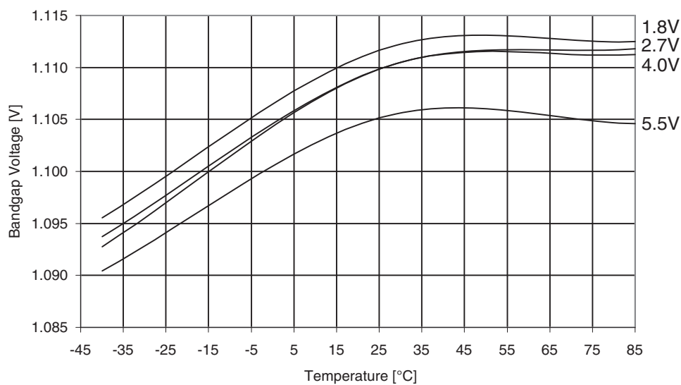
Figure 31-348. Atmel ATmega3290PA: Bandgap voltage vs. temperature.
