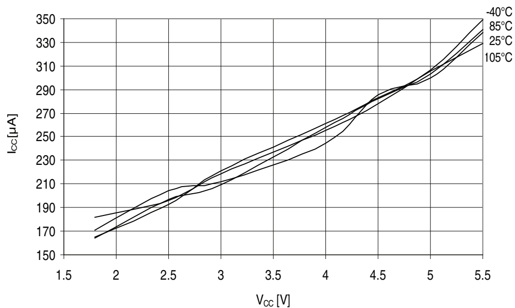
Figure 32-228. ATmega329PA - 105°C: Active Supply Current with ADC at 2MHz vs. V_{CC} )
