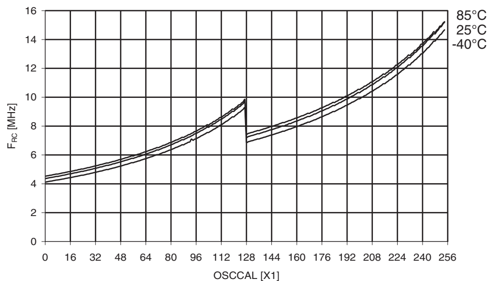
Figure 31-233. Atmel ATmega329PA: Calibrated 8MHz RC oscillator frequency vs. Oscscal value.
