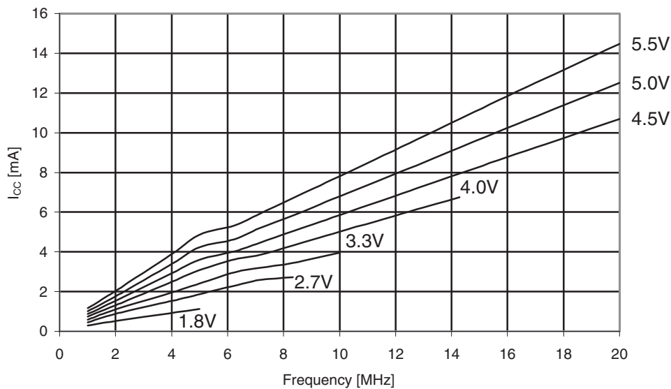
Figure 31-427. ATmega649P: Active supply current vs. frequency (1 - 20MHz).
