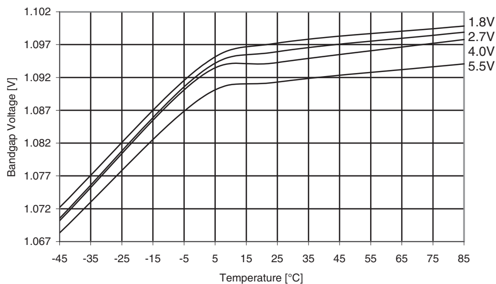
Figure 31-44. ATmega169A: Bandgap voltage vs. temperature.
