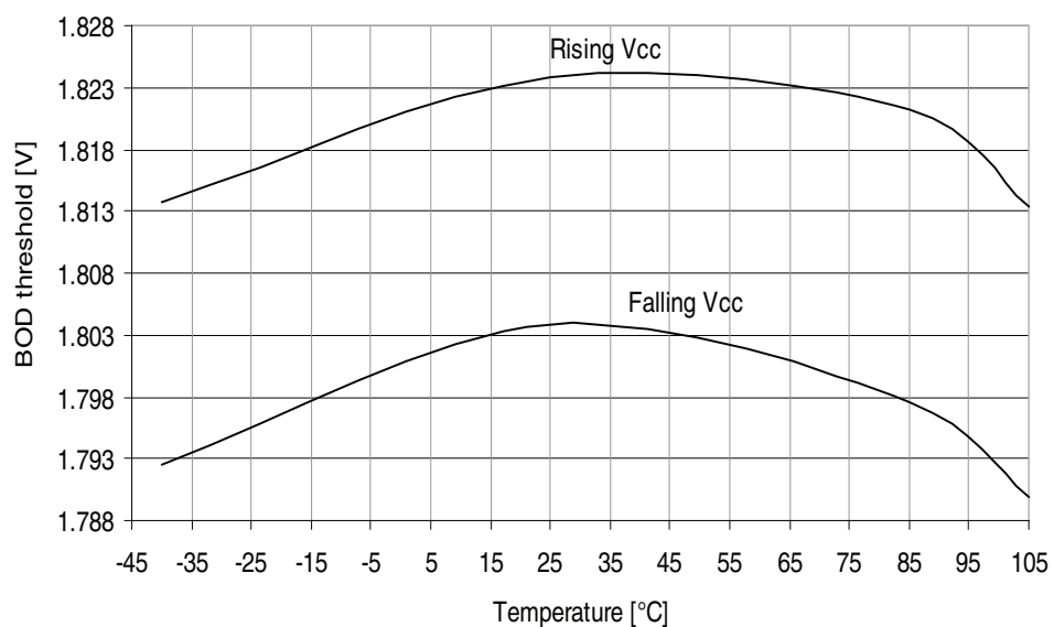
Figure 32-214. ATmega329PA - 105°C: BOD Thresholds vs. Temperature (BOD Level is 1.8V)
