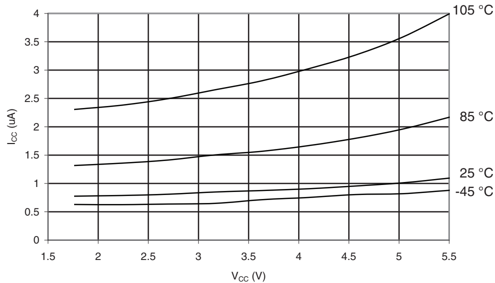
Figure 32-365. ATmega3290PA - 105°C: Standby Supply Current vs. V_{CC} (32kHz Watch Crystal, Watchdog Timer Disabled)
