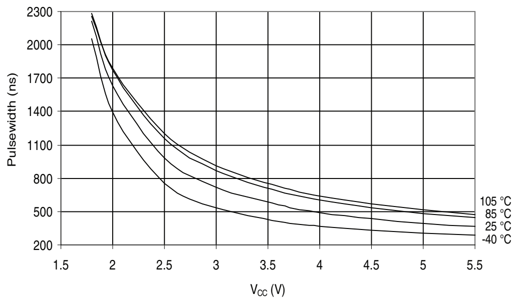
Figure 32-415. ATmega3290PA - 105°C: Minimum Reset Pulse Width vs. V_{CC}
