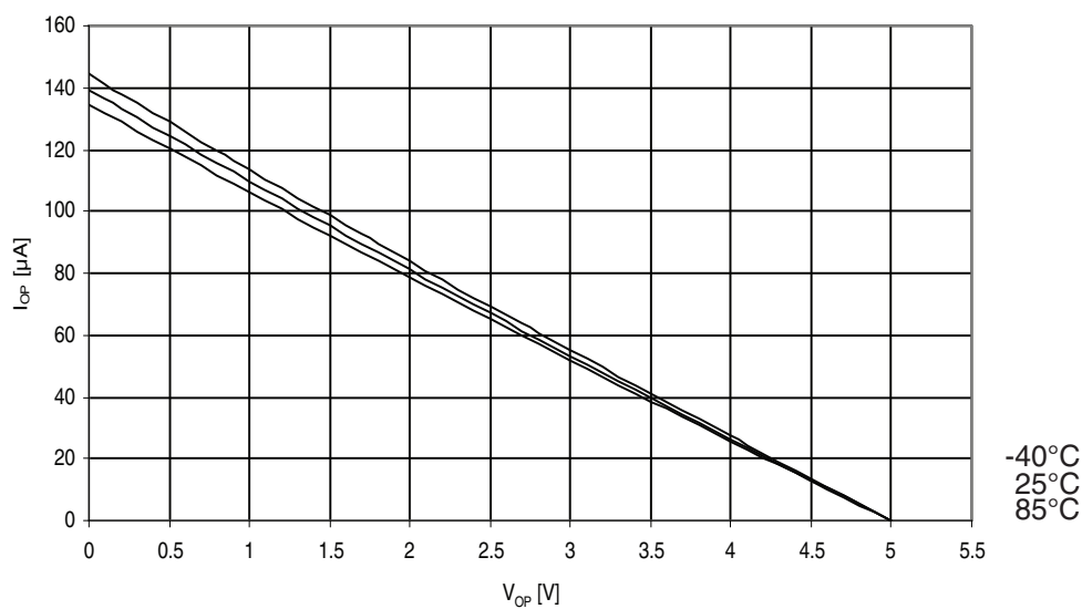
Figure 31-320. Atmel ATmega3290PA: I/O pin pull-up resistor current vs. input voltage ( V_{CC} = 5V ).
