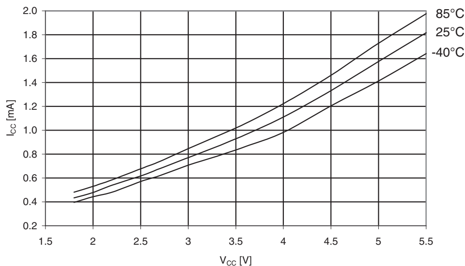
Figure 31-312. ATmega3290PA: Idle supply current vs. V_{CC} (Internal RC oscillator, 8MHz).
