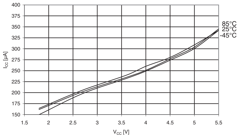
Figure 31-115. Atmel ATmega169PA: Active supply current with ADC at 50kHz vs. V_{CC} .
