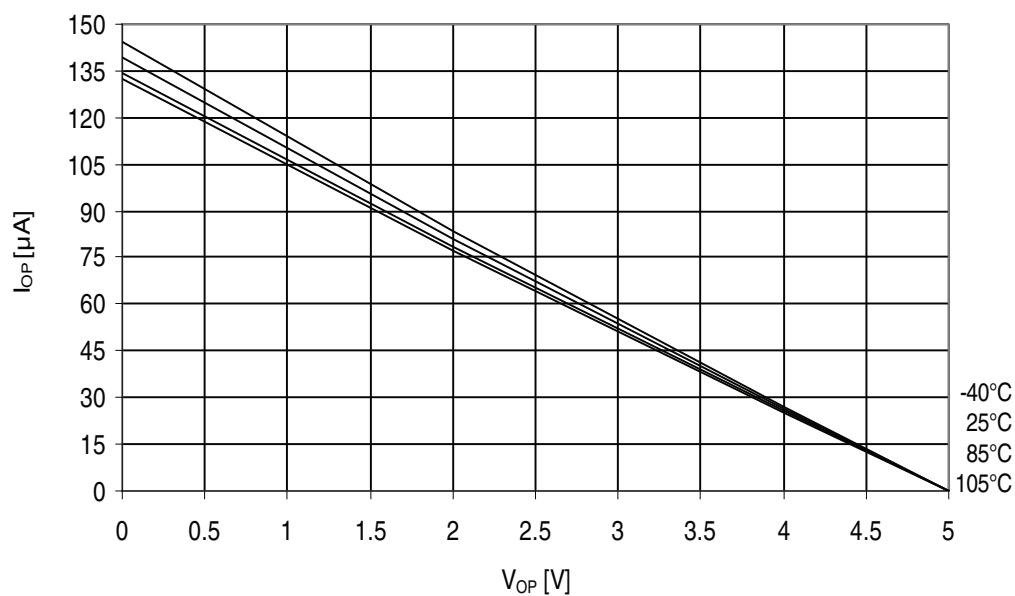
Figure 32-367. ATmega3290PA - 105°C: I/O Pin Pull-up Resistor Current vs. Input Voltage ( V_{CC} = 5V )
