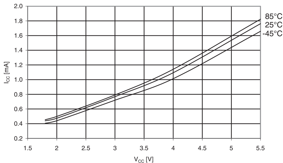
Figure 31-555. ATmega6490P: Idle supply current vs. V_{CC} (Internal RC oscillator, 8MHz).
