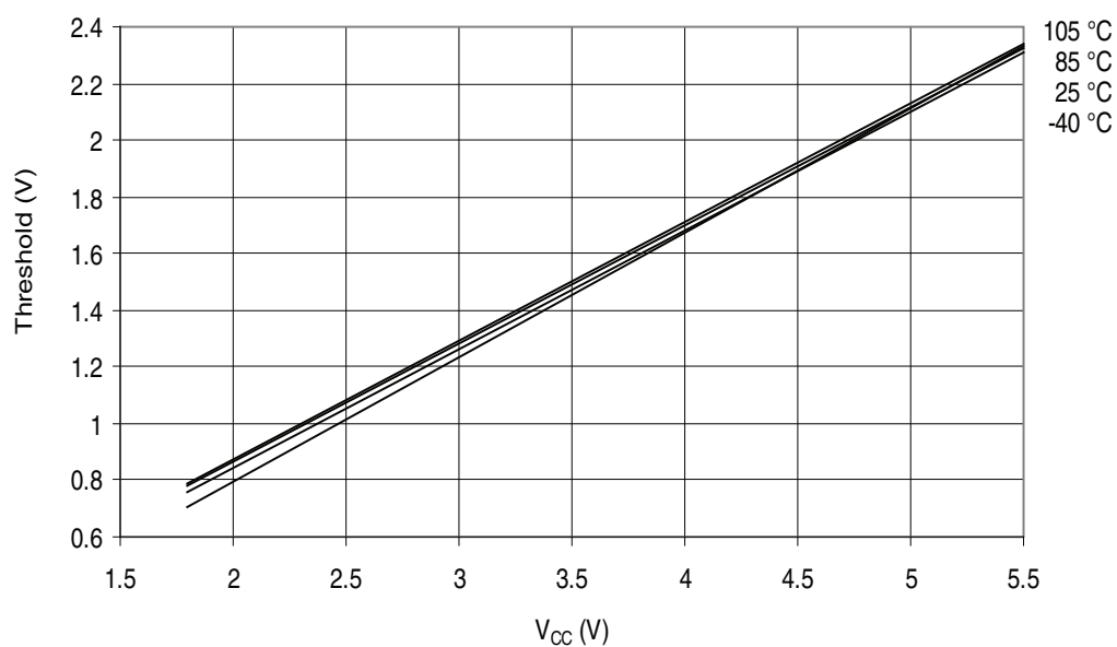
Figure 32-389. ATmega3290PA - 105°C: Reset Input Threshold Voltage vs. V_{CC} ( V_{IL} , Reset Pin Read as “0”)
