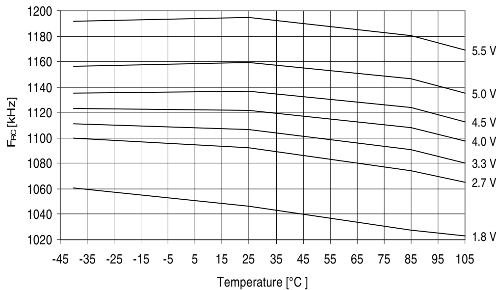
Figure 32-102. ATmega329A - 105°C: Watchdog Oscillator Frequency vs. Temperature
