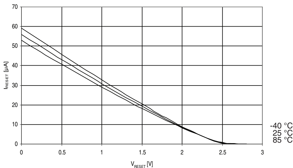
Figure 31-264. ATmega3290A: Reset pull-up resistor current vs. reset pin voltage ( V_{CC} = 2.7V ).
