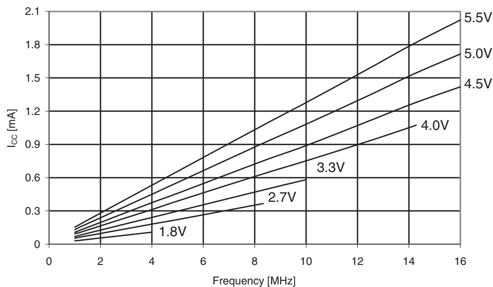
Figure 31-123. Atmel ATmega169PA: Reset supply current vs. V_{CC} (1 - 16MHz, excluding current through the reset pull-up).
