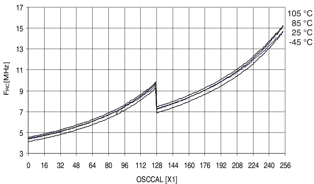
Figure 32-223. ATmega329PA - 105°C: Calibrated 8MHz RC Oscillator Frequency vs. Oscal Value
