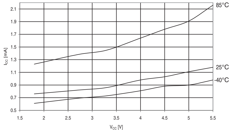
Figure 31-257. Atmel ATmega3290A: Power-save supply current vs. V_{CC} (Watchdog Timer disabled and 32kHz XTAL oscillator running).
