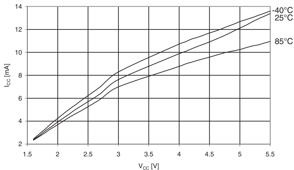
Figure 31-301. Atmel ATmega3290A: Programming current vs. V_{CC} .
