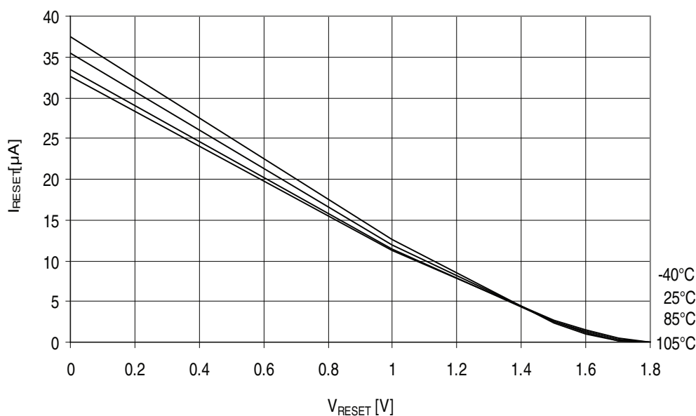
Figure 32-256. ATmega3290A - 105°C: Reset Pull-up Resistor Current vs. Reset Pin Voltage ( V_{CC} = 1.8V )
