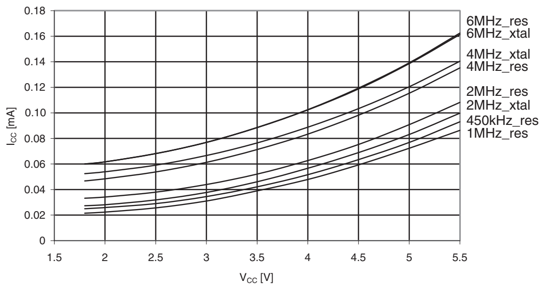
Figure 31-77. Atmel ATmega169PA: Standby supply current vs. V_{CC} (XTAL and Resonator, Watchdog Timer disabled).
