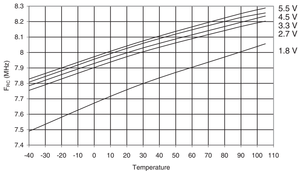
Figure 32-162. ATmega329P-105°C: Calibrated RC Oscillator Frequency vs. Temperature
