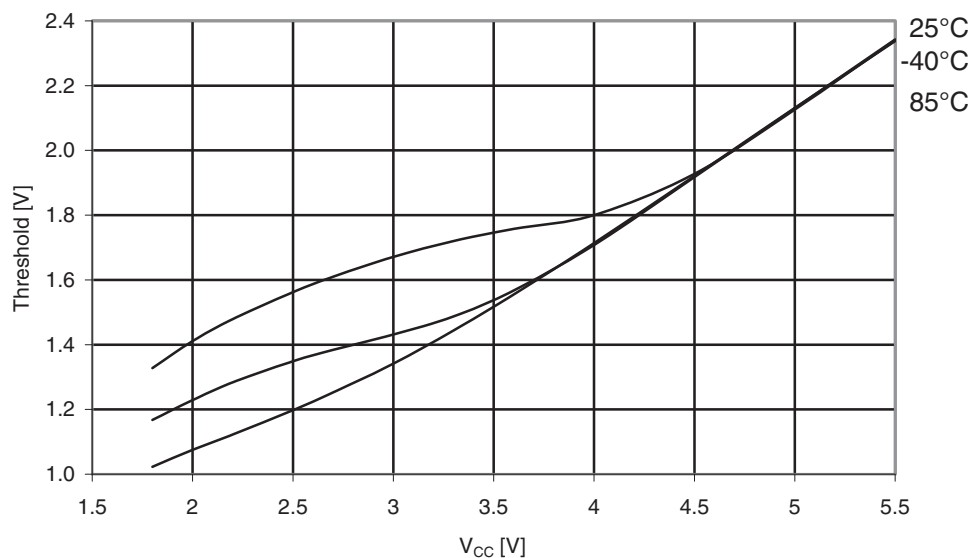
Figure 31-221. Atmel ATmega329PA: Reset Input Threshold voltage vs. V_{CC} ( V_{IH} , reset pin read as “1”).
