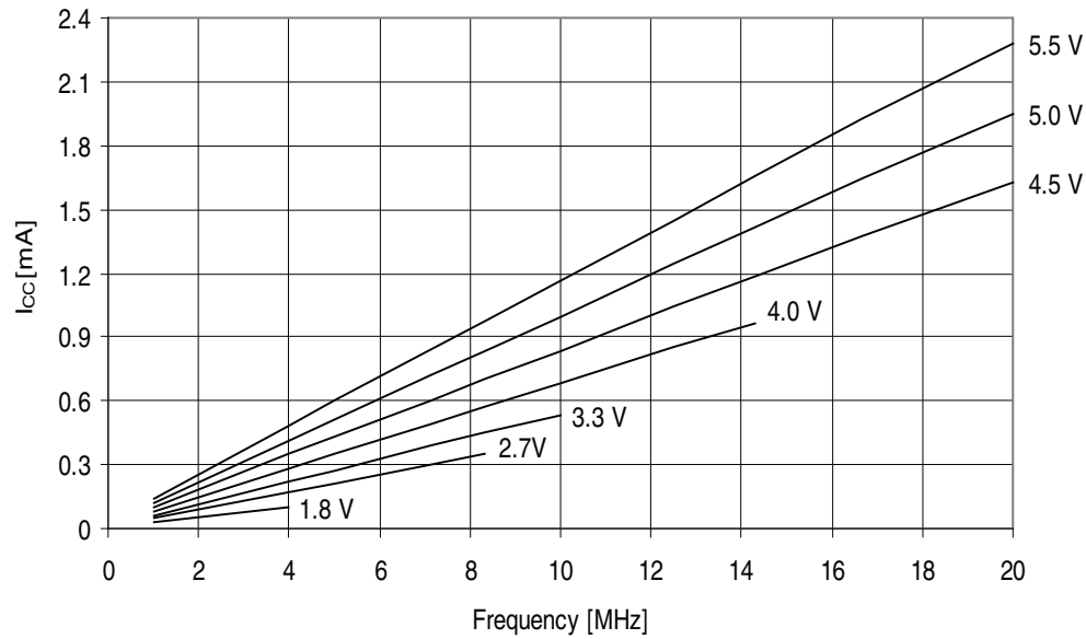
Figure 32-234. ATmega329PA - 105°C: Reset Supply Current vs. V_{CC} (1 - 20MHz, Excluding Current Through The Reset Pull-up)
