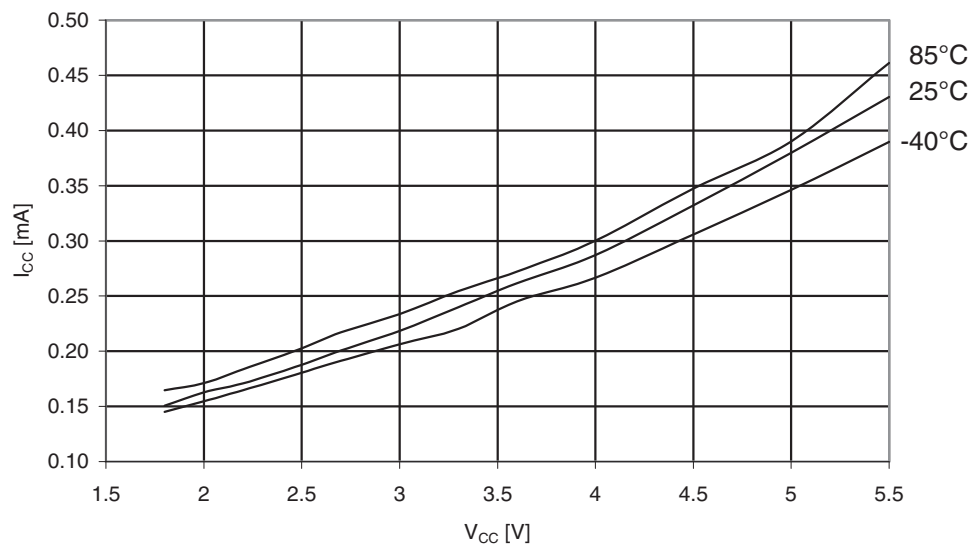
Figure 31-193. Atmel ATmega329PA: Idle supply current vs. V_{CC} (Internal RC oscillator, 1MHz).
