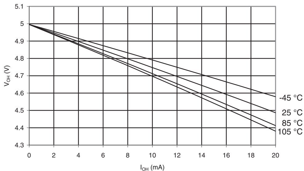
Figure 32-24. ATmega169PA-105°C: I/O Pin Output Voltage vs. Source Current, Port B ( V_{CC} = 5V )
