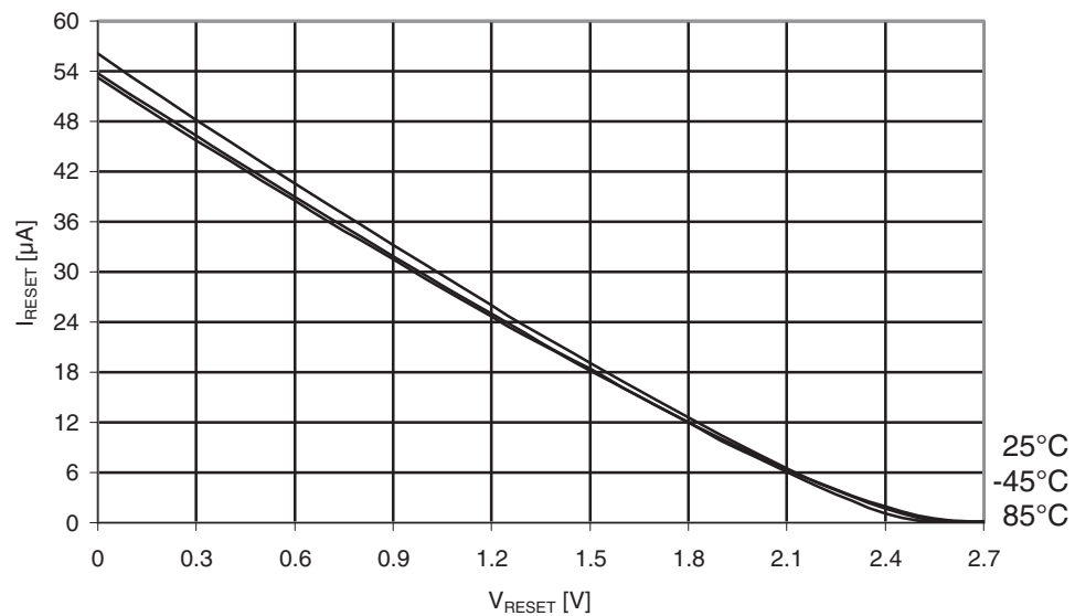
Figure 31-568. Atmel ATmega6490P: Reset pull-up resistor current vs. reset pin voltage ( V_{CC} = 2.7V ).
