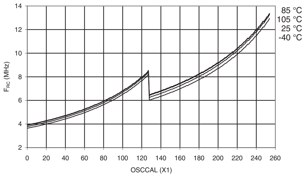
Figure 32-164. ATmega329P-105°C: Calibrated RC Oscillator Frequency vs. Oscal Value
