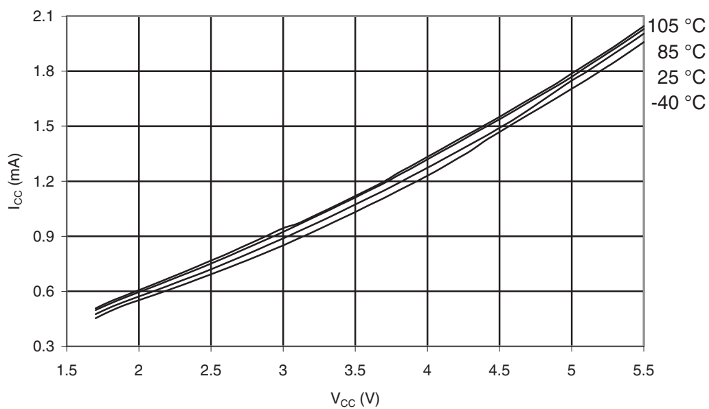
Figure 32-303. ATmega3290PA-105°C: Active Supply Current vs. V_{CC} (Internal RC Oscillator, 1MHz)
