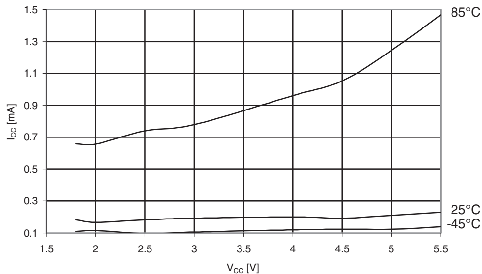
Figure 31-499. Atmel ATmega6490A: Power-down supply current vs. V_{CC} (32kHz watch XTAL).
