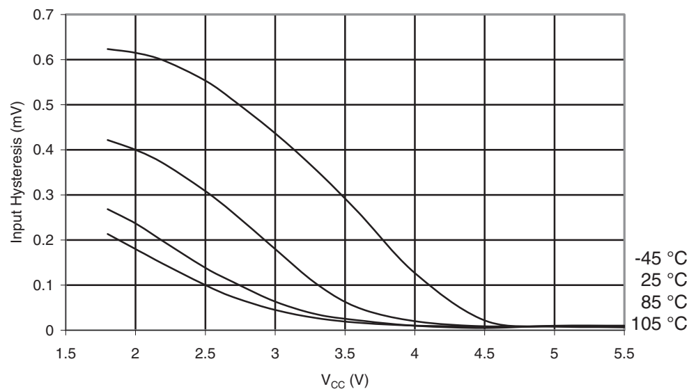
Figure 32-38. ATmega169PA-105°C: Reset Input Pin Hysteresis vs. V_{CC}
