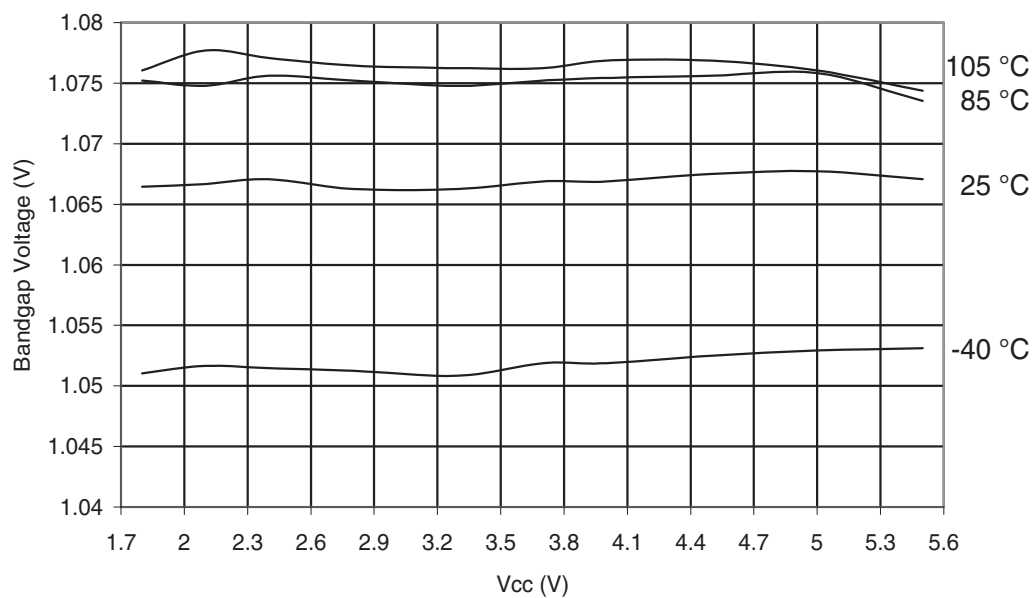
Figure 32-337. ATmega3290PA-105°C: Bandgap Voltage vs. V_{CC}
