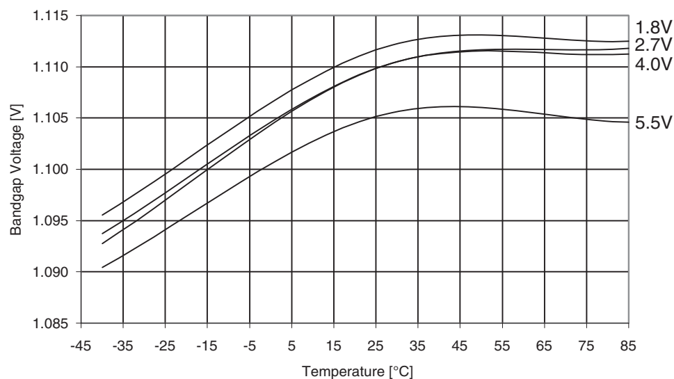
Figure 31-288. ATmega3290A: Bandgap voltage vs. temperature.
