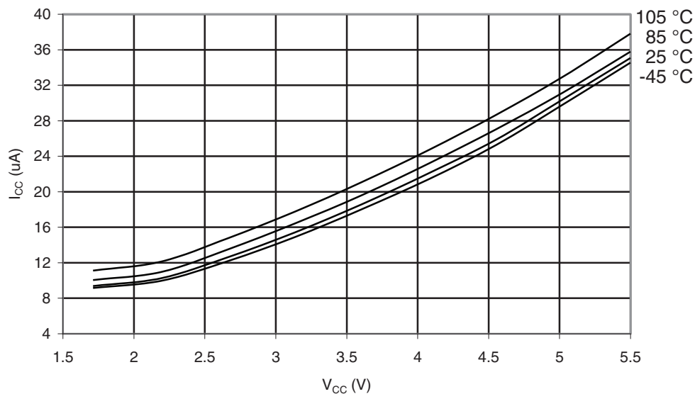
Figure 32-178. ATmega329PA: Active Supply Current vs. V_{CC} (32kHz Watch Crystal)
