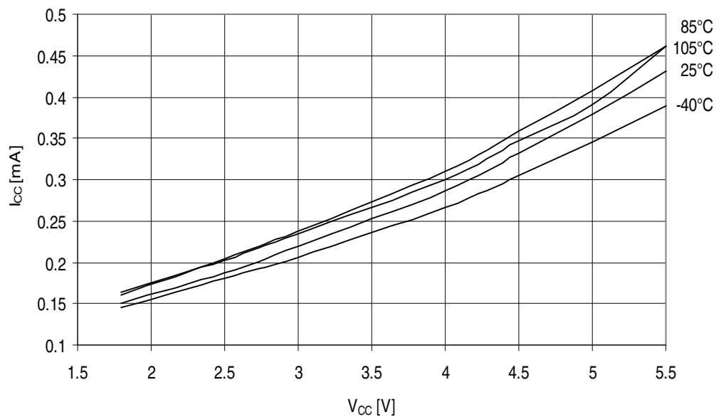
Figure 32-68. ATmega329A - 105°C: Idle Supply Current vs. V_{CC} (32kHz Watch Crystal)
