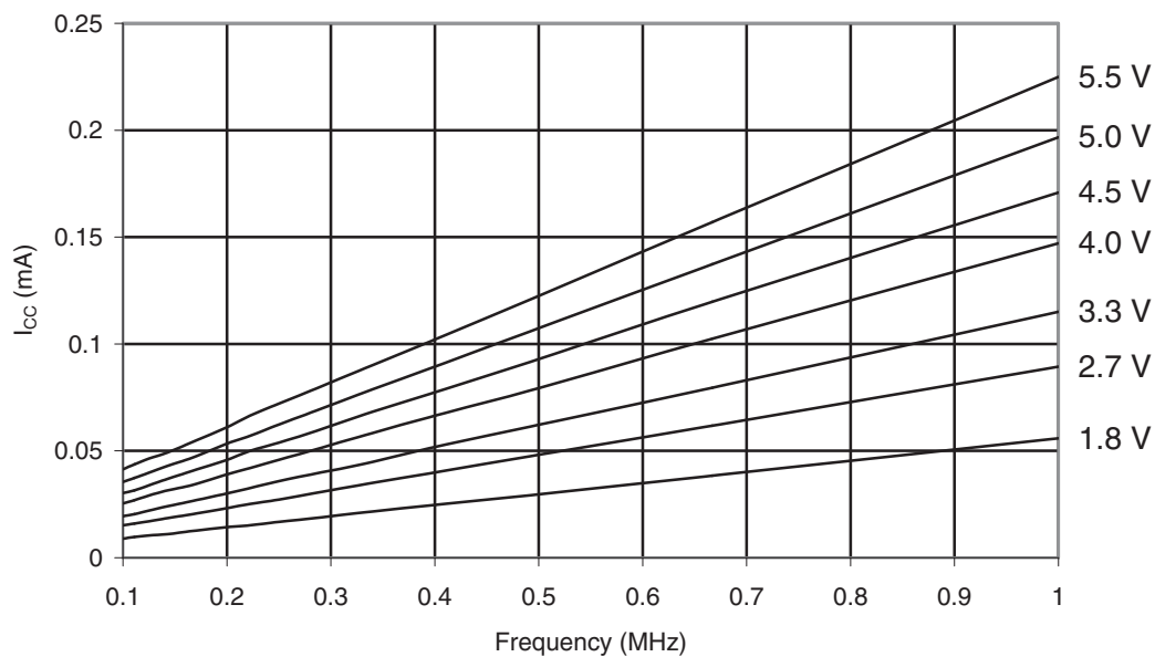
Figure 32-349. ATmega3290PA-105°C: Reset Supply Current vs. V_{CC} (0.1 - 1.0 MHz, Excluding Current Through The Reset Pull-up)
