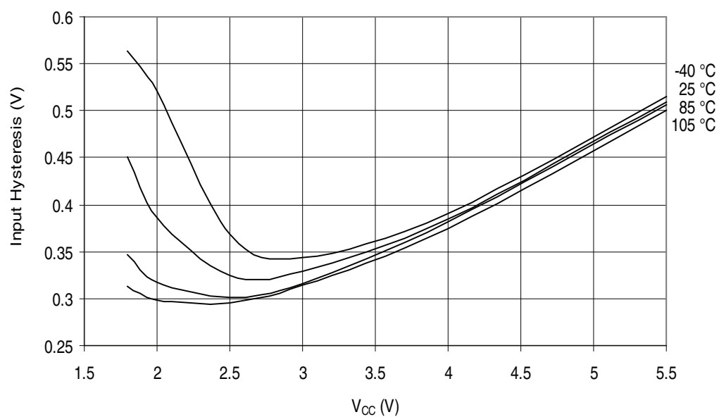
Figure 32-387. ATmega3290PA - 105°C: I/O Pin Input Hysteresis vs. V_{CC}
