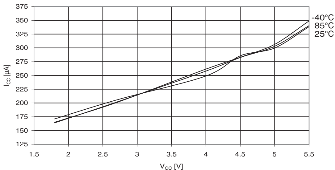
Figure 31-177. Atmel ATmega329A: Active supply current with ADC at 1MHz vs. V_{CC} .
