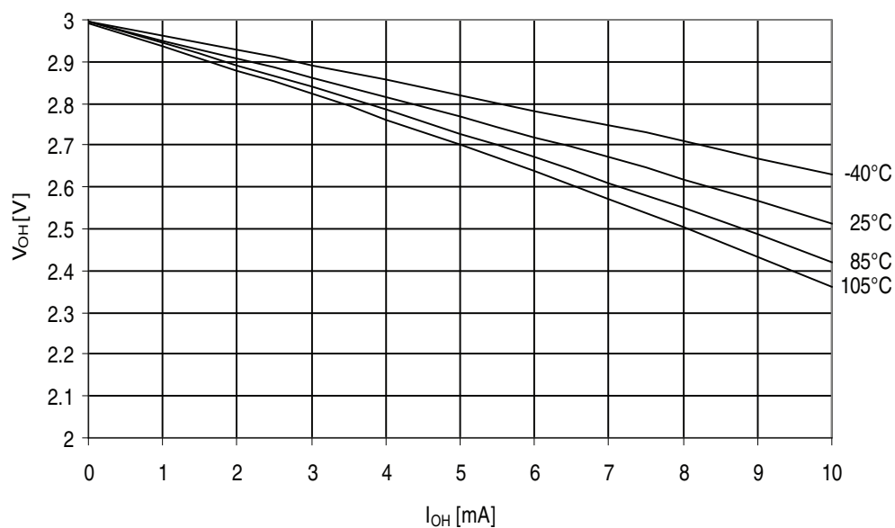
Figure 32-80. ATmega329A - 105°C: I/O Pin Output Voltage vs. Source Current, Ports A, C, D, E, F, G ( V_{CC} = 3V )
