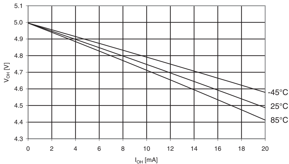
Figure 31-25. Atmel ATmega169A: I/O pin output voltage vs. source current, port B ( V_{CC} = 5V ).
