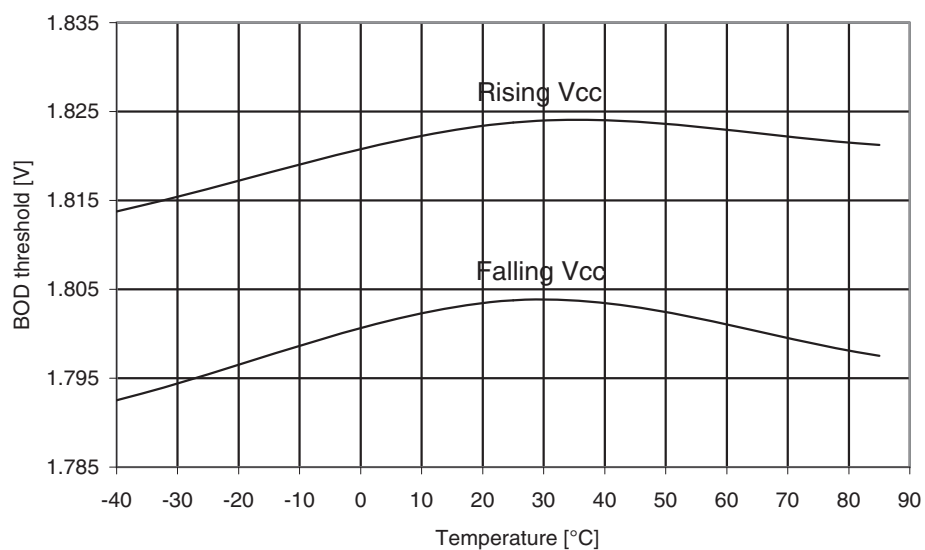
Figure 31-346. Atmel ATmega3290PA: BOD Thresholds vs. temperature (BOD level is 1.8V).
