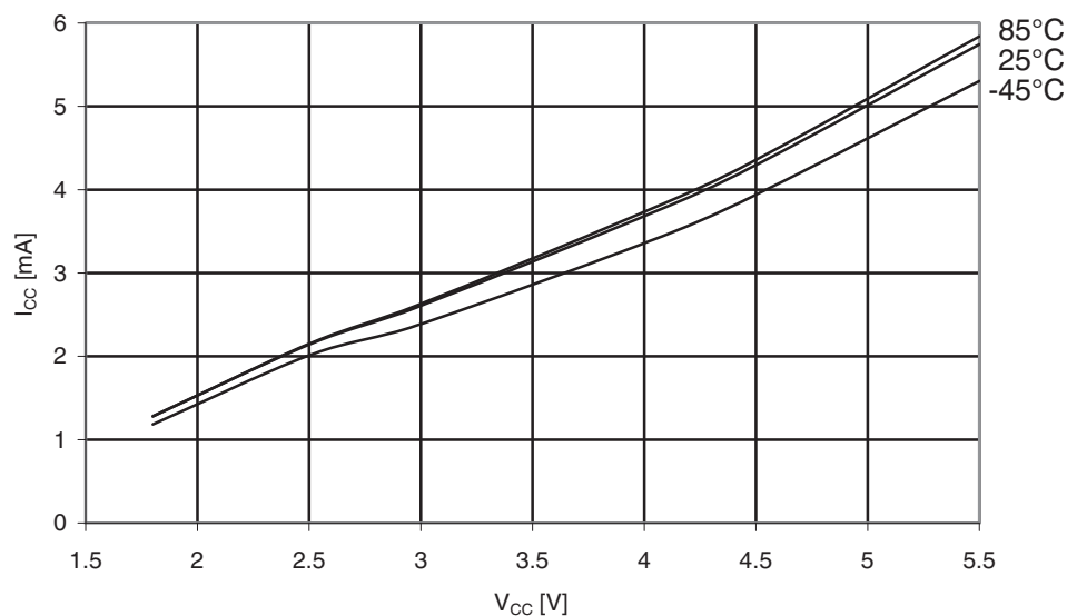
Figure 31-65. Atmel ATmega169PA: Active supply current vs. V_{CC} (Internal RC oscillator, 8MHz).
