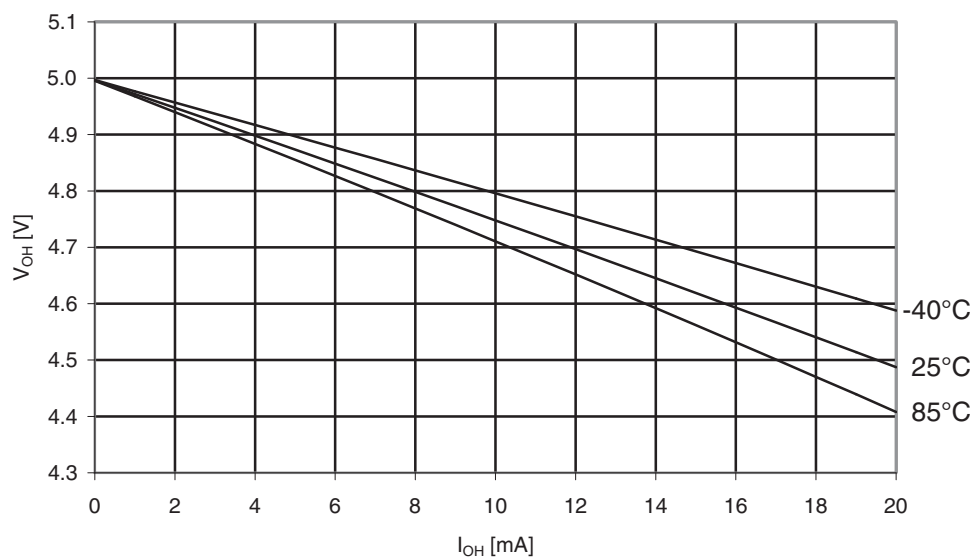
Figure 31-149. Atmel ATmega329A: I/O pin output voltage vs. source current, port B ( V_{CC} = 5V ).
