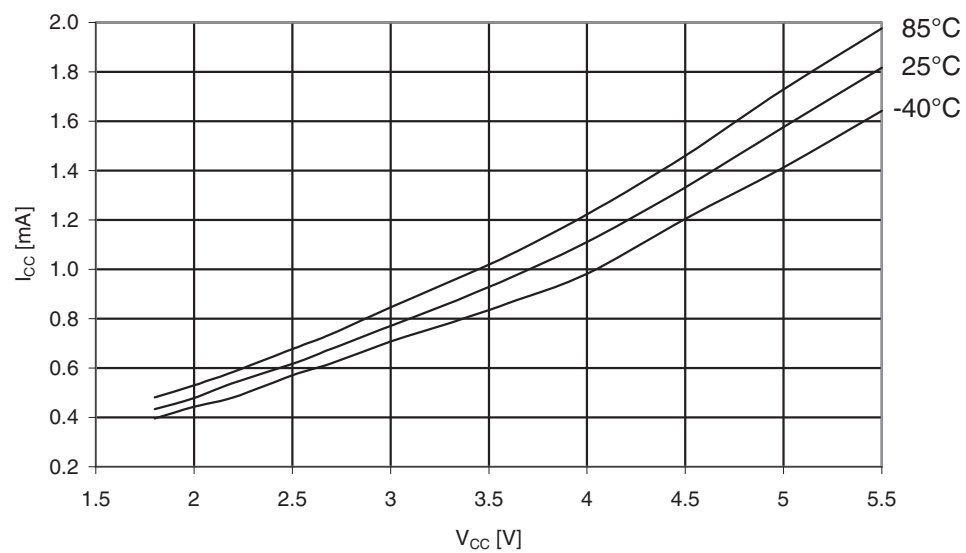
Figure 31-132. ATmega329A: Idle supply current vs. V_{CC} (Internal RC oscillator, 8MHz).
