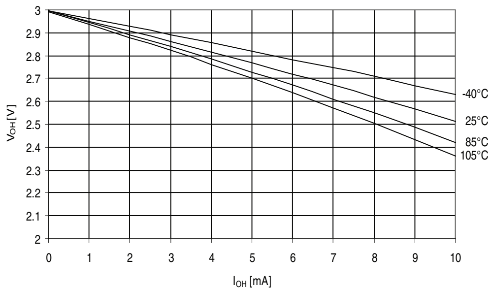
Figure 32-258. ATmega3290A - 105°C: I/O Pin Output Voltage vs. Source Current, Ports A, C, D, E, F, G ( V_{CC} = 3V )
