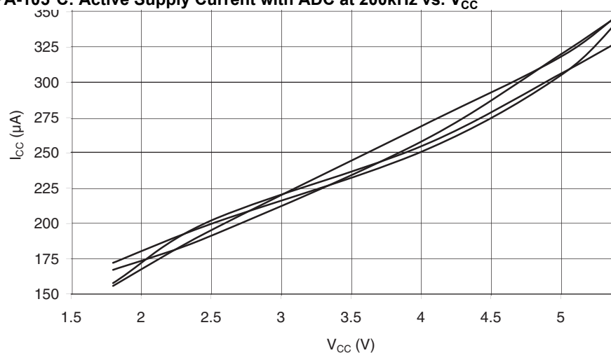
Figure 32-50. ATmega169PA-105°C: Active Supply Current with ADC at 200kHz vs. V_{CC}
