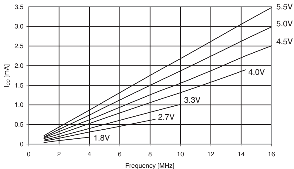
Figure 31-69. Atmel ATmega169PA: Idle supply current vs. frequency (1 - 16MHz).
