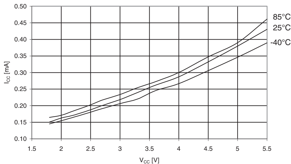
Figure 31-133. Atmel ATmega329A: Idle supply current vs. V_{CC} (Internal RC oscillator, 1MHz).
