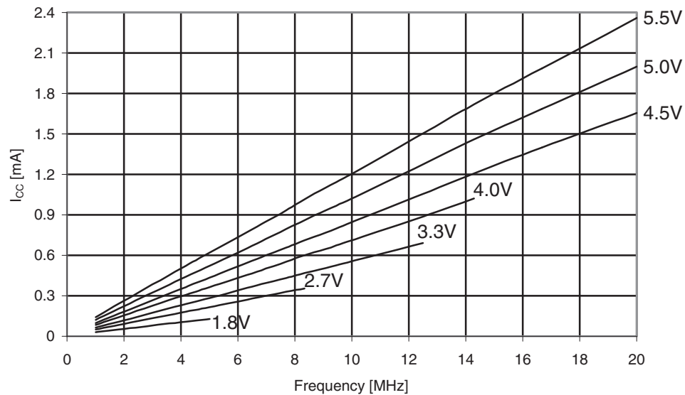
Figure 31-546. ATmega6490A: Reset supply current vs. V_{CC} (1 - 20MHz, excluding current through the reset pull-up).
