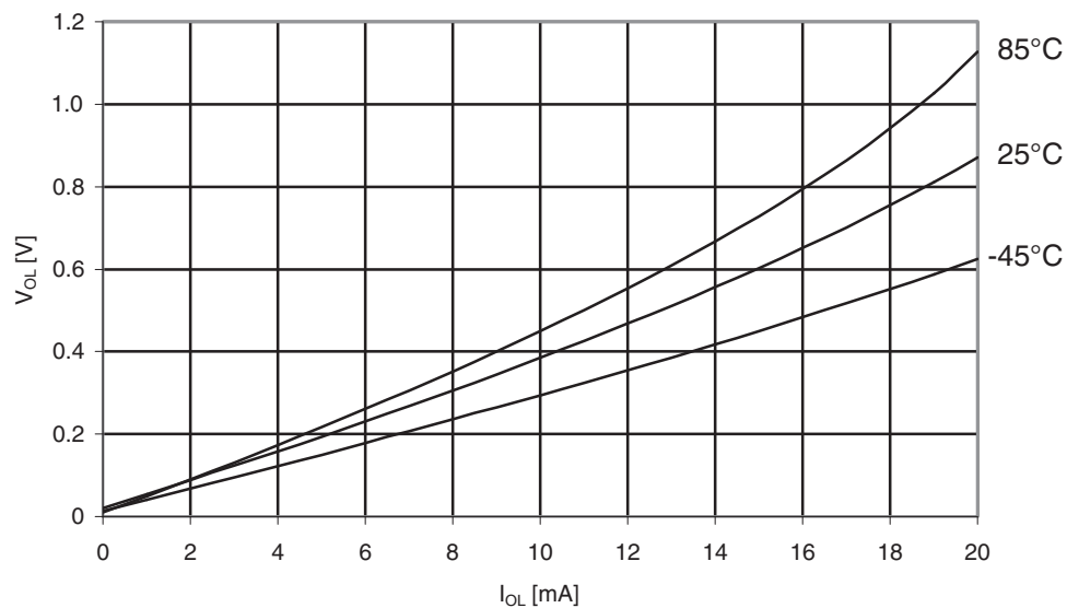
Figure 31-458. Atmel ATmega649P: I/O pin output voltage vs. sink current, port B ( V_{CC} = 2.7V ).
