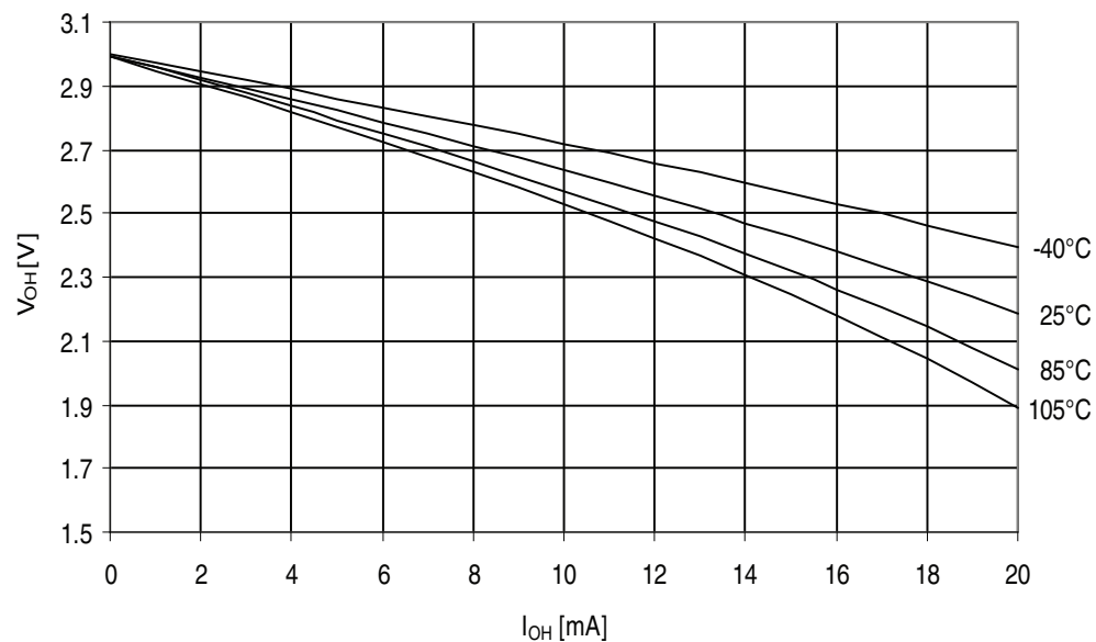
Figure 32-261. ATmega3290A - 105°C: I/O Pin Output Voltage vs. Source Current, Port B ( V_{CC} = 3V )
