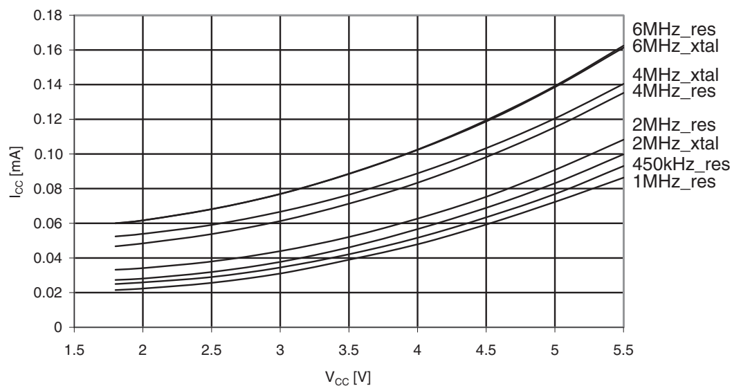
Figure 31-15. Atmel ATmega169A: Standby supply current vs. V_{CC} (XTAL and resonator, Watchdog Timer disabled).
