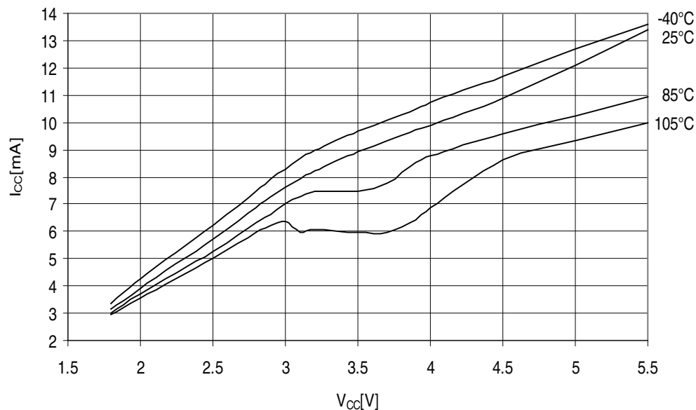
Figure 32-232. ATmega329PA - 105°C: Programming Current vs. V_{CC}
