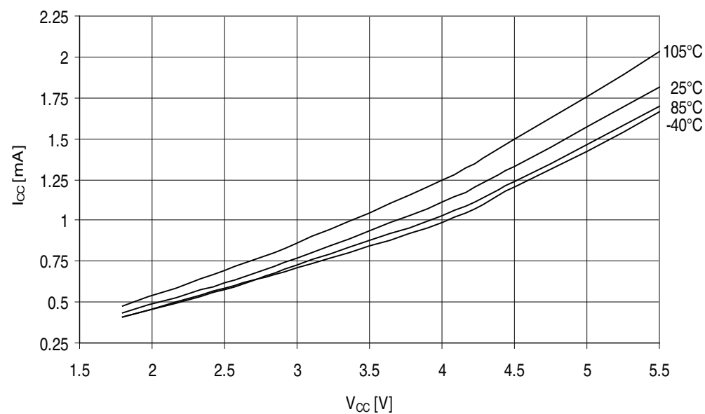
Figure 32-359. ATmega3290PA - 105°C: Idle Supply Current vs. V_{CC} (Internal RC Oscillator, 8 MHz)
