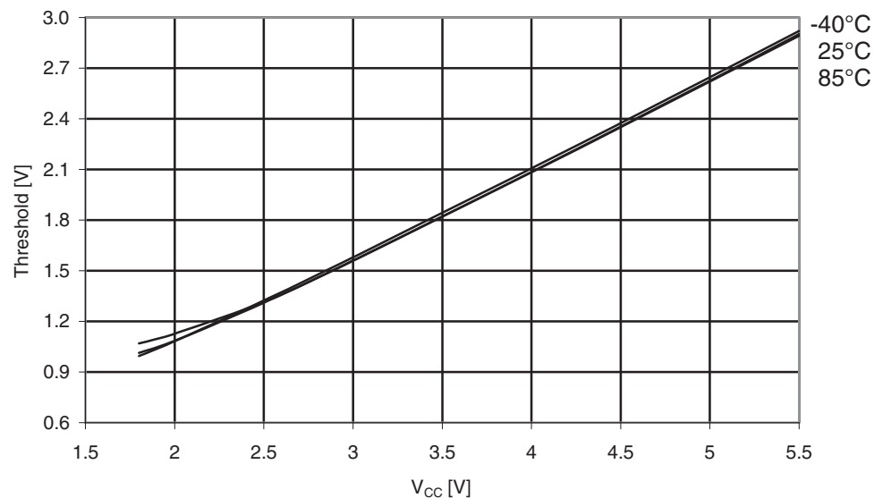
Figure 31-338. Atmel ATmega3290PA: I/O pin Input Threshold voltage vs. V_{CC} ( V_{IH} , I/O pin read as "1").
