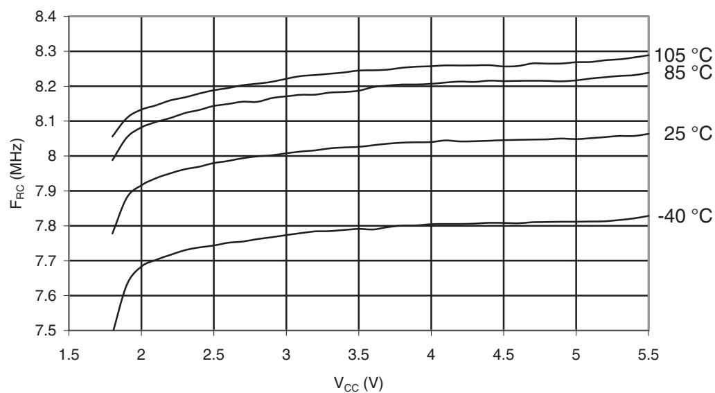
Figure 32-341. ATmega3290PA-105°C: Calibrated RC Oscillator Frequency vs. V_{CC}
