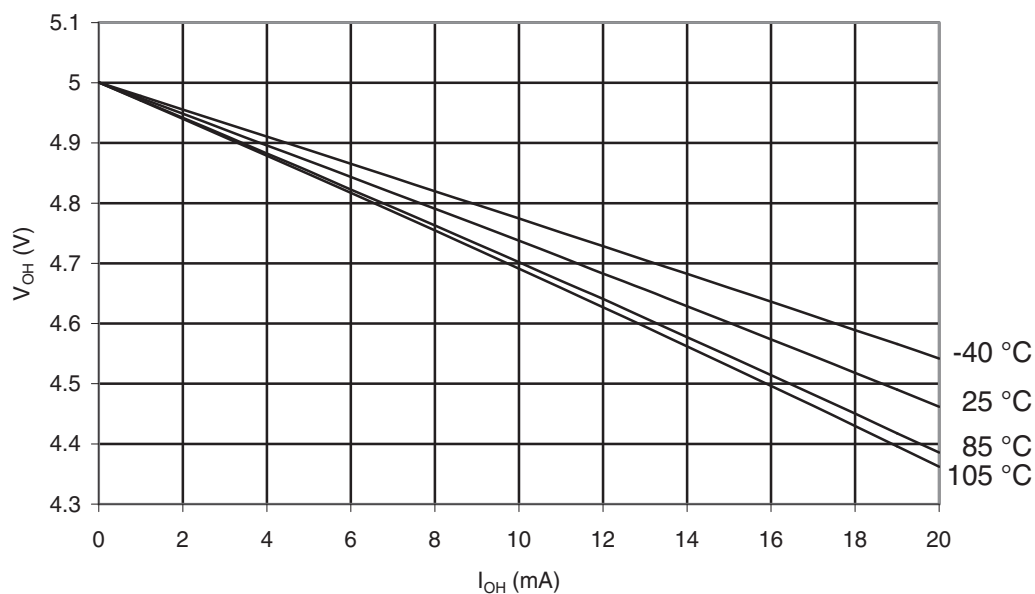
Figure 32-142. ATmega329P-105°C: I/O Pin Output Voltage vs. Source Current, Ports A,C,D,E,F,G ( V_{CC} = 5V )
