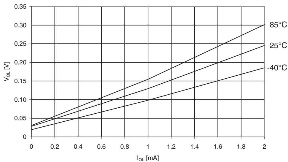
Figure 31-154. ATmega329A: I/O pin output voltage vs. sink current, ports A, C, D, E, F, G ( V_{CC} = 1.8V ).
