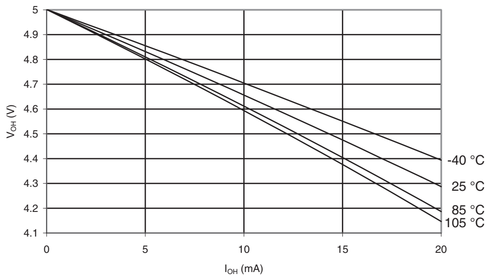
Figure 32-144. ATmega329P-105°C: I/O Pin Output Voltage vs. Source Current, Port B ( V_{CC} = 5V )
