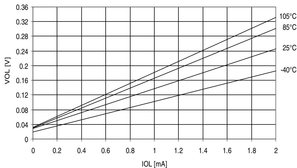
Figure 32-381. ATmega3290PA - 105°C: I/O Pin Output Voltage vs. Sink Current, Ports A, C, D, E, F, G ( V_{CC} = 1.8V )
