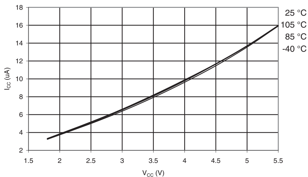
Figure 32-346. ATmega3290PA-105°C: Watchdog Timer Current vs. V_{CC}
