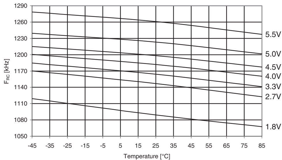
Figure 31-533. Atmel ATmega6490A: Watchdog Oscillator frequency vs. temperature.
