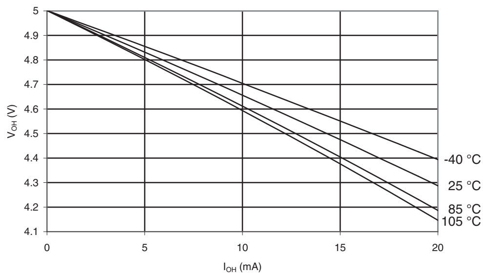
Figure 32-322. ATmega3290PA-105°C: I/O Pin Output Voltage vs. Source Current, Port B ( V_{CC} = 5V )
