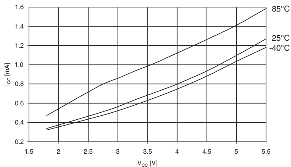
Figure 31-128. ATmega329A: Active supply current vs. V_{CC} (Internal RC oscillator, 1MHz).
