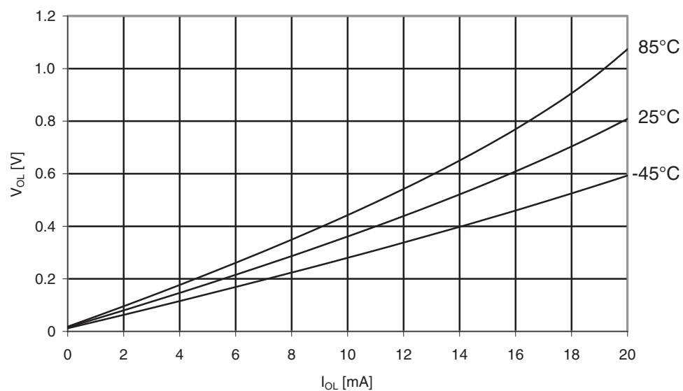
Figure 31-94. ATmega169PA: I/O pin output voltage vs. Sink current, port B ( V_{CC} = 2.7V ).
