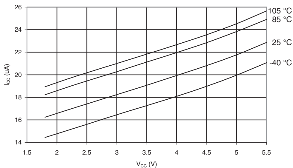
Figure 32-165. ATmega329P-105°C: Brownout Detector Current vs. V_{CC}
