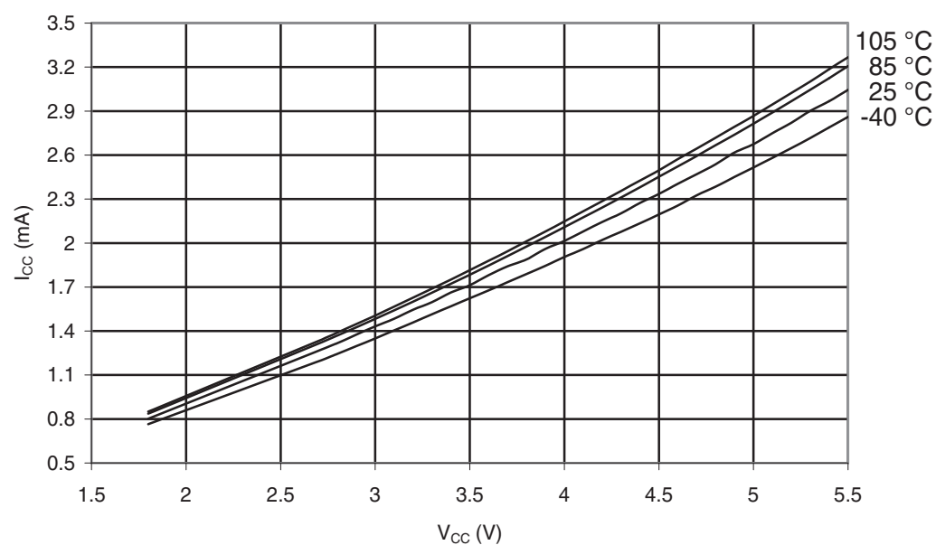
Figure 32-307. ATmega3290PA-105°C: Idle Supply Current vs. V_{CC} (Internal RC Oscillator, 8MHz)
