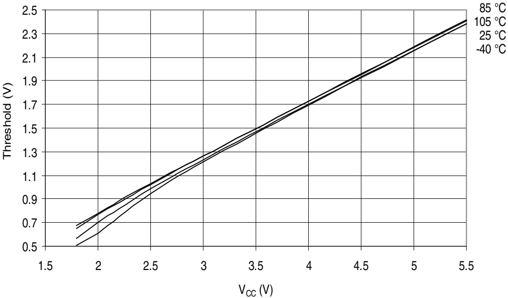
Figure 32-270. ATmega3290A - 105°C: I/O Pin Input Threshold Voltage vs. V_{CC} ( V_{IL} , I/O Pin Read as “0”)
