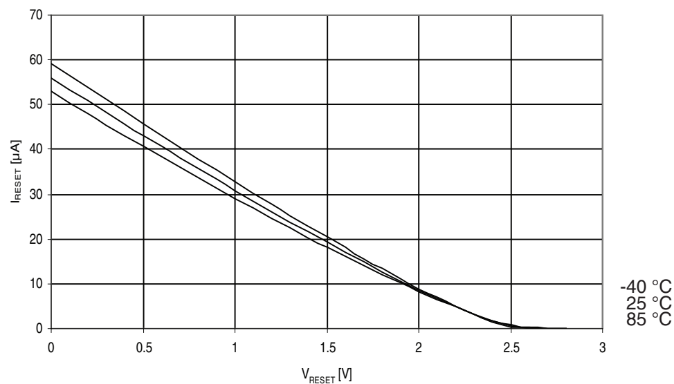
Figure 31-204. ATmega329PA: Reset pull-up resistor current vs. reset pin voltage ( V_{CC} = 2.7V ).
