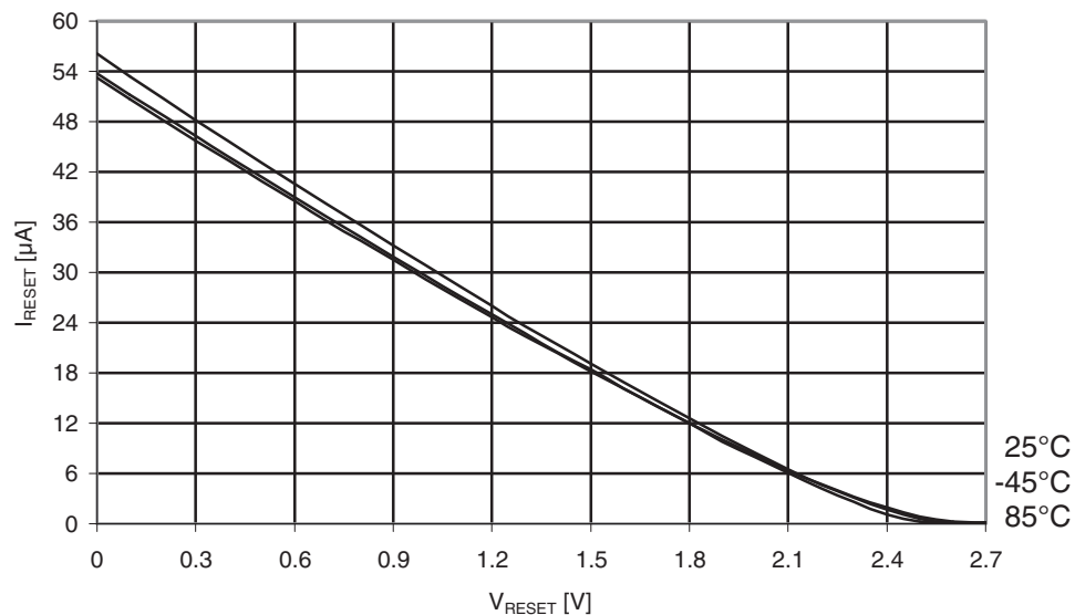
Figure 31-446. Atmel ATmega649P: Reset pull-up resistor current vs. reset pin voltage ( V_{CC} = 2.7V ).
