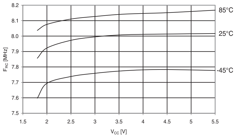
Figure 31-112. ATmega169PA: Calibrated 8MHz RC oscillator frequency vs. V_{CC} .
