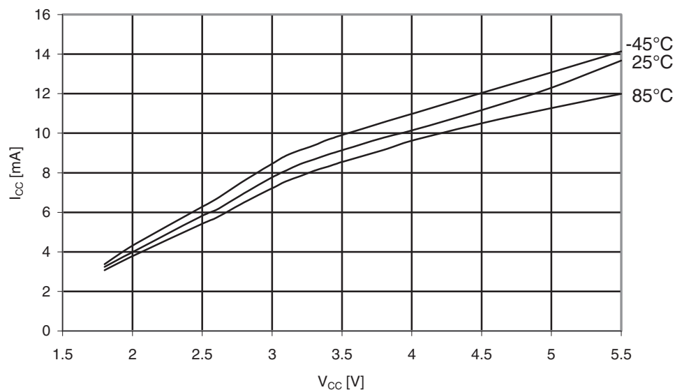
Figure 31-121. Atmel ATmega169PA: Programming current vs. V_{CC} .
