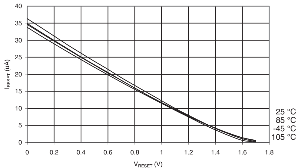
Figure 32-20. ATmega169PA-105°C: Reset Pull-up Resistor Current vs. Reset Pin Voltage ( V_{CC} = 1.8V )
