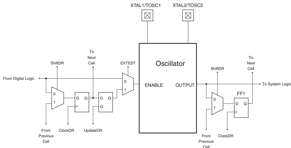
Figure 26-5. Boundary-scan cells for oscillators and clock options.
