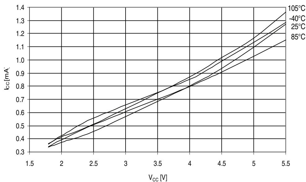
Figure 32-177. ATmega329PA - 105°C: Active Supply Current vs. V_{CC} (Internal RC Oscillator, 1MHz)
