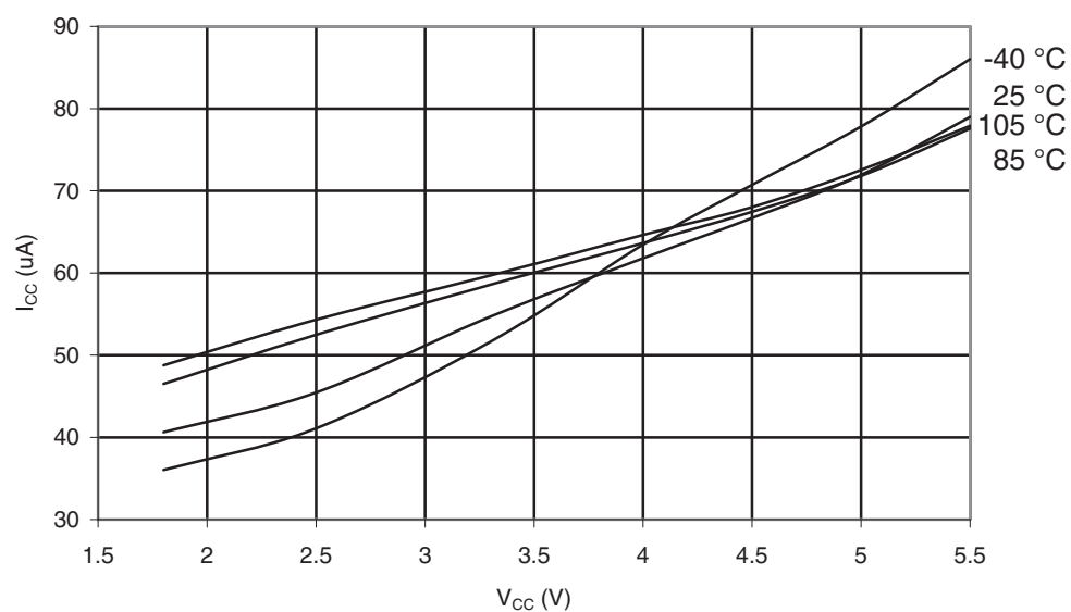
Figure 32-169. ATmega329P-105°C: Analog Comparator Current vs. V_{CC}
