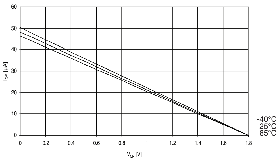
Figure 31-322. Atmel ATmega3290PA: I/O pin pull-up resistor current vs. input voltage ( V_{CC} = 1.8V ).
