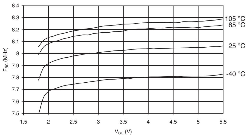
Figure 32-163. ATmega329P-105°C: Calibrated RC Oscillator Frequency vs. V_{CC}
