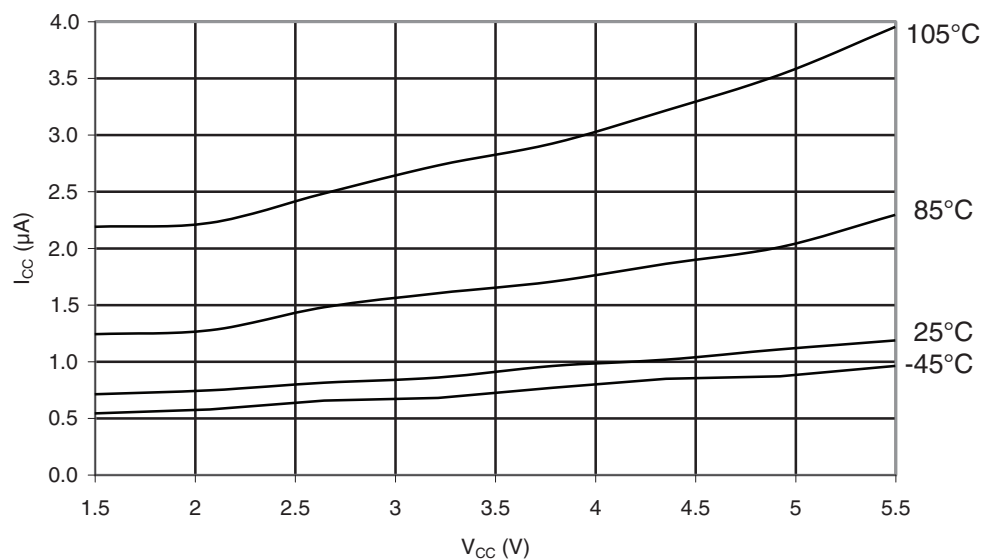
Figure 32-186. ATmega329PA - 105°C: Power-save Supply Current vs. V_{CC} (Watchdog Timer Disabled)
