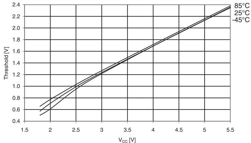
Figure 31-522. ATmega6490A: I/O pin input Threshold voltage vs. V_{CC} ( V_{IL} , I/O pin read as “0”).
