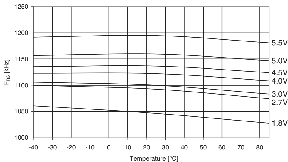
Figure 31-230. ATmega329PA: Watchdog Oscillator frequency vs. temperature.
