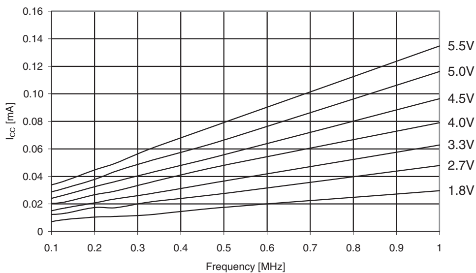
Figure 31-302. ATmega3290A: Reset supply current vs. V_{CC} (0.1 - 1.0MHz, excluding current through the reset pull-up).
