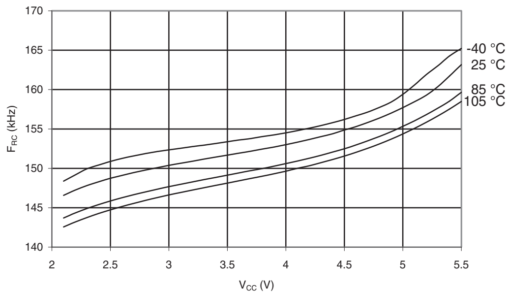
Figure 32-161. ATmega329P-105°C: Watchdog Oscillator Frequency vs. V_{CC}
