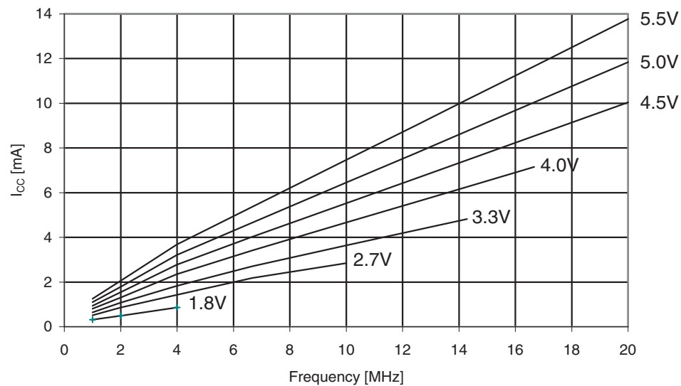
Figure 31-306. ATmega3290PA: Active supply current vs. frequency (1 - 20MHz).
