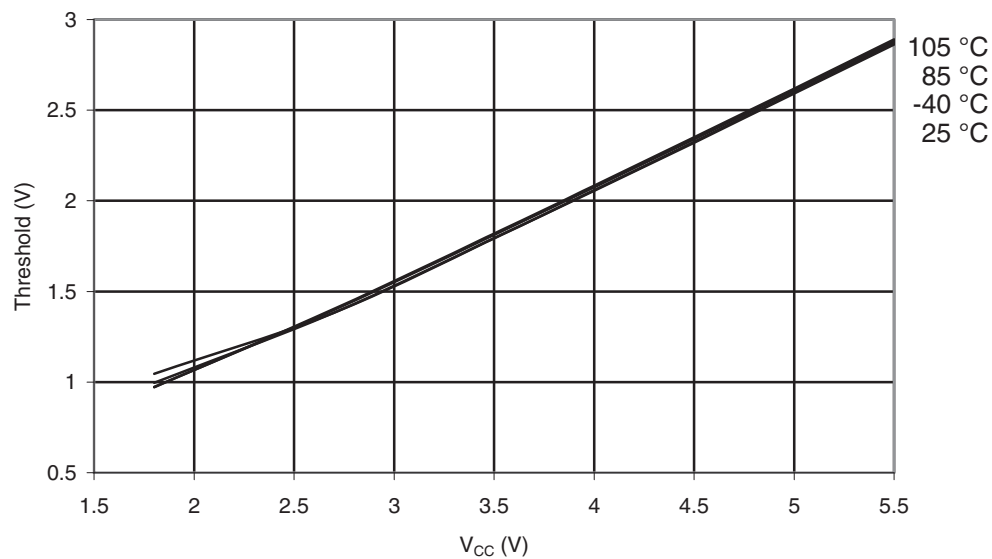
Figure 32-328. ATmega3290PA-105°C: I/O Pin Input Threshold Voltage vs. V_{CC} ( V_{IH} , I/O Pin Read as “1”)
