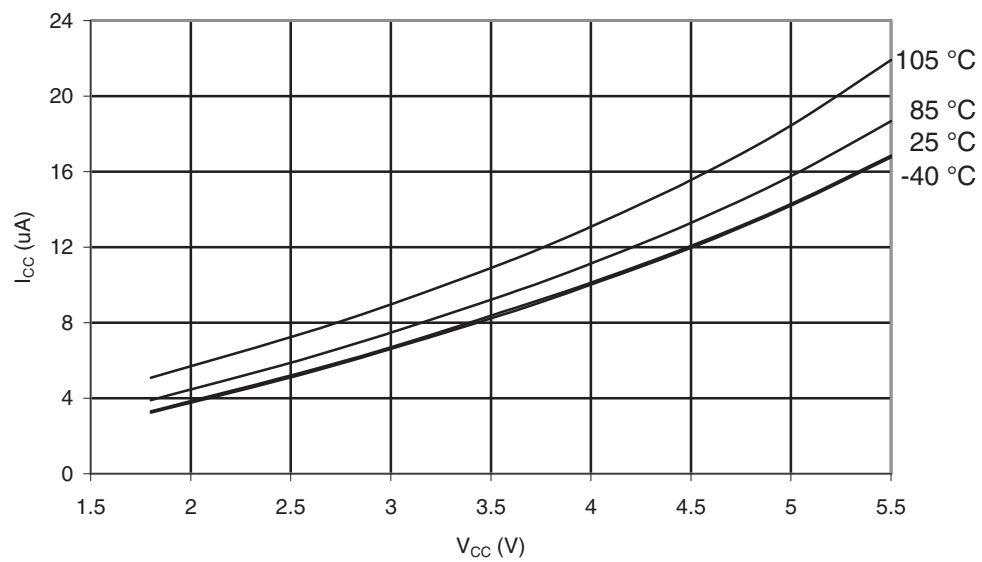
Figure 32-133. ATmega329P-105°C: Power-down Supply Current vs. V_{CC} (Watchdog Timer Enabled)
