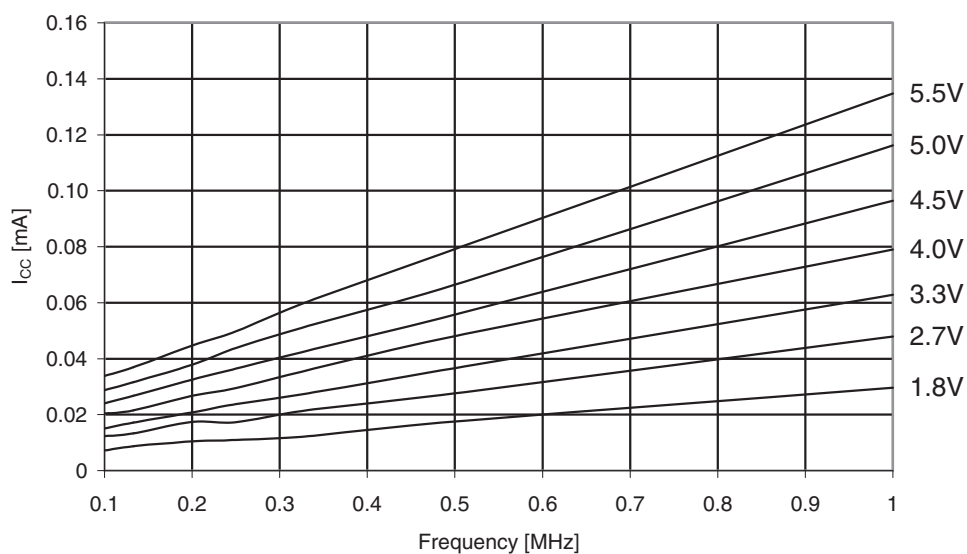
Figure 31-182. ATmega329A: Reset supply current vs. V_{CC} (0.1 - 1.0MHz, excluding current through the reset pull-up).
