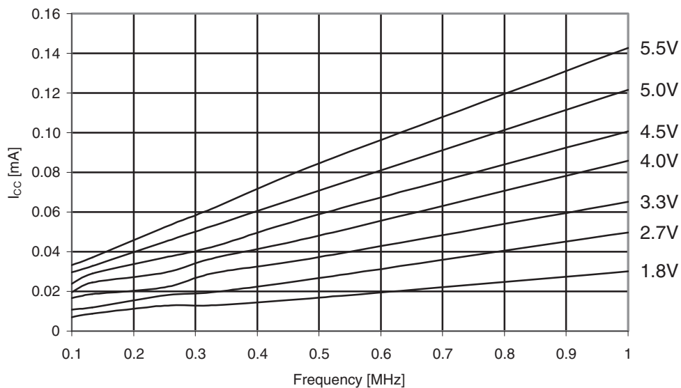
Figure 31-606. Atmel ATmega6490P: Reset supply current vs. V_{CC} (0.1 - 1.0MHz, excluding current through the reset pull-up).
