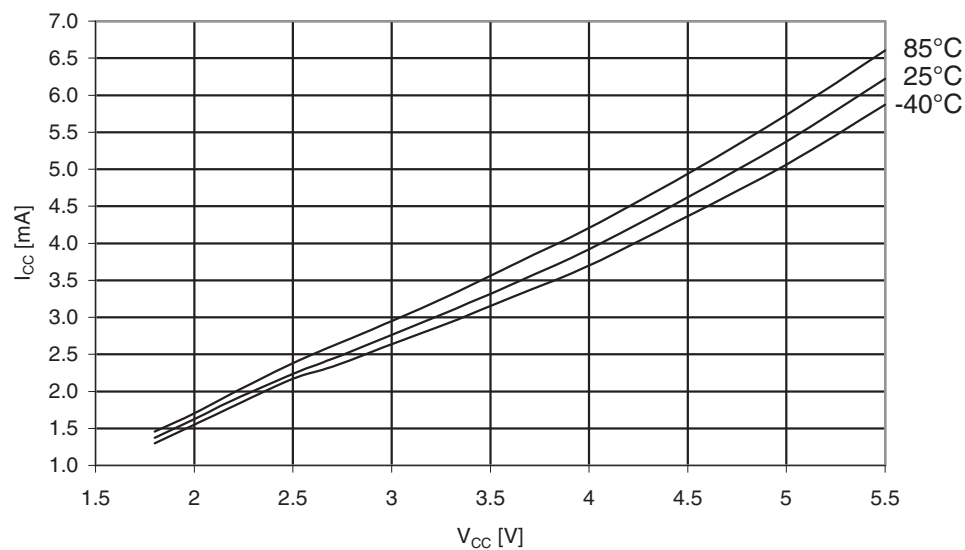
Figure 31-187. Atmel ATmega329PA: Active supply current vs. V_{CC} (Internal RC oscillator, 8MHz).
