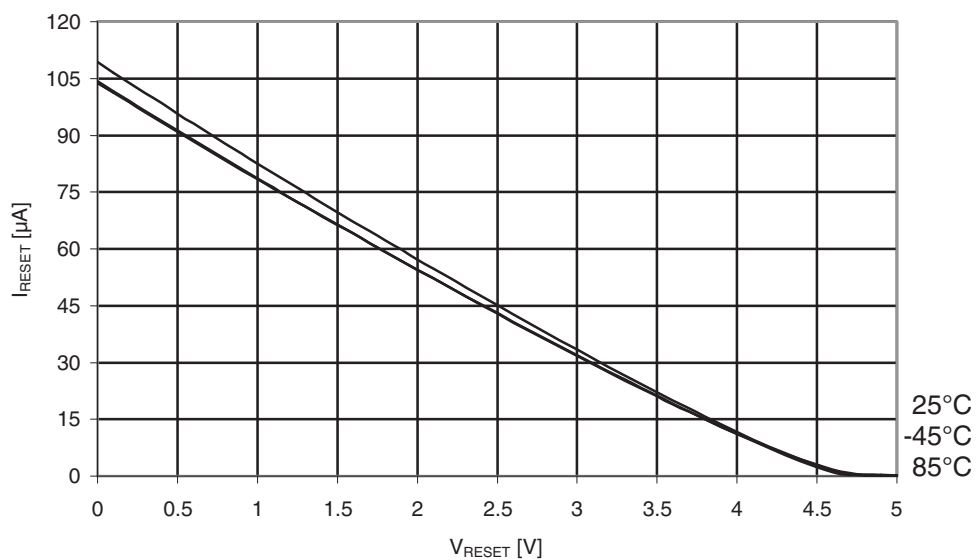
Figure 31-567. ATmega649A: Reset pull-up resistor current vs. reset pin voltage ( V_{CC} = 5V ).
