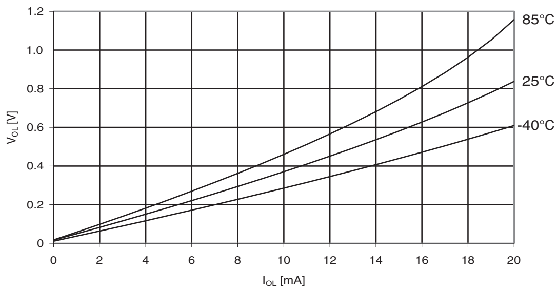
Figure 31-336. Atmel ATmega3290PA: I/O pin output voltage vs. sink current, port B ( V_{CC} = 2.7V ).
