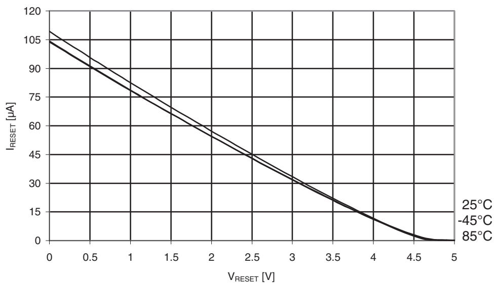
Figure 31-506. ATmega6490A: Reset pull-up resistor current vs. reset pin voltage ( V_{CC} = 5V ).
