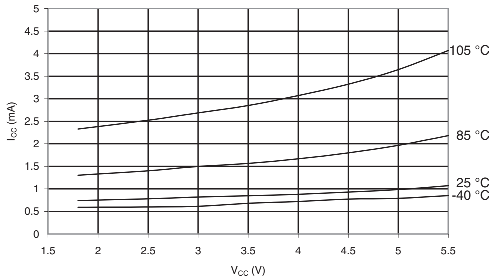
Figure 32-135. ATmega329P-105°C: Standby Supply Current vs. V_{CC} (32kHz Watch Crystal, Watchdog Timer Disabled)
