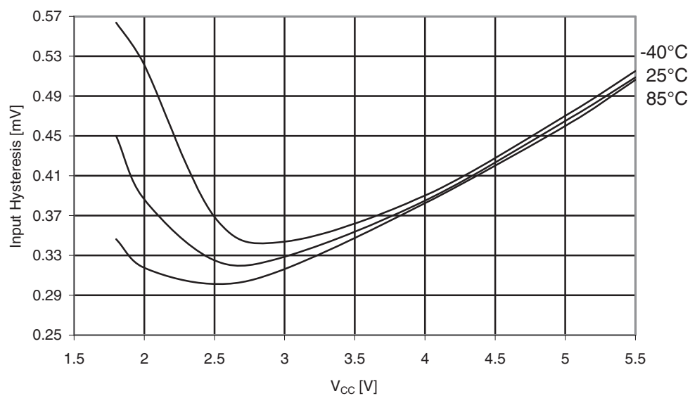
Figure 31-160. ATmega329A: I/O pin Input Hysteresis vs. V_{CC} .
