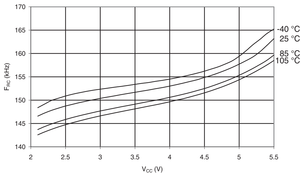
Figure 32-339. ATmega3290PA-105°C: Watchdog Oscillator Frequency vs. V_{CC}
