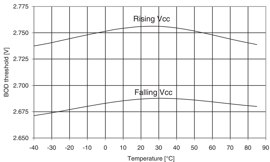
Figure 31-225. Atmel ATmega329PA: BOD Thresholds vs. temperature (BOD level is 2.7V).
