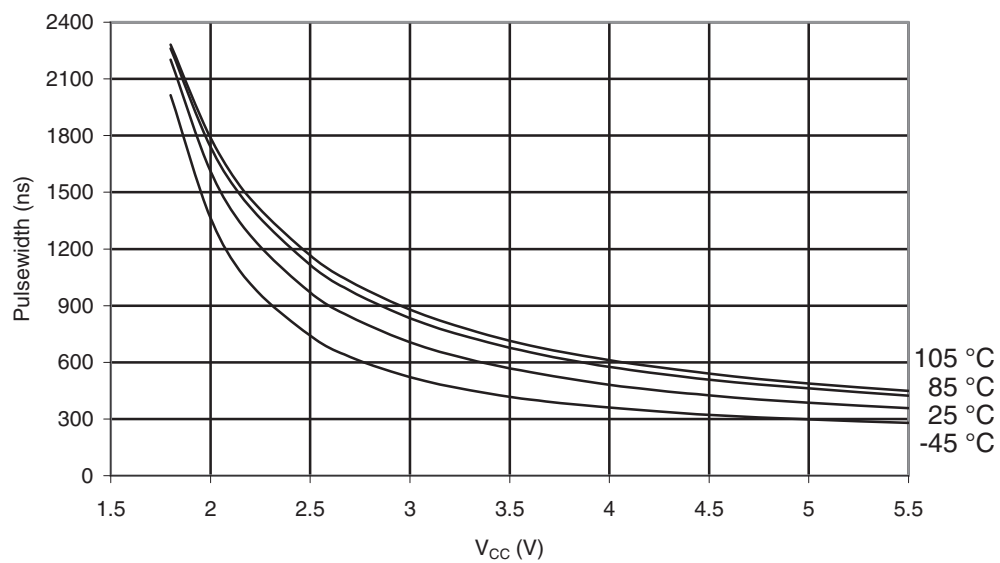
Figure 32-58. ATmega169PA-105°C: Minimum Reset Pulse Width vs. V_{CC}
