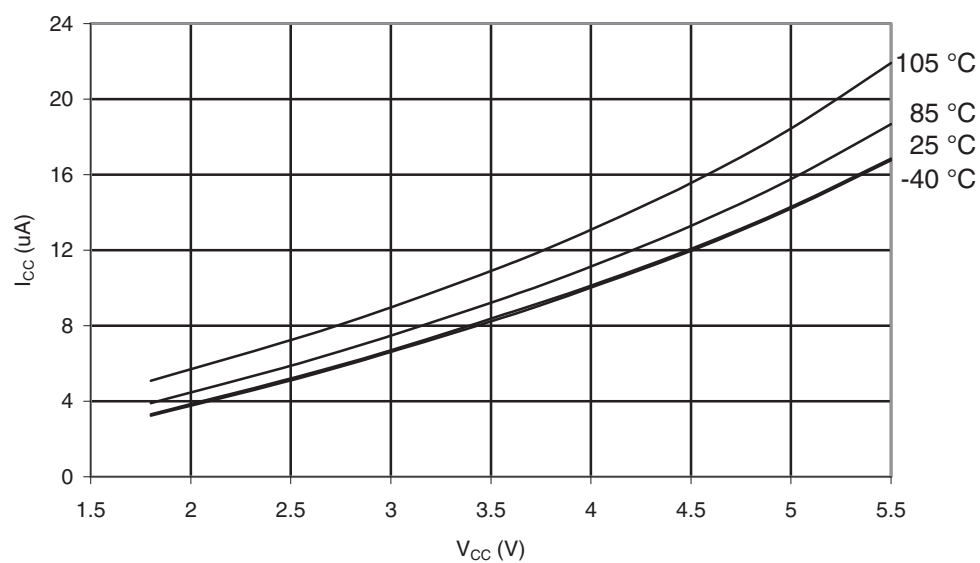
Figure 32-311. ATmega3290PA-105°C: Power-down Supply Current vs. V_{CC} (Watchdog Timer Enabled)
