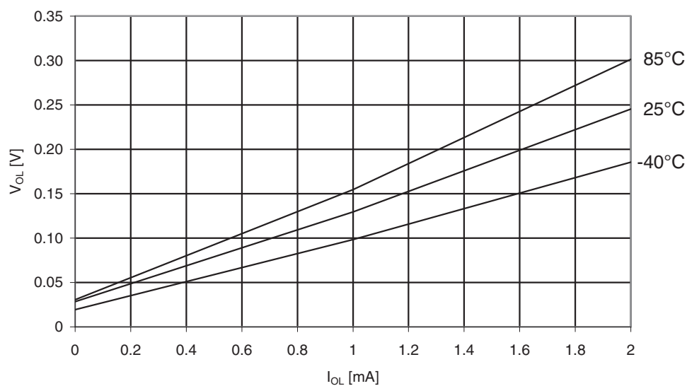
Figure 31-334. Atmel ATmega3290PA: I/O pin output voltage vs. sink current, ports A, C, D, E, F, G ( V_{CC} = 1.8V ).
