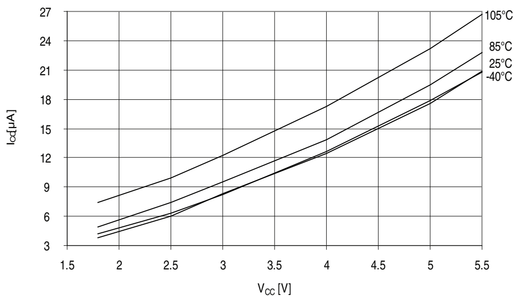
Figure 32-414. ATmega3290PA - 105°C: Reset Current vs. V_{CC} (1 - 20MHz, Excluding Current Through The Reset Pull-up and No Clock)
