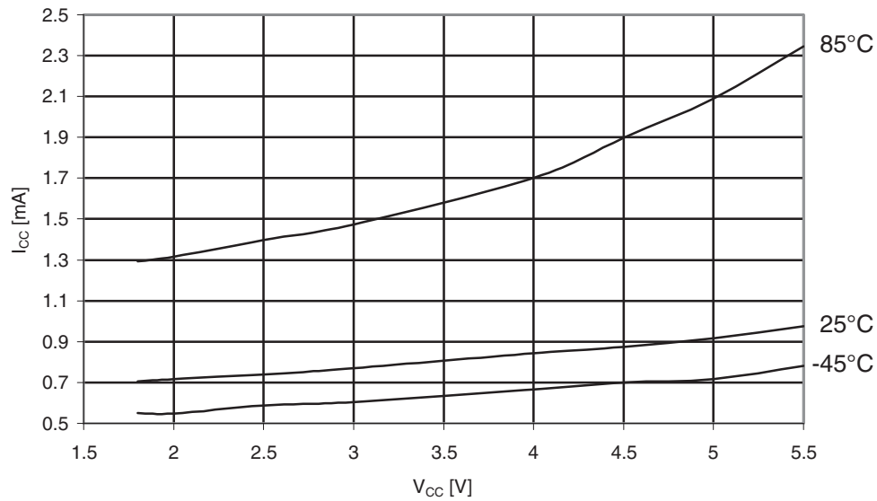
Figure 31-440. Atmel ATmega649P standby supply current vs. V_{CC} (32kHz watch XTAL, Watchdog Timer disabled).
