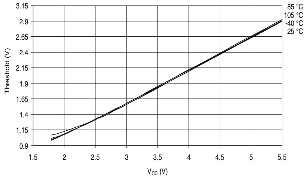
Figure 32-206. ATmega329PA - 105°C: I/O Pin Input Threshold Voltage vs. V_{CC} ( V_{IH} , I/O Pin Read as “1”)
