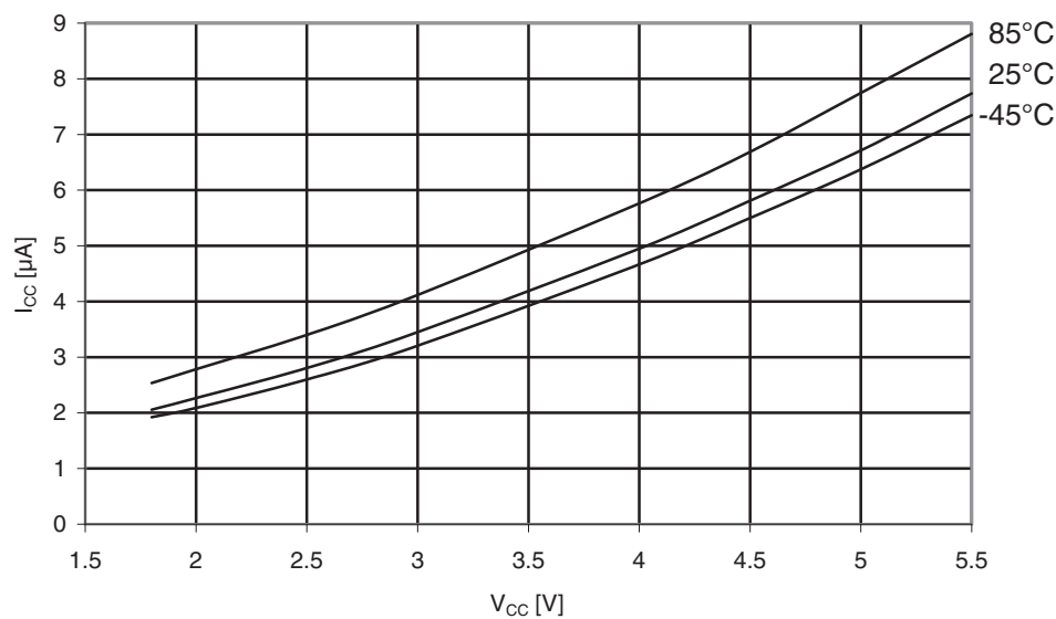
Figure 31-72. ATmega169PA: Idle supply current vs. V_{CC} (32kHz watch XTAL).
