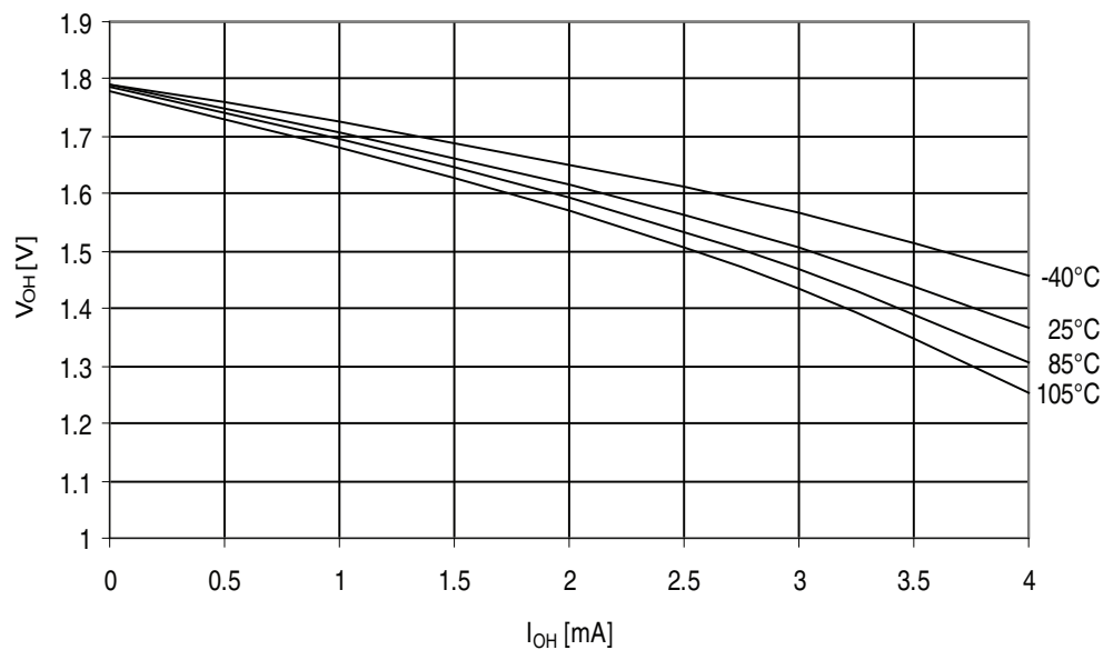
Figure 32-259. ATmega3290A - 105°C: I/O Pin Output Voltage vs. Source Current, Ports A, C, D, E, F, G ( V_{CC} = 1.8V )
