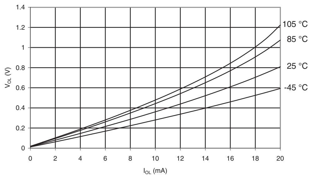
Figure 32-31. ATmega169PA-105°C: I/O Pin Output Voltage vs. Sink Current, Port B ( V_{CC}=2.7V )
