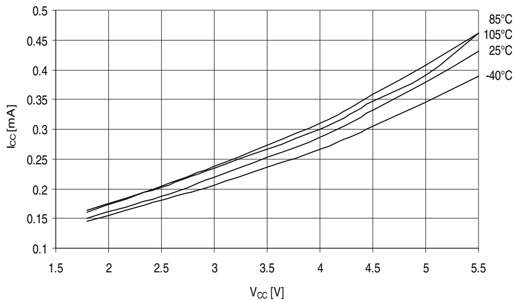
Figure 32-182. ATmega329PA - 105°C: Idle Supply Current vs. V_{CC} (Internal RC Oscillator, 1MHz)
