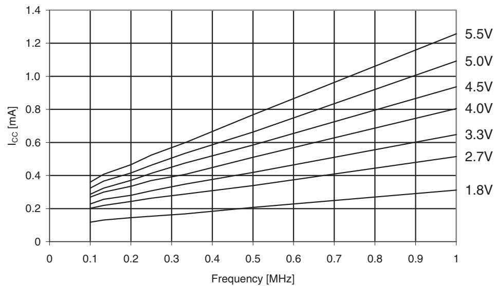
Figure 31-305. ATmega3290PA: Active supply current vs. low frequency (0.1 - 1.0MHz).
