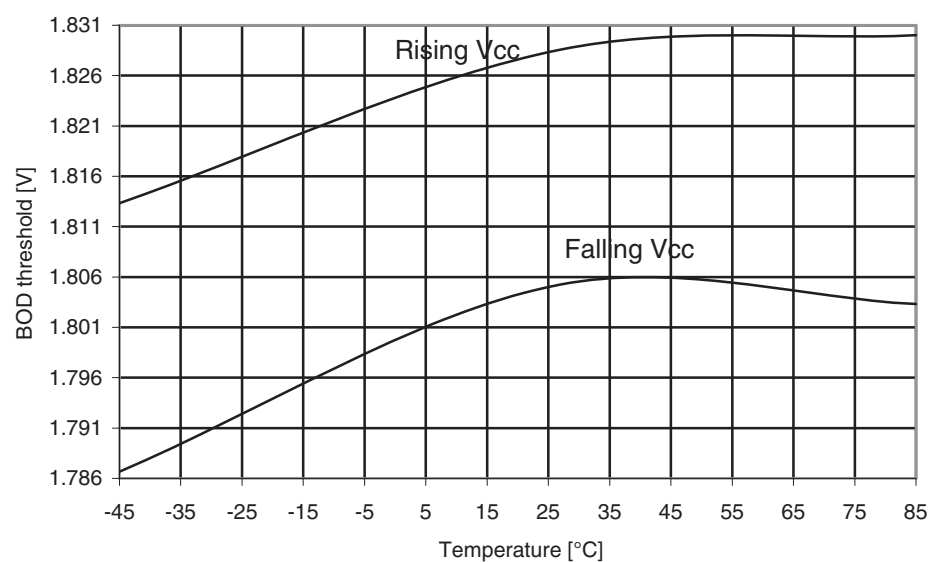
Figure 31-104. ATmega169PA: BOD Thresholds vs. temperature (BOD level is 1.8V).
