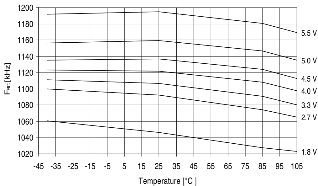
Figure 32-280. ATmega3290A - 105°C: Watchdog Oscillator Frequency vs. Temperature
