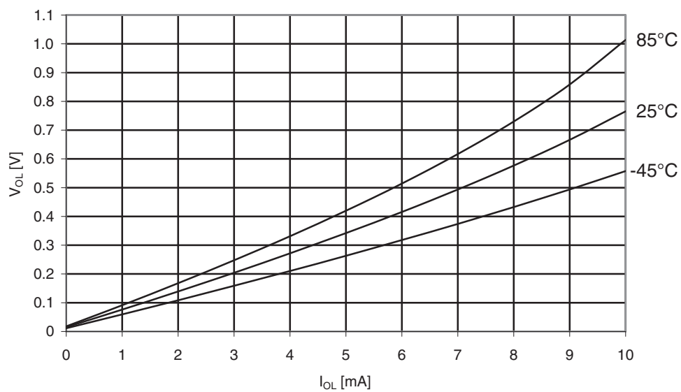
Figure 31-28. ATmega169A: I/O pin output voltage vs. sink current, ports A, C, D, E, F, G ( V_{CC} = 5V ).
