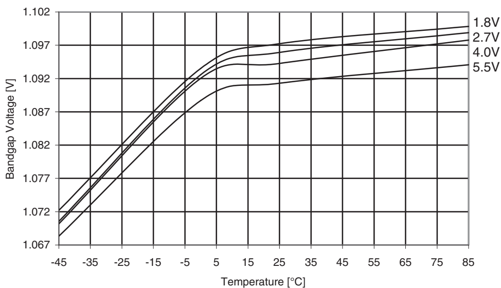
Figure 31-106. ATmega169PA: Bandgap voltage vs. temperature.
