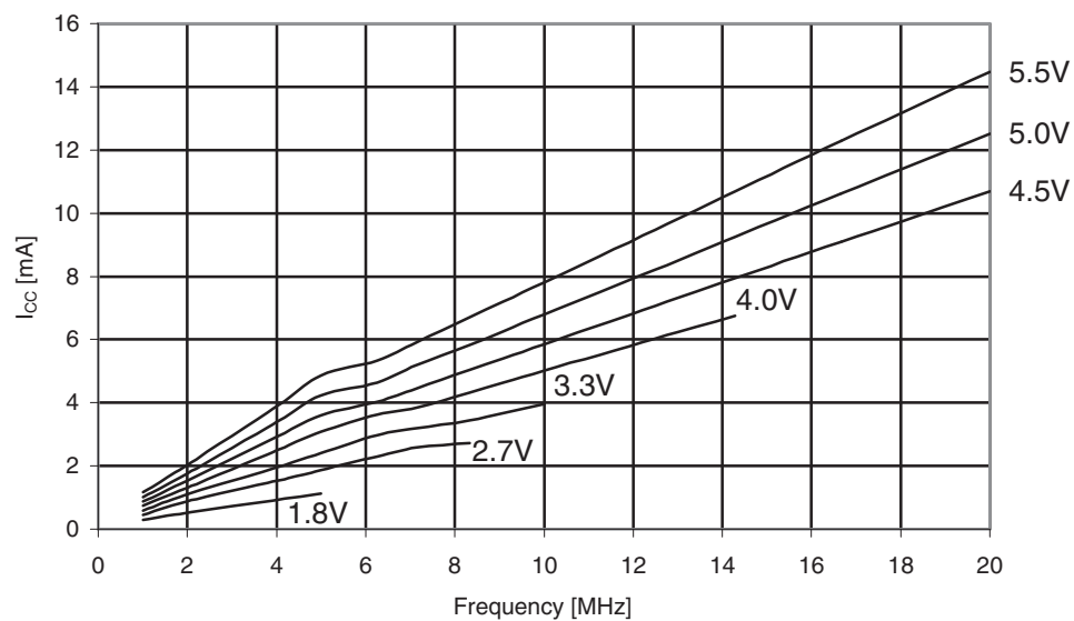
Figure 31-371. Atmel ATmega649A: Idle supply current vs. frequency (1 - 20MHz).
