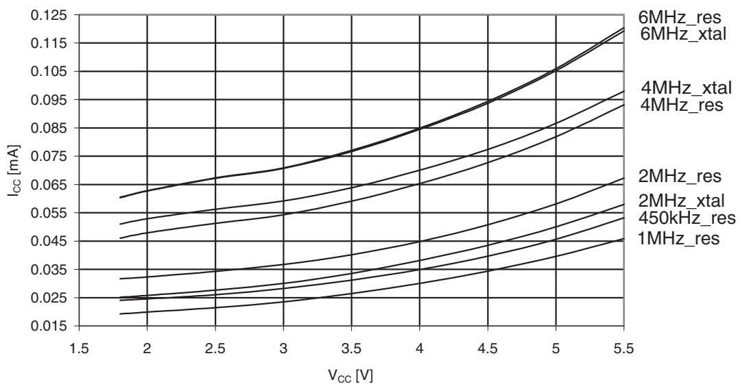
Figure 31-563. ATmega6490P: Standby supply current vs. V_{CC} (XTAL and resonator, Watchdog Timer disabled).
