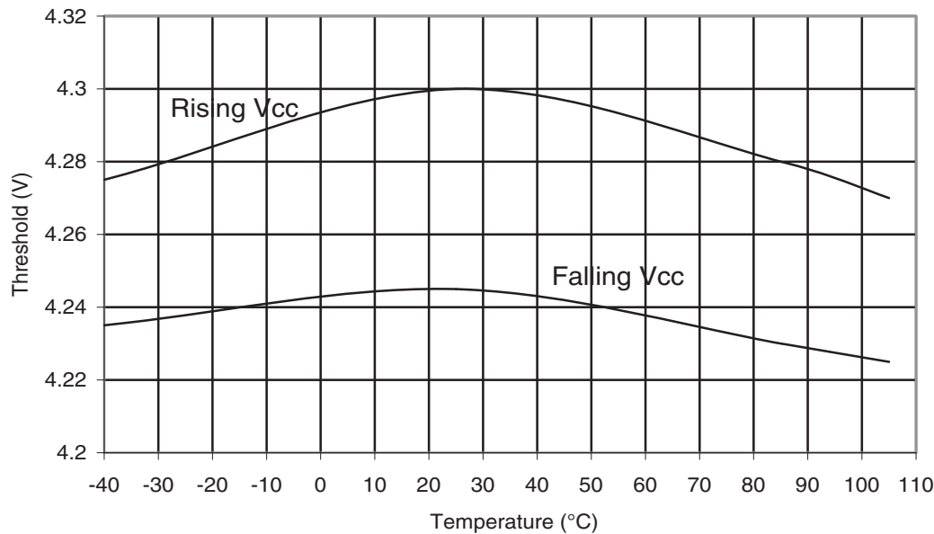
Figure 32-156. ATmega329P-105°C: BOD Thresholds vs. Temperature (BOD Level is 4.3V)
