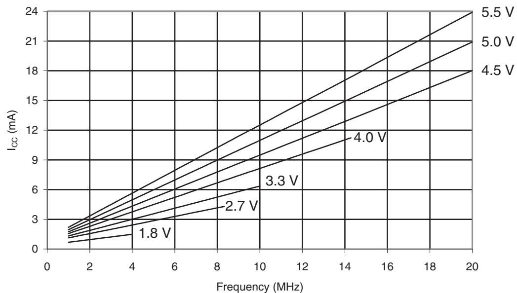
Figure 32-301. ATmega3290PA-105°C: Active Supply Current vs. Frequency (1 - 20MHz)
