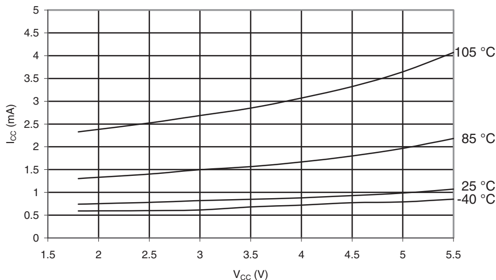
Figure 32-313. ATmega3290PA-105°C: Standby Supply Current vs. V_{CC} (32kHz Watch Crystal, Watchdog Timer Disabled)
