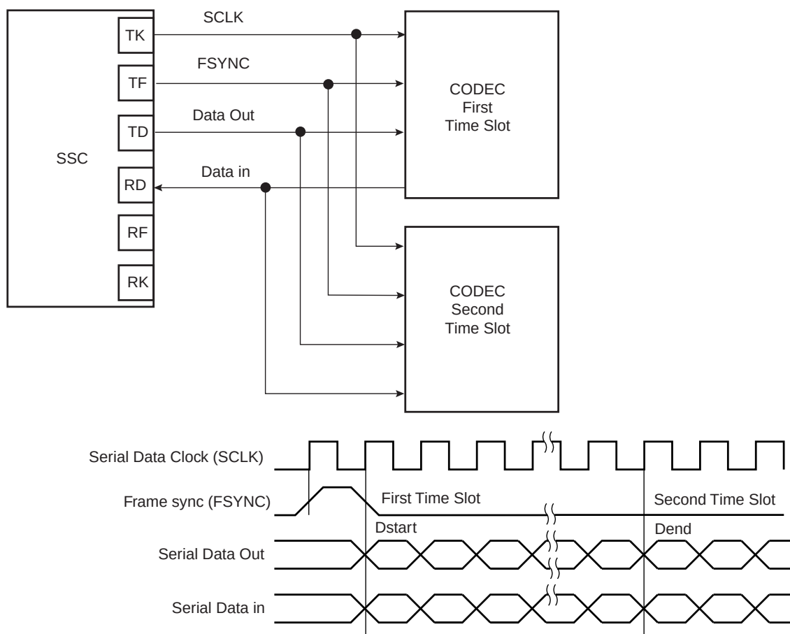
Figure 32-21. Time Slot Application Block Diagram
