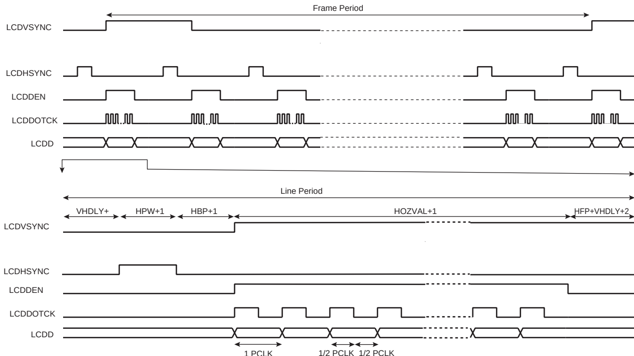
Figure 47-5. STN Panel Timing, CLKMOD 0
