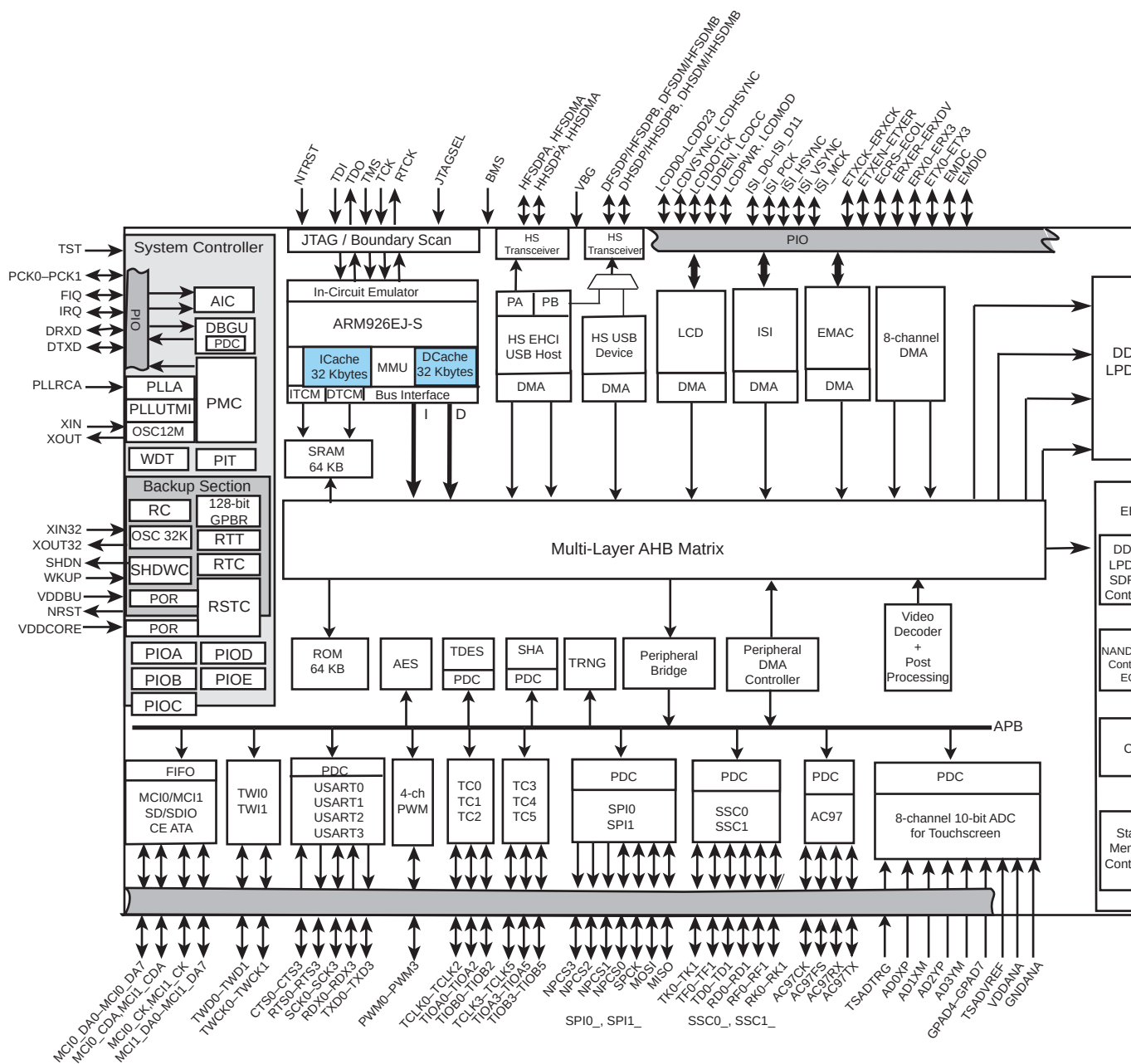
Figure 1-1. SAM9M11 Block Diagram
