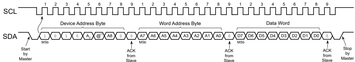
Figure 7-1. Byte Write
