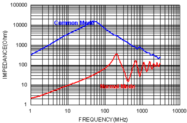
ACT4532L-510-2P-TF
