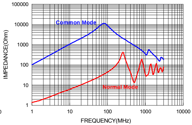
ACT4532L-220-2P-TF
