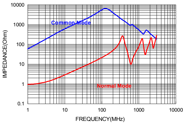
ACT4532L-110-2P-TF
