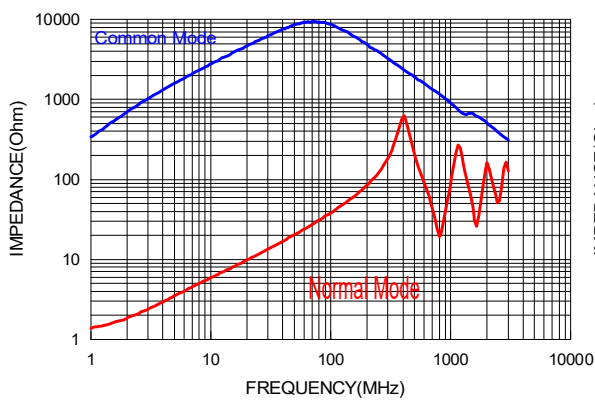
ACT3225L-510-2P-TF
