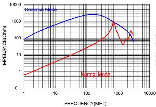
ACT3225L-110T-2P-TF
