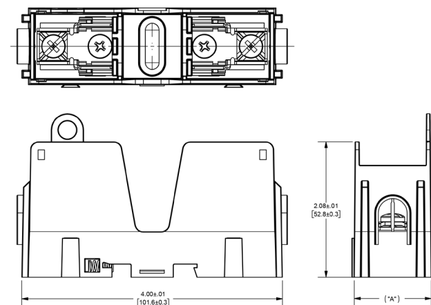
Figure 3: Class J 30A - Pressure Plate
