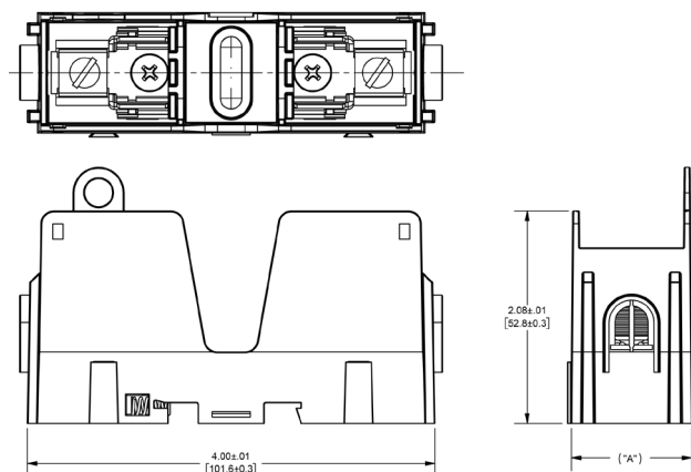
Figure 1: Class J 30A - Box Connector
