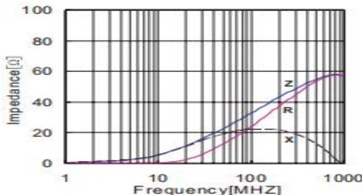
产品特性曲线图：Product Characteristic Curve
