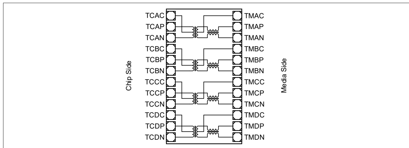
Figure 22 Schematic of an Ethernet Transformer Device
