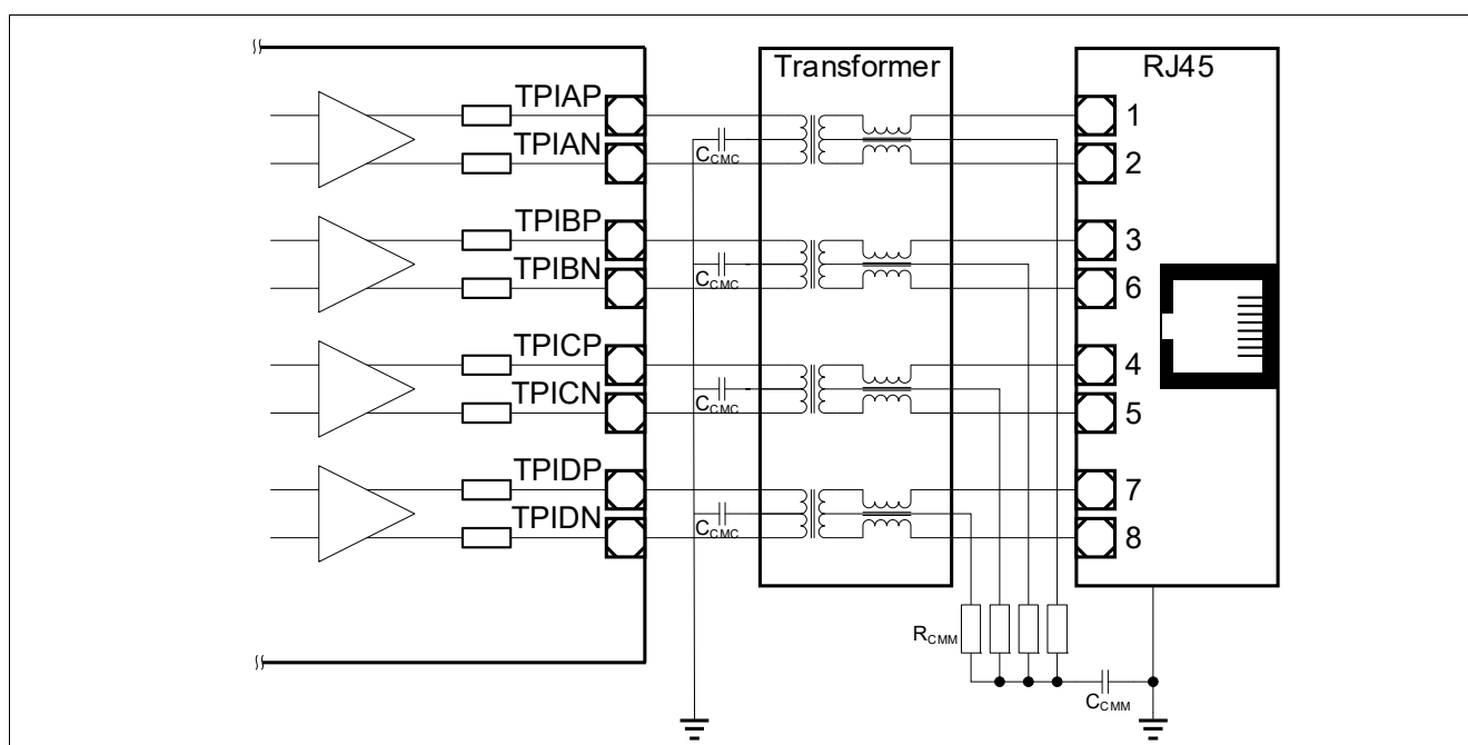
Figure 5 Twisted-Pair Interface of MxL86211C Including Transformer and RJ45 Plug
