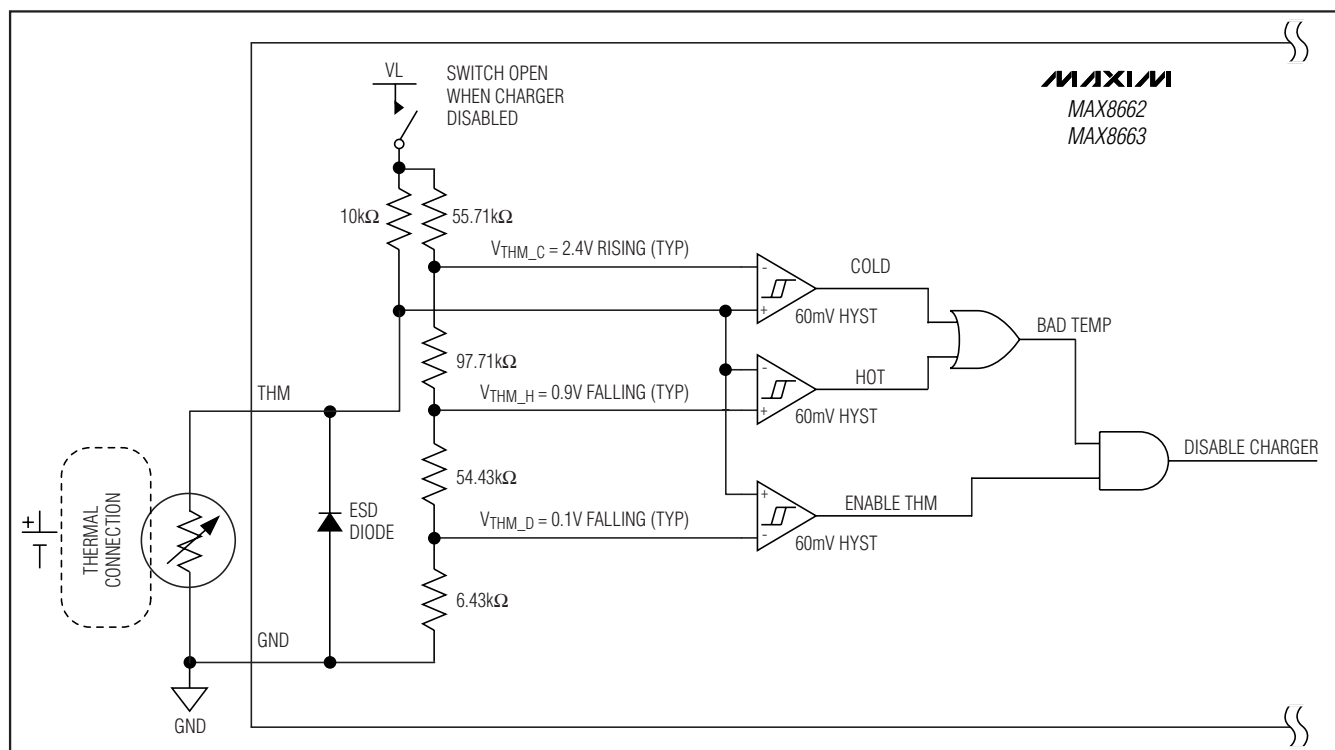
Figure 6. Thermistor Input
