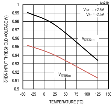
SHDN INPUT THRESHOLD VOLTAGE vs. TEMPERATURE
