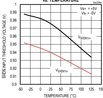
SHDN INPUT THRESHOLD VOLTAGE vs. TEMPERATURE
