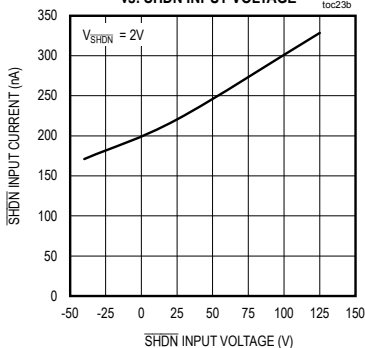
SHDN INPUT CURRENT vs. SHDN INPUT VOLTAGE
