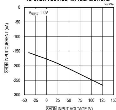
SHDN INPUT CURRENT vs. SHDN VOLTAGE vs. TEMPERATURE
