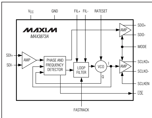
Figure 5. Functional Diagram
