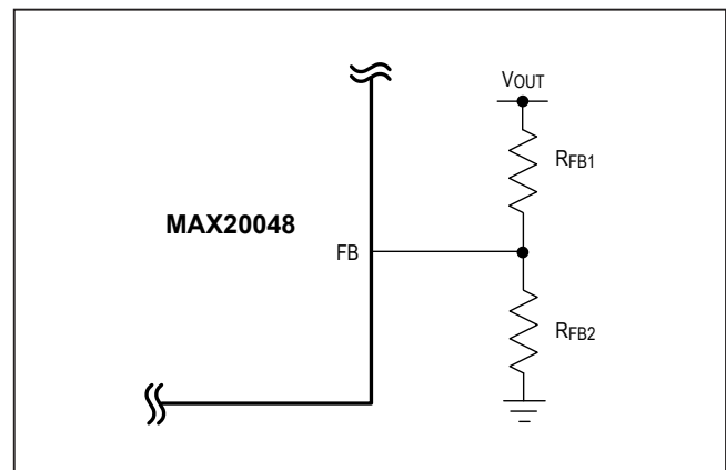
Figure 1. Setting the Output Voltage for the MAX20048
