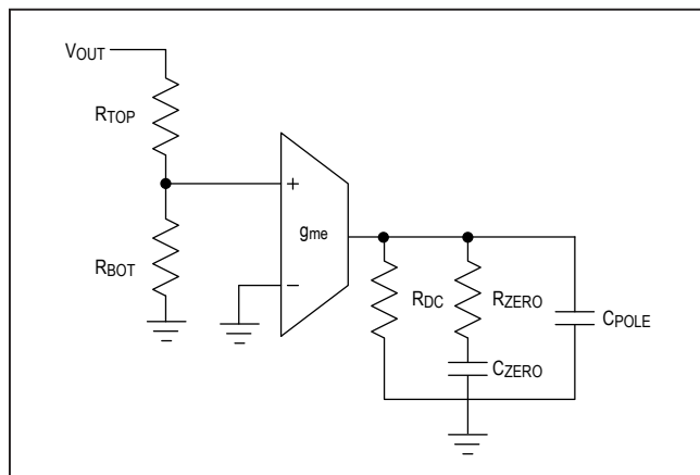
Figure 2. Setting the Output Voltage for the MAX20048.
