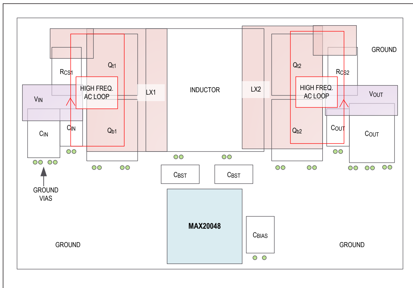
Figure 3. Recommended PCB Layout for the MAX20048.
