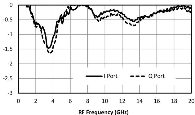
Downconversion Conversion Loss Compression (dB) 17 dBm LO Power, 5 dBm RF Power
