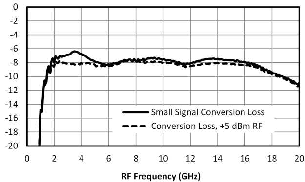
Downconversion Conversion Loss Compression (dB) 17 dBm LO Power, 5 dBm RF Power
