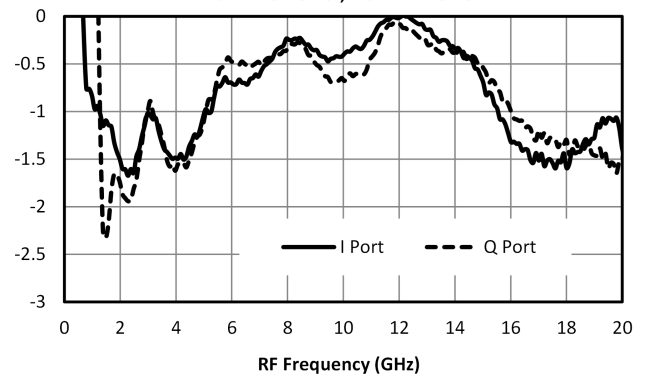
Upconversion Conversion Loss Compression (dB) 17 dBm LO Power, 2 dBm IF Power
