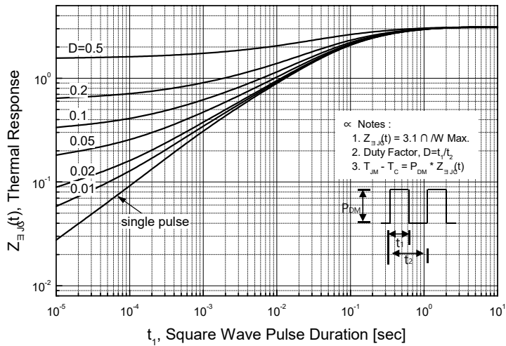
Figure 11-2. Transient Thermal Response Curve for SLF10N70C
