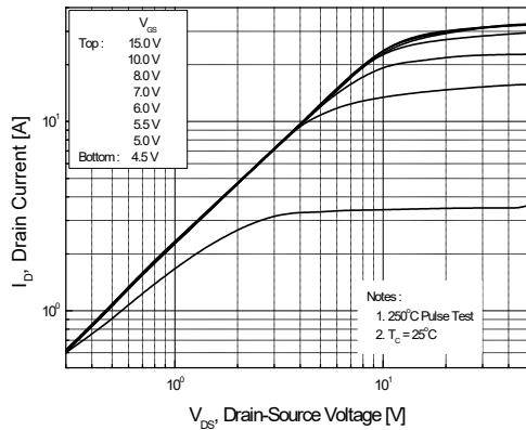
Figure 1. On-Region Characteristics
