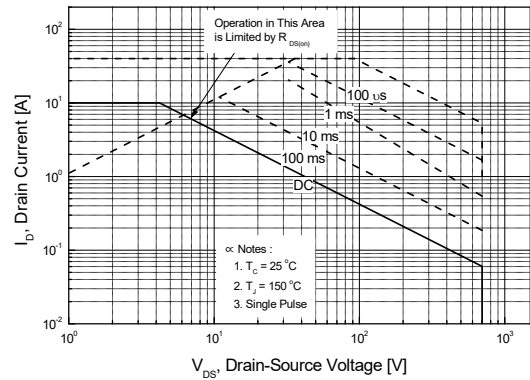
Figure 9-2. Maximum Safe Operating Area for SLF10N70C
