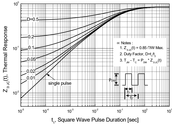
Figure 11-1. Transient Thermal Response Curve for SLP10N70C
