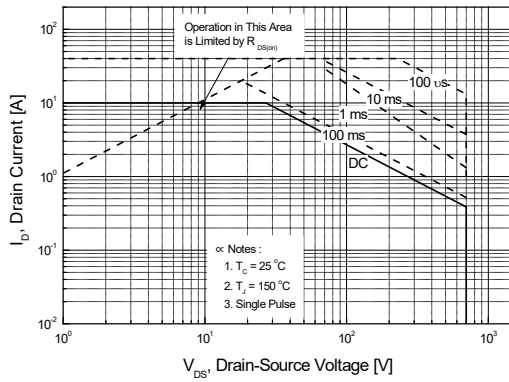
Figure 9-1. Maximum Safe Operating Area for SLP10N70C
