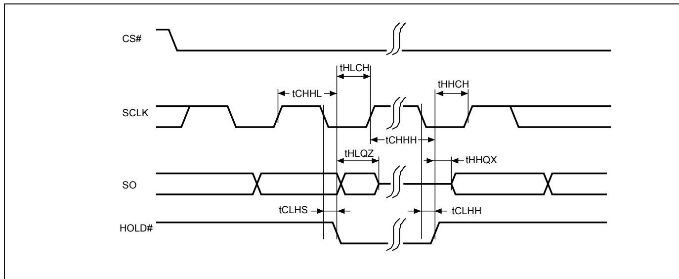
Figure 9. Hold Timing
