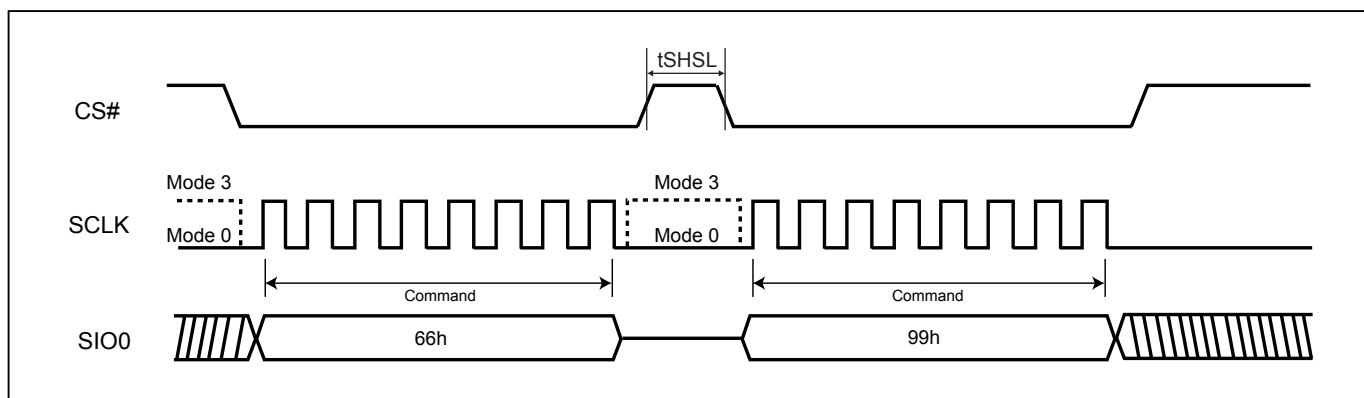
Figure 38. Reset Sequence
