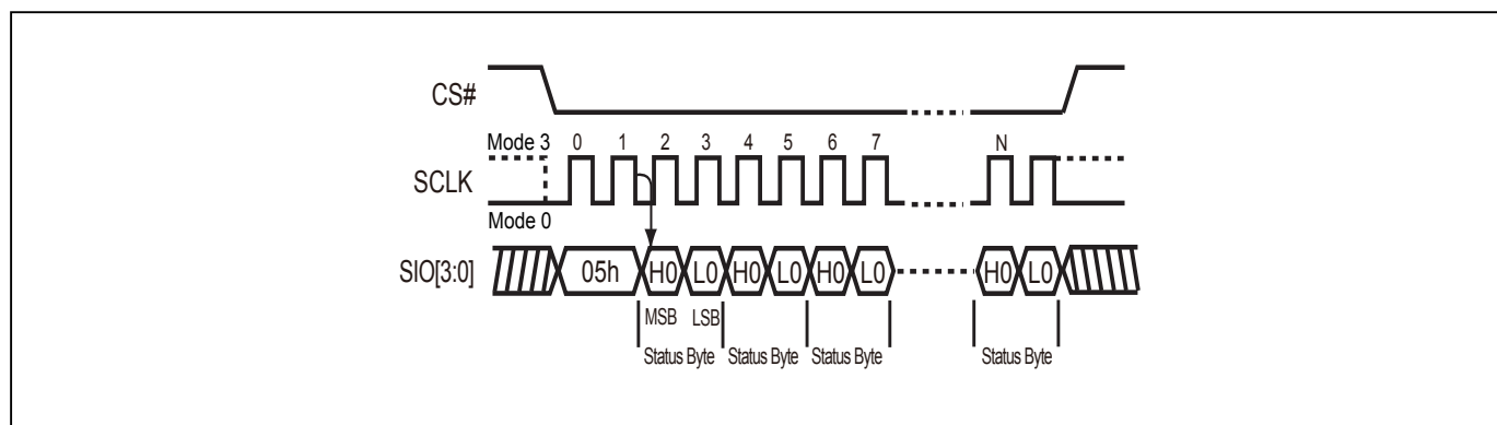
Figure 26. Read Status Register (RDSR) Sequence (QPI Mode)
