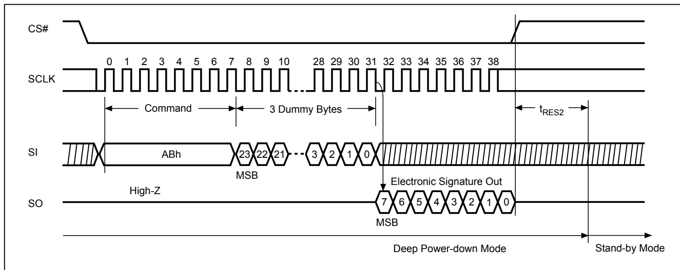
Figure 27. Release from Deep Power-down and Read Electronic Signature (RES) Sequence (Command ABh)
