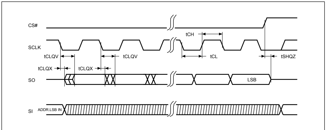
Figure 7. Output Timing
