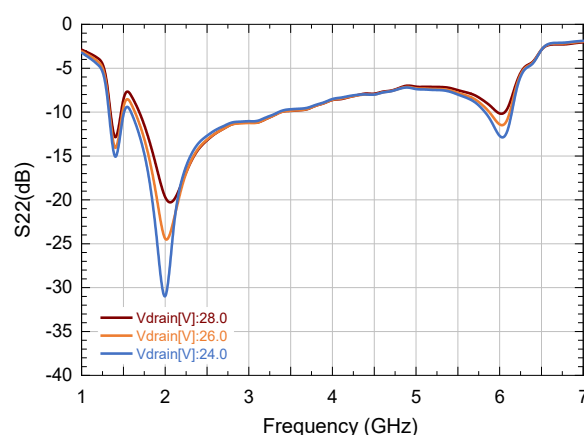
S22 Voltage vs. Frequency @ 25°C
