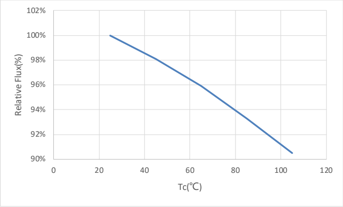
Case Temperature vs. Relative Luminous flux (IF=45mA)
