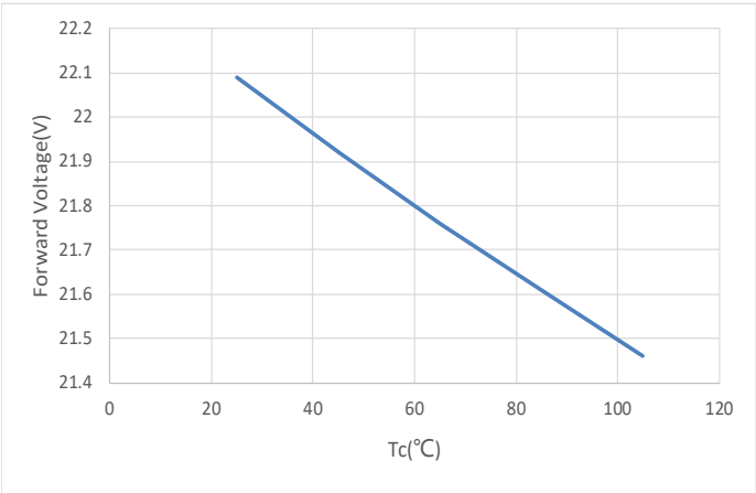
Case Temperature vs. Forward Voltage (IF=45mA)
