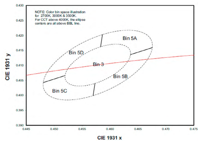
Figure 7. Color space definition for LUXEON HL4X.
