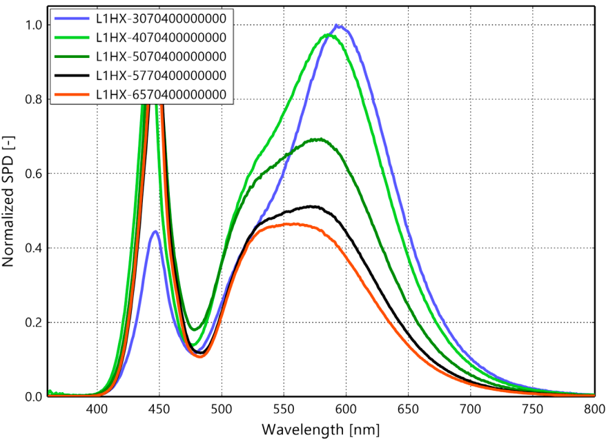
Figure 1a. Typical normalized power vs. wavelength for LUXEON HL4X 70 CRI at 1400mA, T_j=85^\circ\text{C} .
