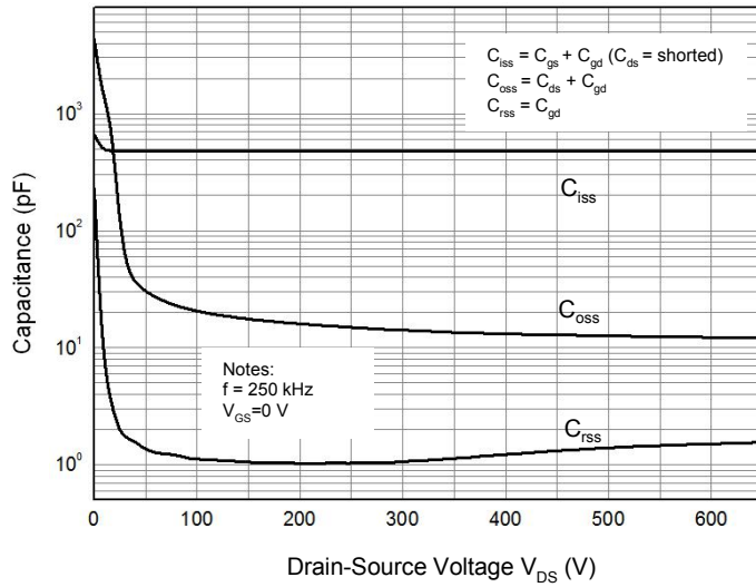
Figure 7. Capacitance Characteristics
