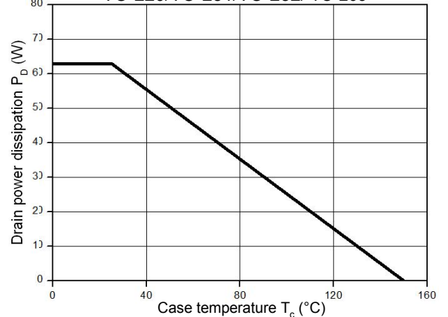
Figure 10.2 Power Dissipation vs. Temperature TO-220/TO-251/TO-252/ TO-263
