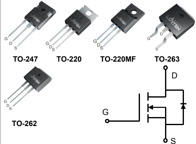
N-Channel MOSFET
