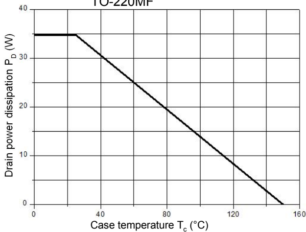
Figure 10.1 Power Dissipation vs. Temperature TO-220MF
