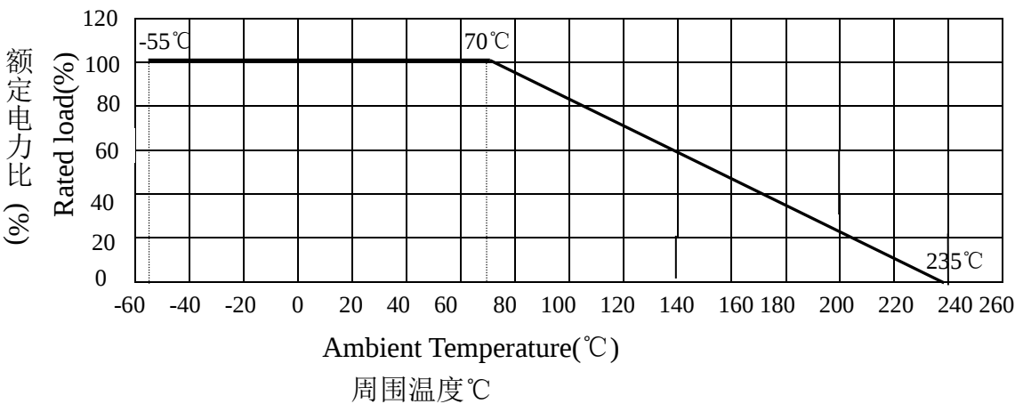
图一 电力递减曲线 Figure 1 Power derating curve
