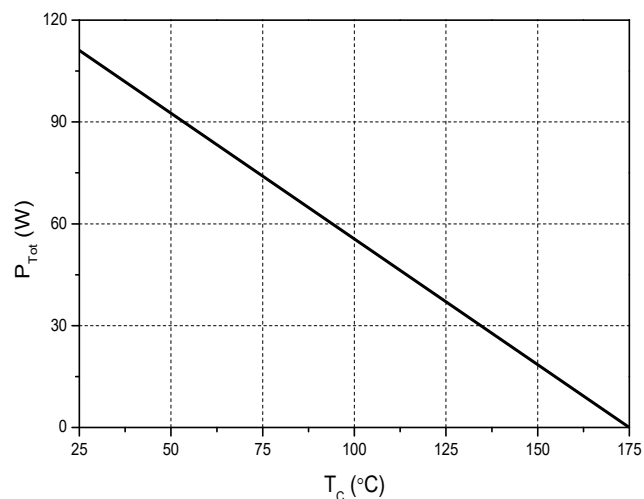
Figure 6. Power Derating
