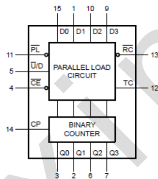
Figure 2. Functional diagram
