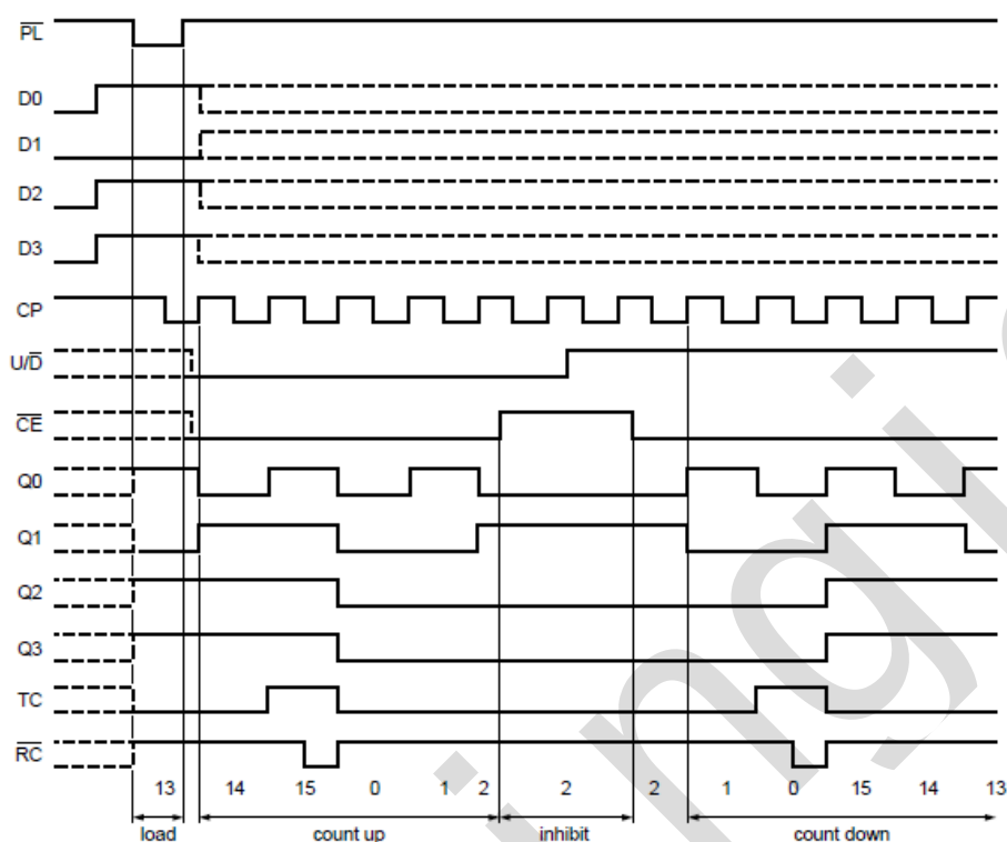
Figure 7. Typical timing sequence
