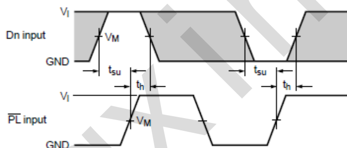
Figure 16. The parallel load input (PL) to data input (Dn) set-up and hold times
