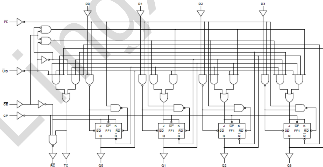
Figure 3. Logic diagram
