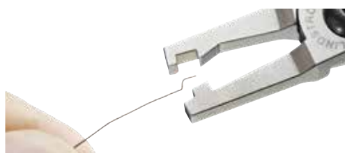
RX331A-31 bend and cut pliers create precise two-angle bend and cuts lead the same length every time.
