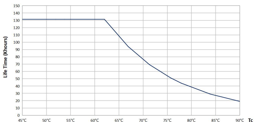
Lifetime Curve
