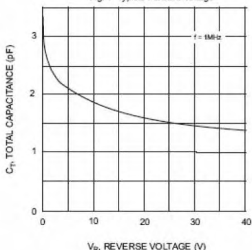
Fig. 3 Typical Capacitance
