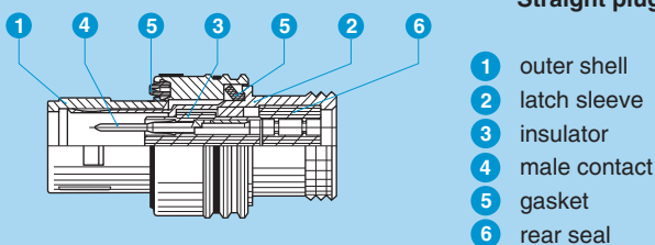
Straight plug
