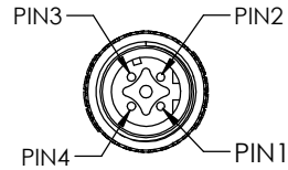
"P1" M12 SHIELD MALE 4 POSITION D-CODED
