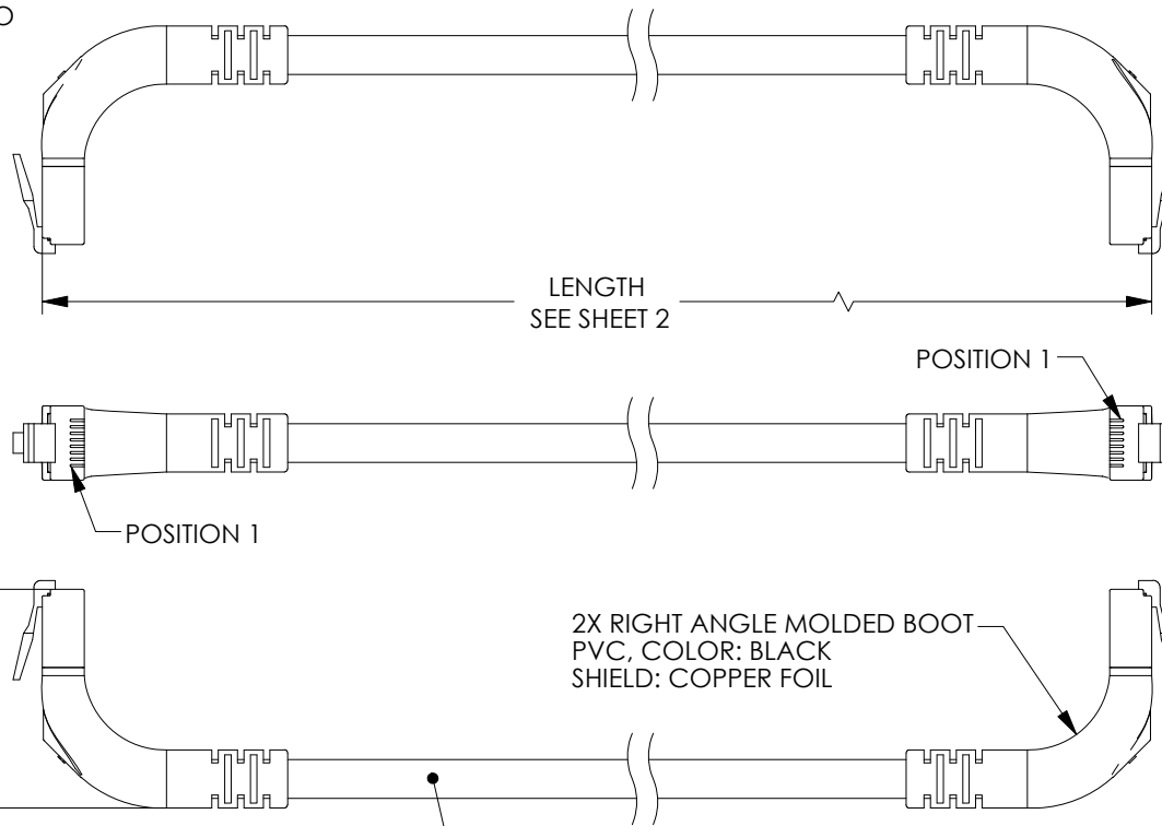
P1 SHIELDED RJ45 MODULAR PLUG GOLD PLATED CONTACTS (8P8C)
