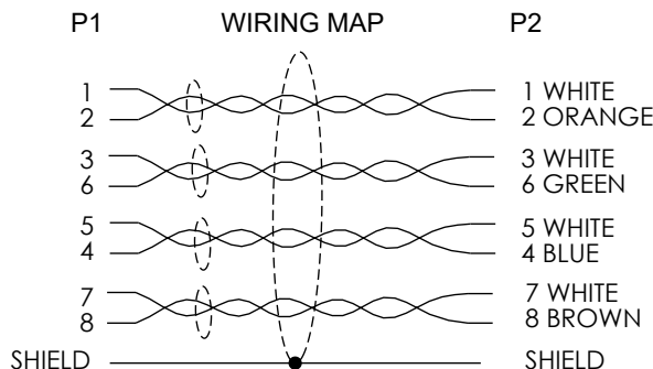
2X RJ45 SHIELDED PLUG GOLD PLATED CONTACTS
