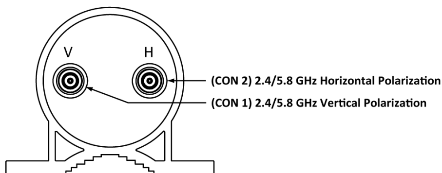
BOTTOM VIEW
