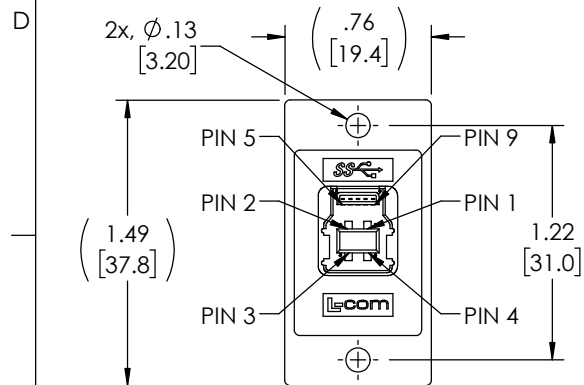
"J1" USB 3.0 TYPE "B" FEMALE CONNECTOR 30u" GOLD PLATED CONTACTS NICKEL PLATED SHELL
