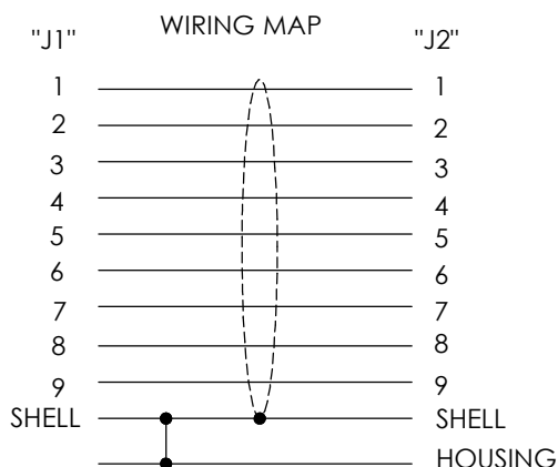
"J1" USB 3.0 TYPE "A" FEMALE CONNECTOR 30u" GOLD PLATED CONTACTS NICKEL PLATED SHELL
