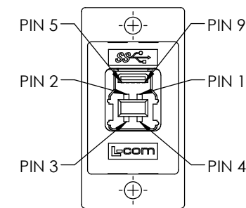
"J2" USB 3.0 TYPE "B" FEMALE CONNECTOR 30u" GOLD PLATED CONTACTS NICKEL PLATED SHELL
