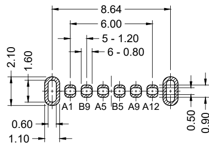
Recommended PCB Layout Tolerance: \pm 0.05 (Top View)
