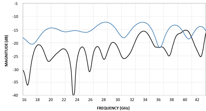
Return Loss
