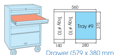
Drawer (579 x 380 mm)
