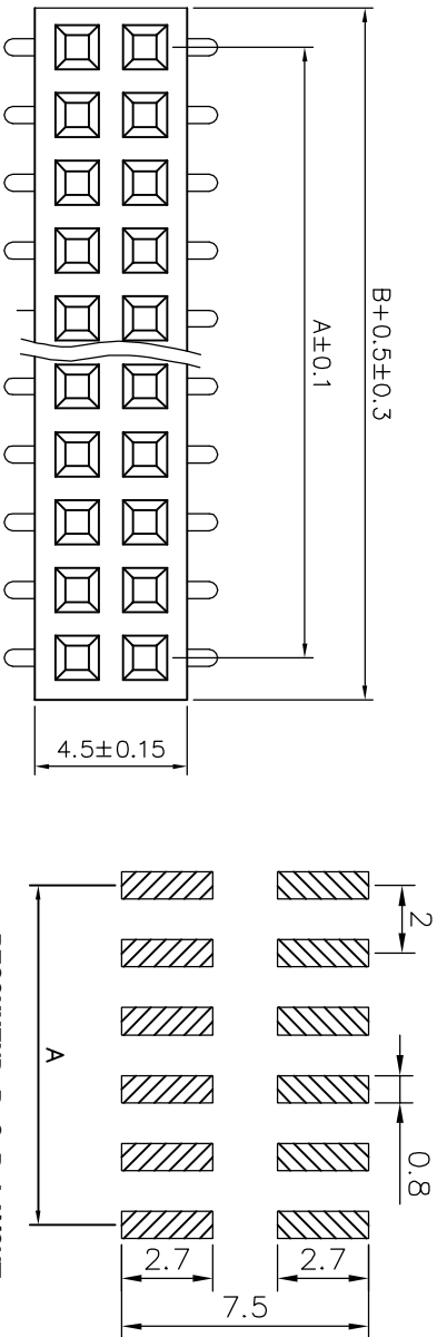
RECOMMEND P.C.B LAYOUT PCB TOLERANCE: ±0.05 (TOP VIEW)
