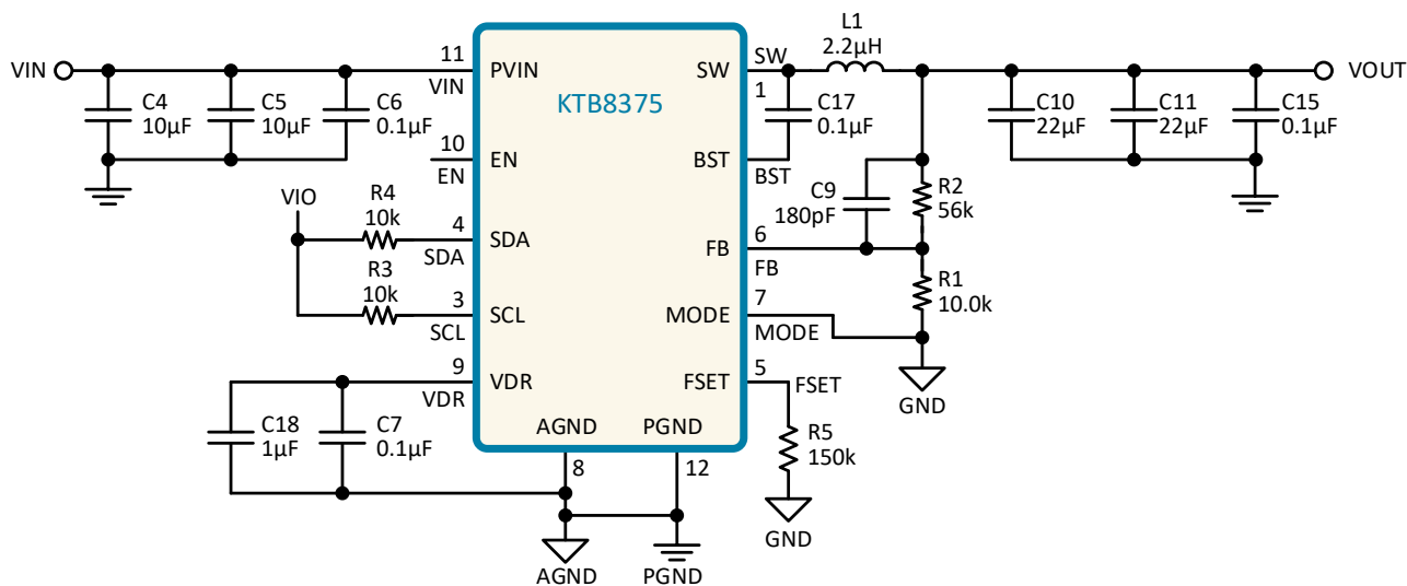
Figure 3. Typical Application Schematic
