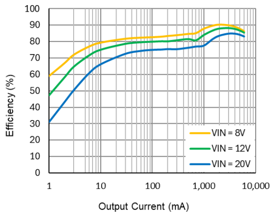
Efficiency vs. Output Current (VOUT = 1.0V) L = 1.0\mu\text{H} , f_{sw} = 500\text{kHz} , Auto-Skip mode
