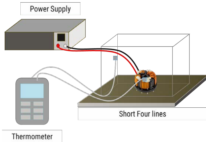
Figure 1 - Measurement system
