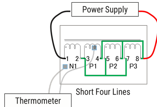
Figure 2 - Schematics
