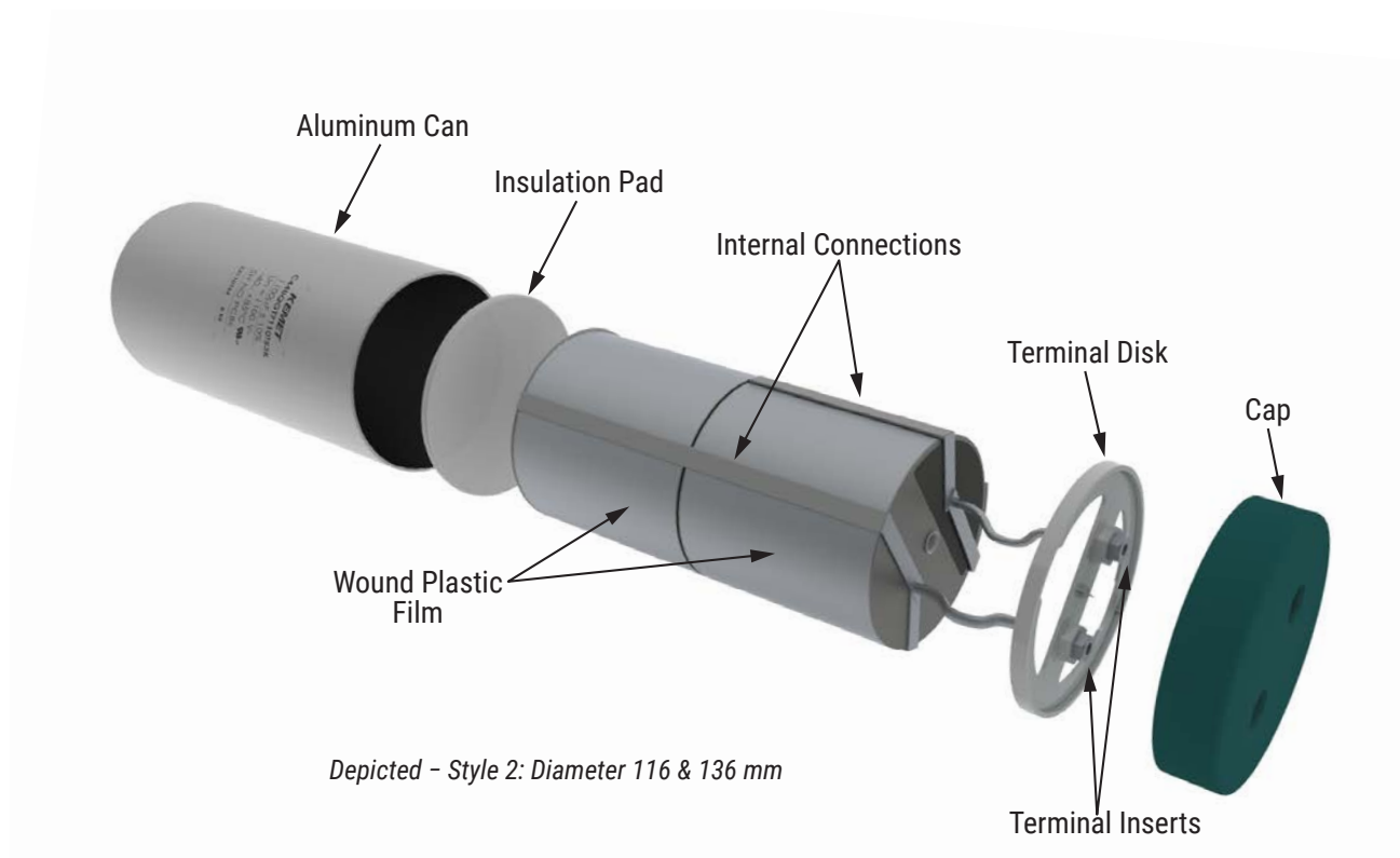
Style 2 Diameter 116 & 136 mm
