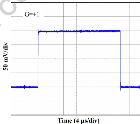
Fig. 11 Small-Signal Step Response at 5V
