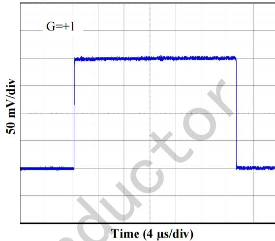
Fig. 9 Small-Signal Step Response at 2.7V
