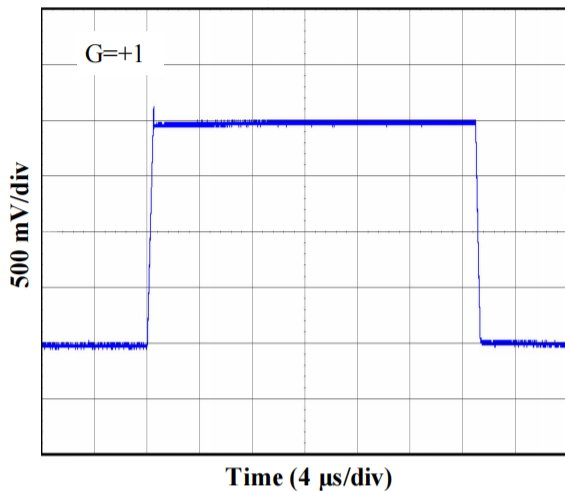
Fig. 8 Large-Signal Step Response at 2.7V
