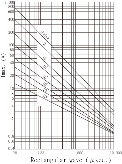
PULSE LIFETIME RATINGS- 5mm 05U180M~05U680K
