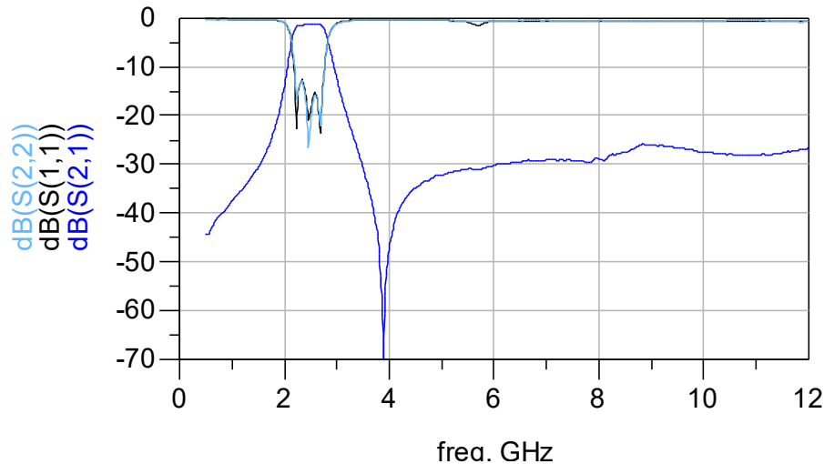
Insertion loss, Return Loss & Harmonic Attenuation
