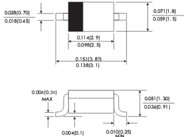
SOD-123
